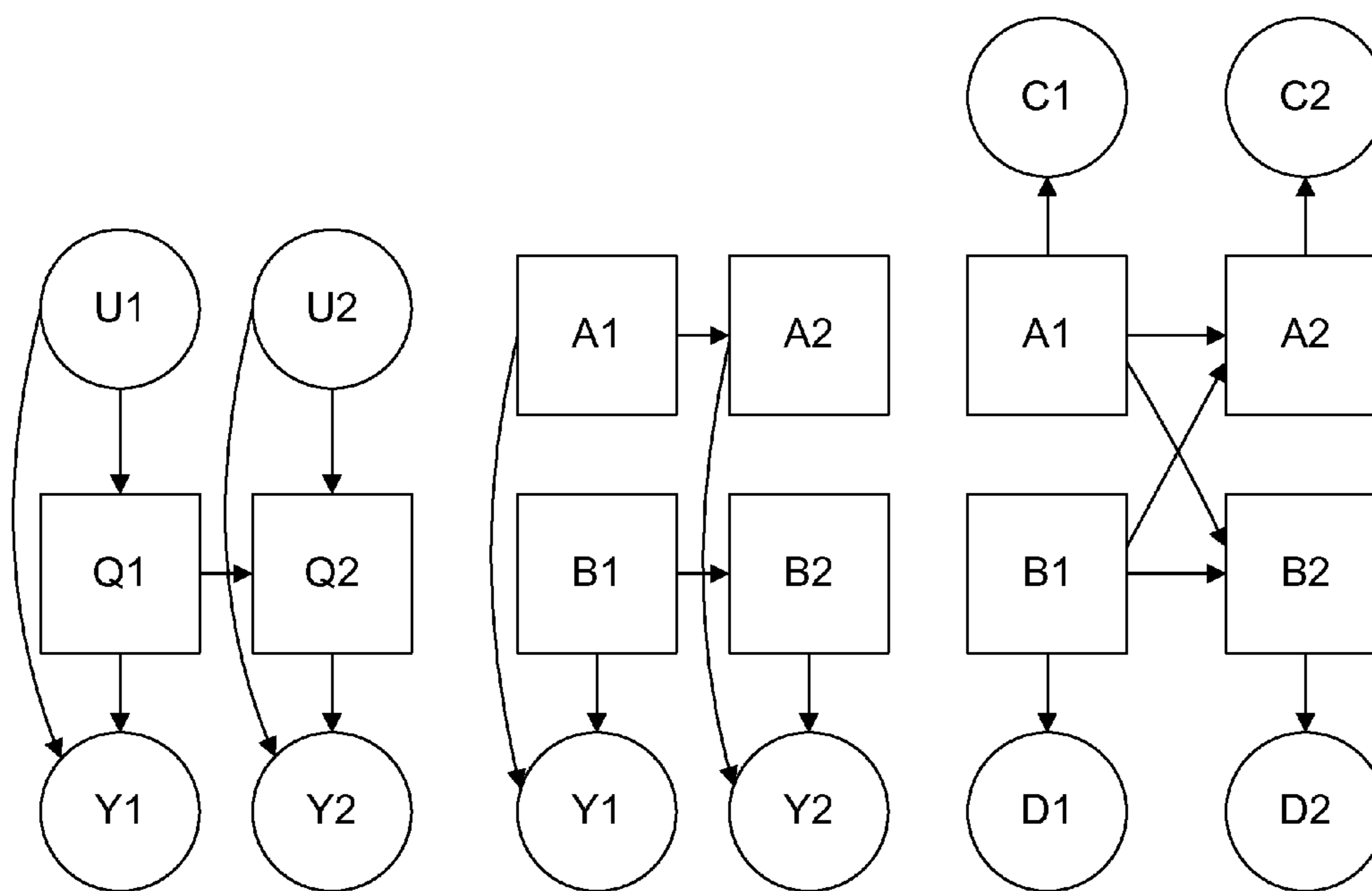
Input-output HMM
