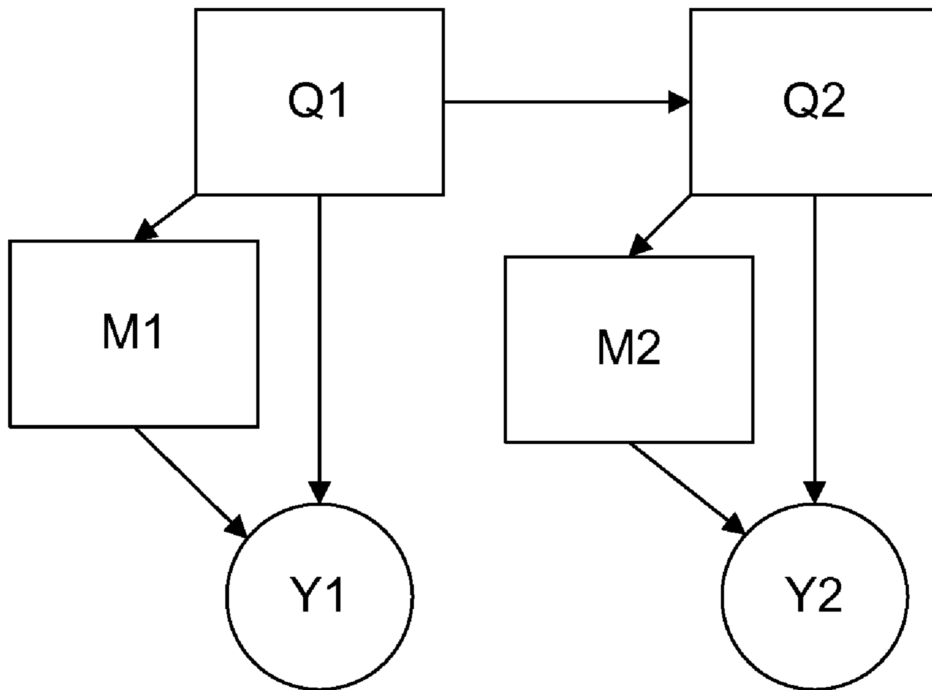
HMM with mixture of Gaussians output
