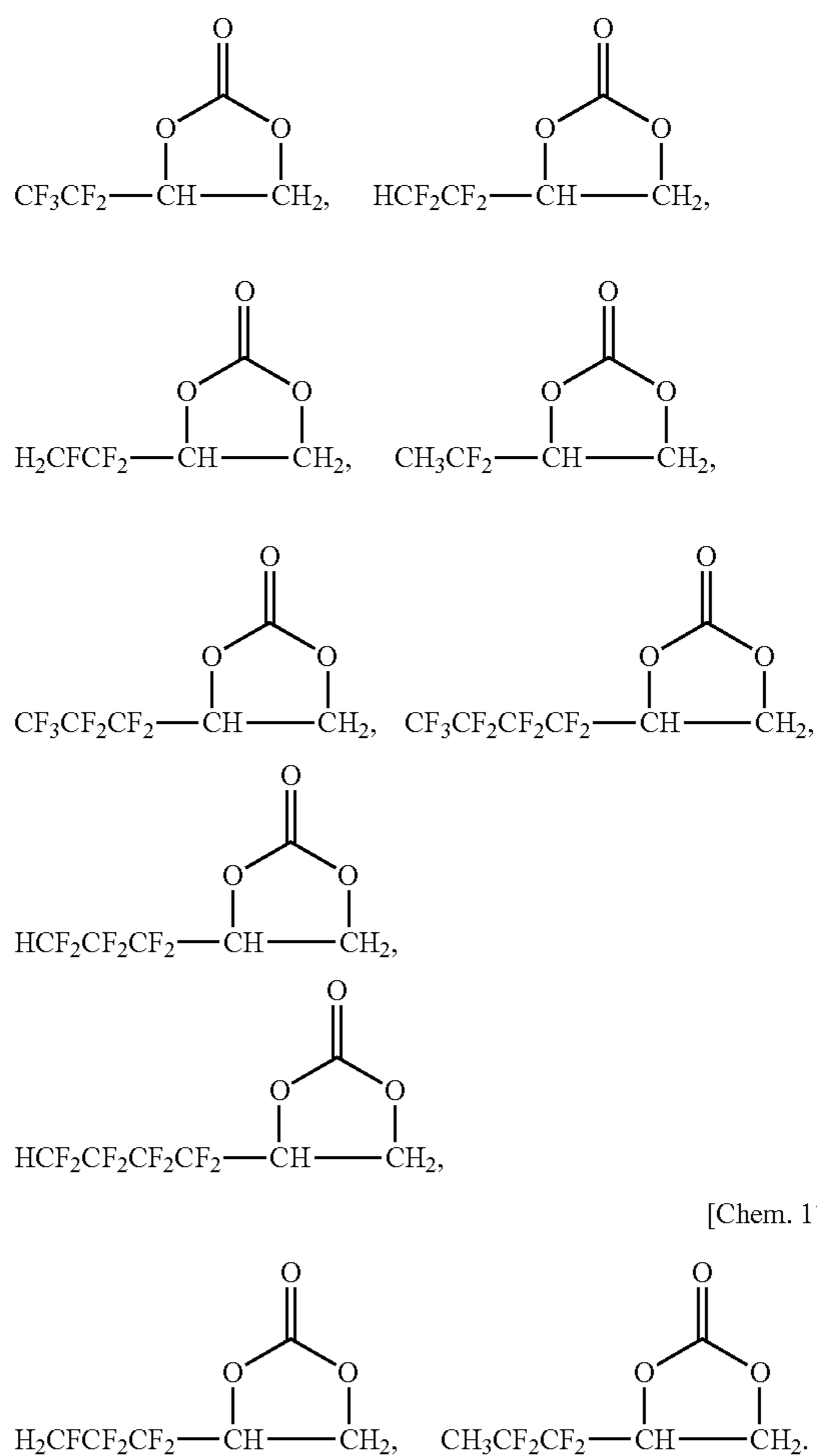
[Chem. 16.]
