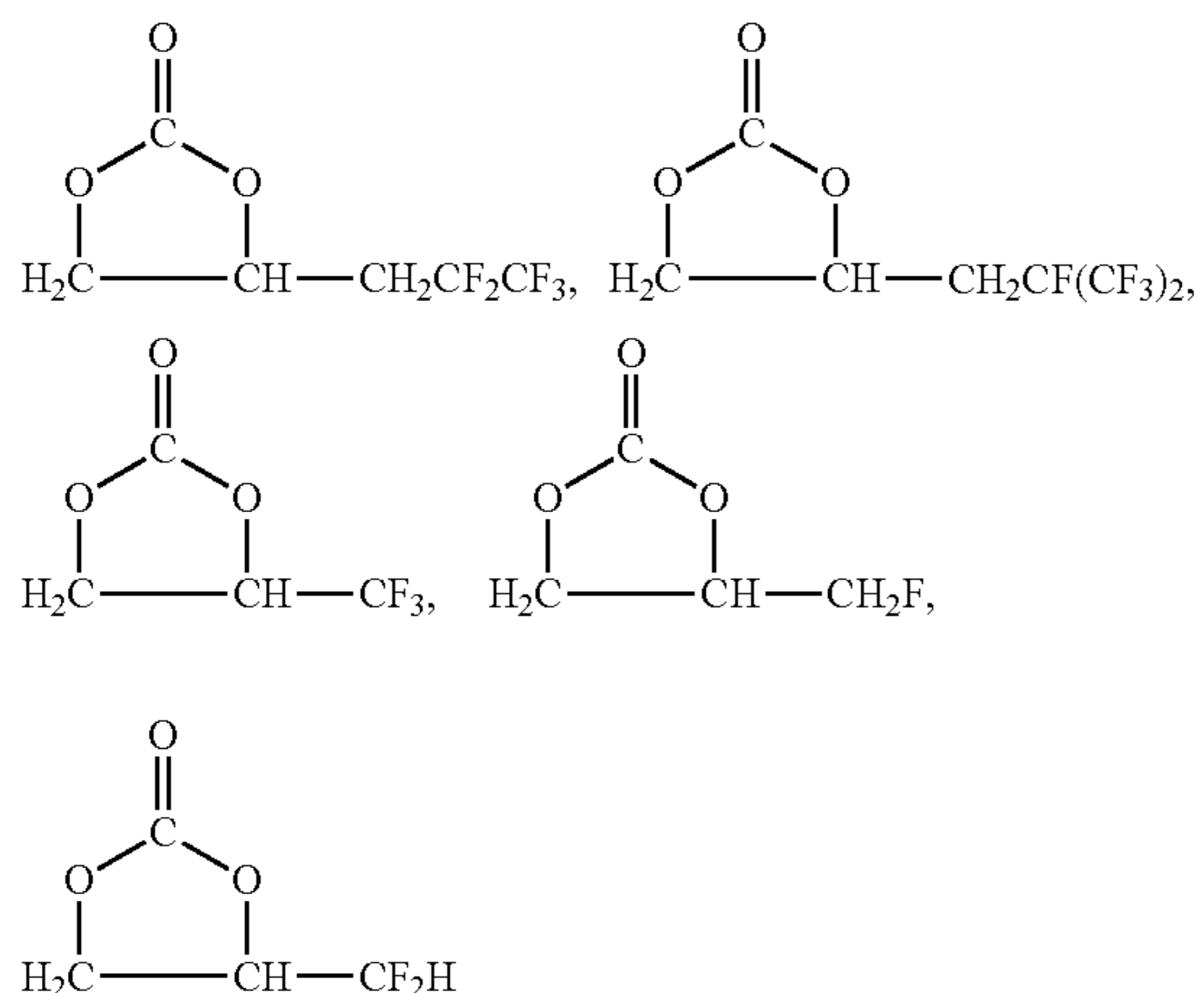
[Chem. 15]
