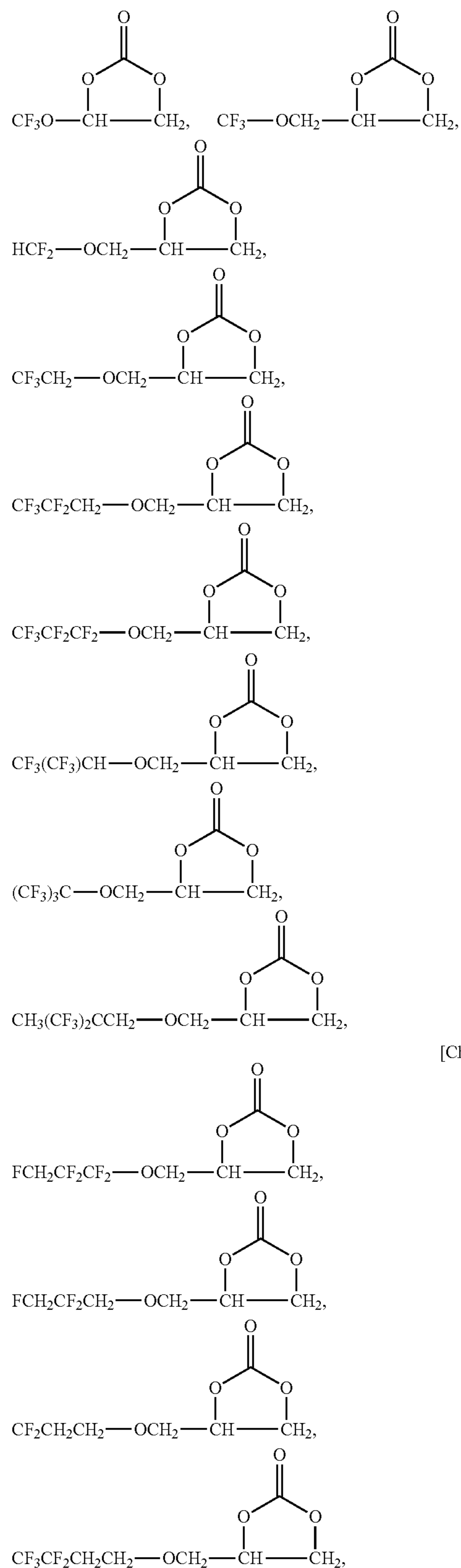
[Chem. 18]
