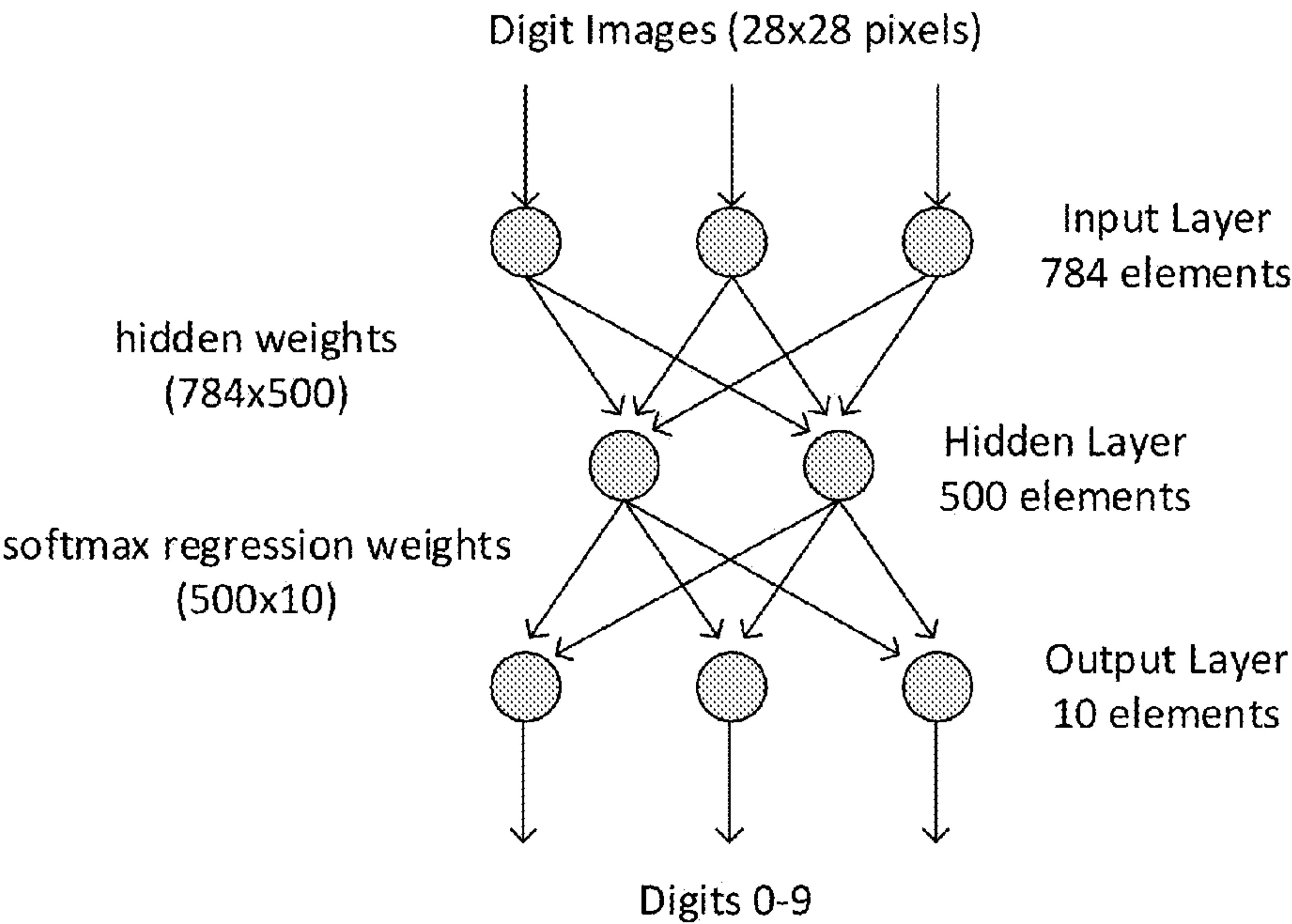
FIG. 1 Multilayer Perceptron Digit Recognition Example.
