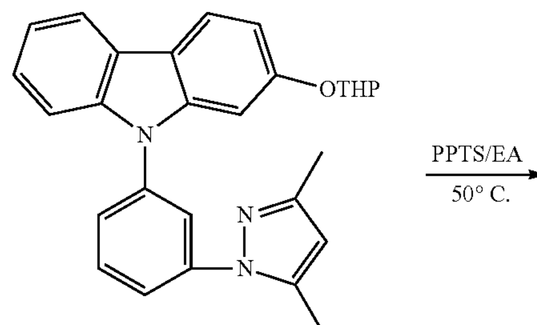
N-[3-(3,5-Dimethylpyrazol-1-yl)phenyl]-2- tetrahydropyranyloxy-carbazole
