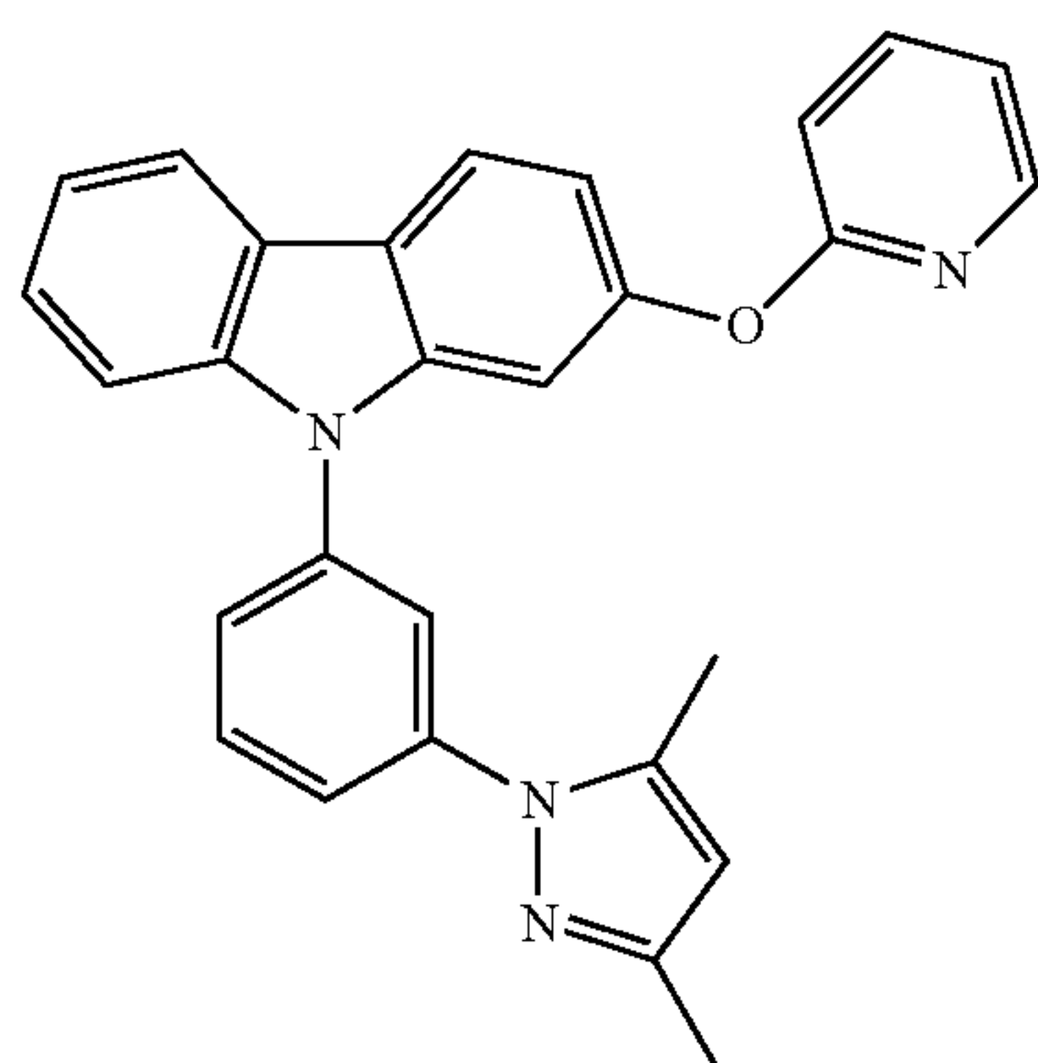
N-[3-(3,5-Dimethylpyrazolyl)phenyl]-2-(pyridinyl-2-oxy)carbazole
