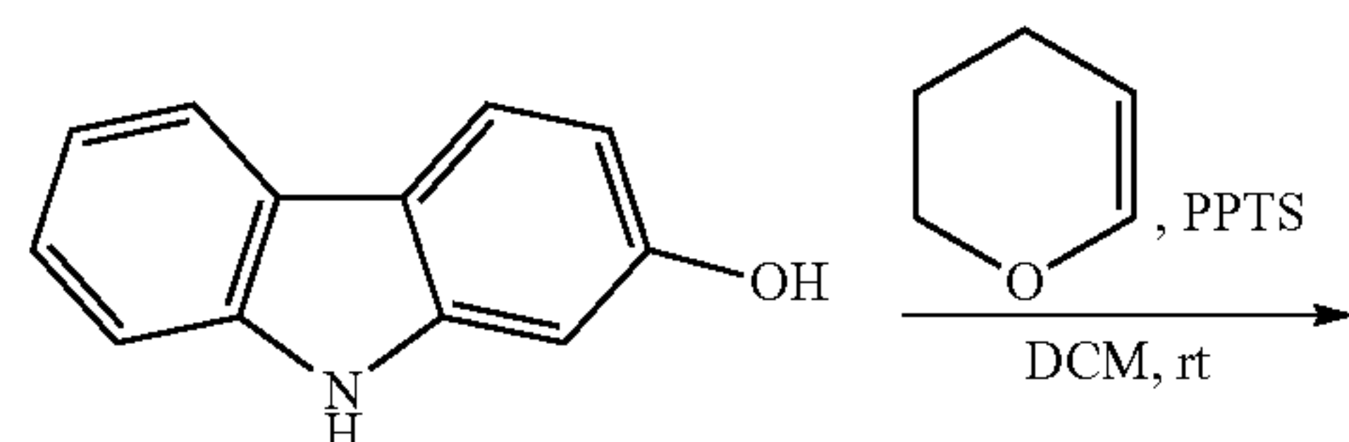
2-hydroxycarbazole
