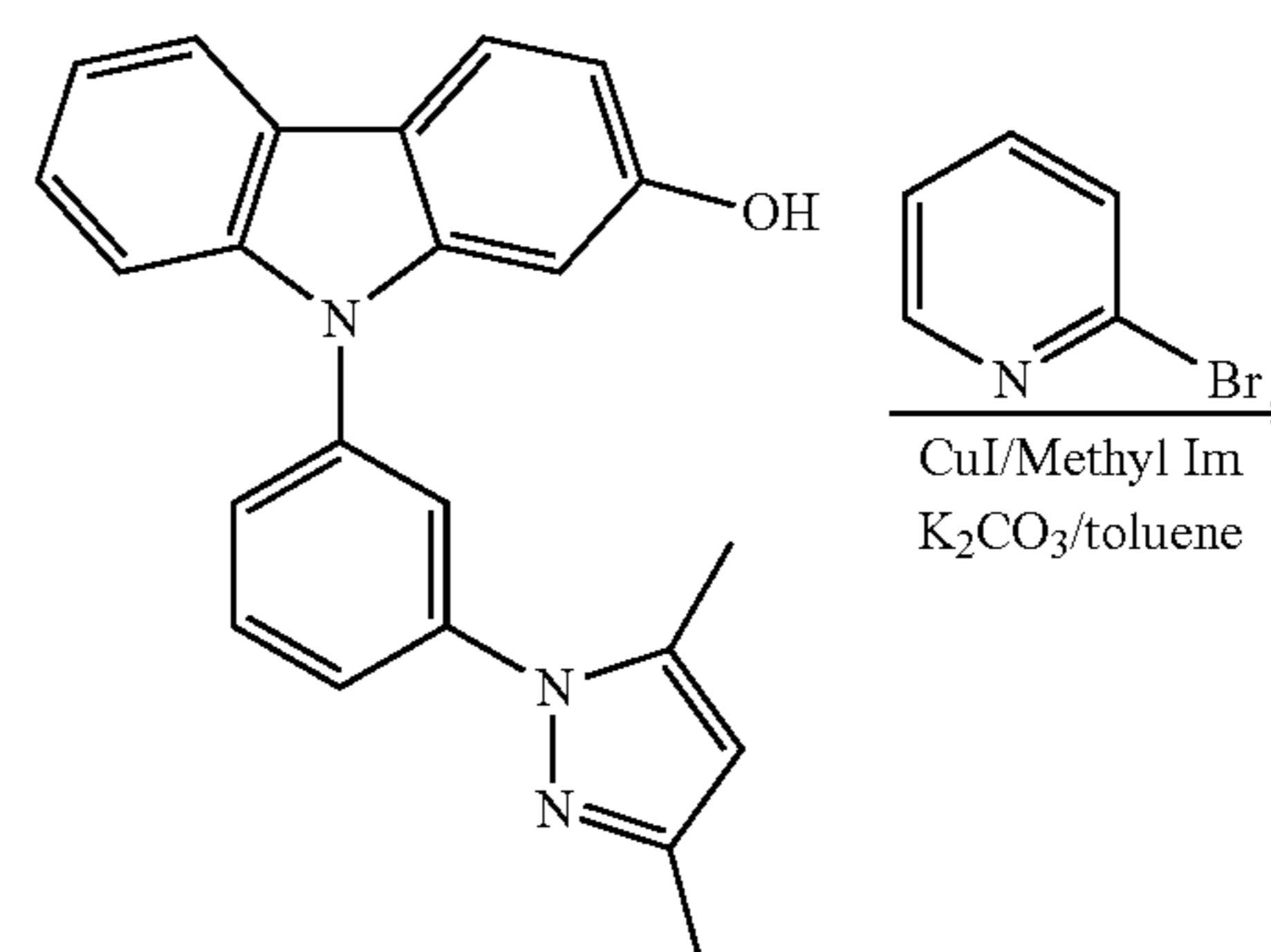
N-(3,5-Dimethylpyrazolyl)phenyl-2-hydroxycarbazole
