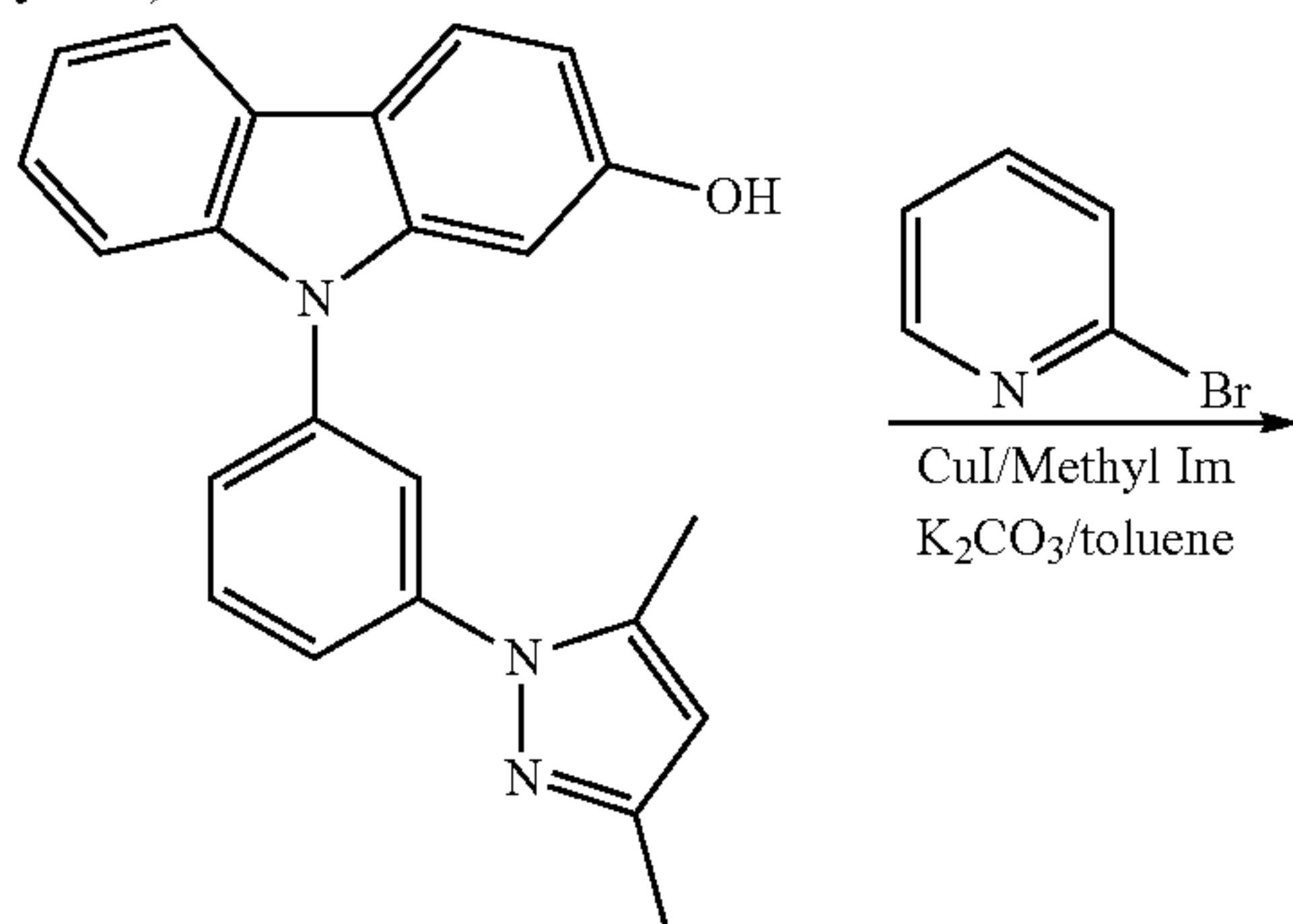
N-(3,5-Dimethylpyrazolyl)phenyl-2-hydroxycarbazole
