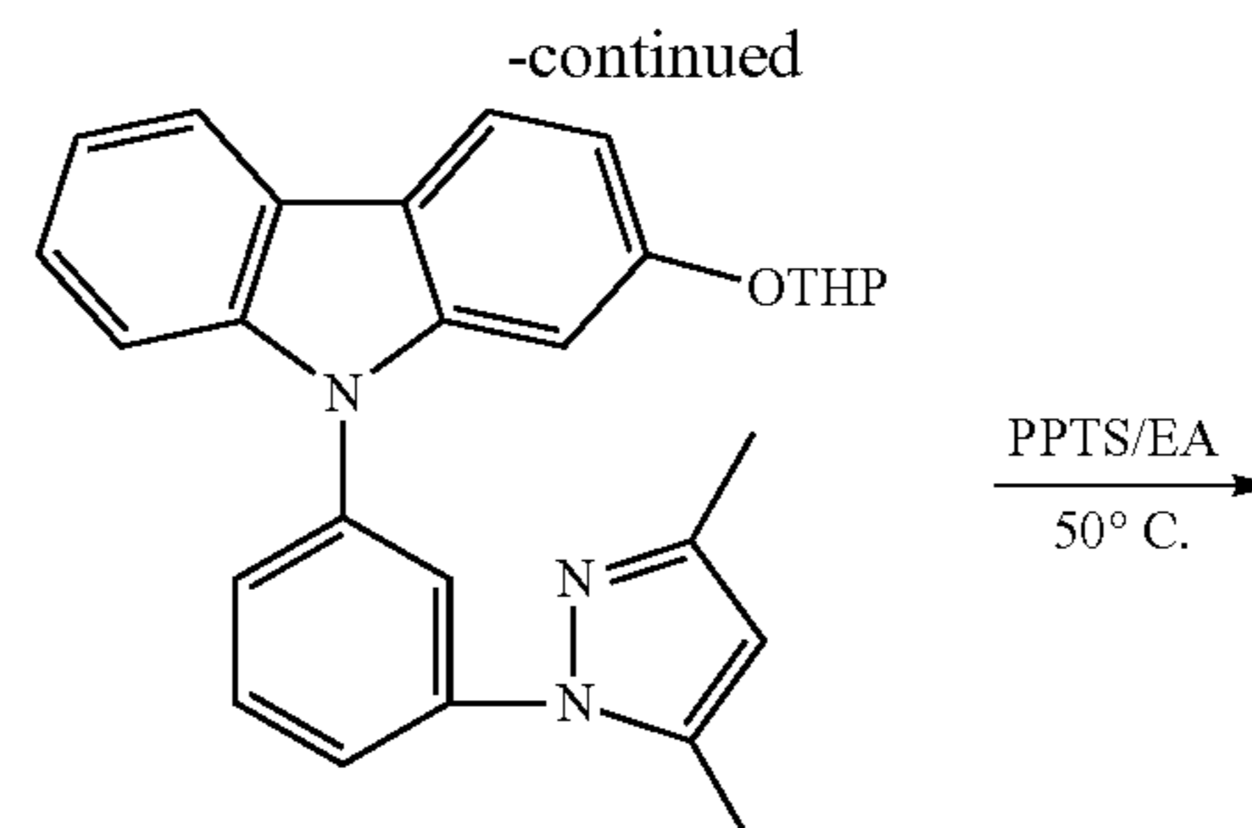
N-[3-(3,5-Dimethylpyrazolyl)phenyl]-2-tetrahydropyranyloxy-carbazole
