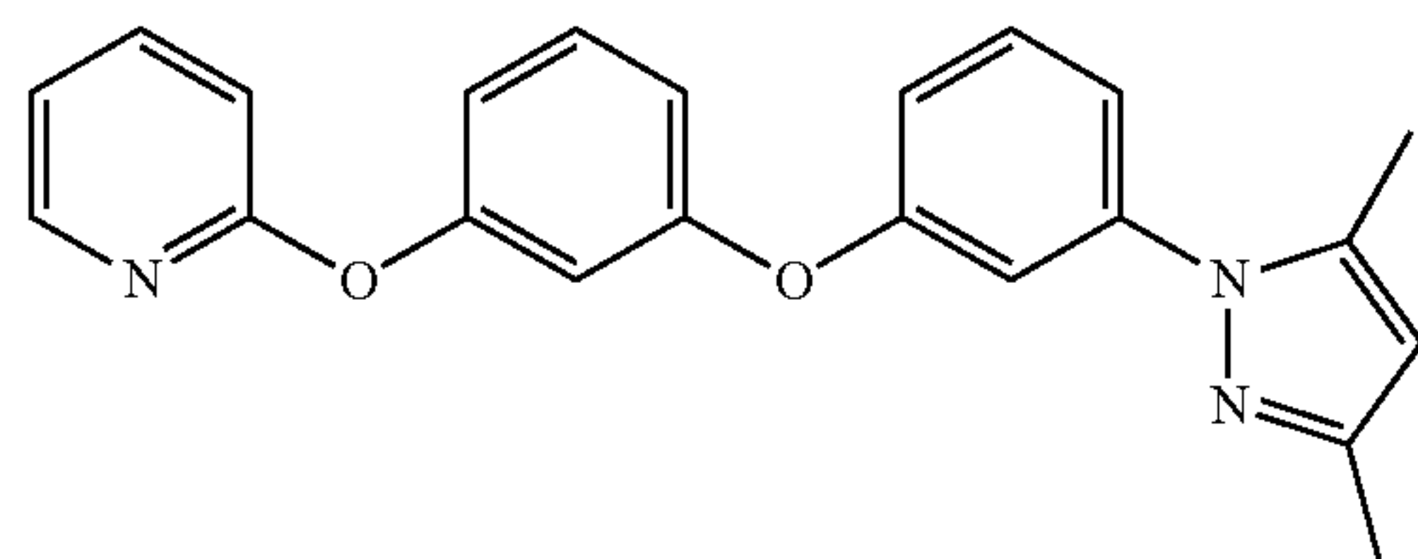
2-(3-(3-(3,5-dimethyl-1H-pyrazol-1-yl) phenoxy)phenoxy)pyridine
