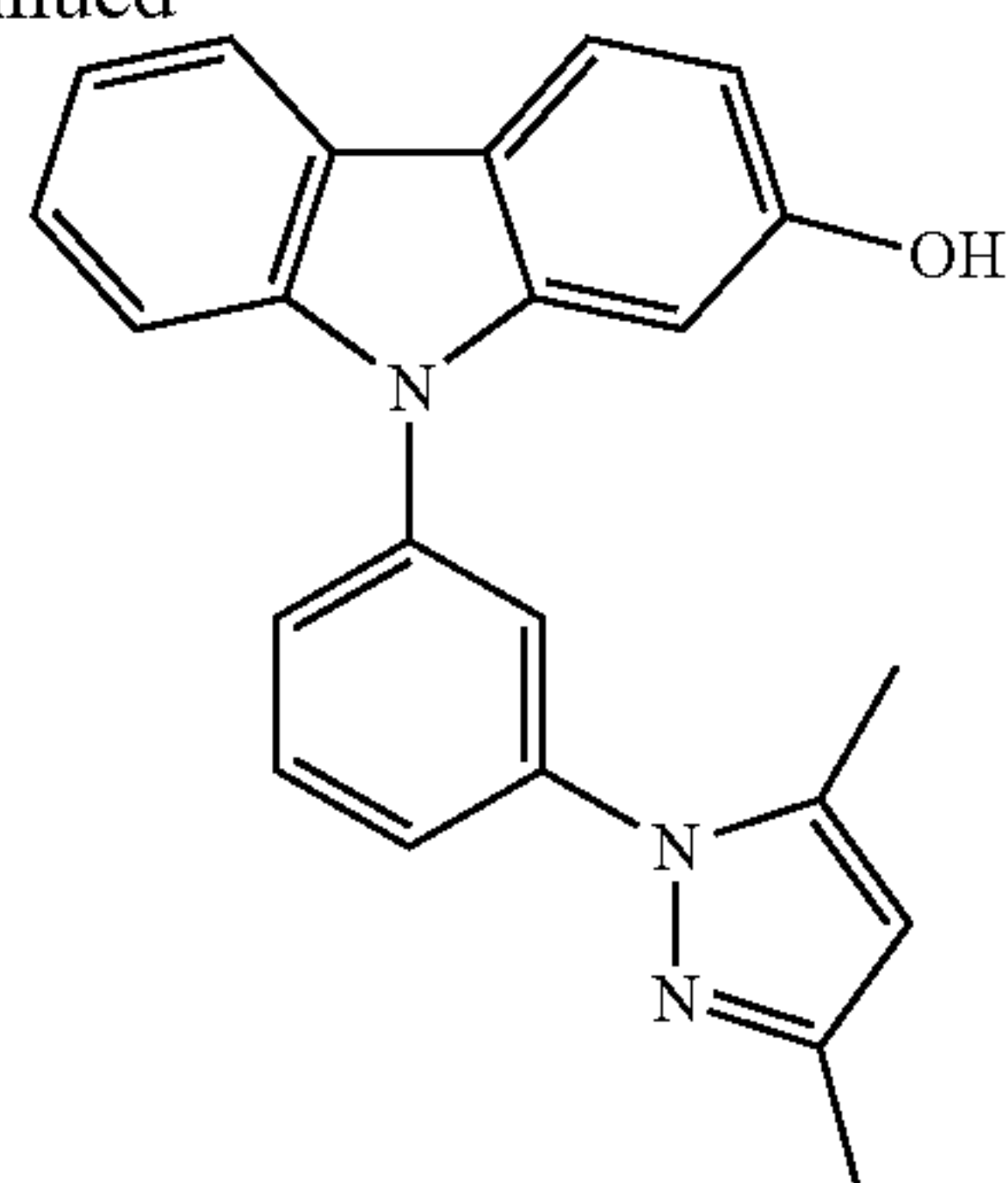
N-(3,5-Dimethylpyrazolyl)phenyl-2-hydroxycarbazole
