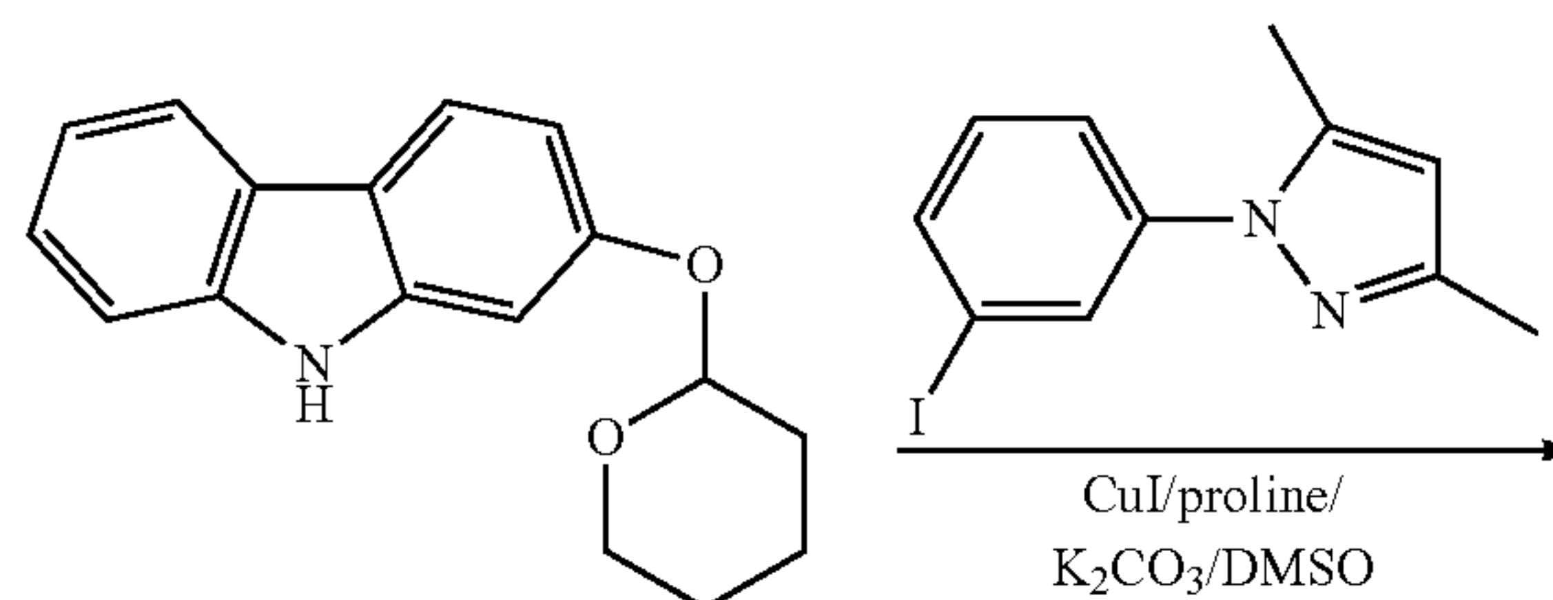
2-tetrahydropyranyloxy-carbazole
