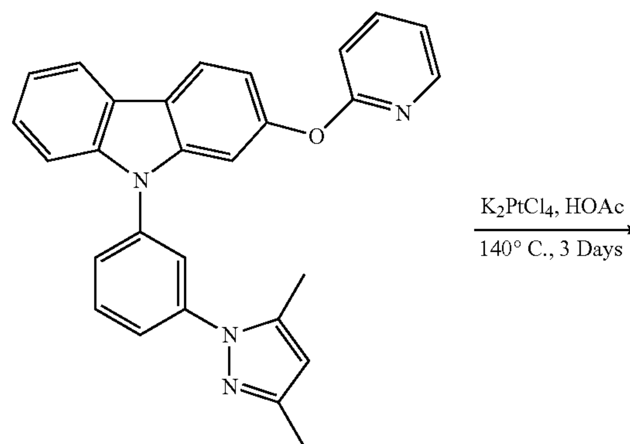
N-[3-(3,5-Dimethylpyrazolyl)phenyl]-2-(pyridinyl-2-oxy)carbazole
