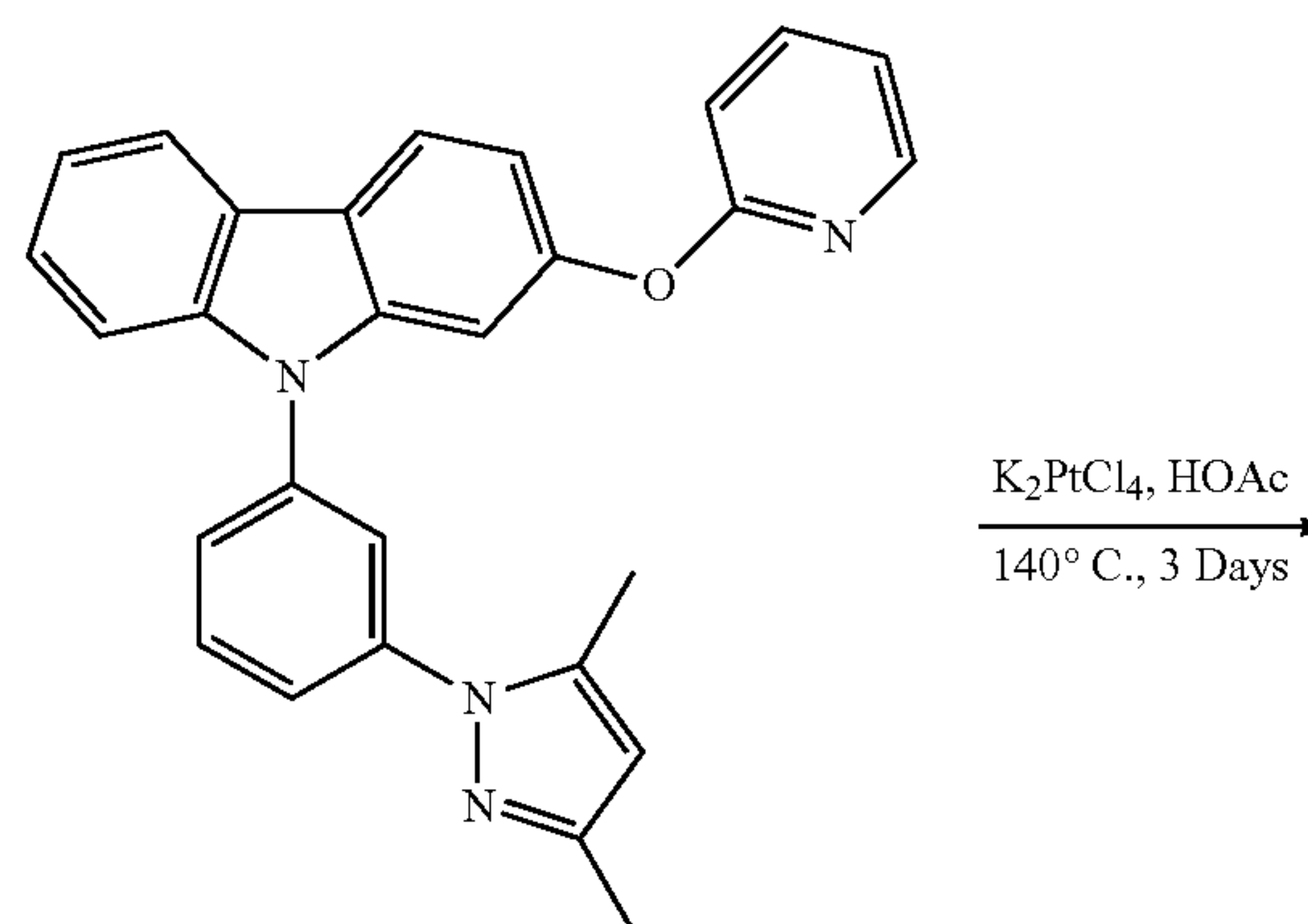
N-[3-(3,5-Dimethylpyrazol-1-yl)phenyl]-2- (pyridin-2-yloxy)-carbazole
