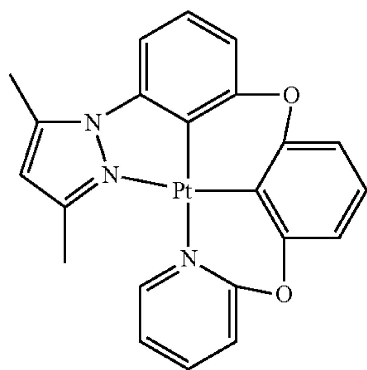
Pt-001 Complex
