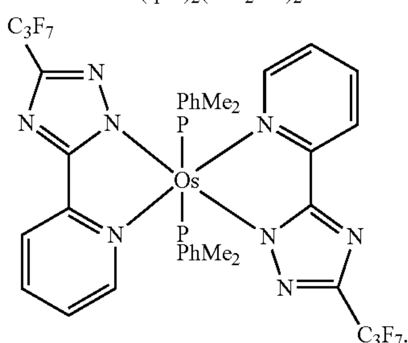
Os(bptz) 2 (PPhMe 2 ) 2
