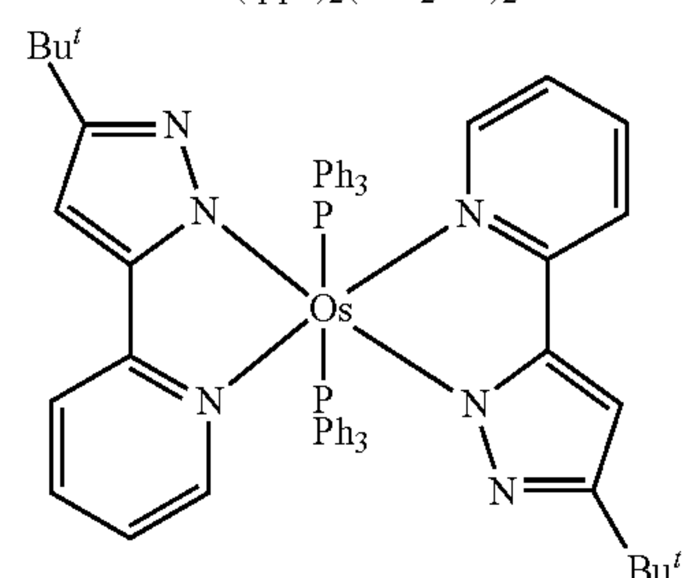
Os(bppz) 2 (PPh 3 ) 2
