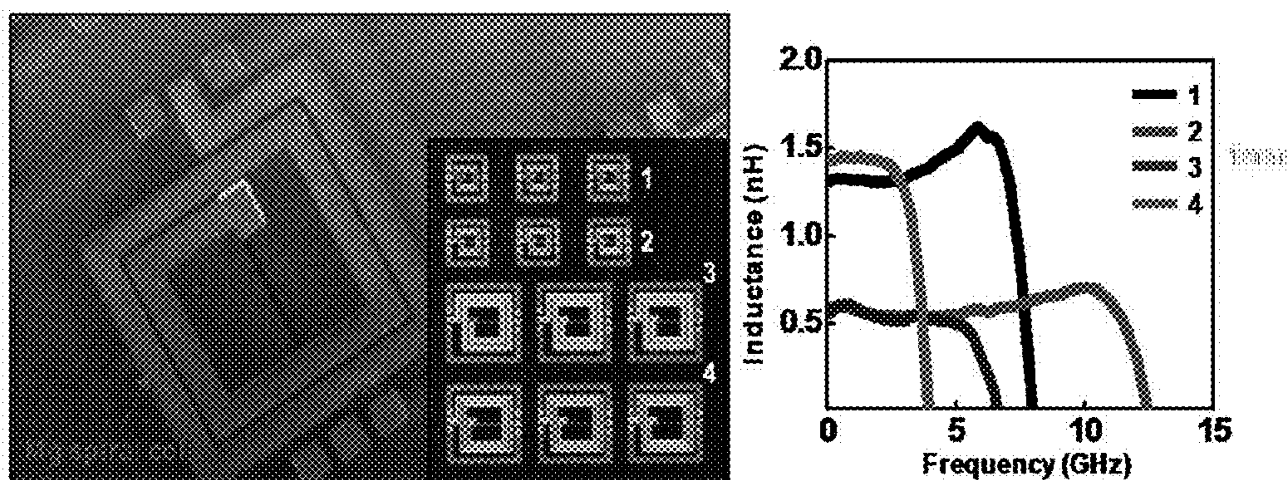
Inductor array on Mo foil (~10 \mu\text{m} thick)
