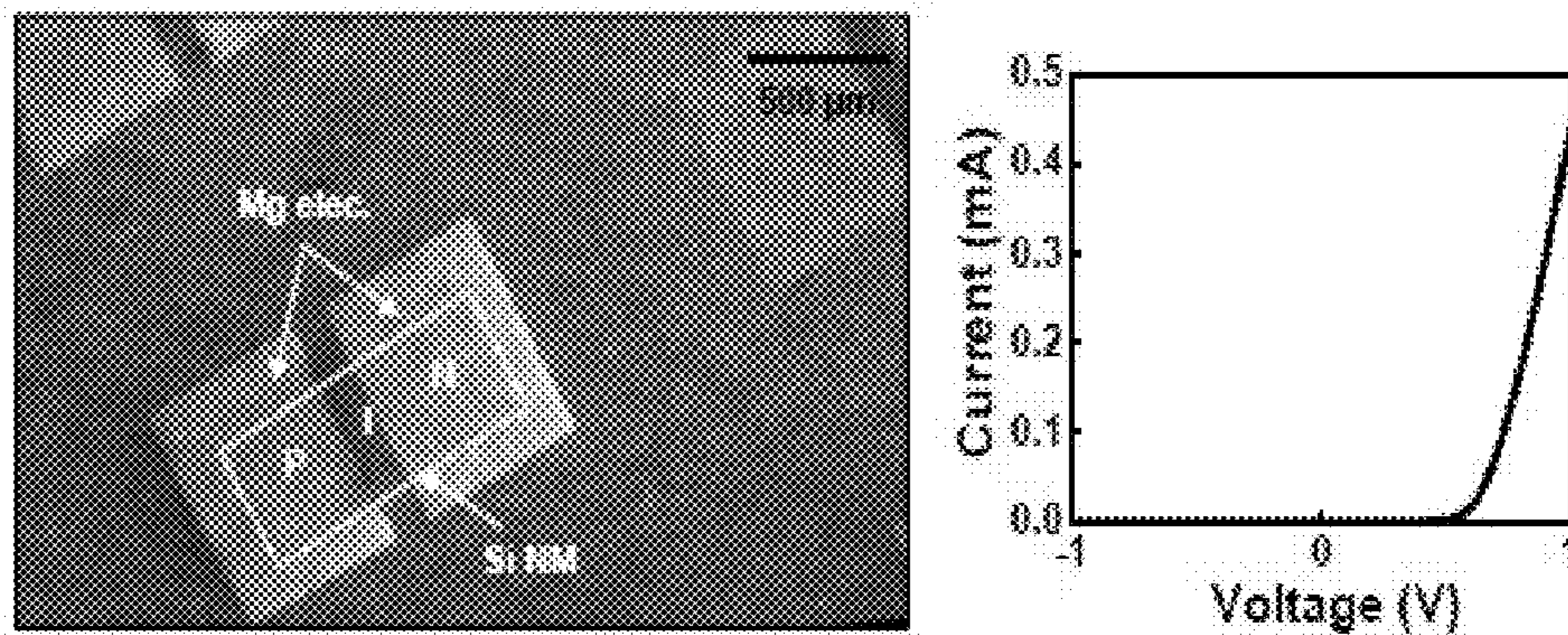
Diode array on Zn foil (~10 \mu\text{m} thick)
