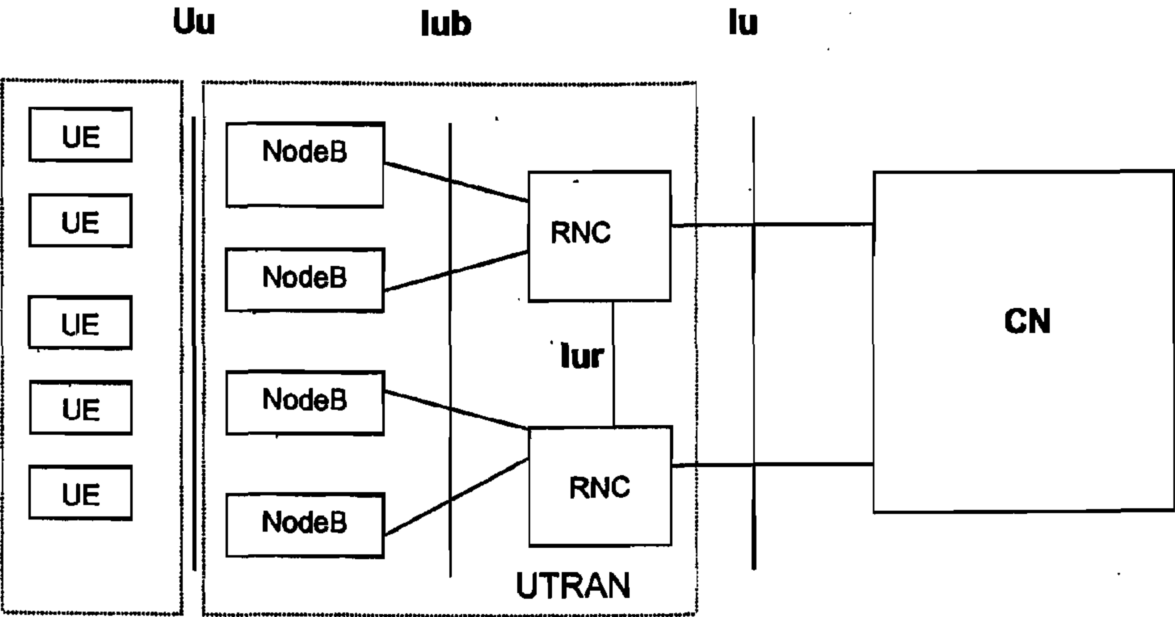
Figure 1 (Prior Art)
