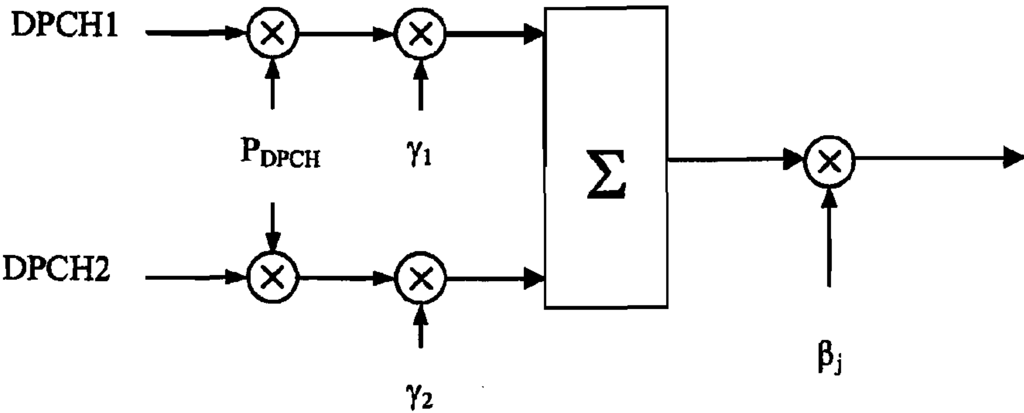
Figure 3 (Prior Art)
