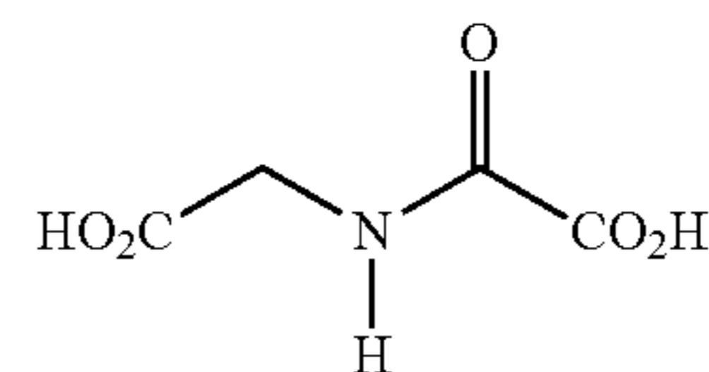
(N-oxalyl glycine)
