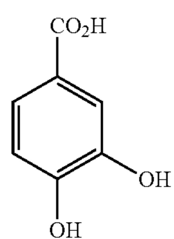
Protocatechuic acid
