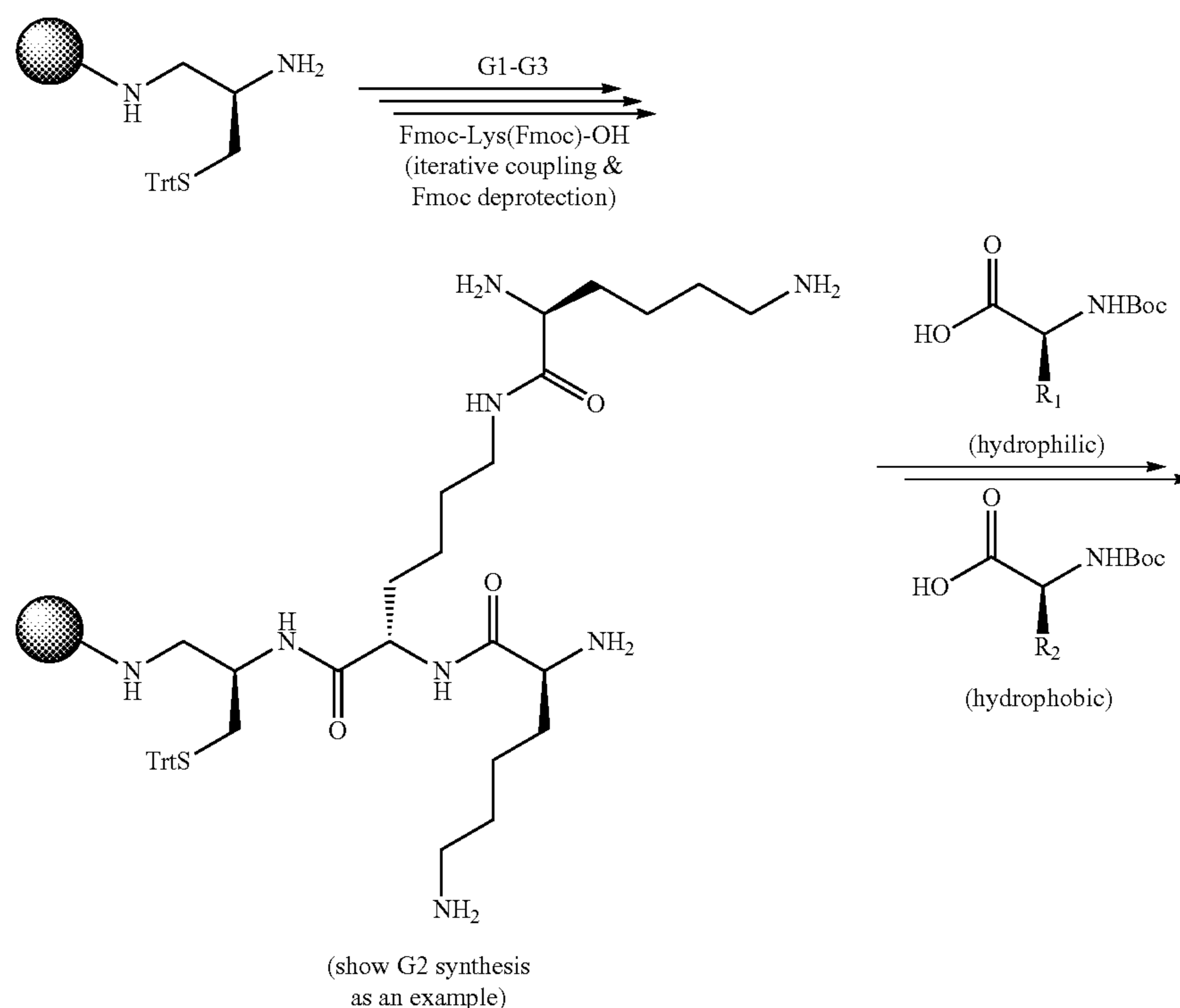
SCHEME 2
