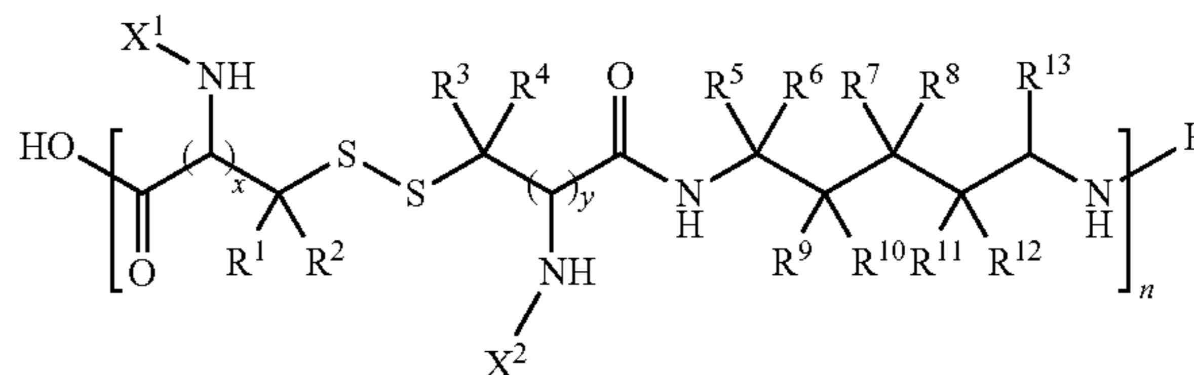
Formula I
