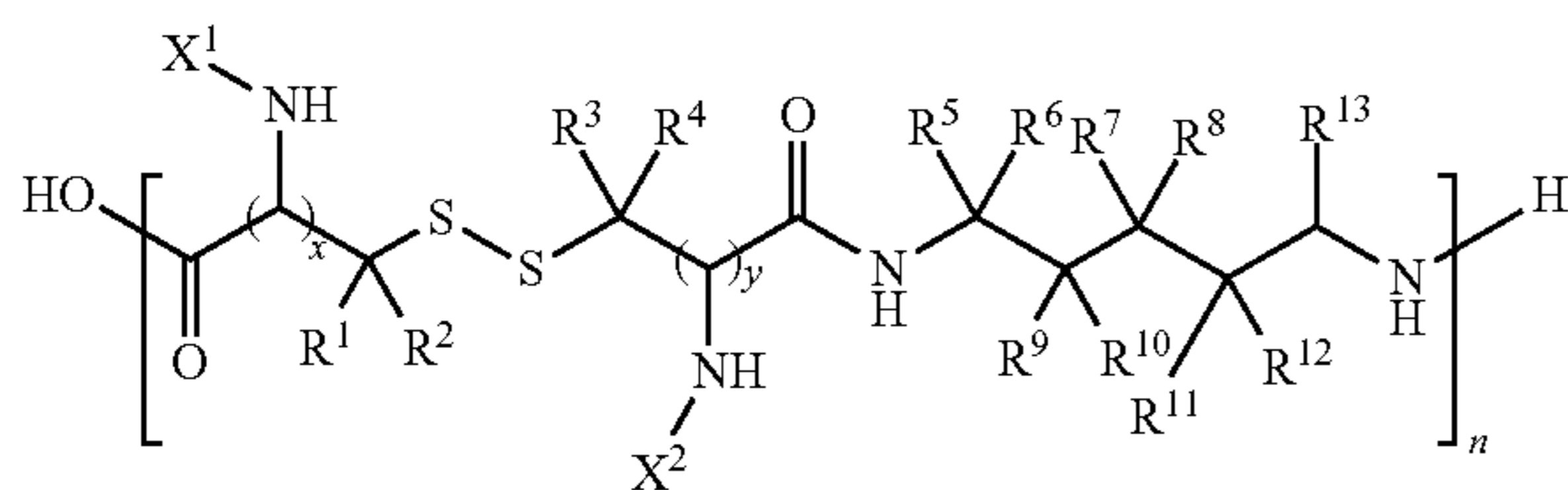
Formula I
