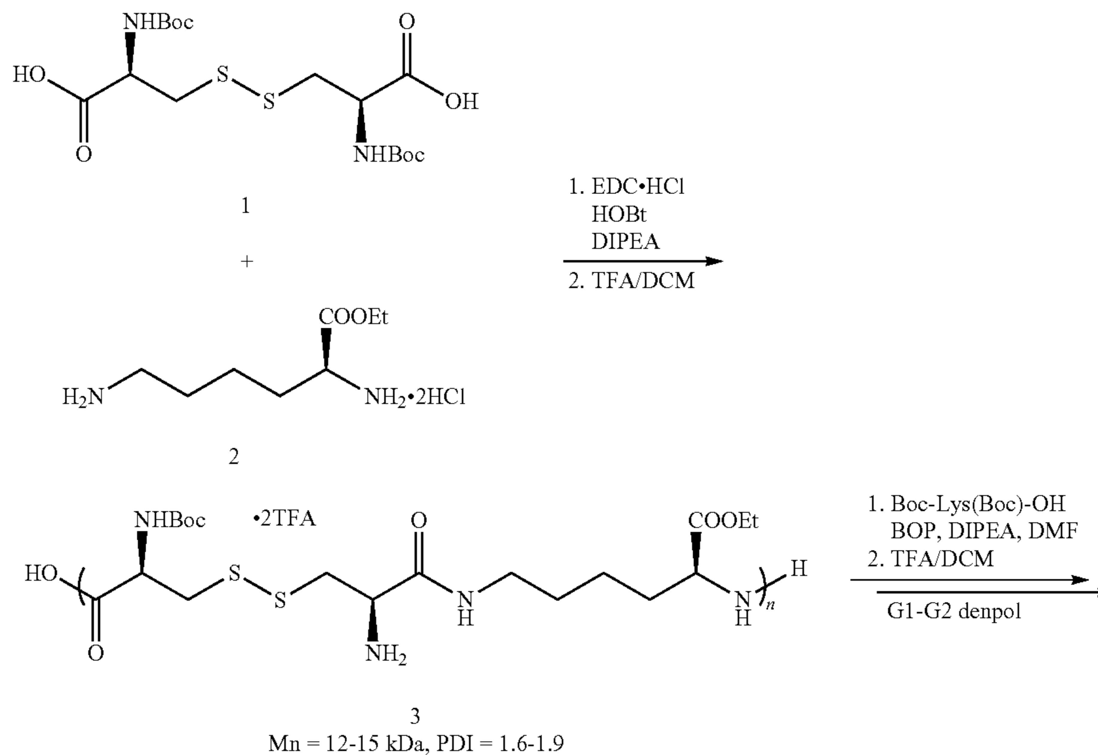
SCHEME 5
