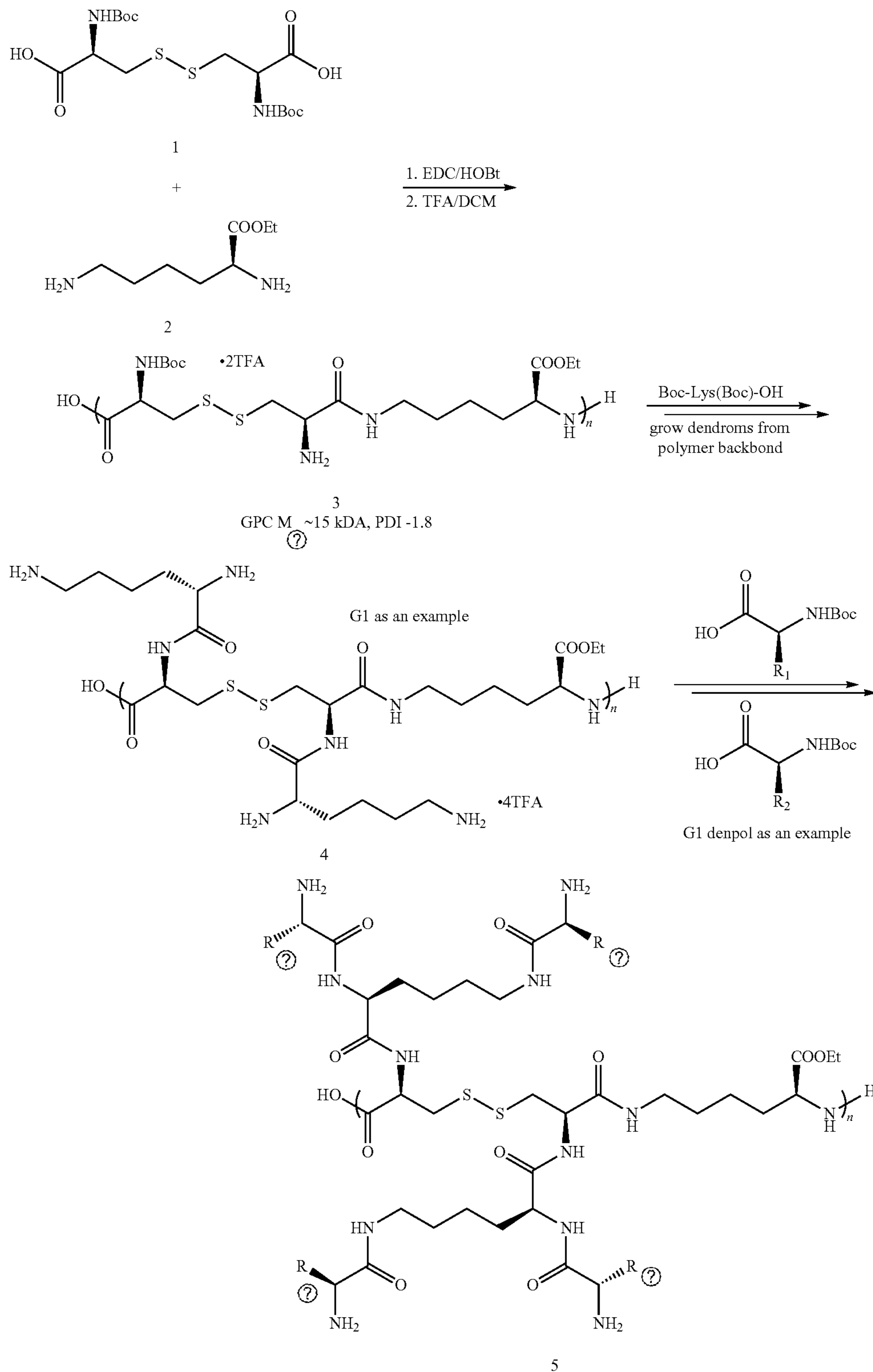
SCHEME 1
