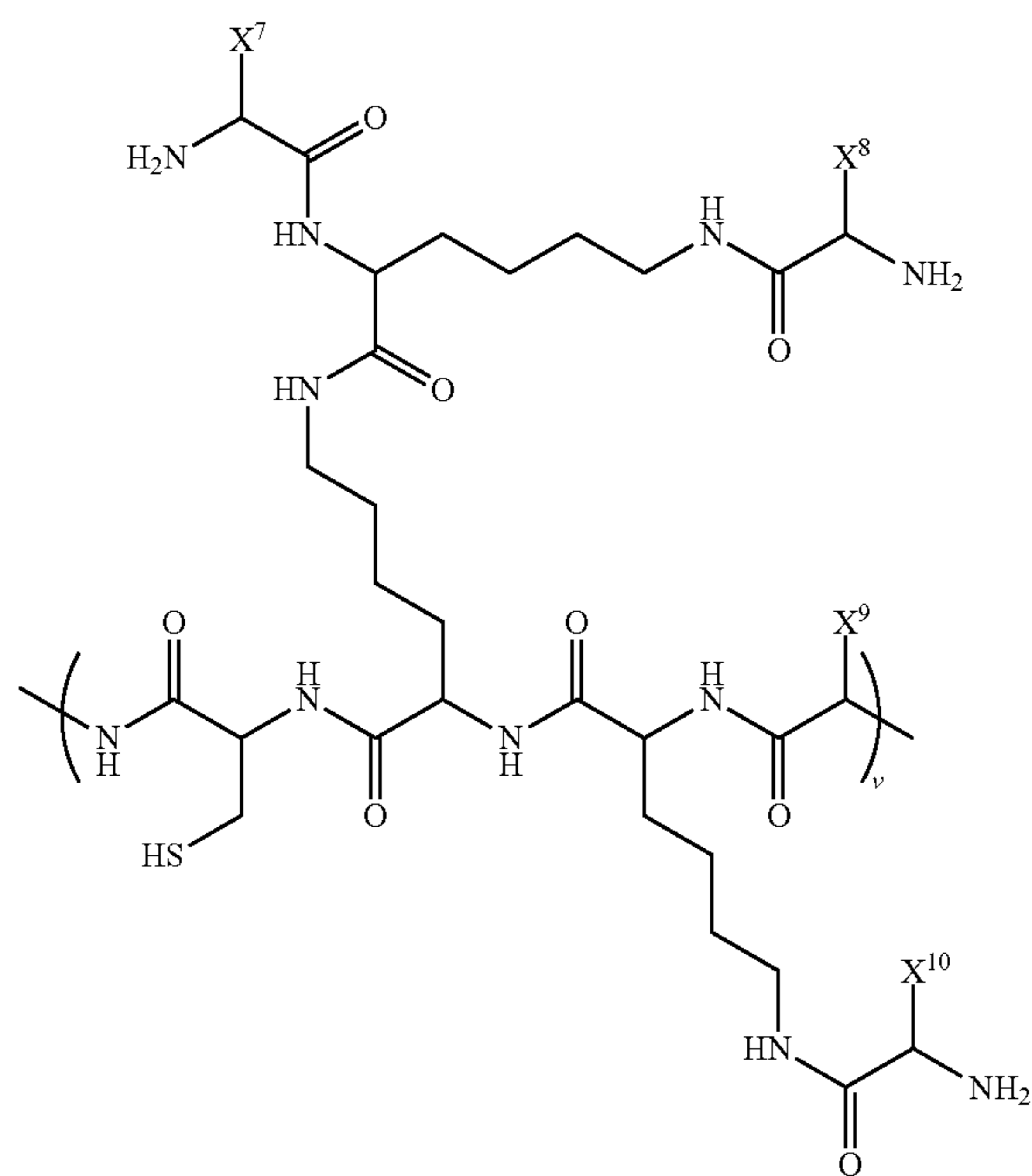
Formula III
