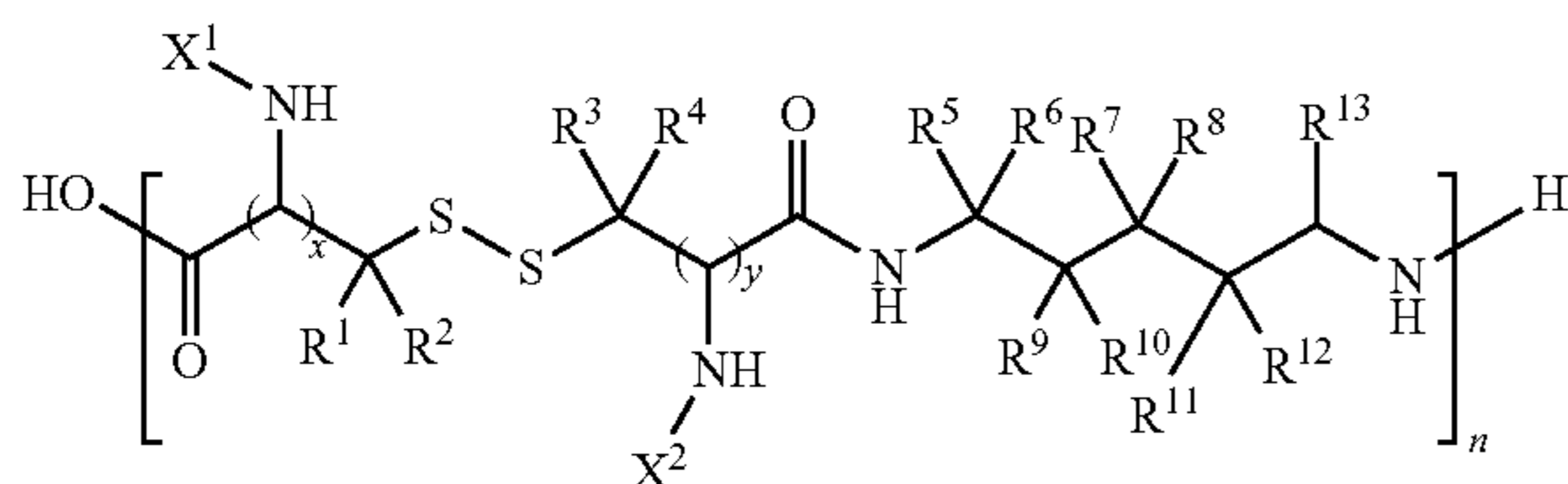
Formula I
