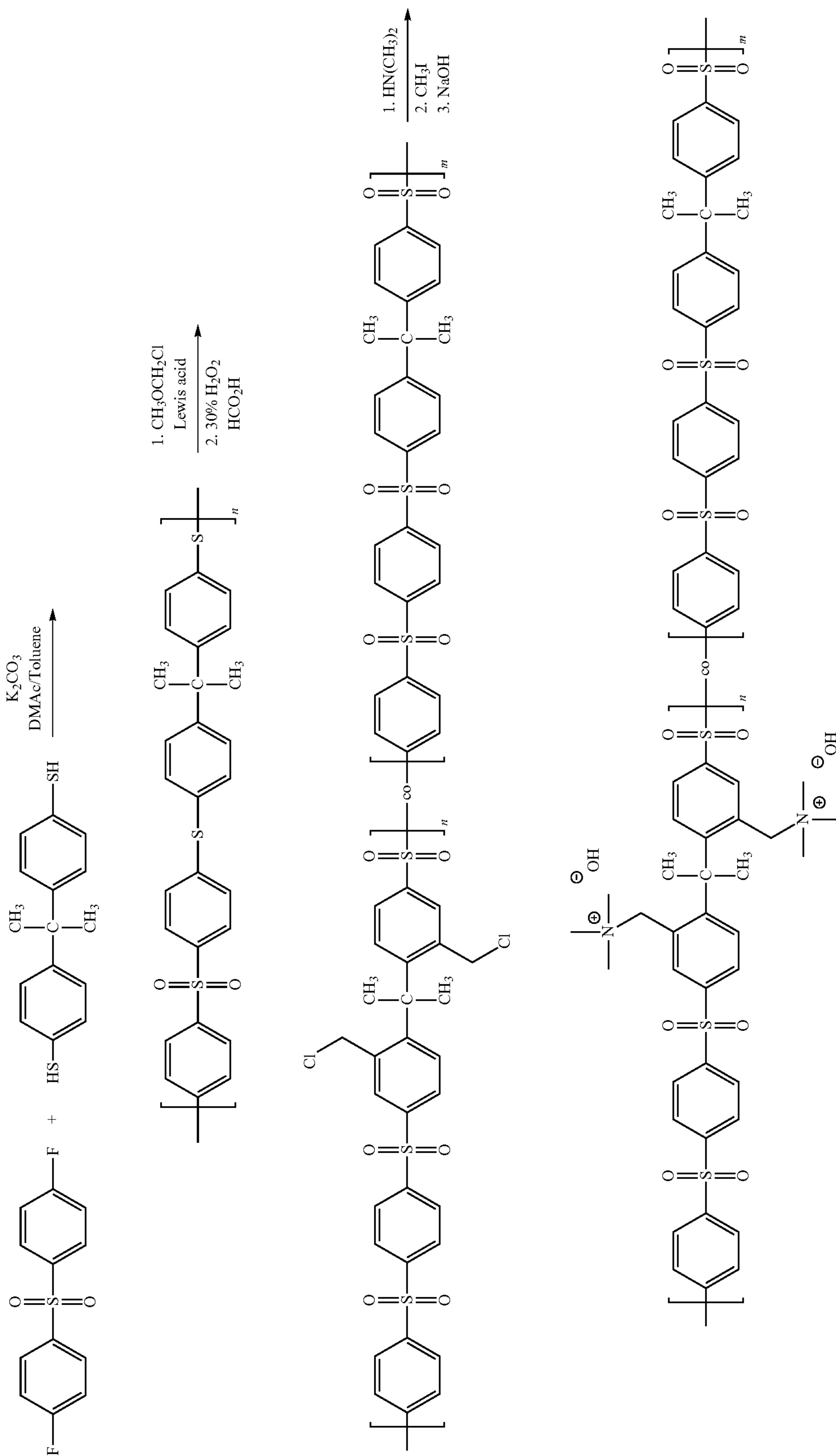
Scheme III
