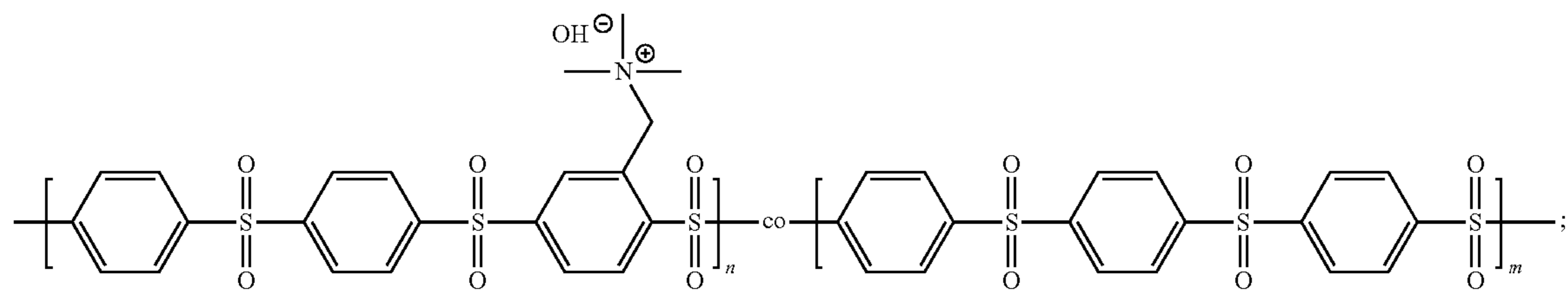
Copolymer 2
