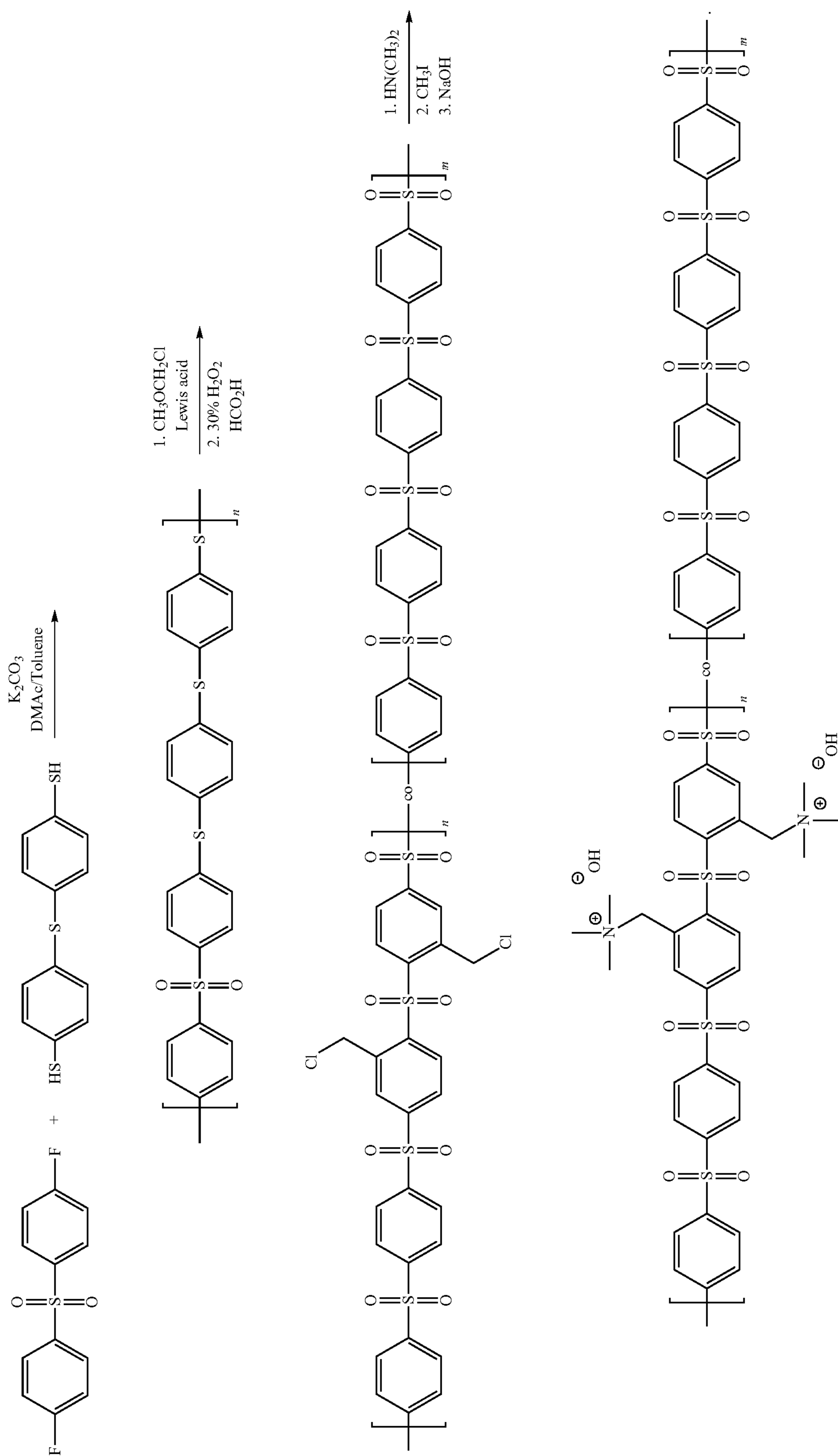
Scheme II
