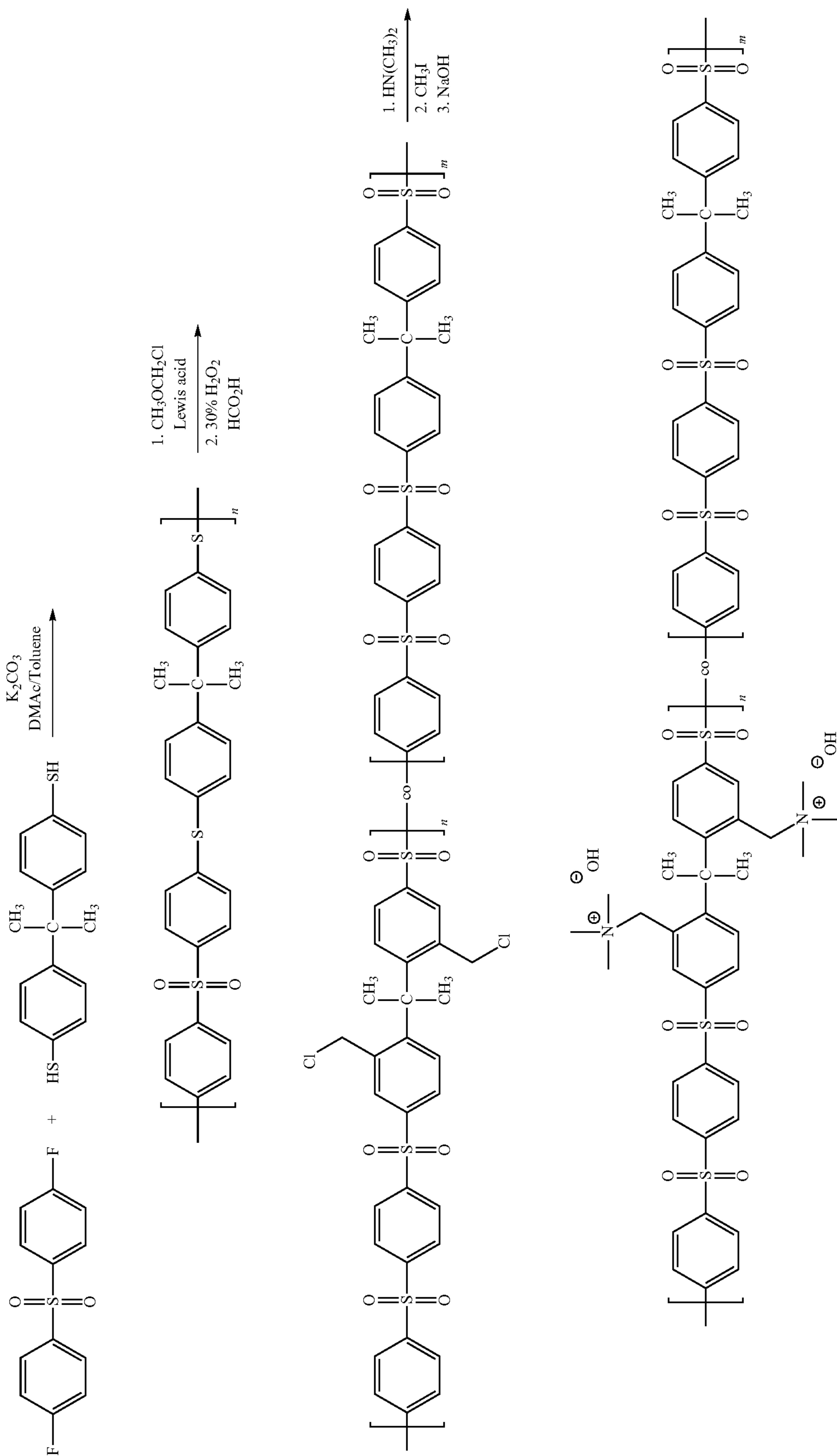
Scheme III
