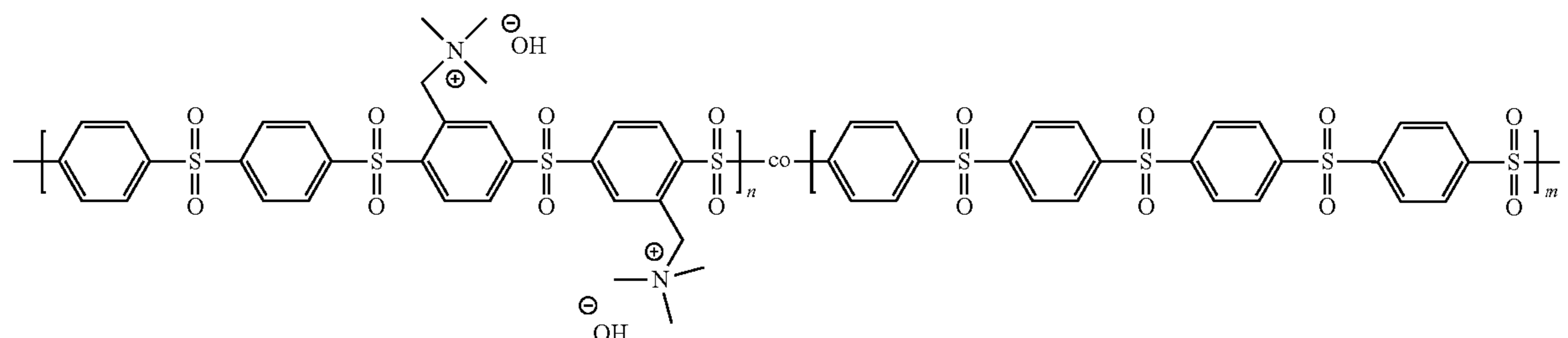
Copolymer 3
