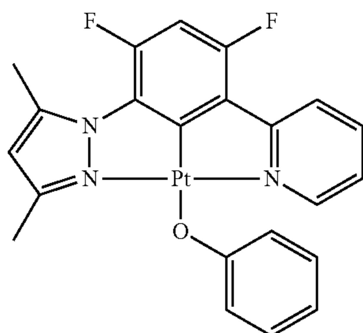
DMPz—DFPh—Py—PtOPh
