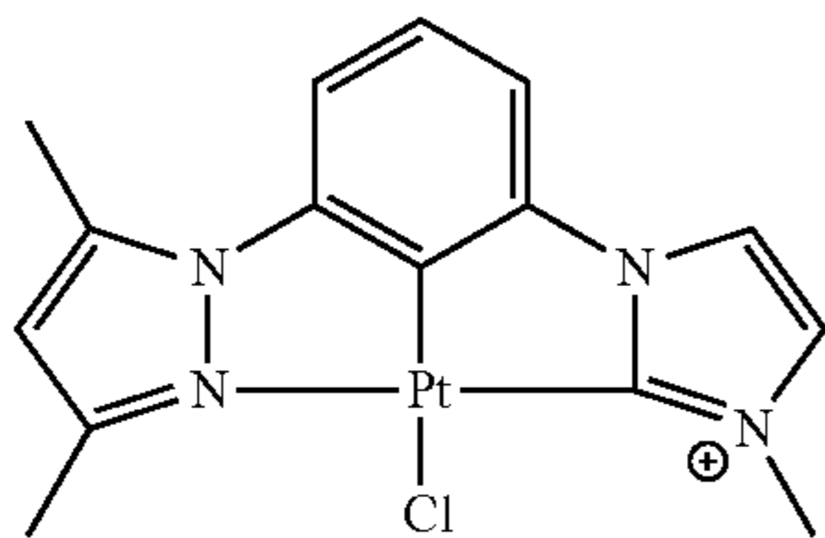
DMPz—Ph—MIzCb—PtCl
