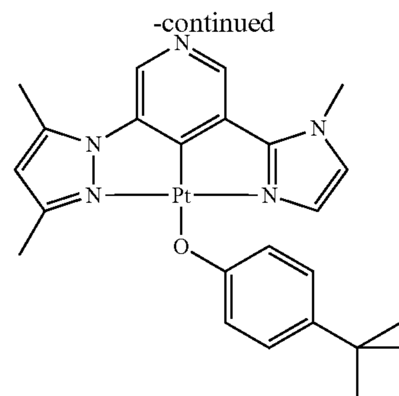
DMPz—Py—MIz—PtOPhBu
