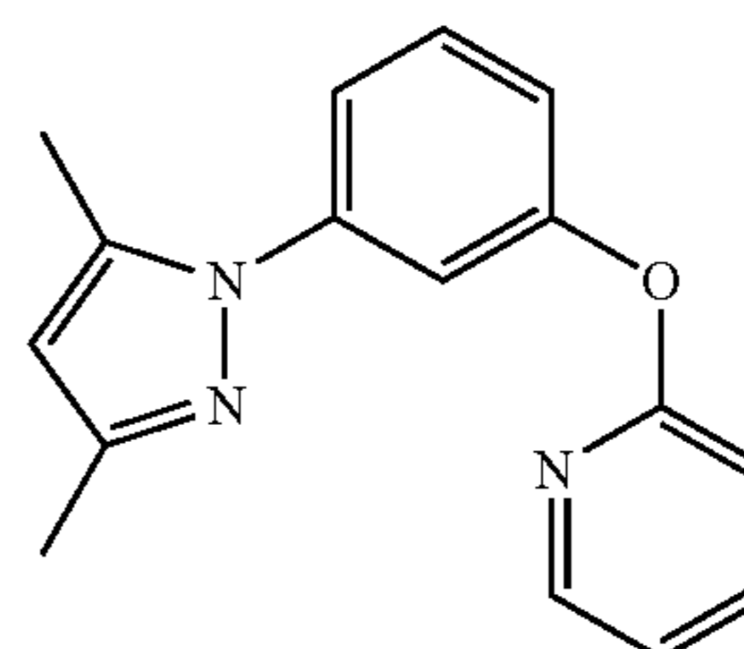
DMPz-Ph-O-Py
