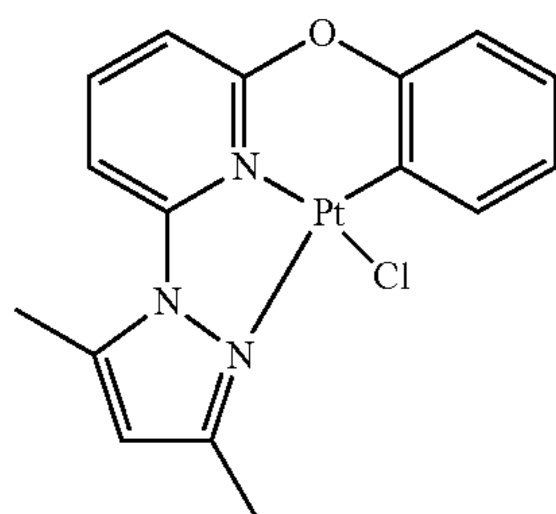
DMPz-Py-O-Ph-PtCl
