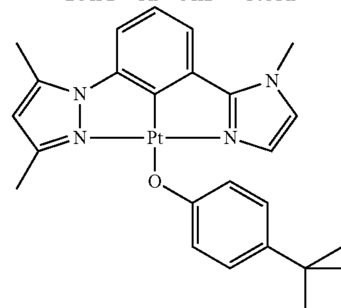
DMPz—Ph—MIz—PtOPhBu
