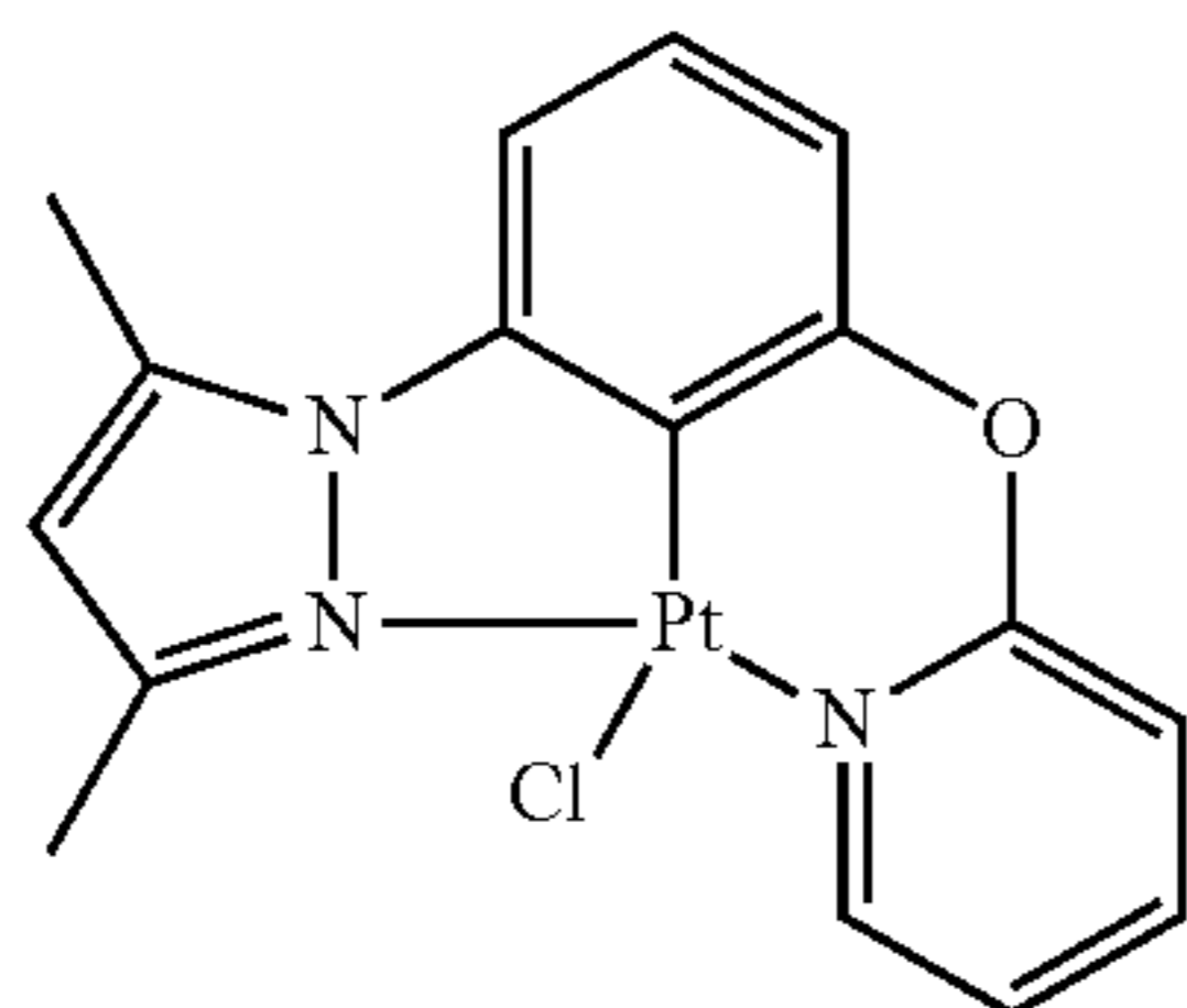
DMPz-Ph-O-Py-PtCl
