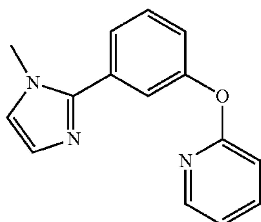
MIz-Ph-O-Py
