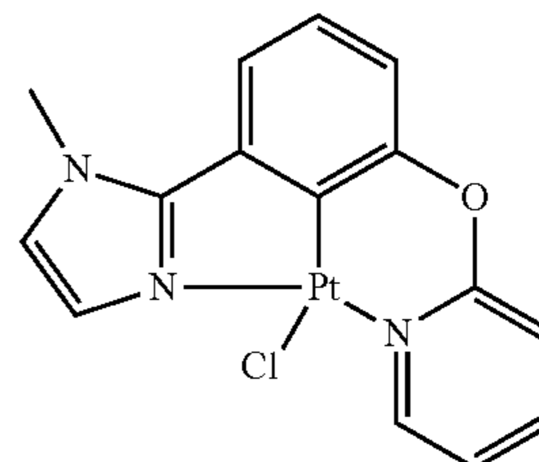
MIz-Ph-O-Py-PtCl
