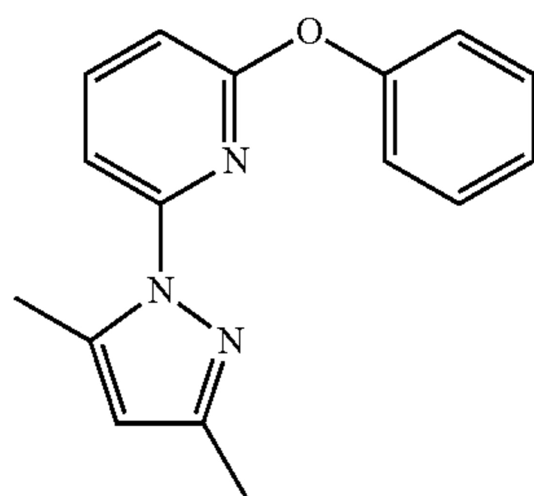
DMPz-Py-O-Ph
