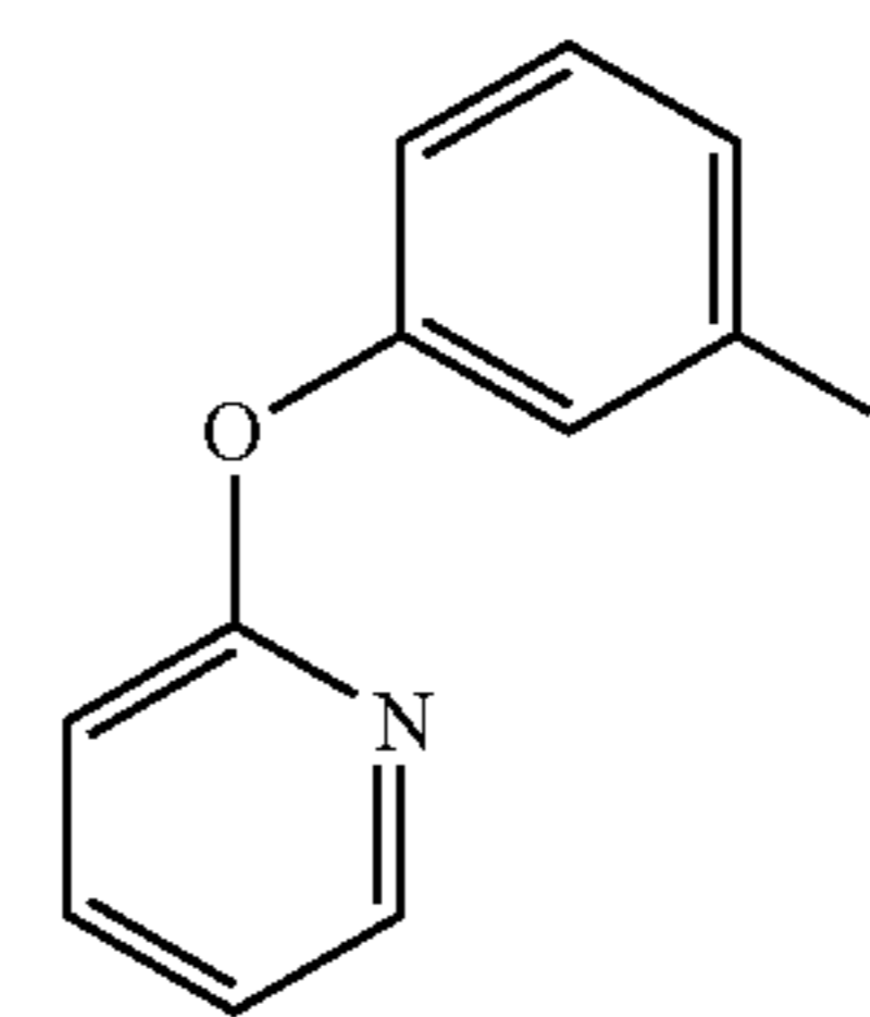
Py-O-Ph-I
