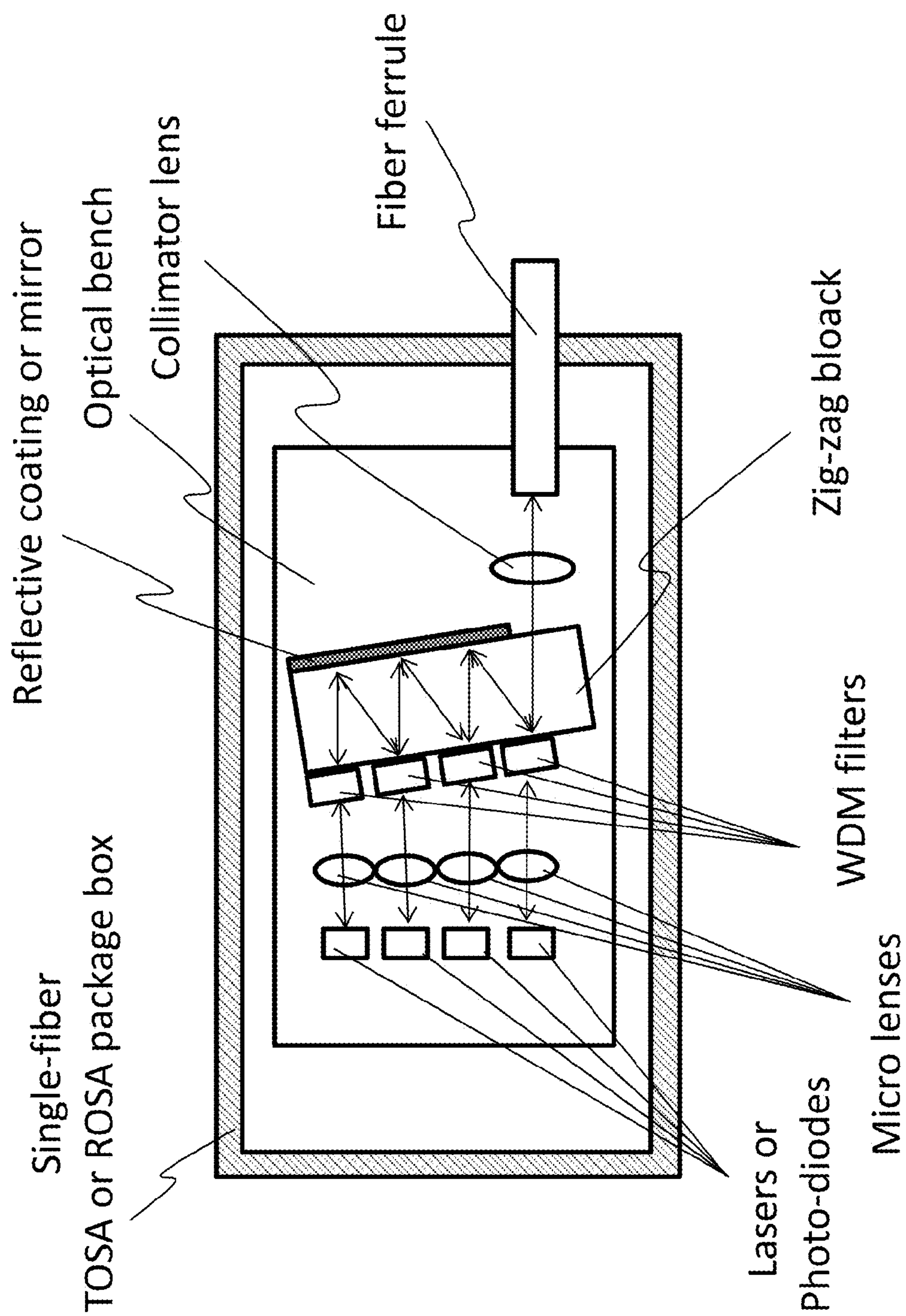
FIG. 2 (Prior art)
