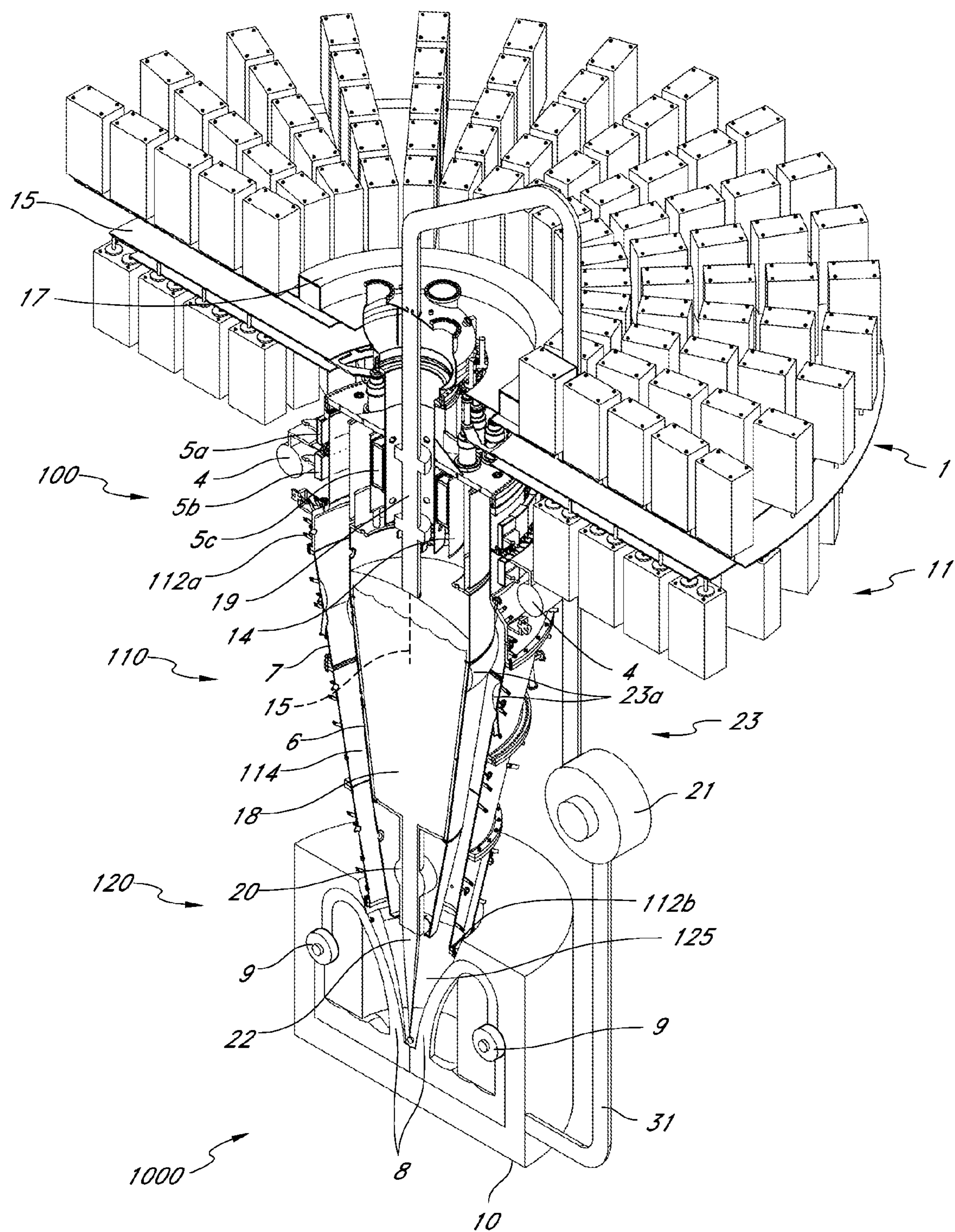
FIG. 1D
