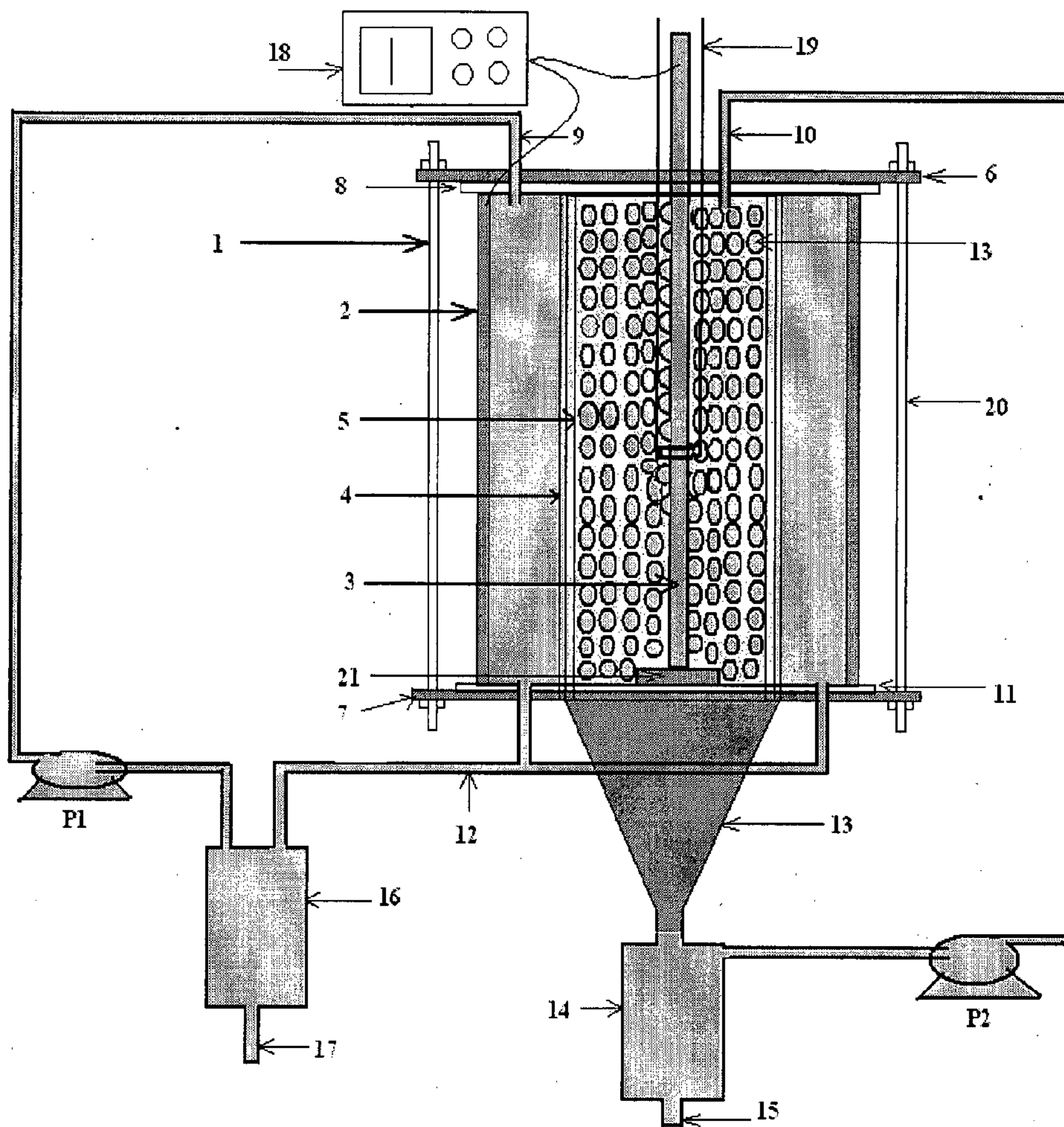
Electrochemical cell for recovery of metals
