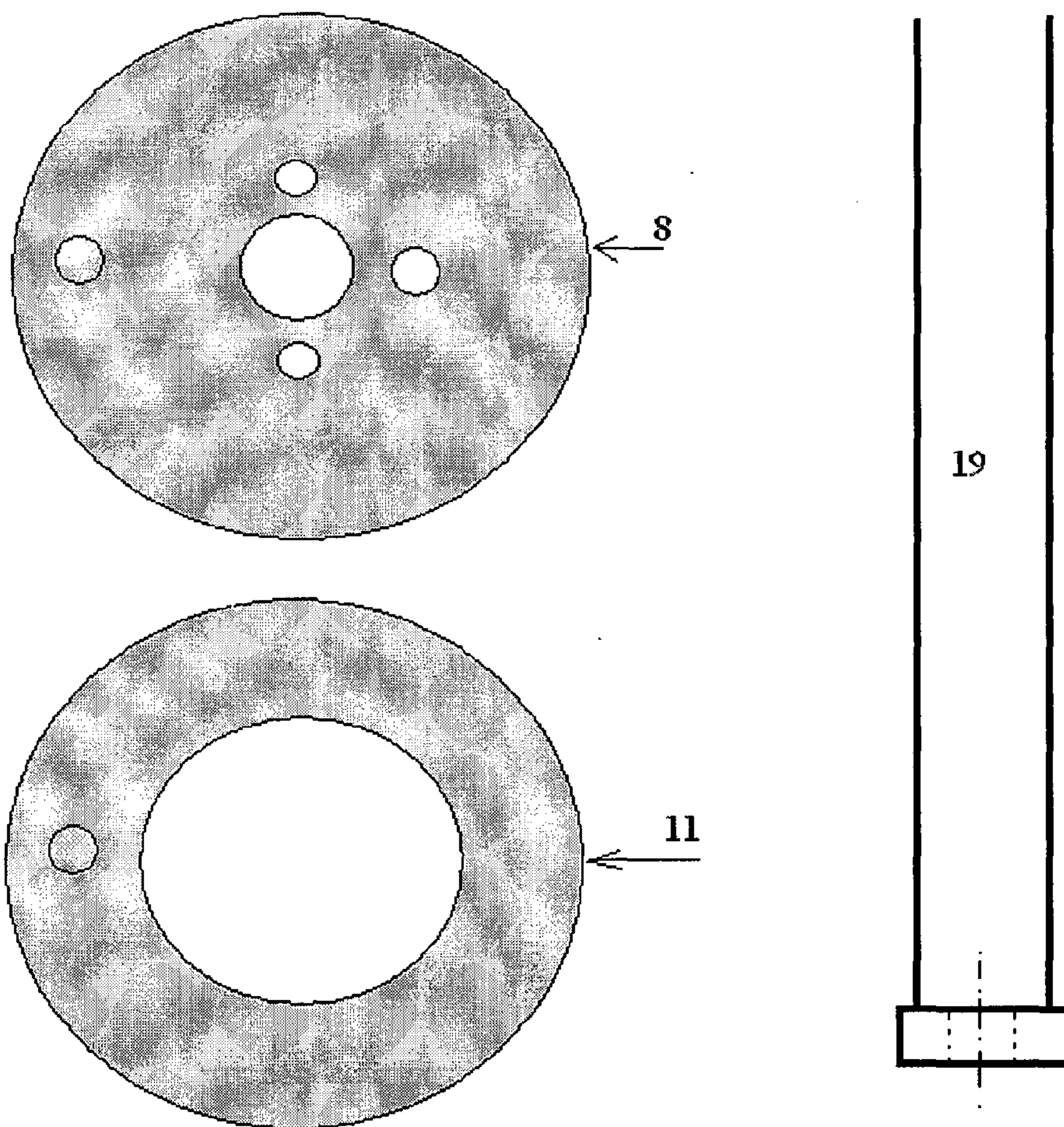
Top view of first end and second end Teflon gasket and mechanical scraper
