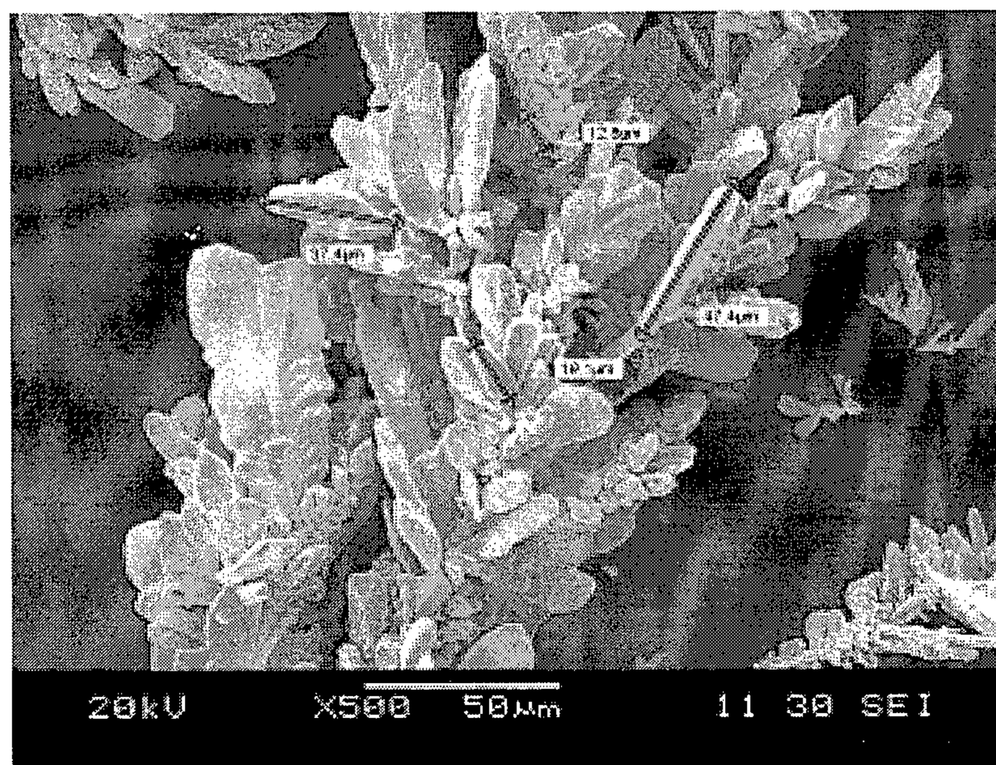
SEM image of deposited copper powder
