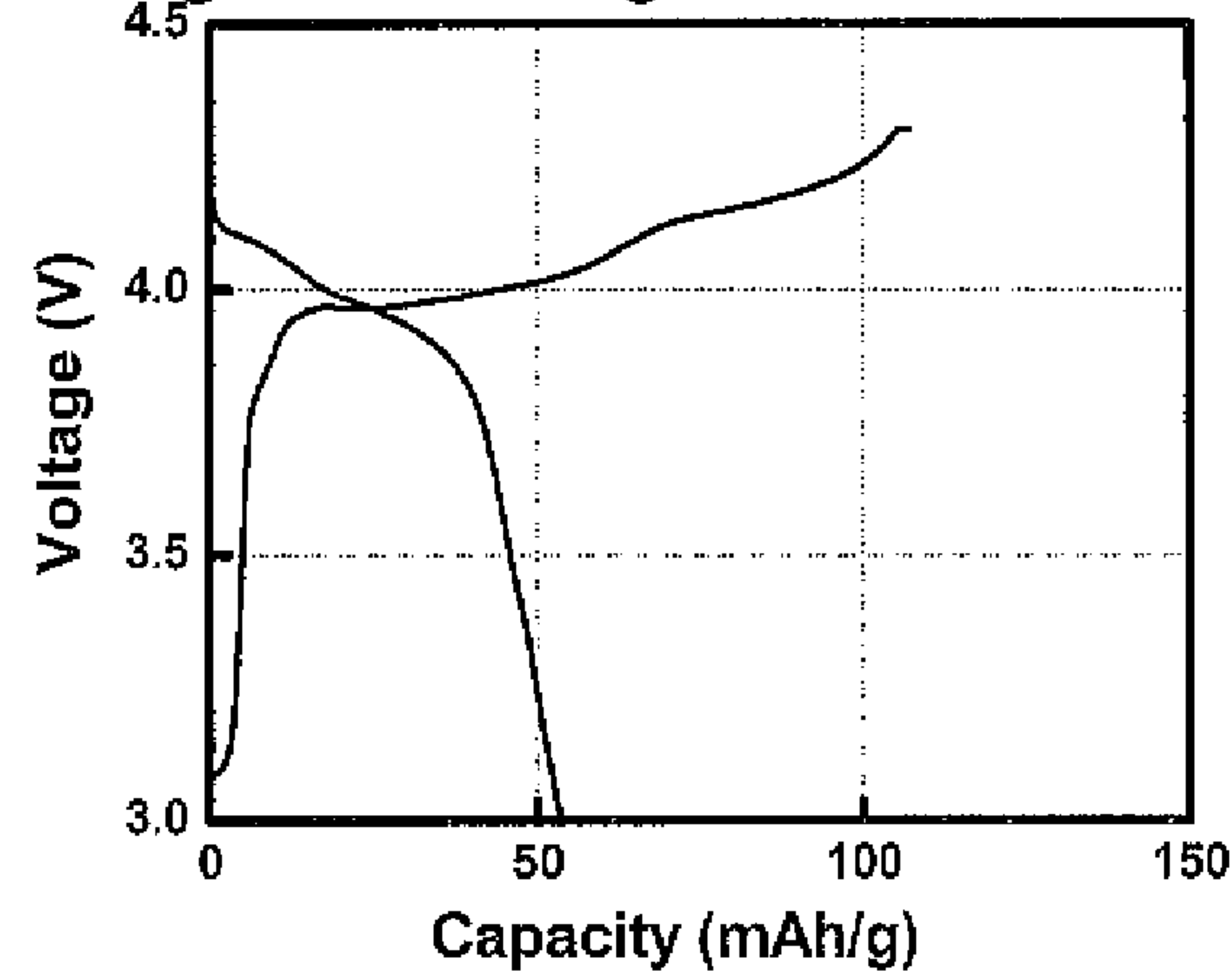
Initial Charge & Discharge Curves of Example 17
