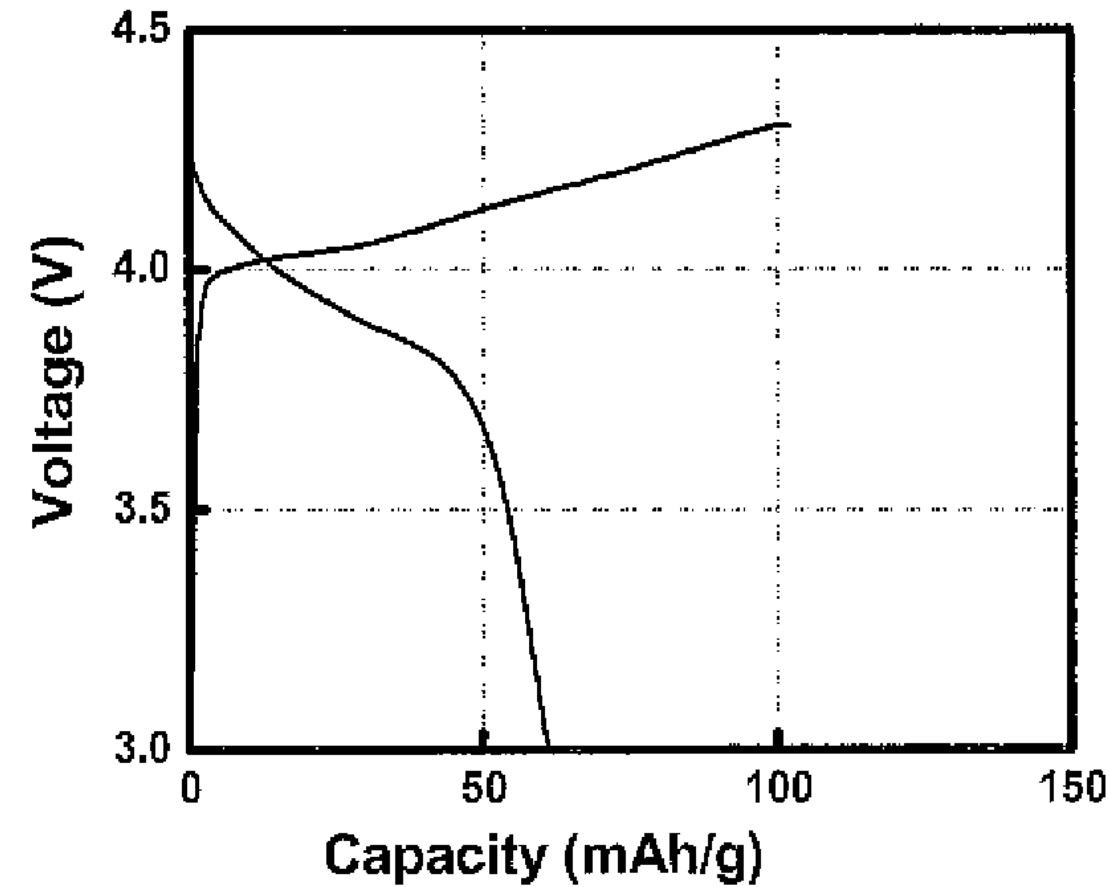
Initial Charge & Discharge Curves of Example 16
