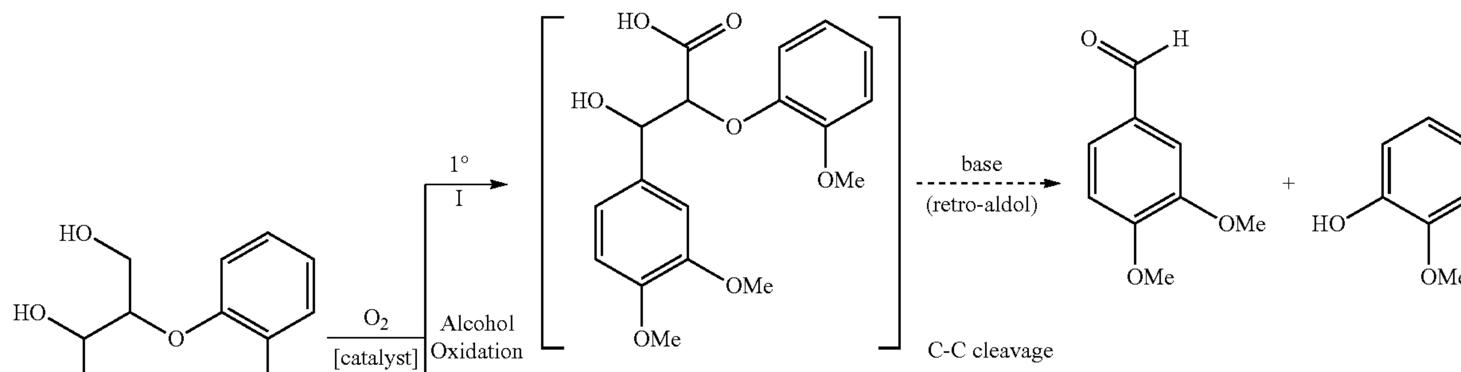
Scheme 3. Chemoselective alcohol oxidation strategies for lignin/lignin model compounds.
