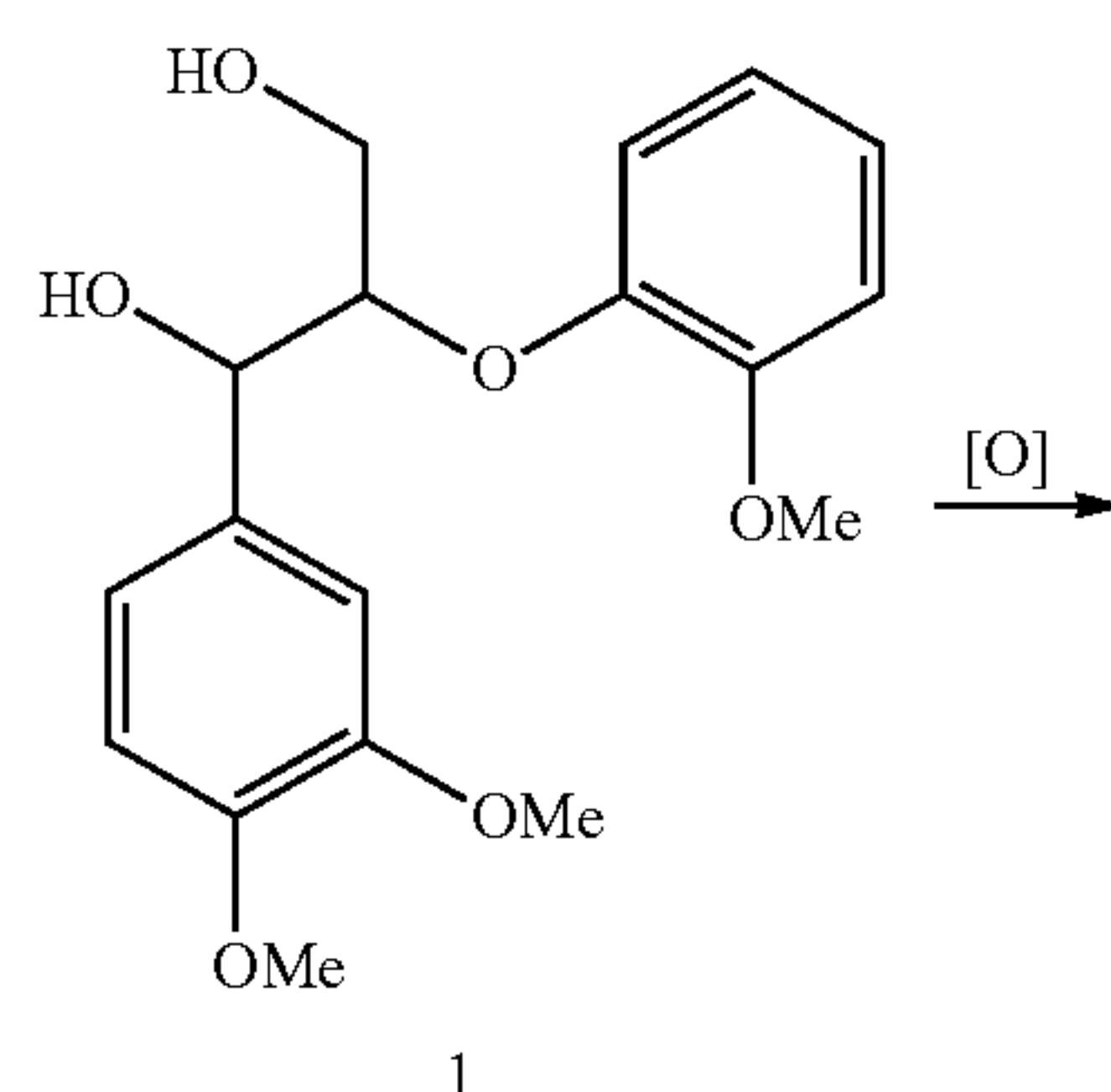
Scheme 4. Chemoselective oxidation of primary and secondary alcohol groups in model compound 1.
