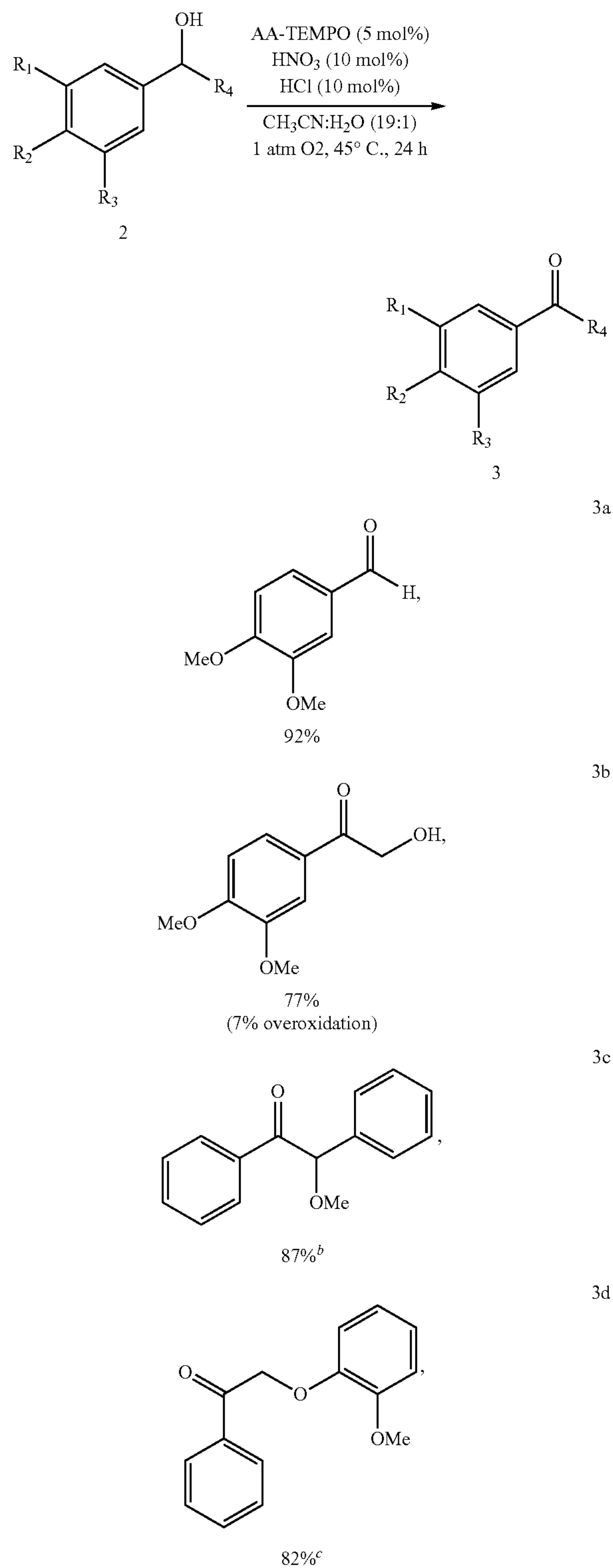
Scheme 5. Metal-free aerobic oxidation of lignin model compounds
