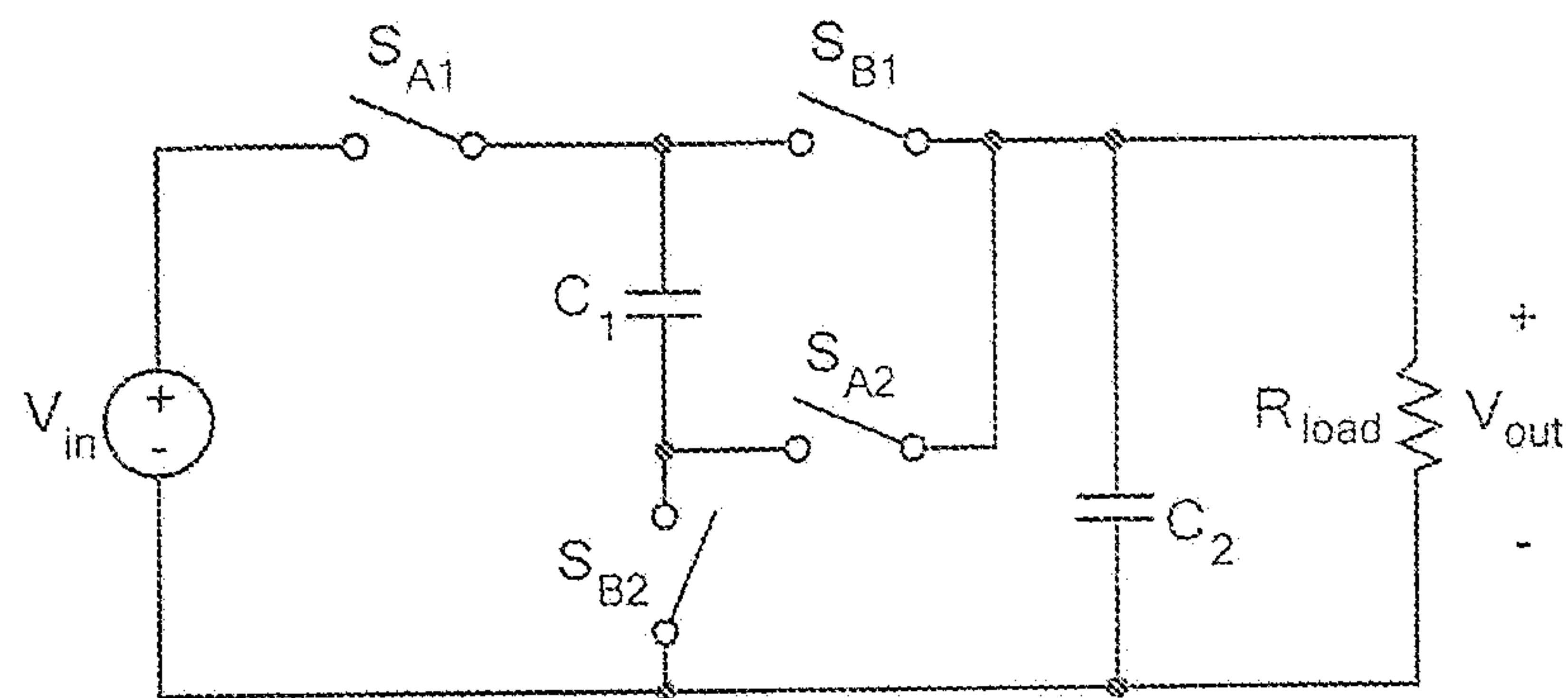
FIG. 1 PRIOR ART
