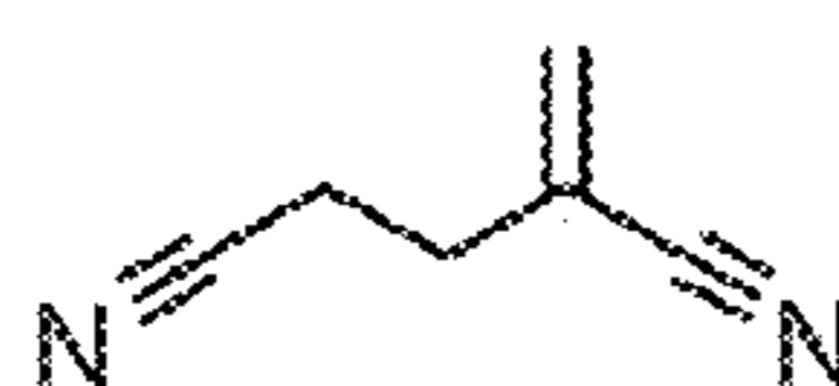
19 D 2-methyleneglutaronitrile
