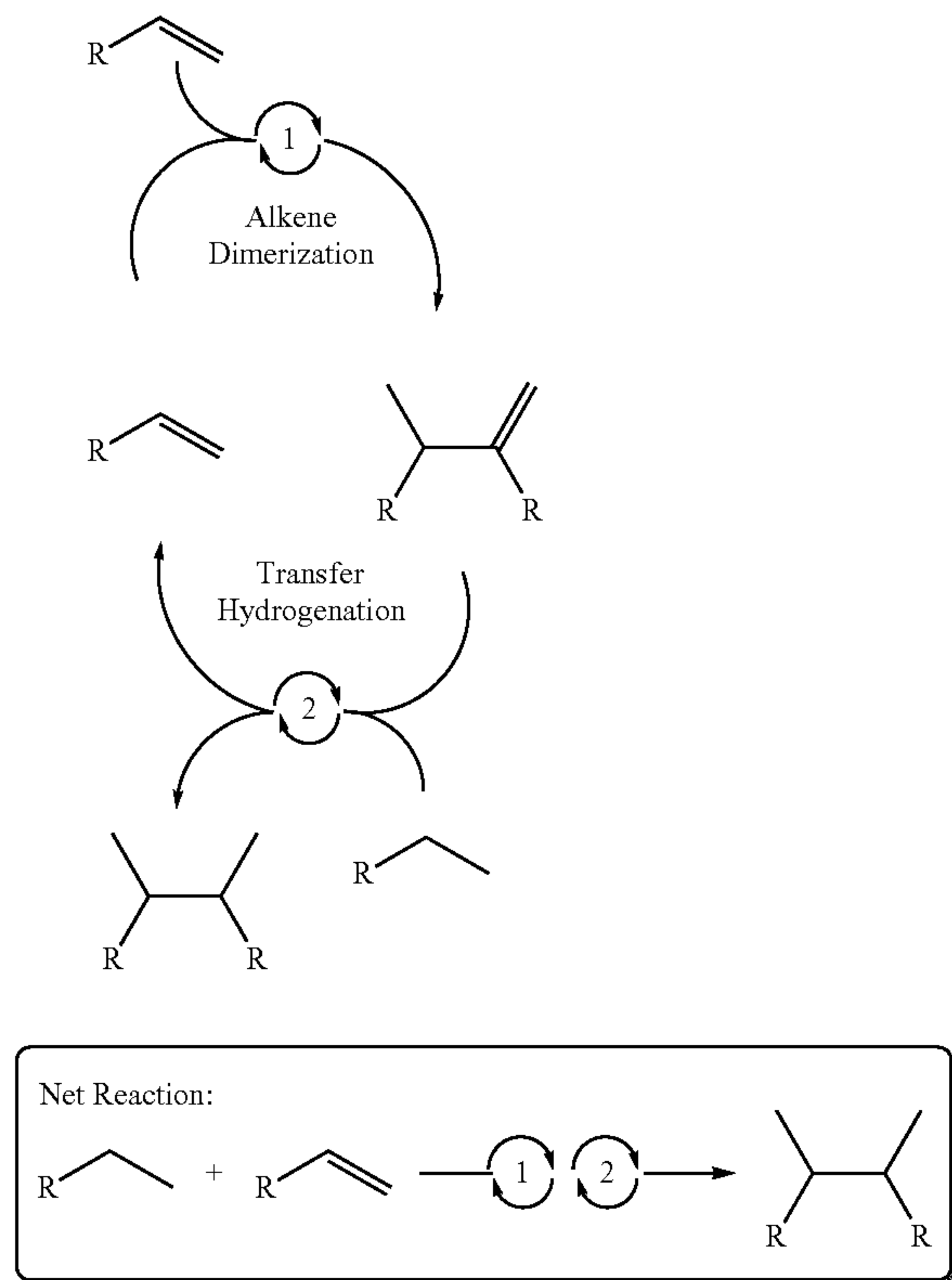
Scheme I: Idealized Tandem Catalytic Approach toward Alkane/Alkene Upgrading
