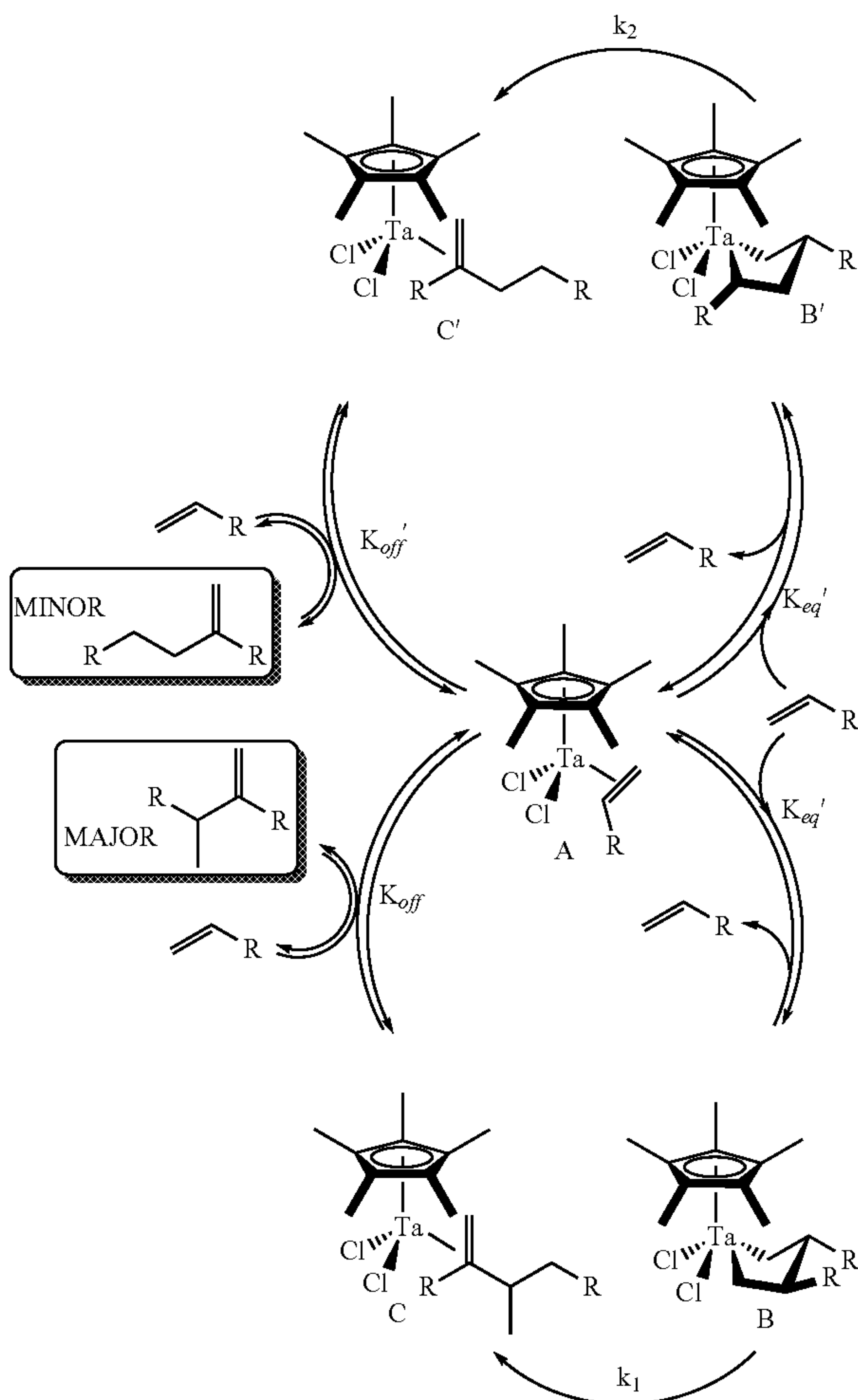
Scheme V: Postulated Catalytic Cycles for the Dimerization of 1-Alkenes into Two Regioisomers Catalyzed by 1
