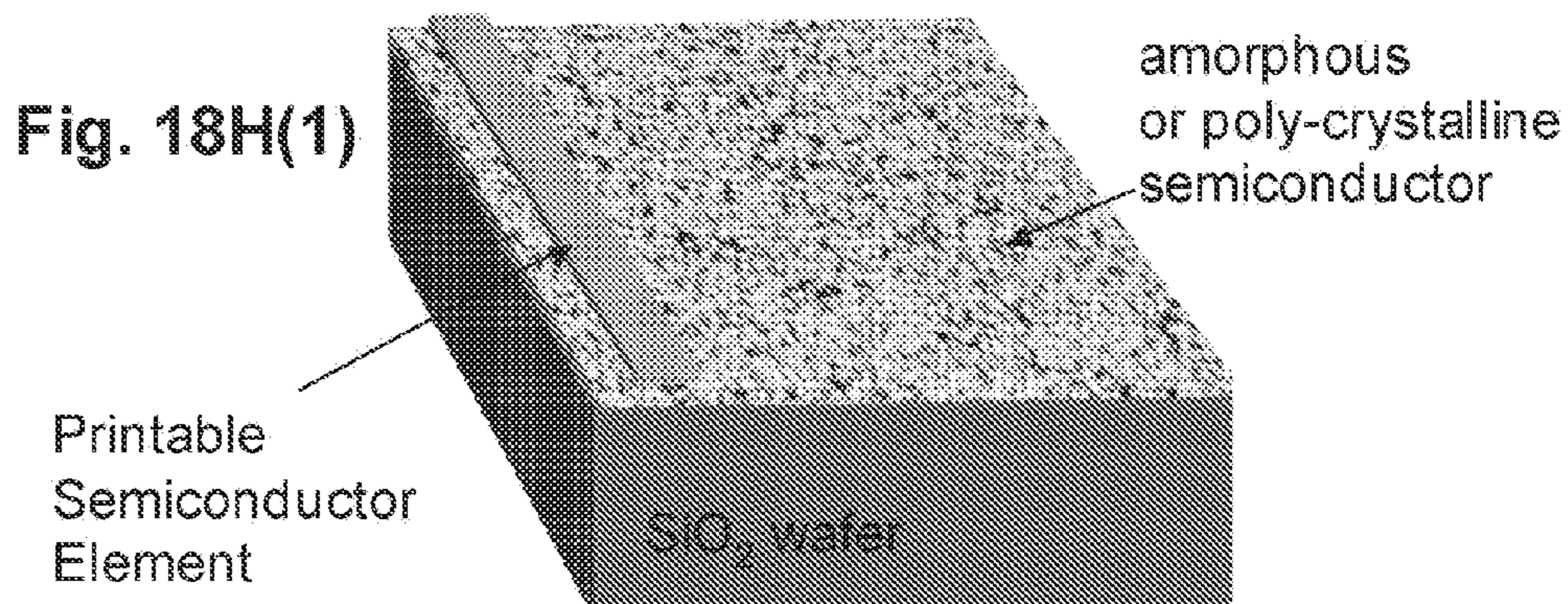
Transfer of a Printable Semiconductor Element (seed)
