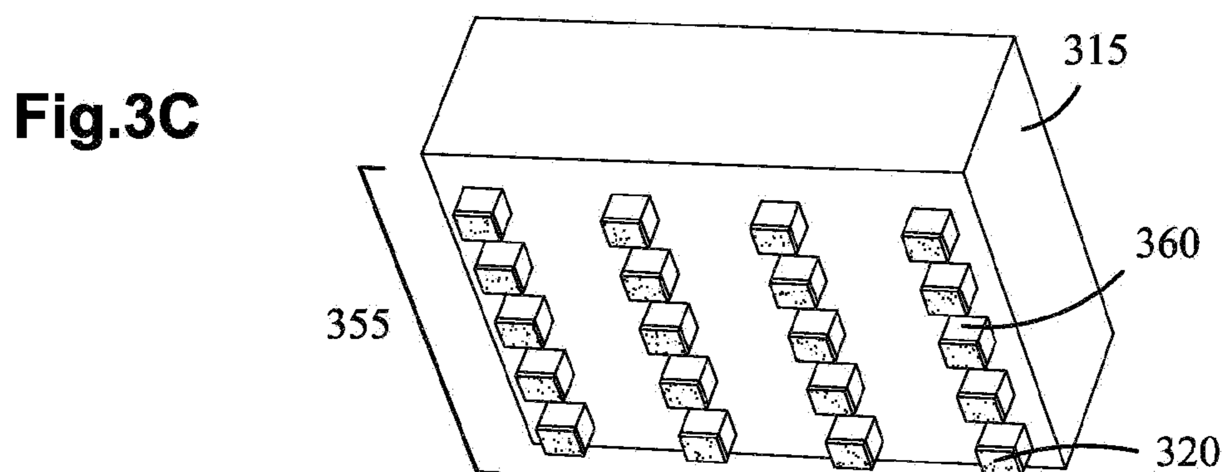
c) Structured stamp inked with an adhesive
