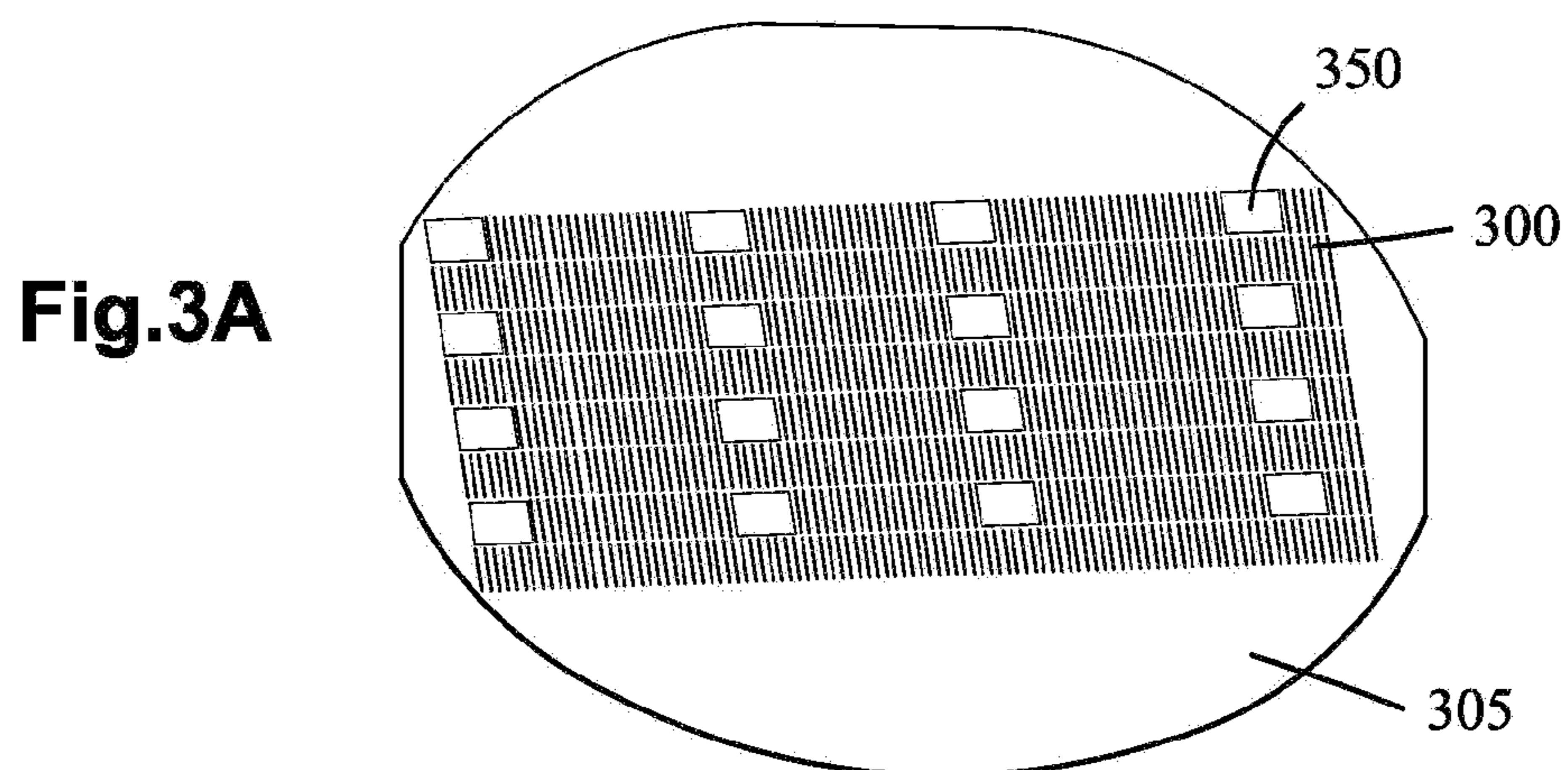
a) Selective coating of the mother substrate with an adhesive material
