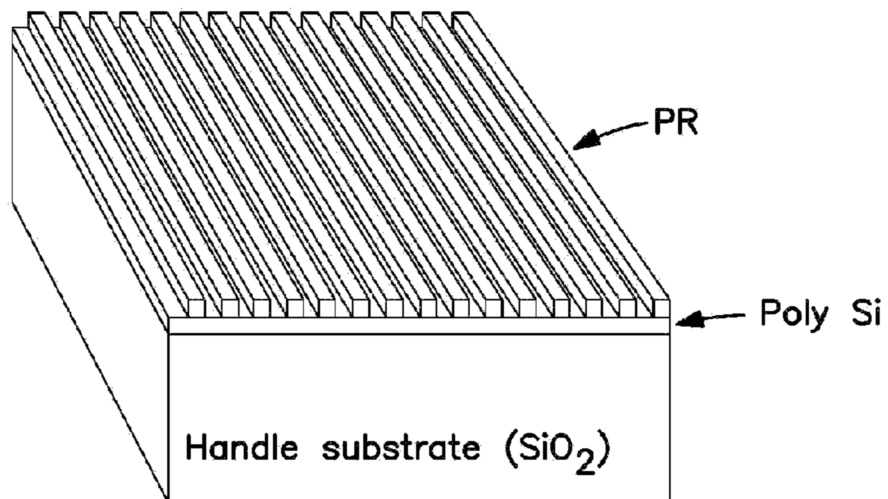
i) \mu s-Si shape definition
