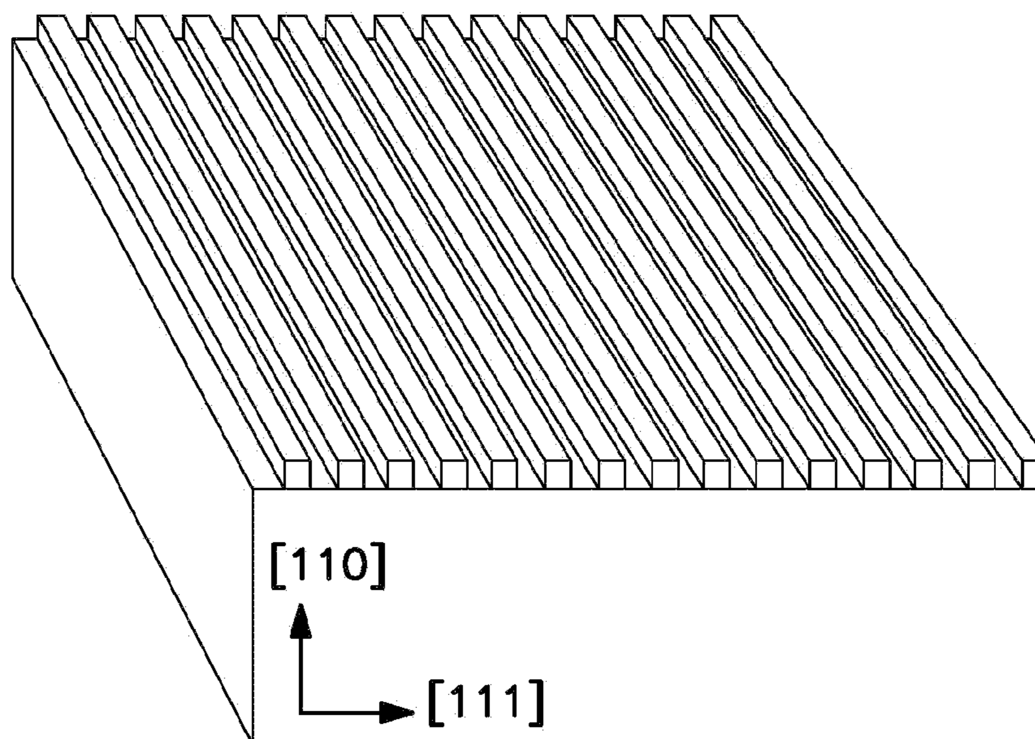
i) \mu\text{s-Si} shape definition
