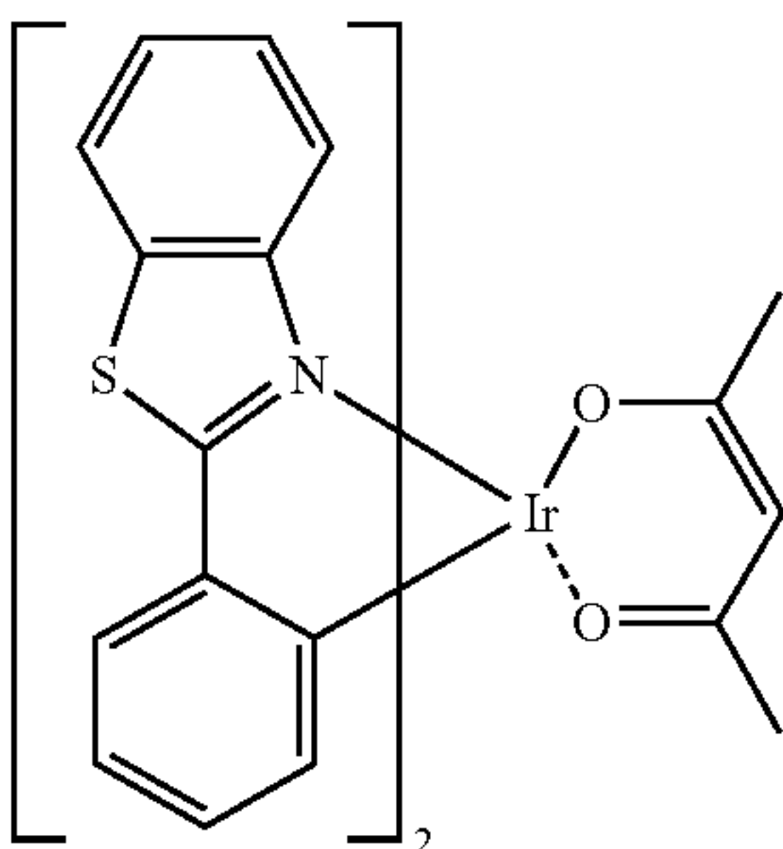
Ir(BT) 2 (acac)
