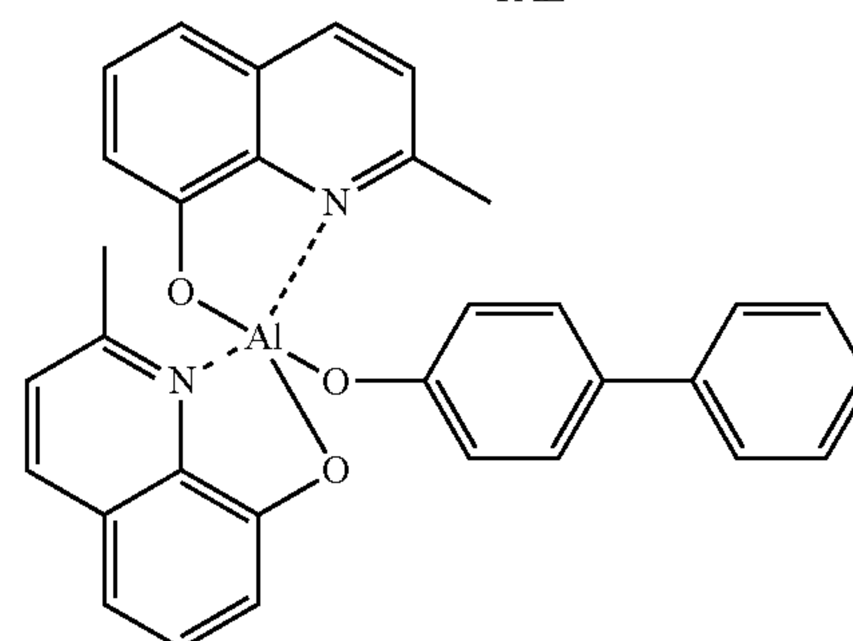
BAIq
