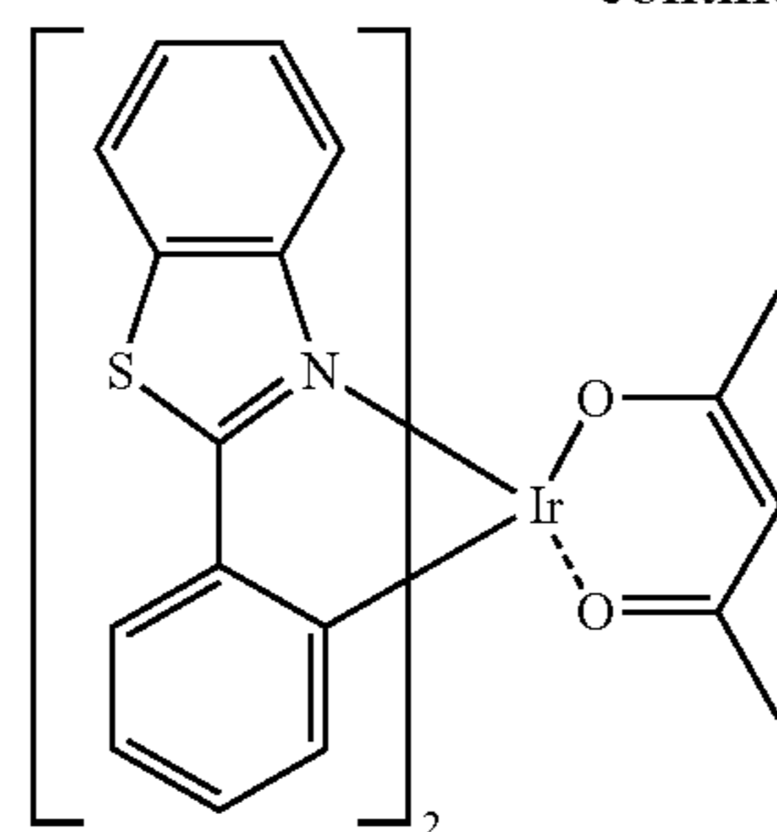
Ir(BT) 2 (acac)
