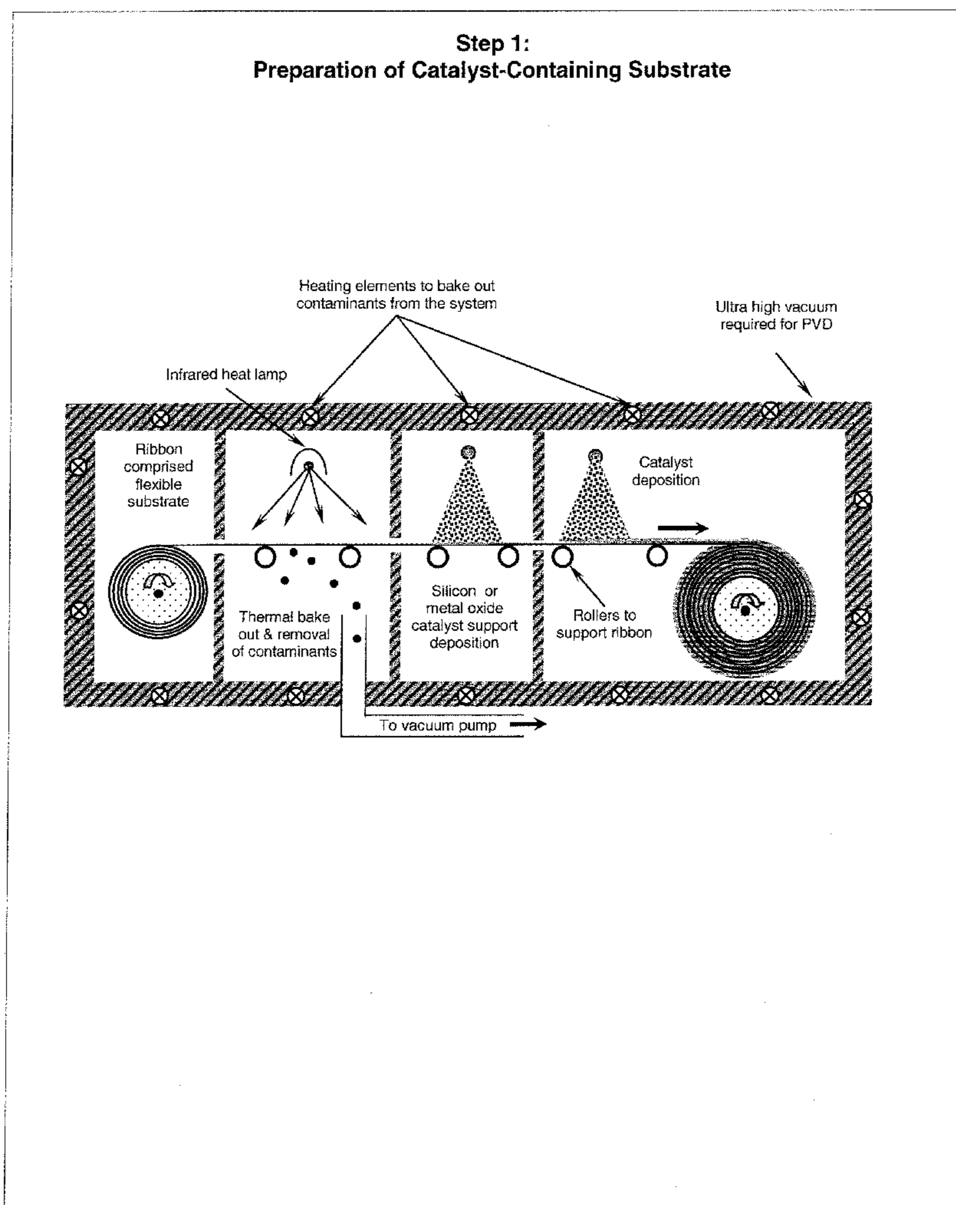
System for treating growth substrate prior to carbon nanotube growth.
