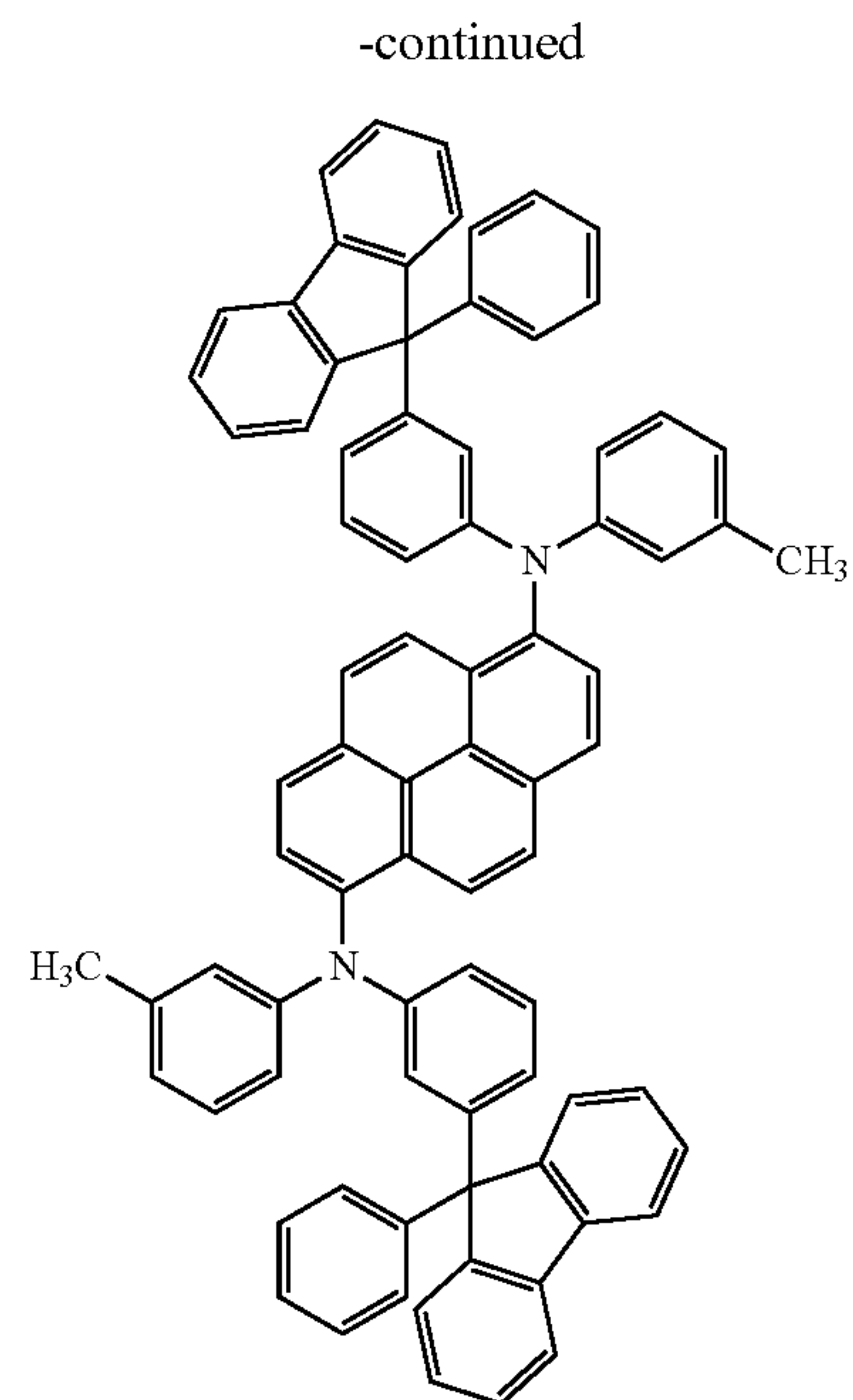
1,6mMemFLPAPrn
