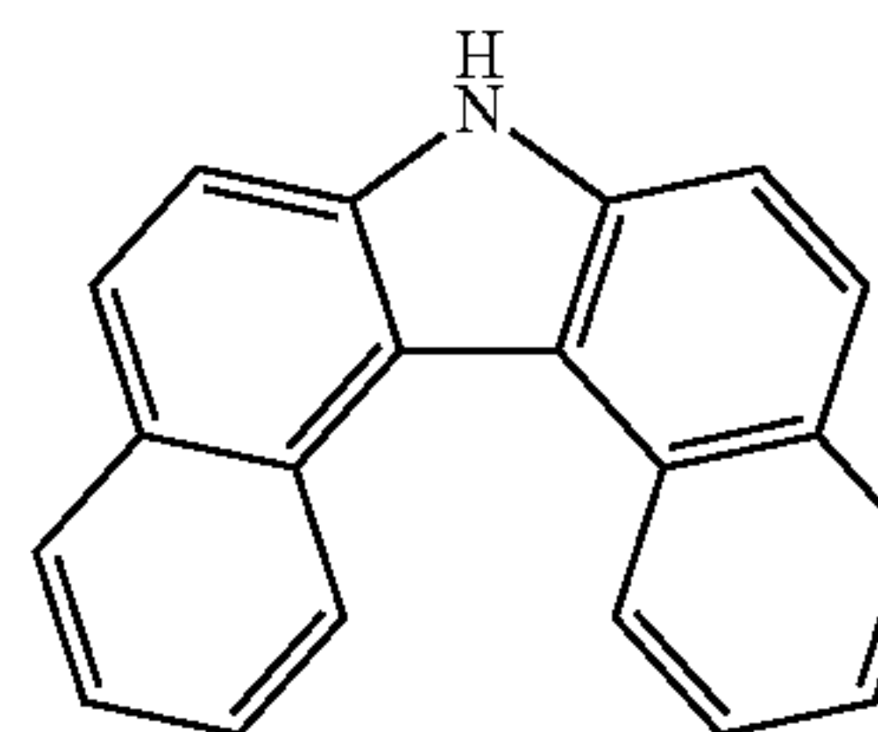
\text{C}_{20}\text{H}_{13}\text{N} Exact Mass: 267.10
