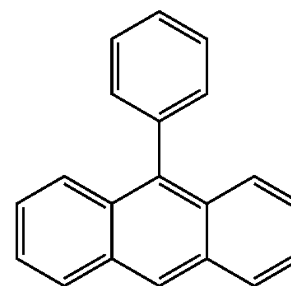
\text{C}_{20}\text{H}_{14} Exact Mass: 254.11
