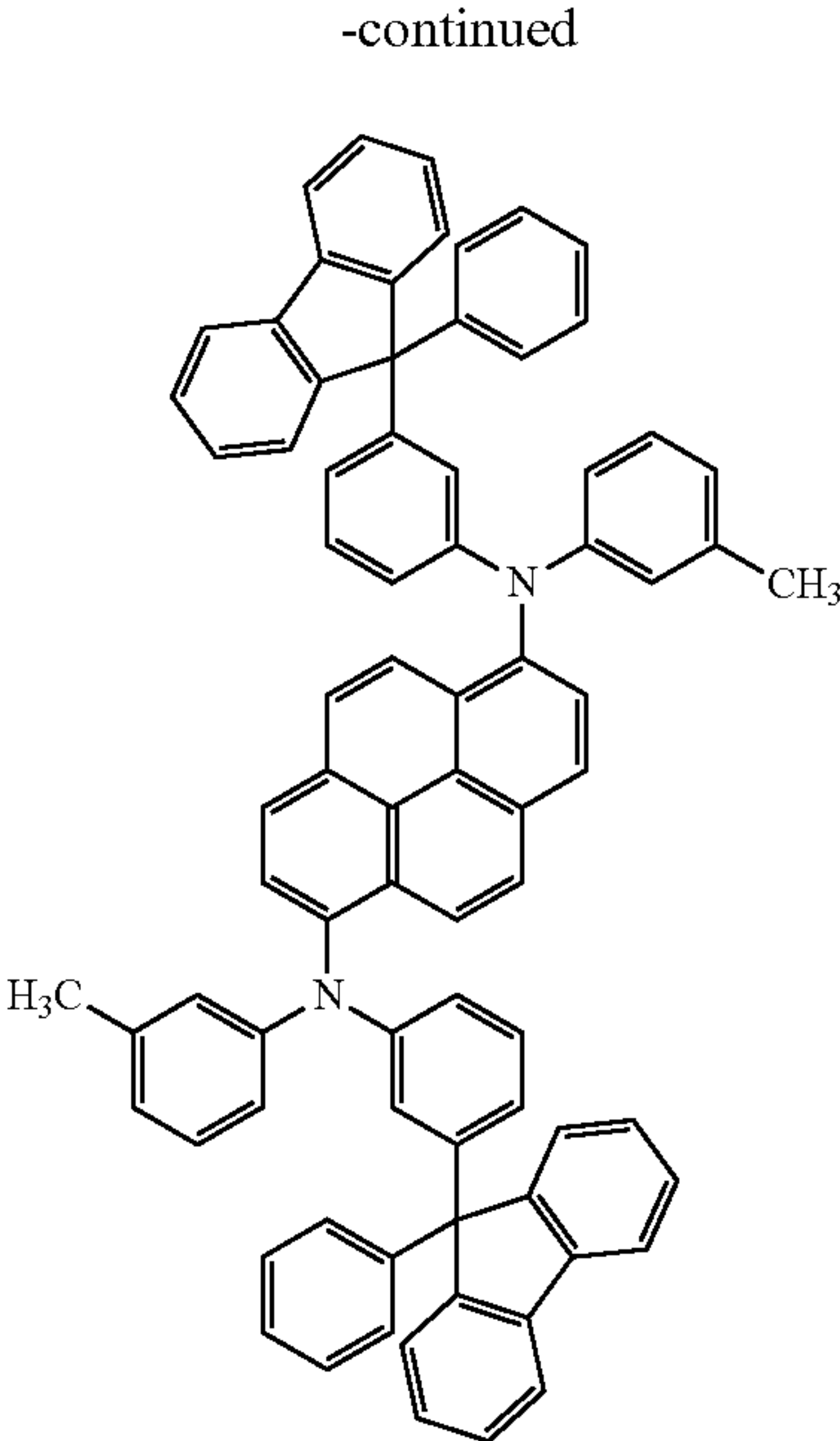
1,6mMemFLPAPrn
