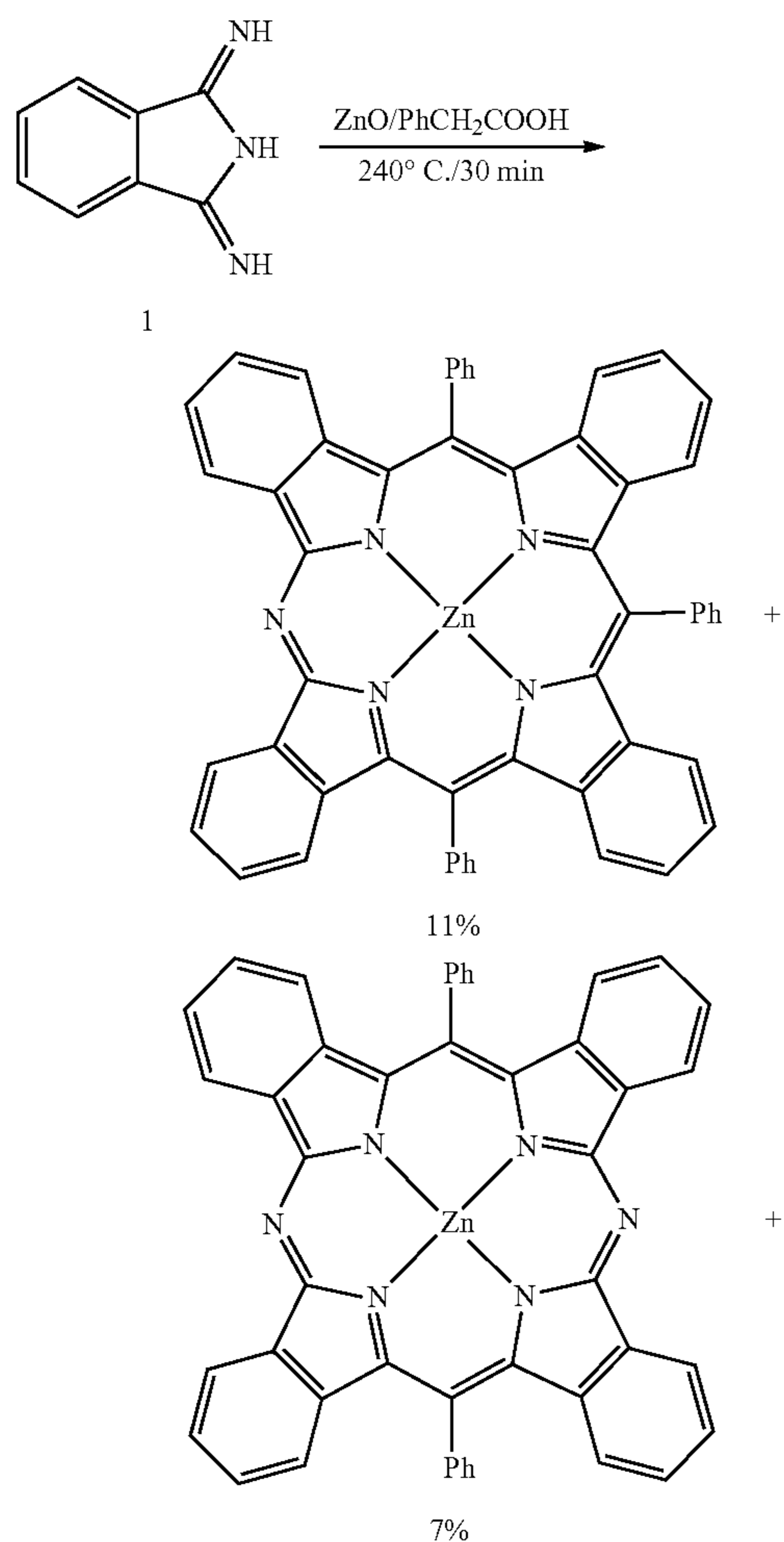
Scheme 1. Preparation of Exemplary Azaporphyrins
