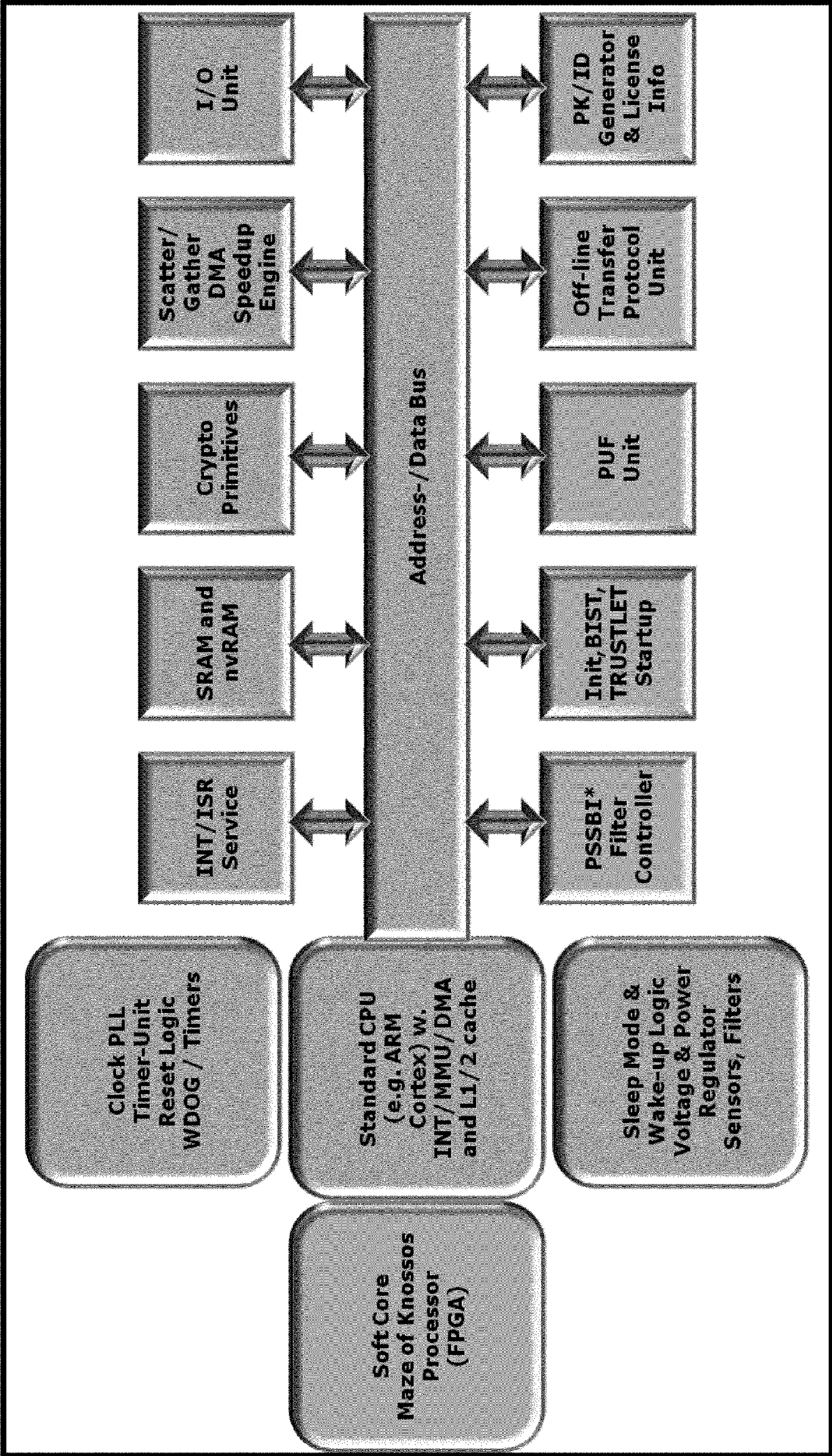
Figure 1: Block diagram of the CASTOR HSM.
