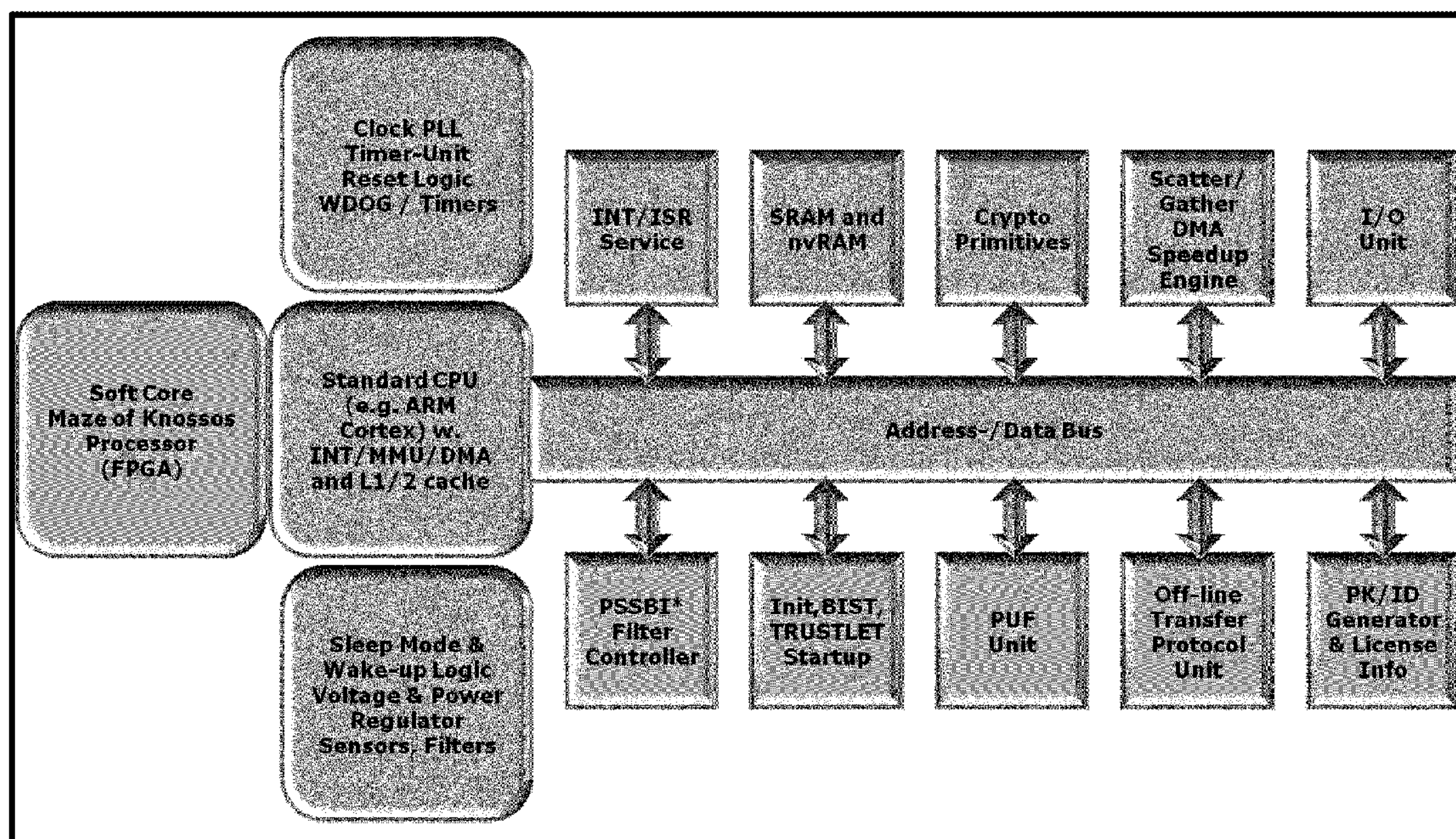
Block diagram of the CASTOR HSM.
