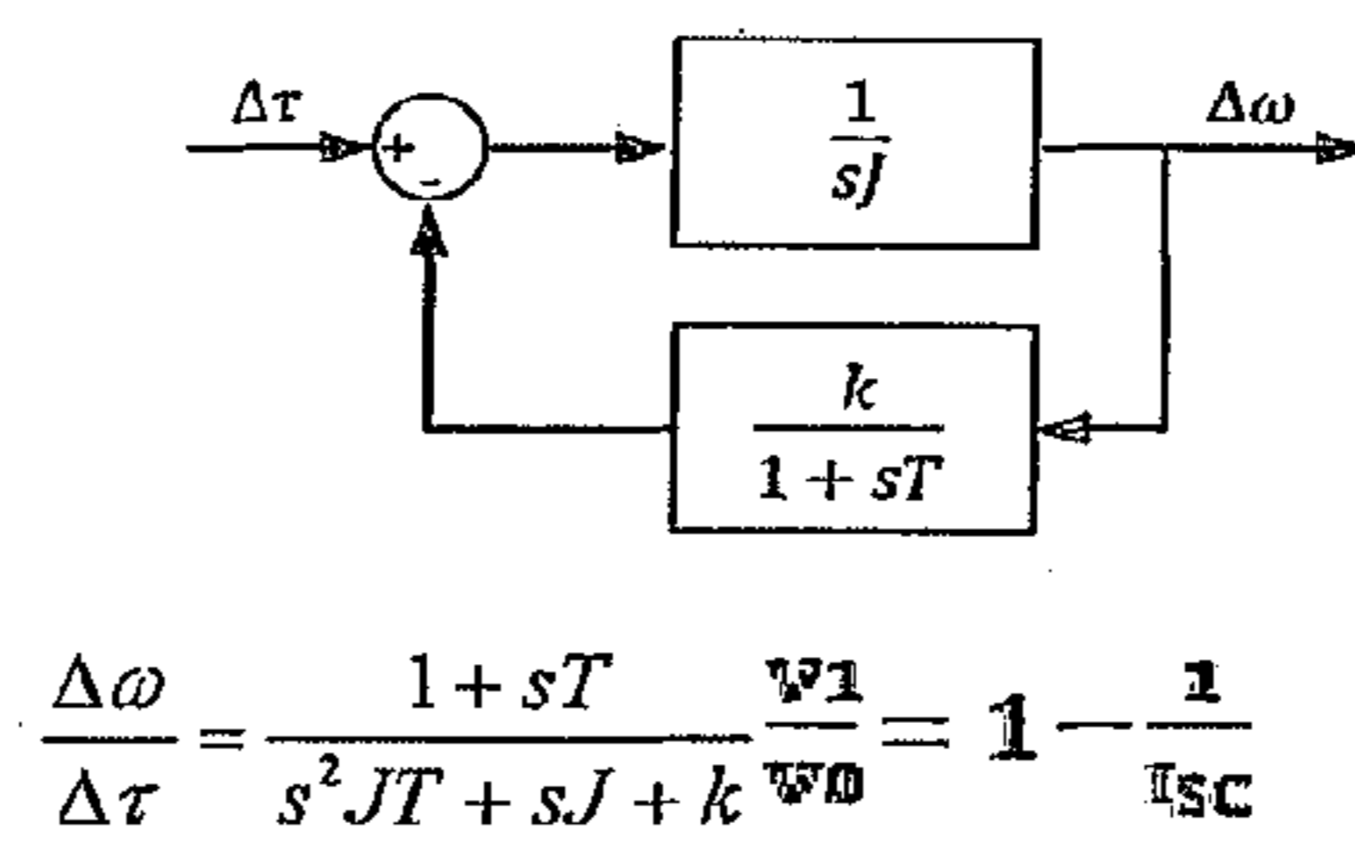
Figure 2. Block diagram, and transfer function of a DDC controller
