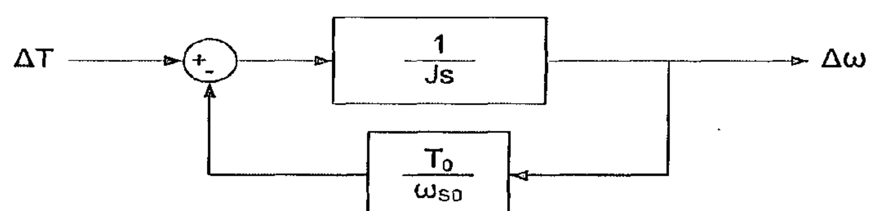
Figure 4 - Block diagram and Transfer function for a LDC Controller
