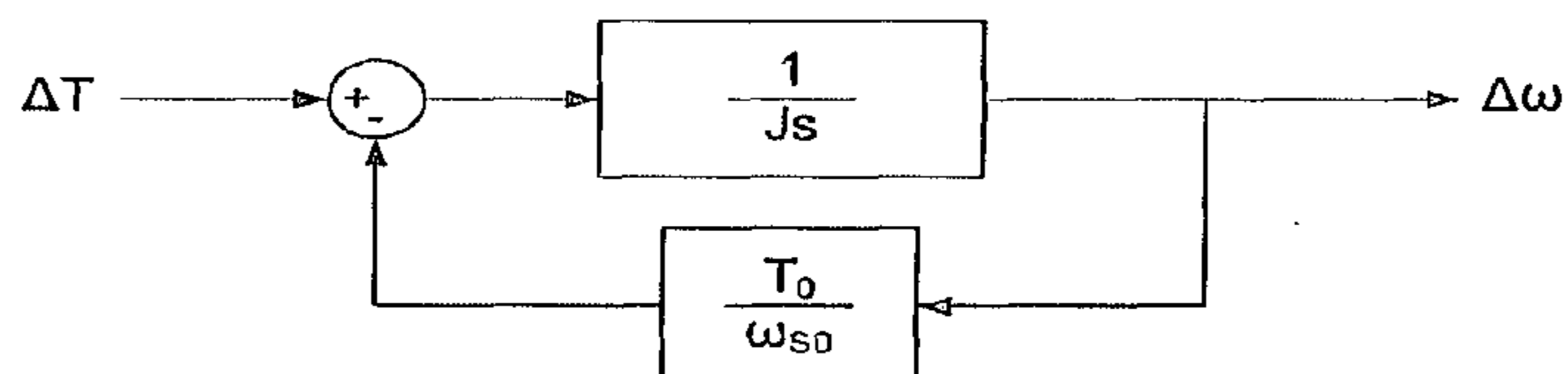
Figure 4 - Block diagram and Transfer function for a LDC Controller
