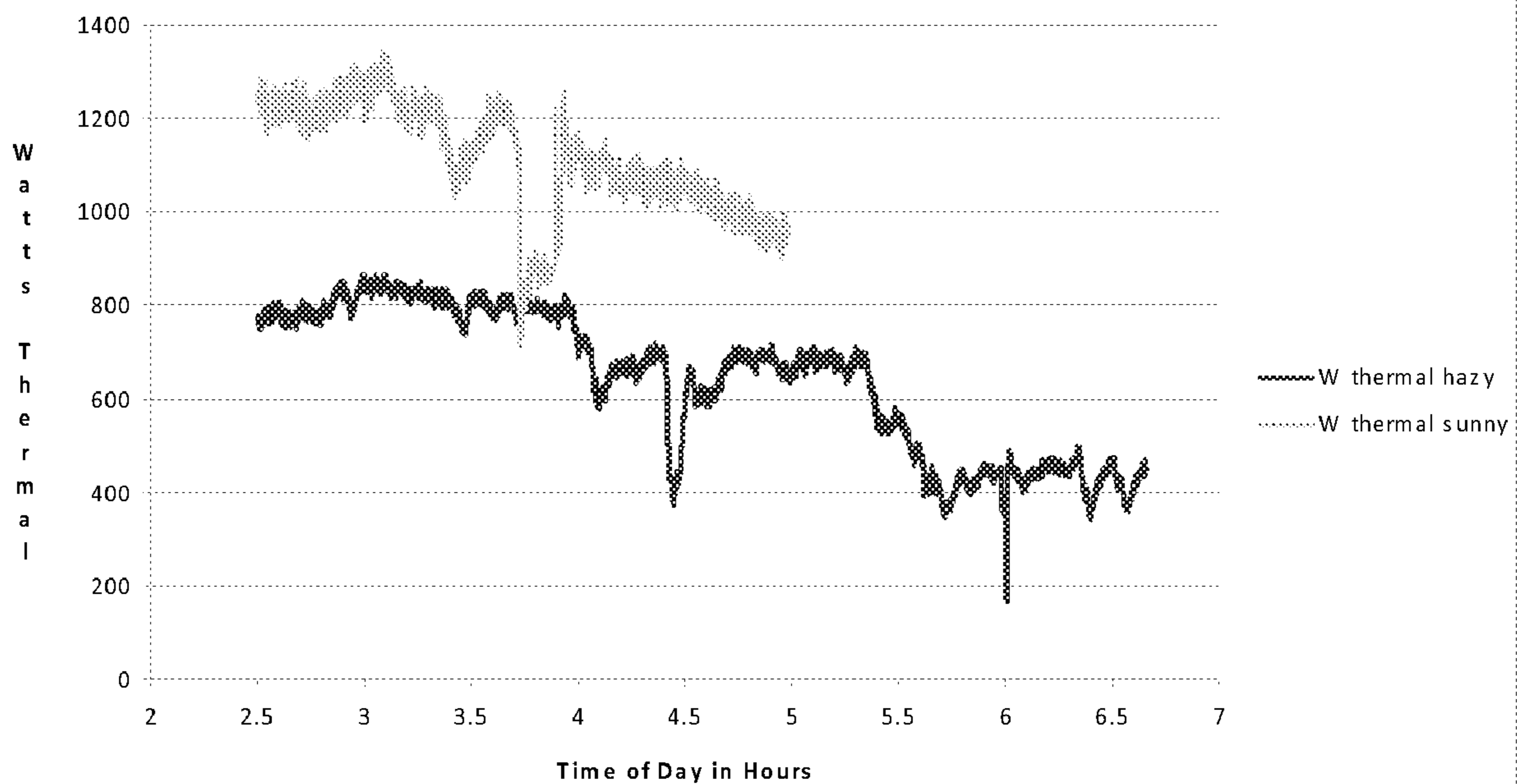
Comparison of Thermal Energy Output sunny vs. overcast
