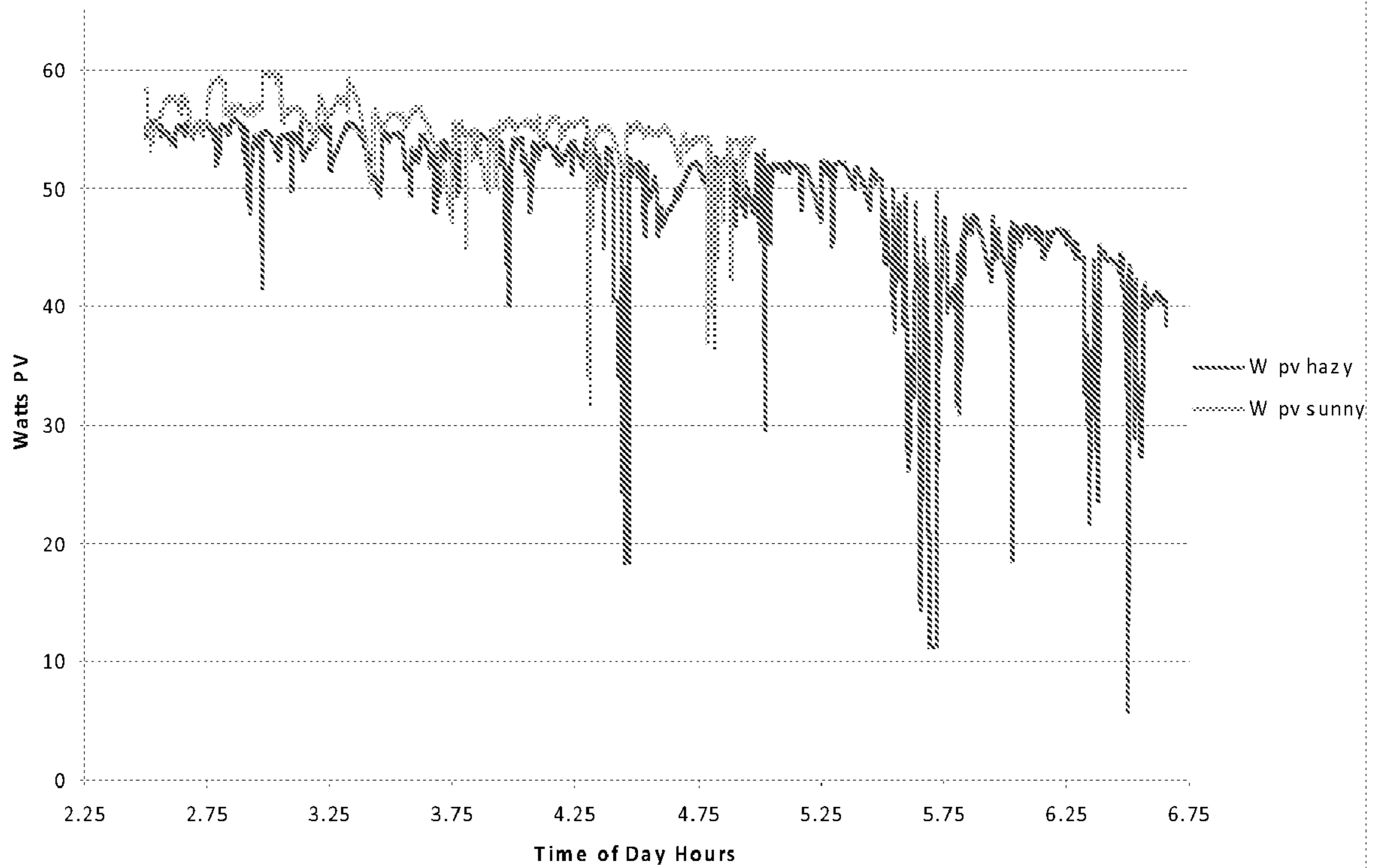
Watts Electrical Hazy vs Sunny Day
