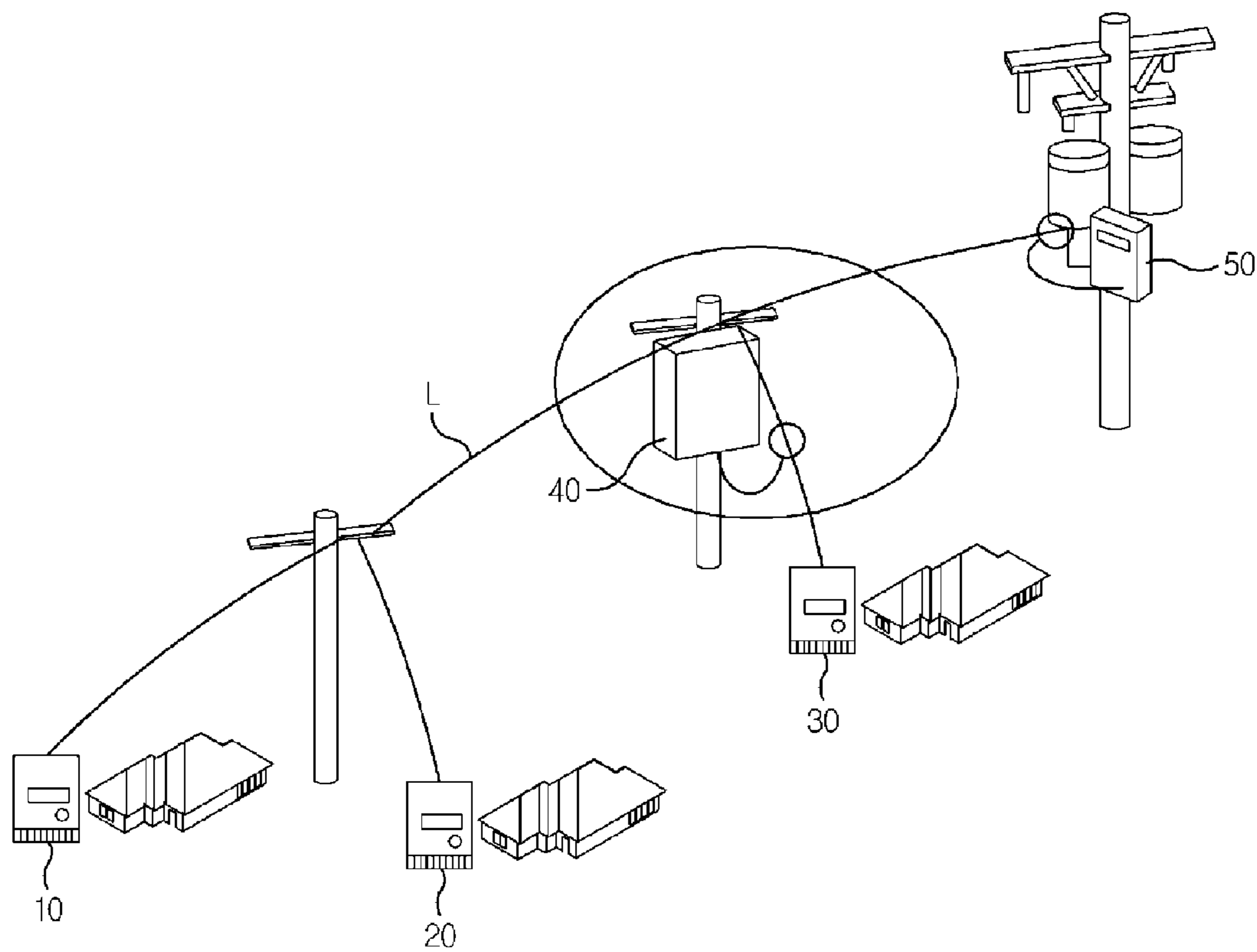
FIG. 1 (PRIOR ART)
