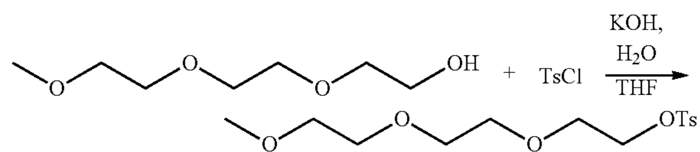
Scheme 1. Monomer synthesis
