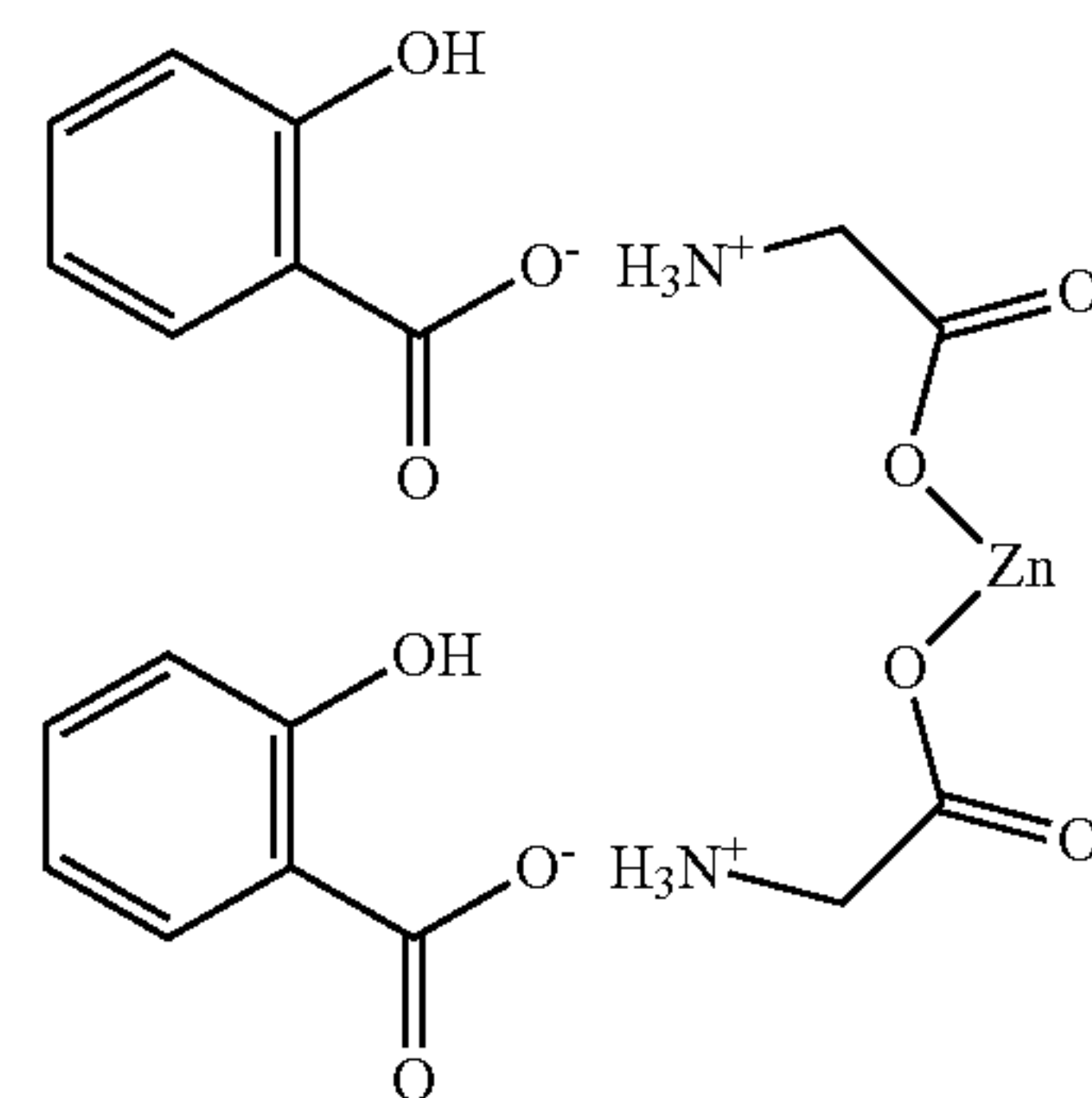
Zinc Glycine Salicylate Salt
