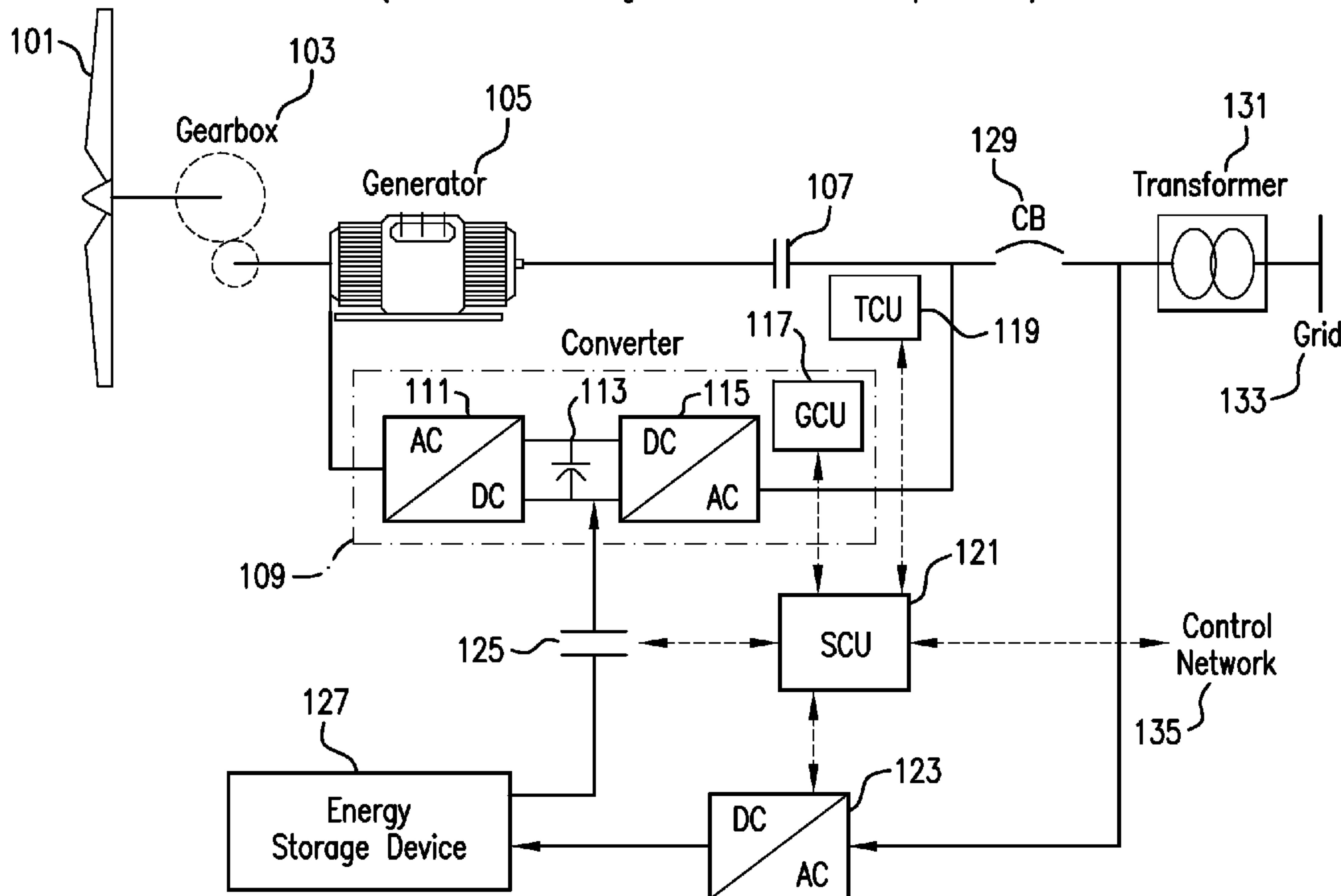
Type 3 Wind Turbine Generator (Double-Fed Configuration - Isolated Operations)
