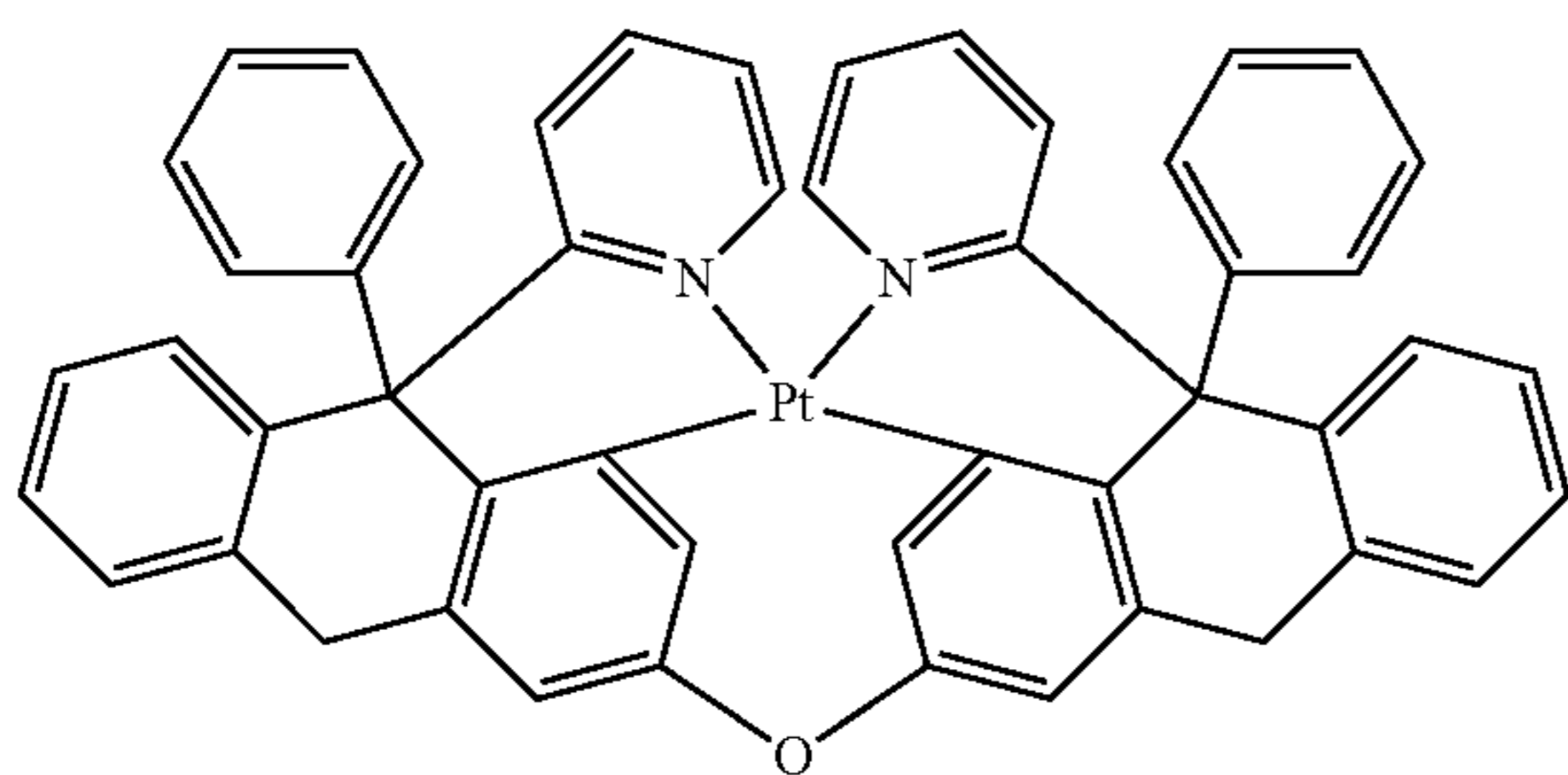
Compound 96
