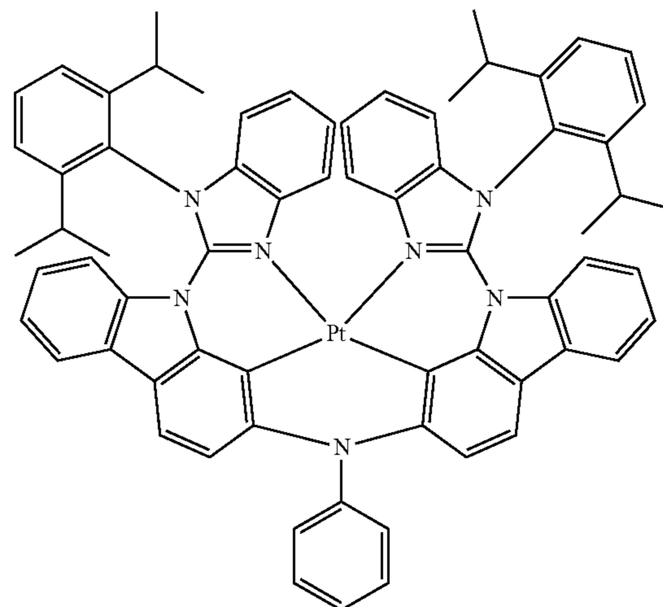
Compound 57
