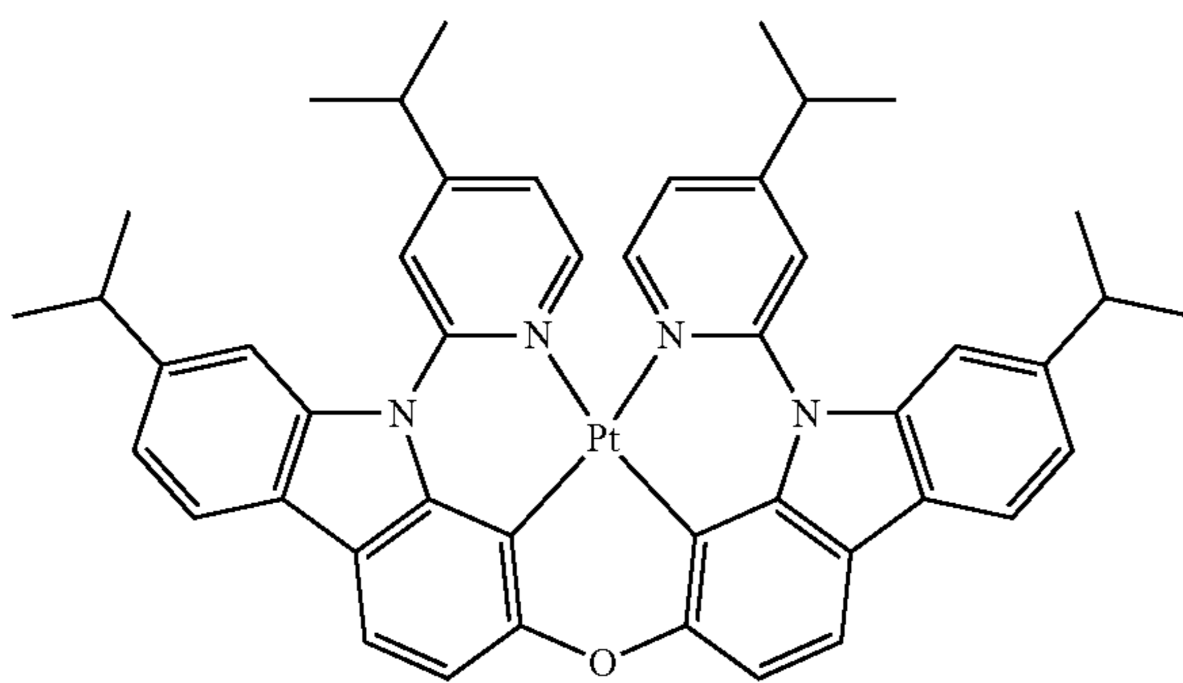
Compound 20
