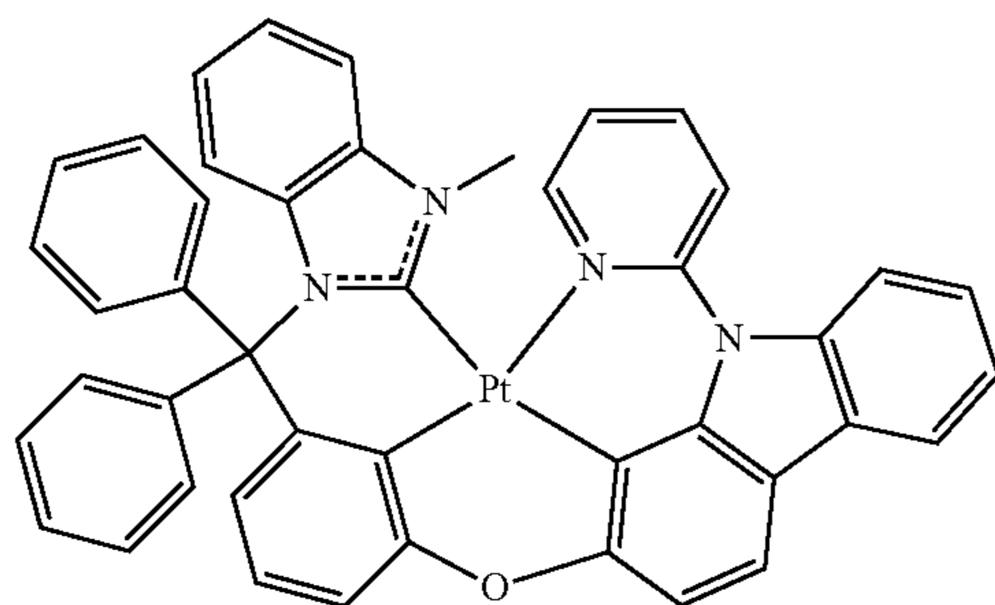
Compound 78
