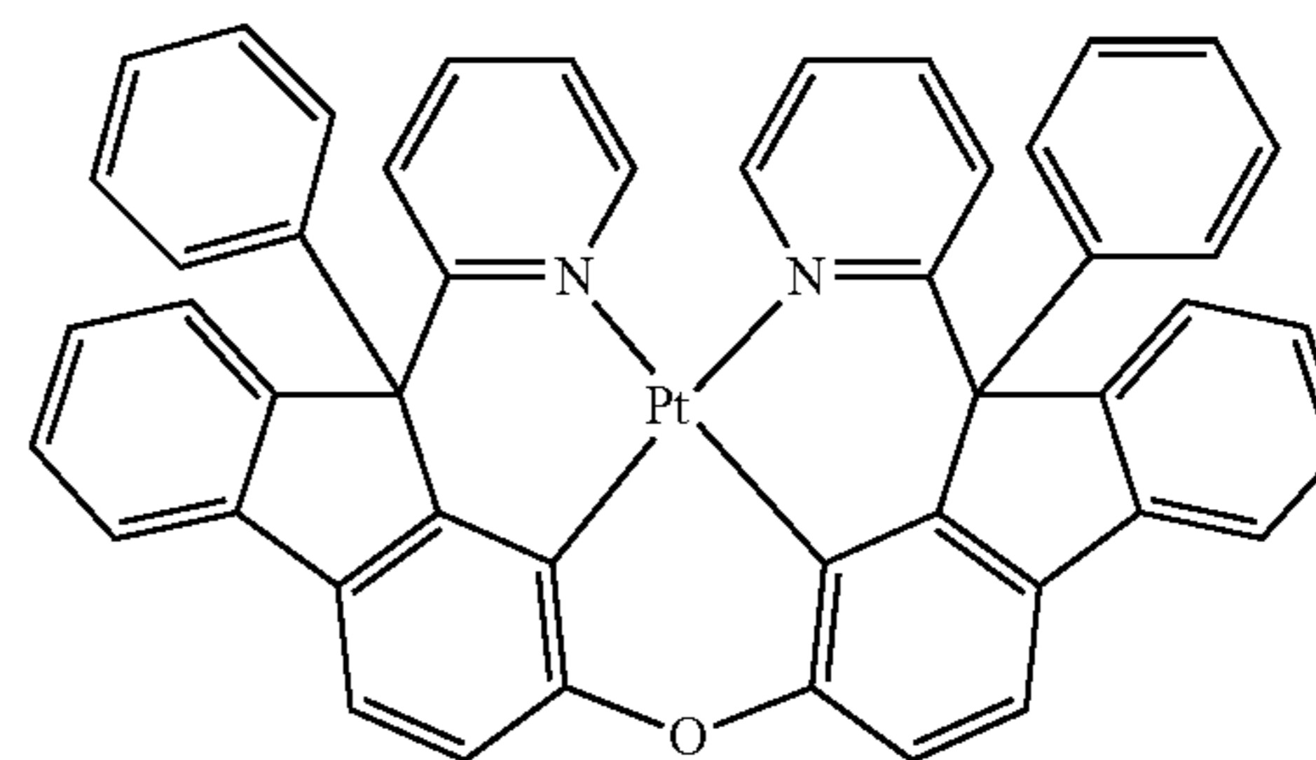
Compound 93
