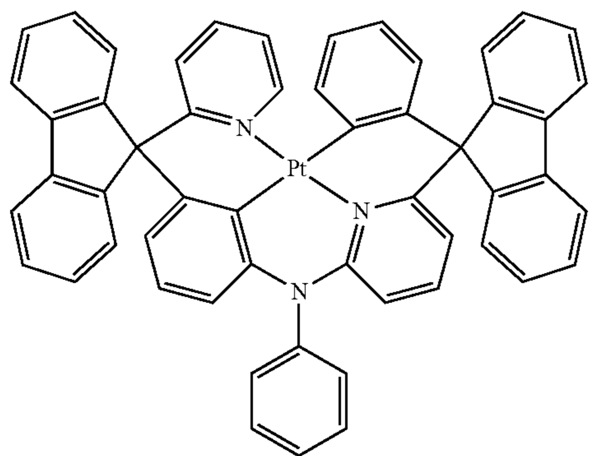
Compound 132
