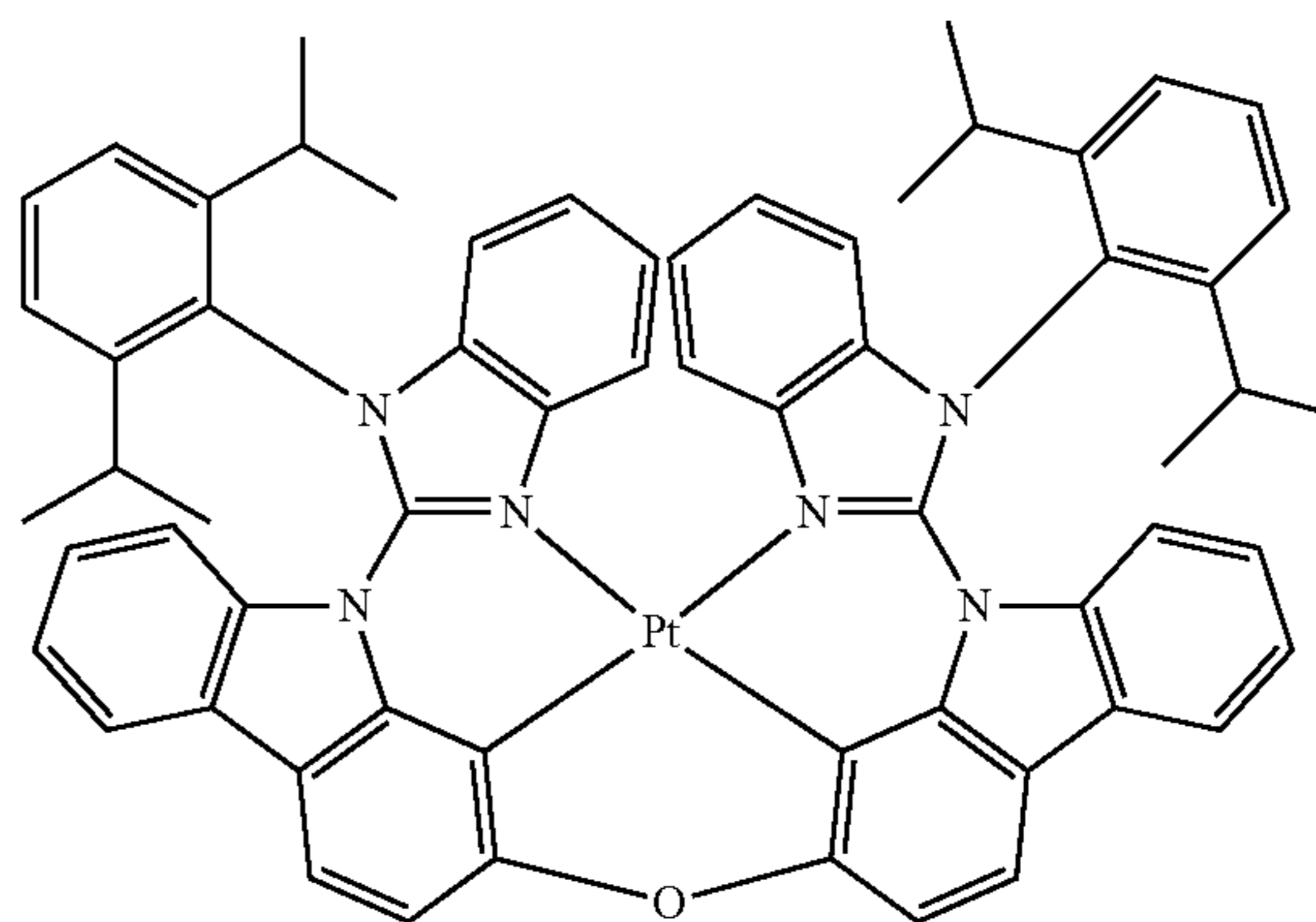
Compound 56
