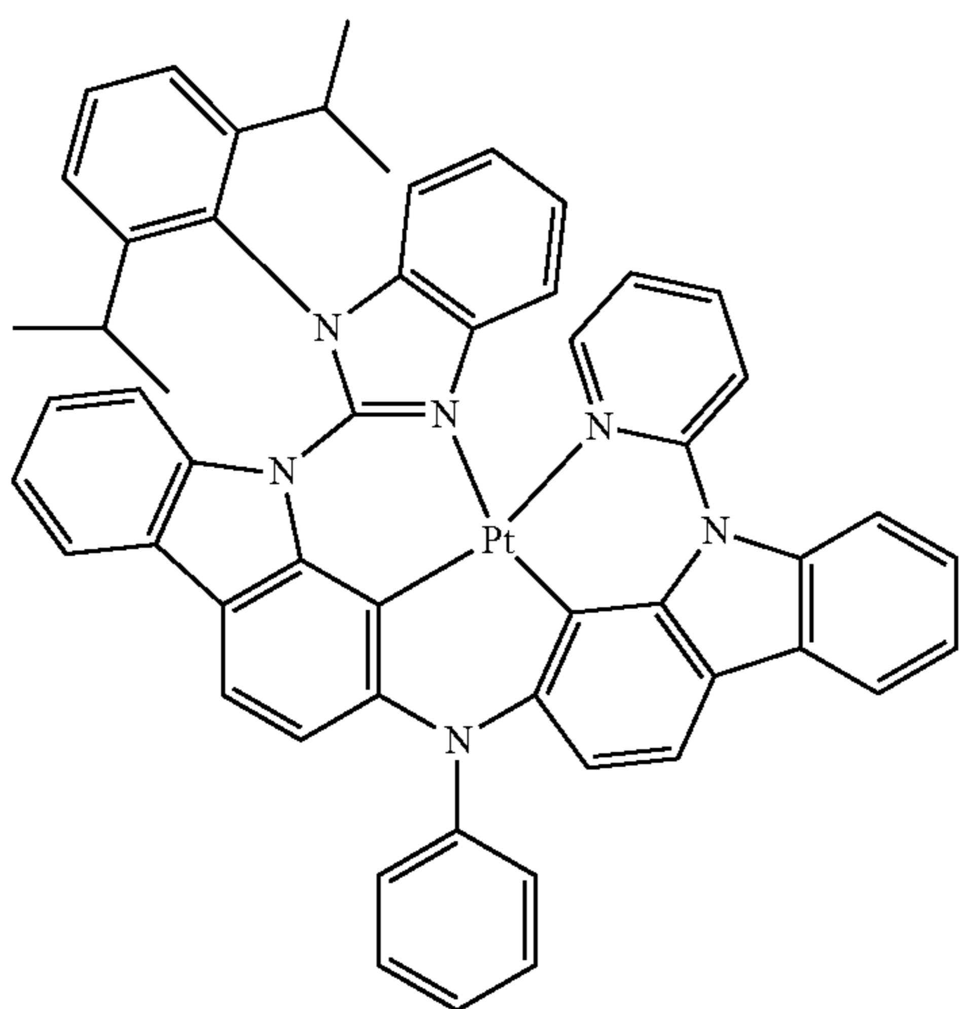
Compound 62
