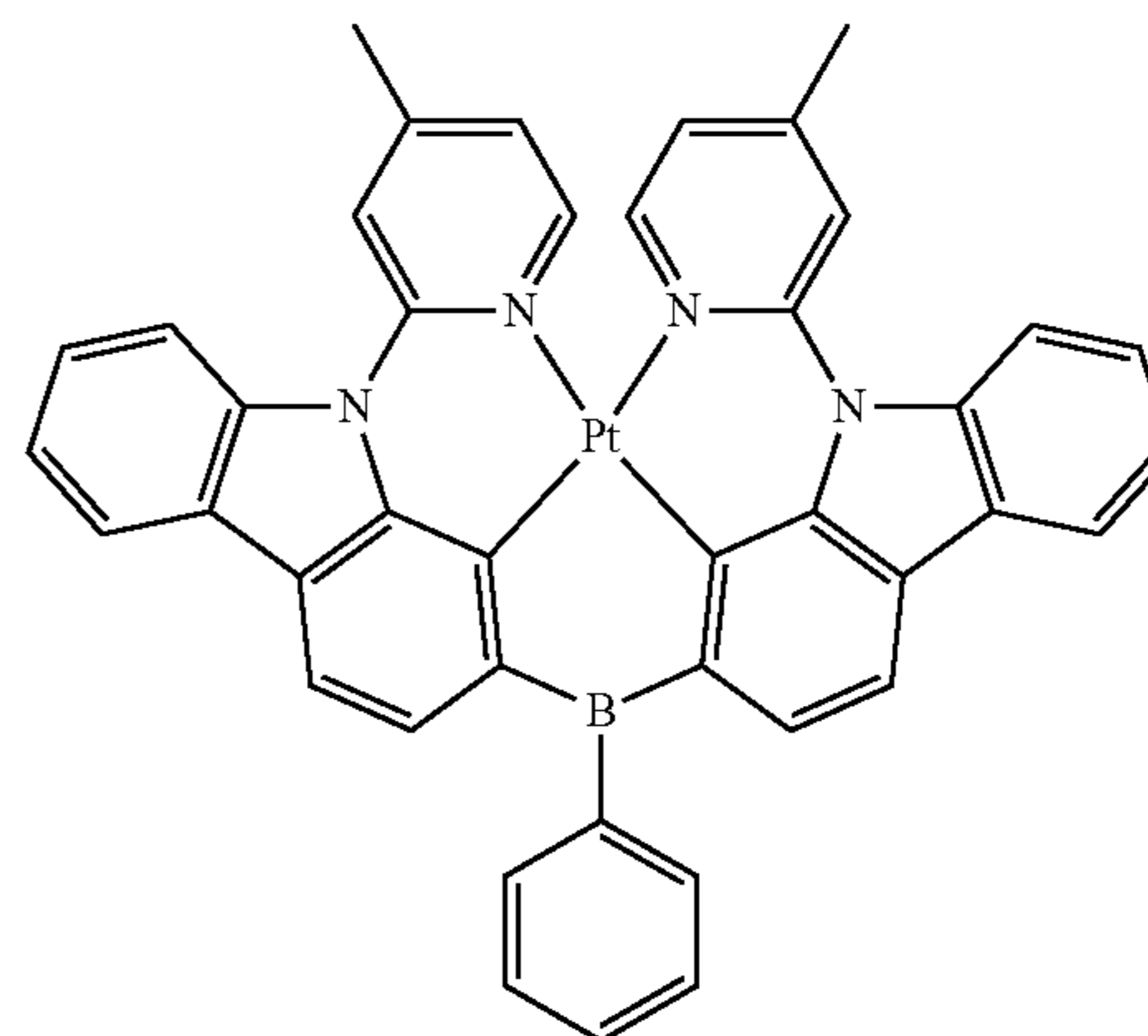
Compound 11
