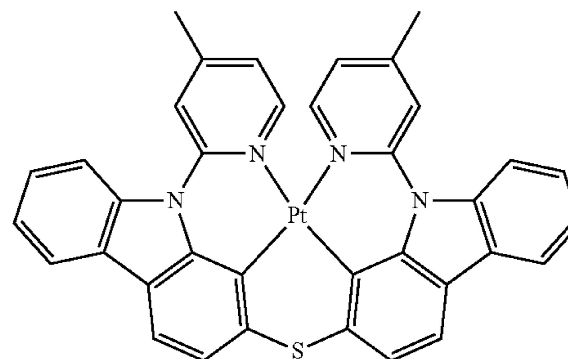
Compound 10
