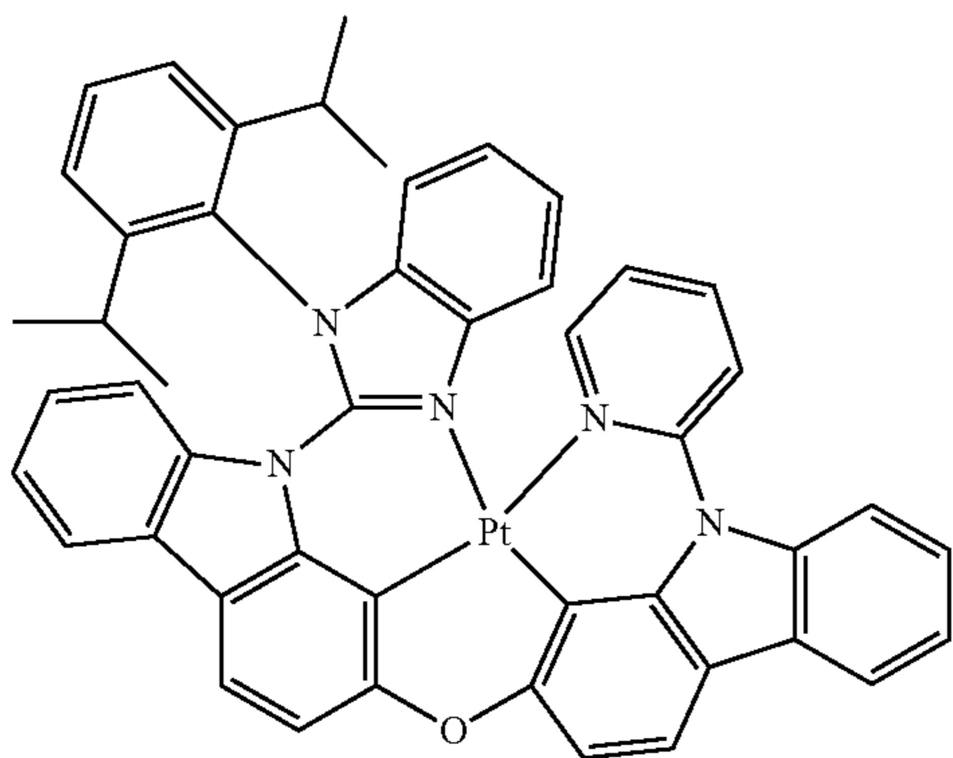
Compound 58
