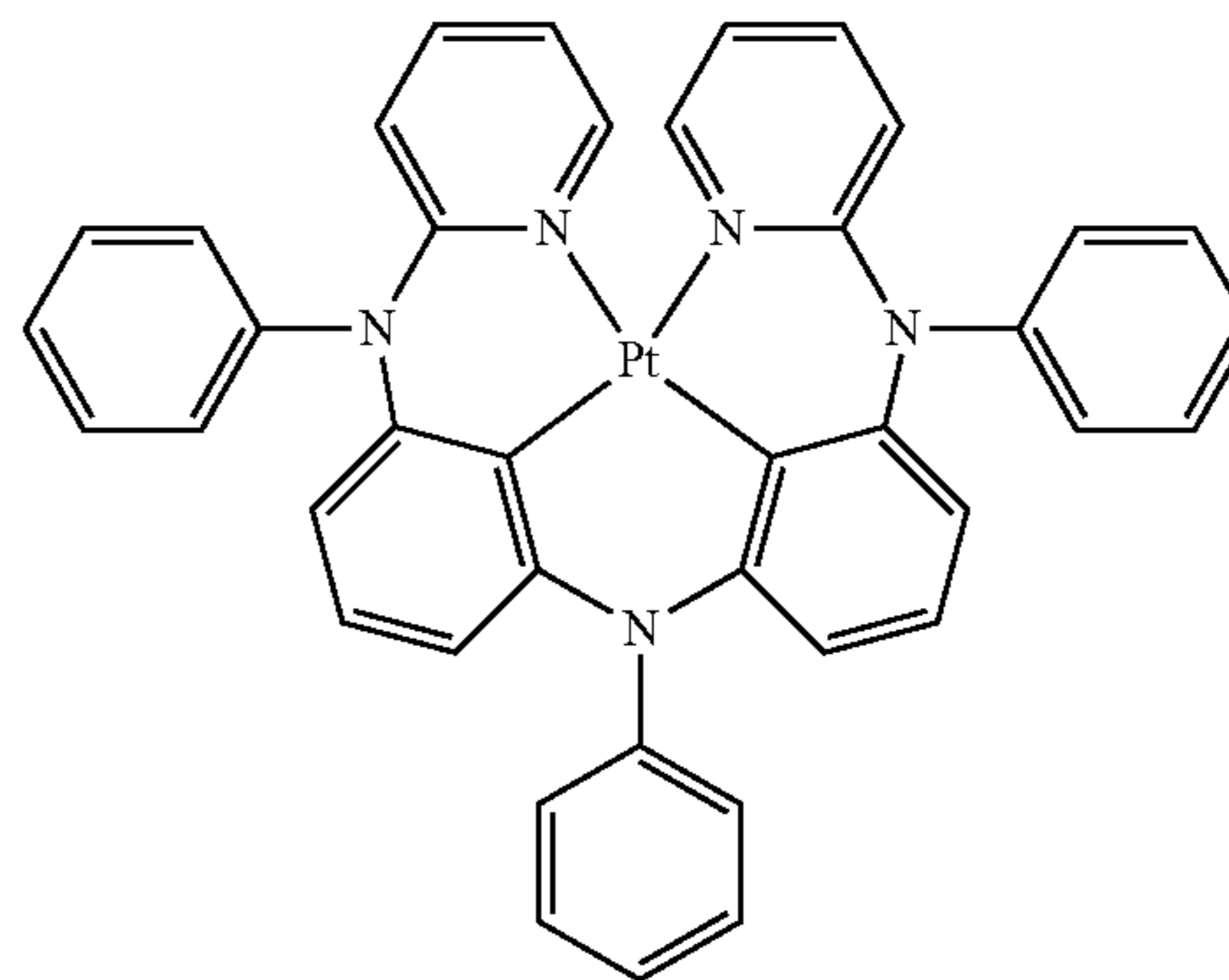
Compound 26
