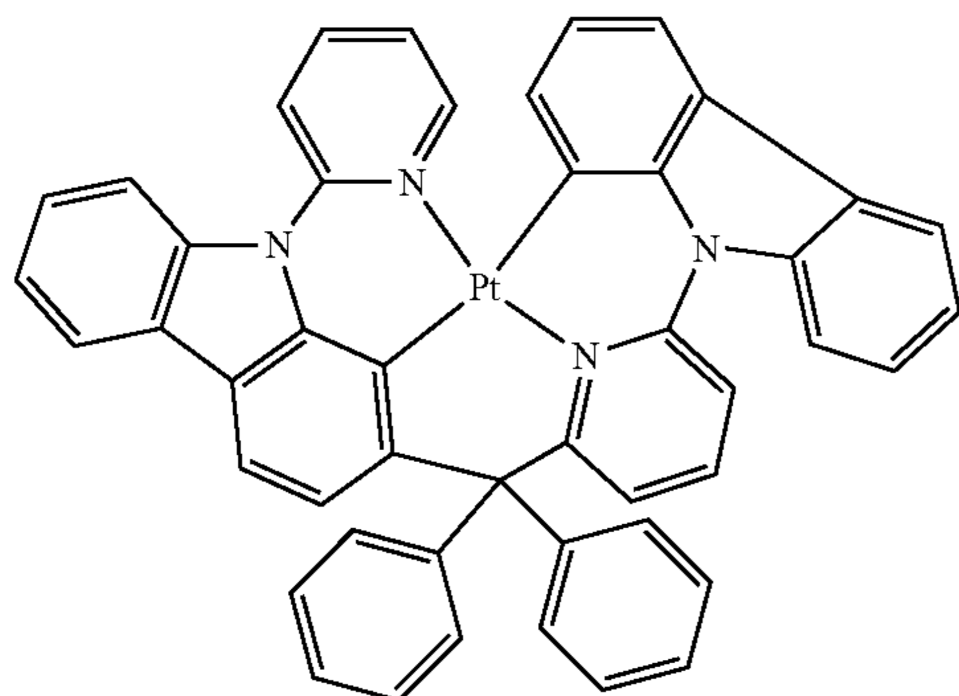
Compound 101
