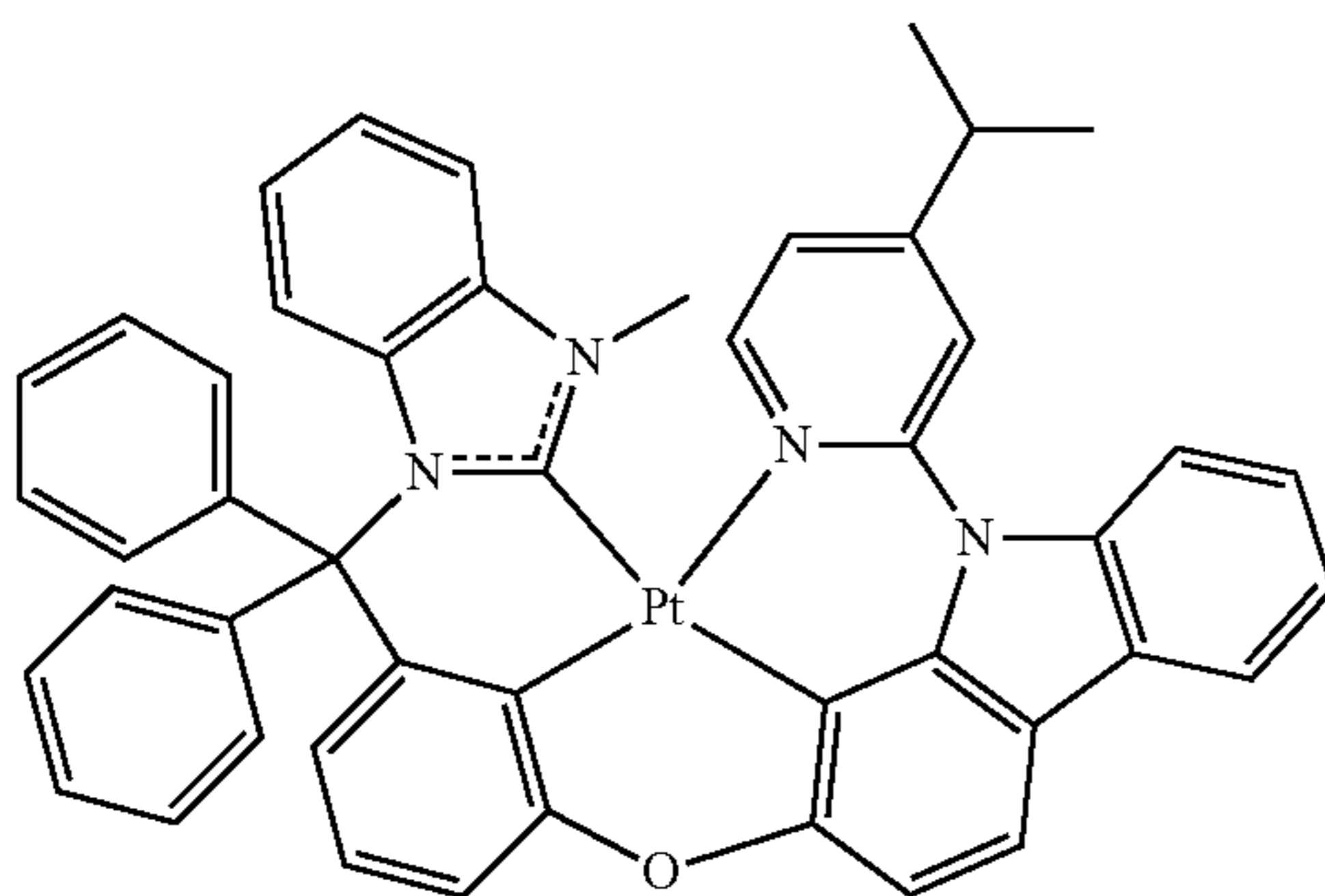
Compound 78
