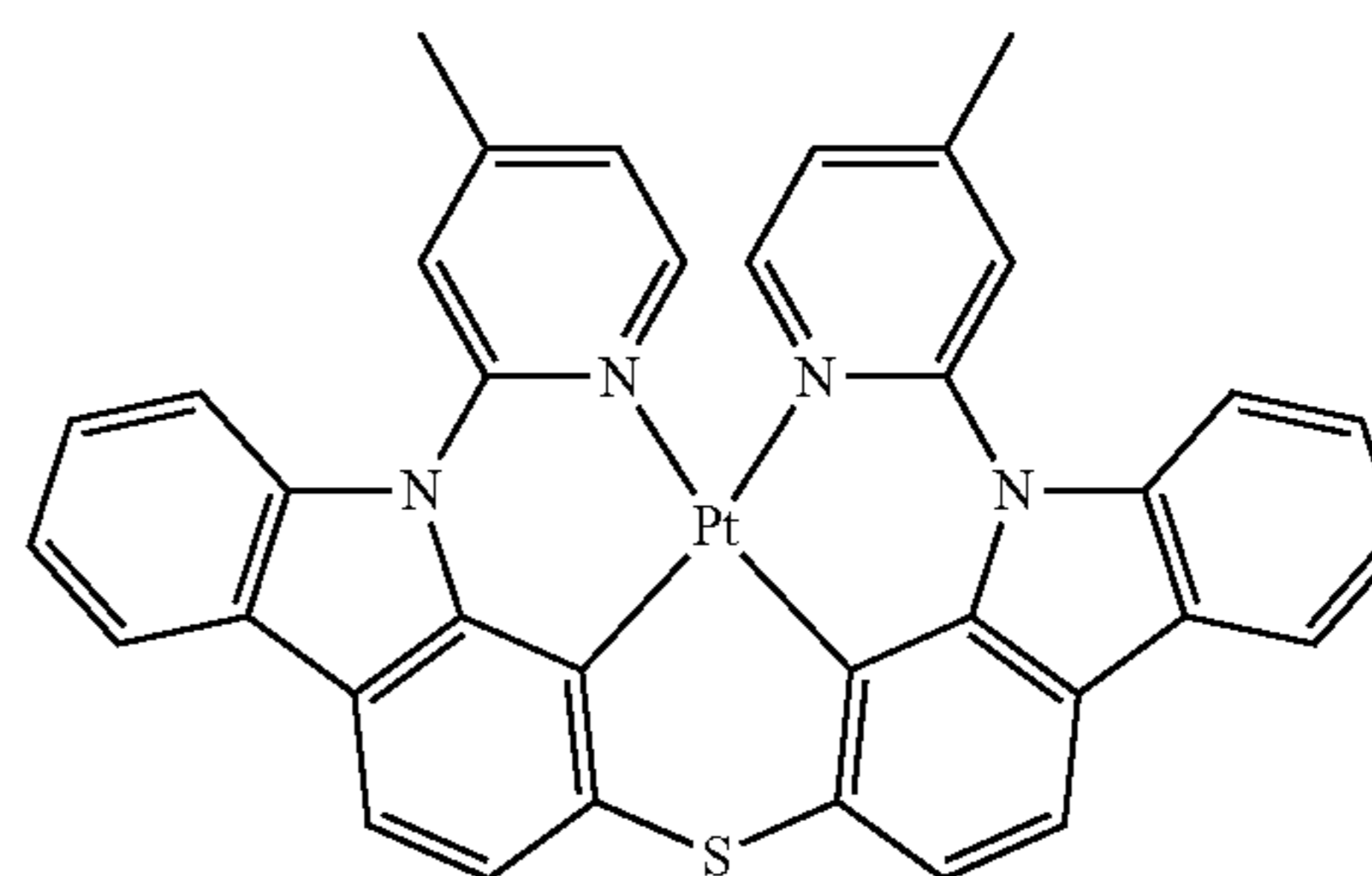
Compound 9
