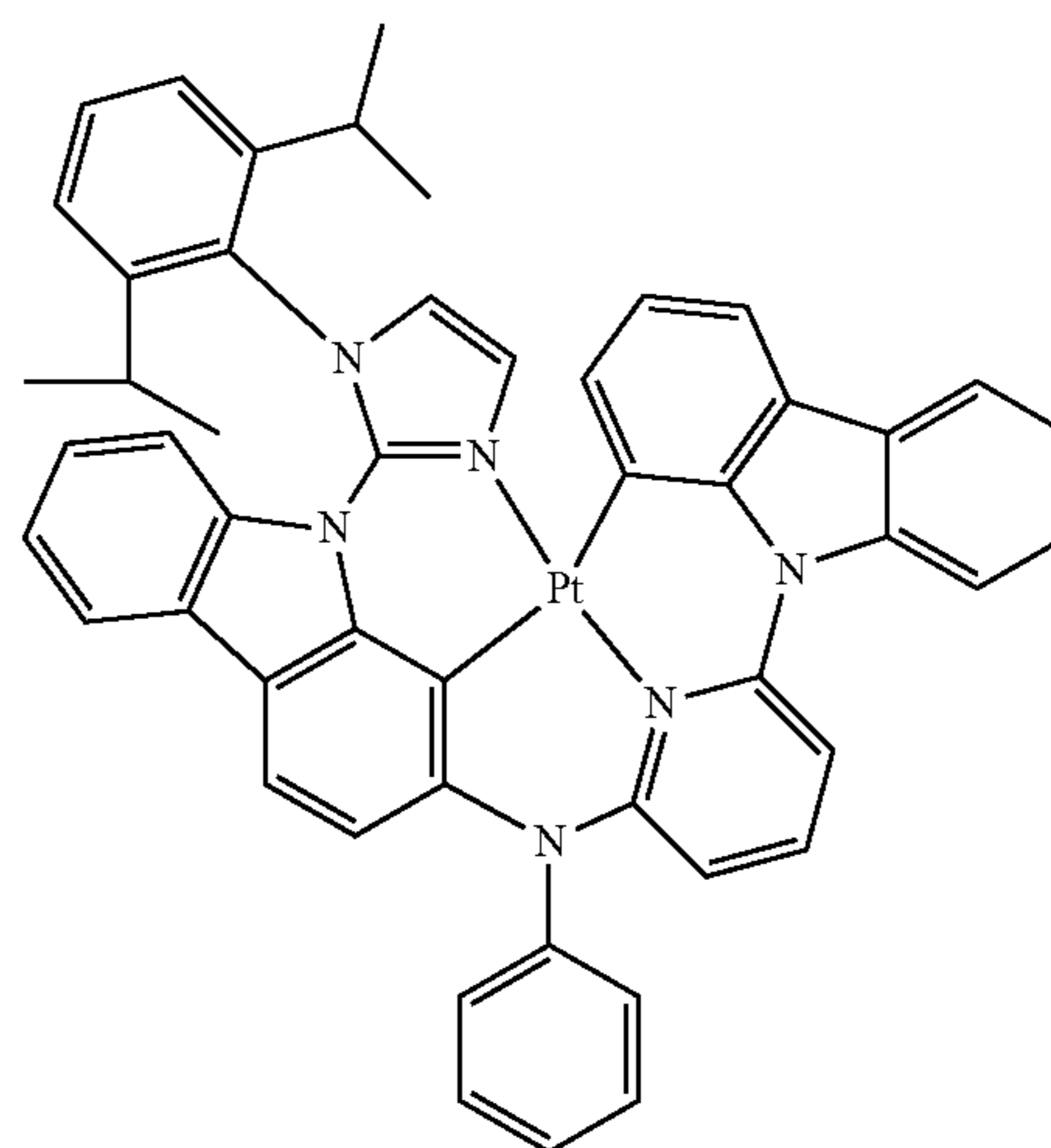
Compound 125
