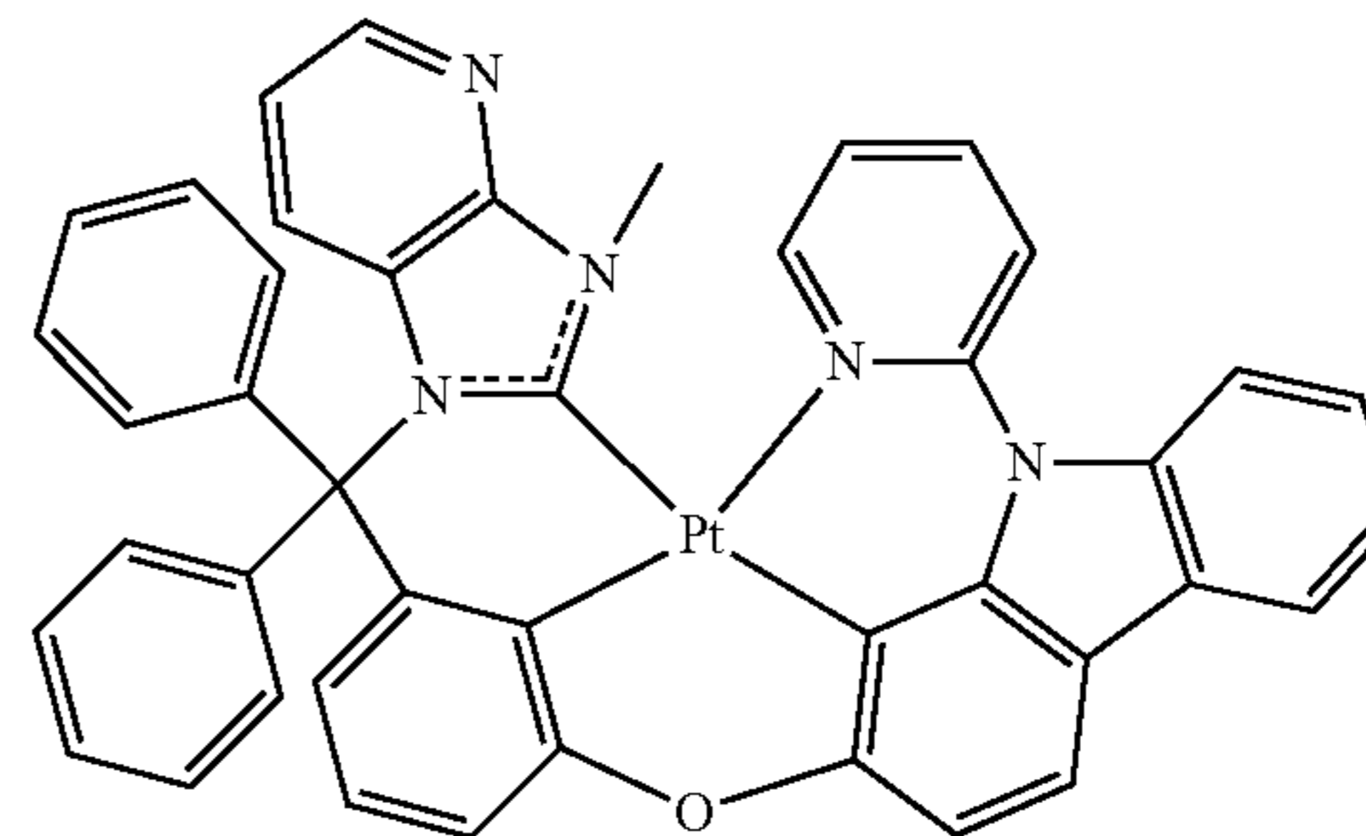
Compound 83
