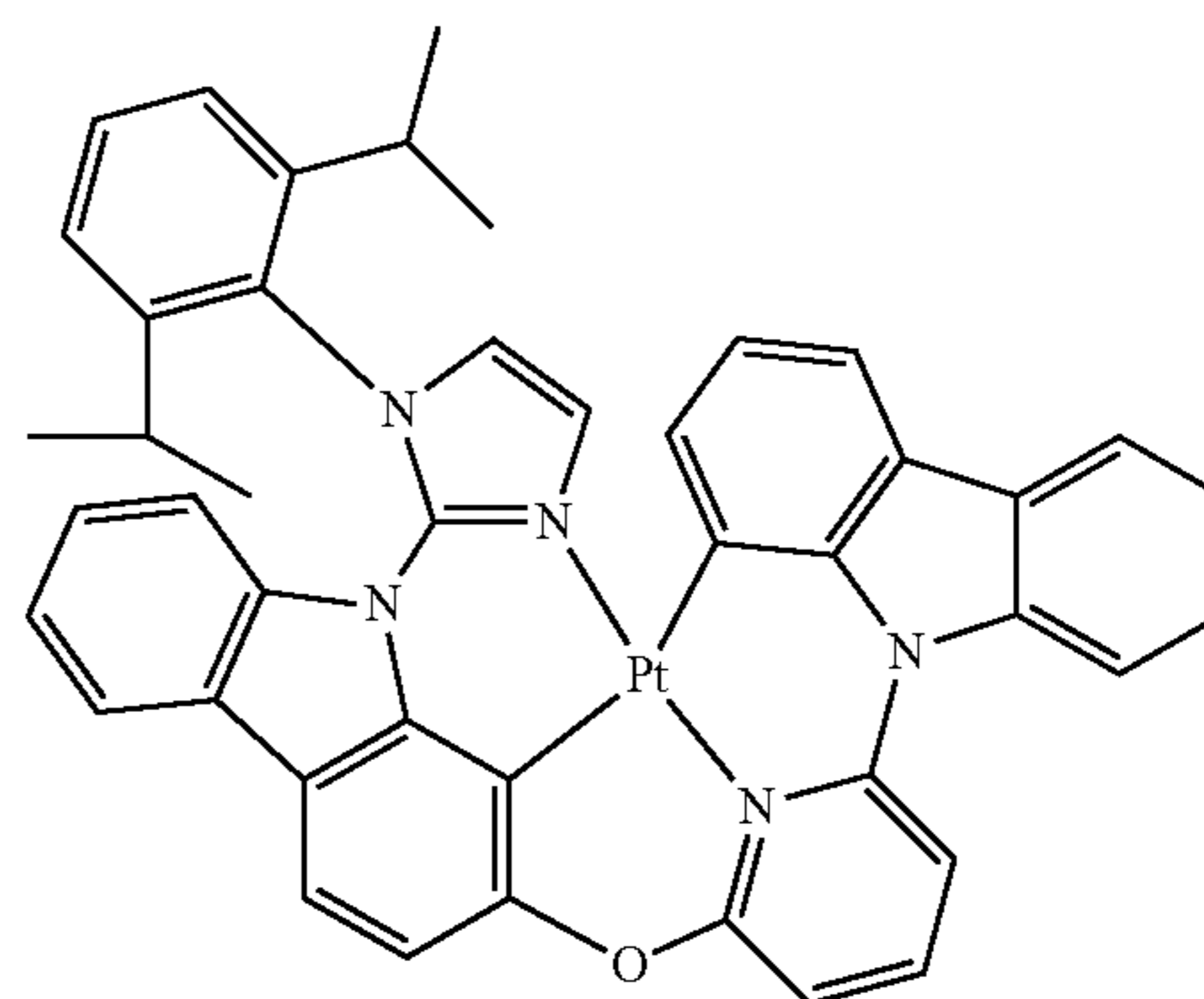
Compound 124
