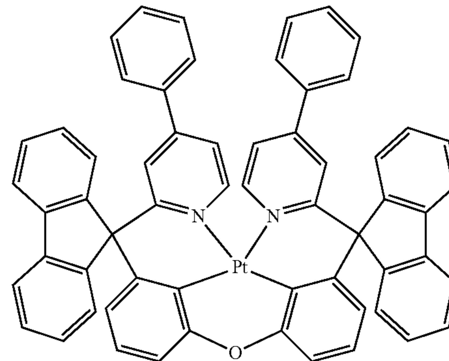
Compound 92
