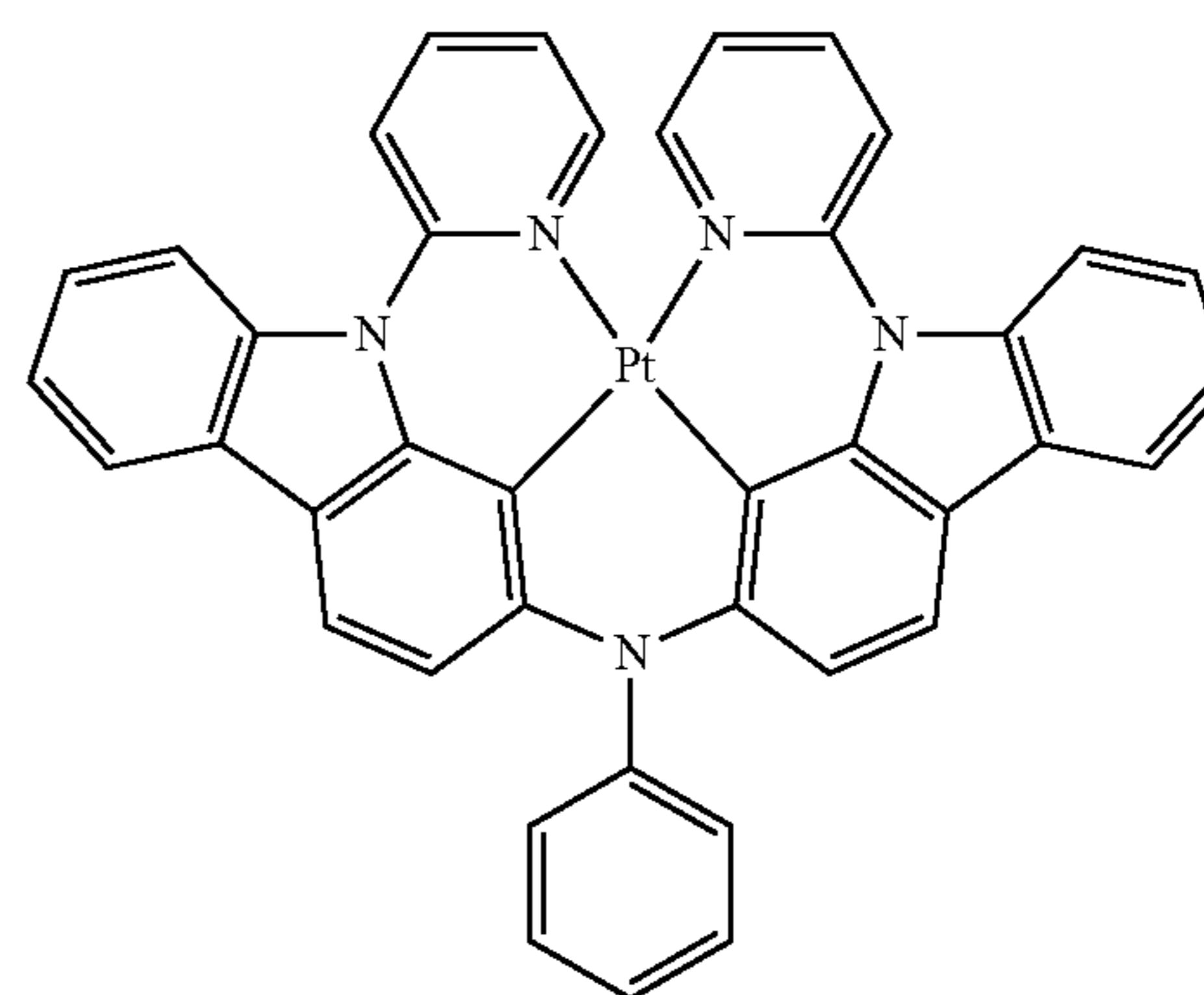
Compound 2
