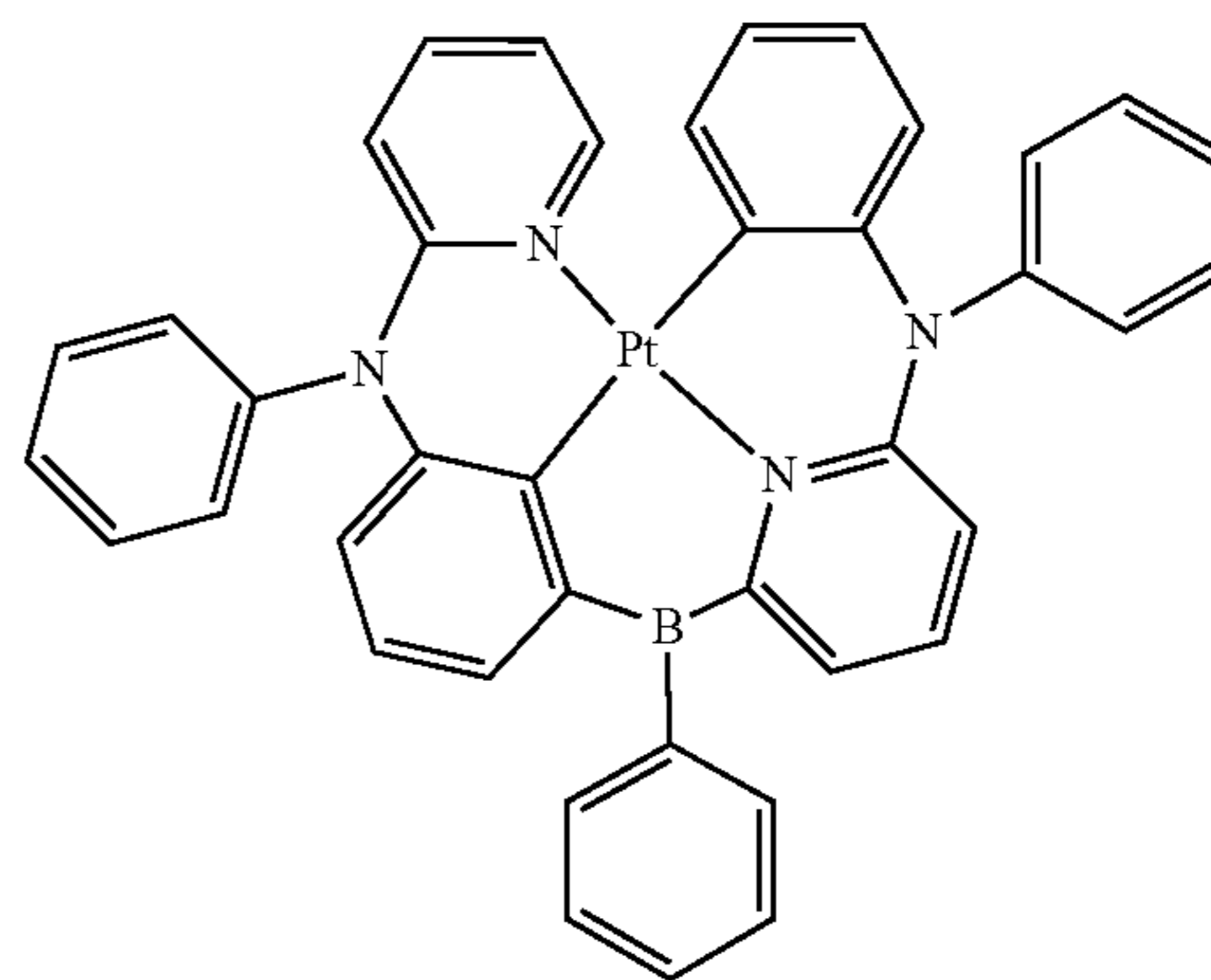
Compound 118
