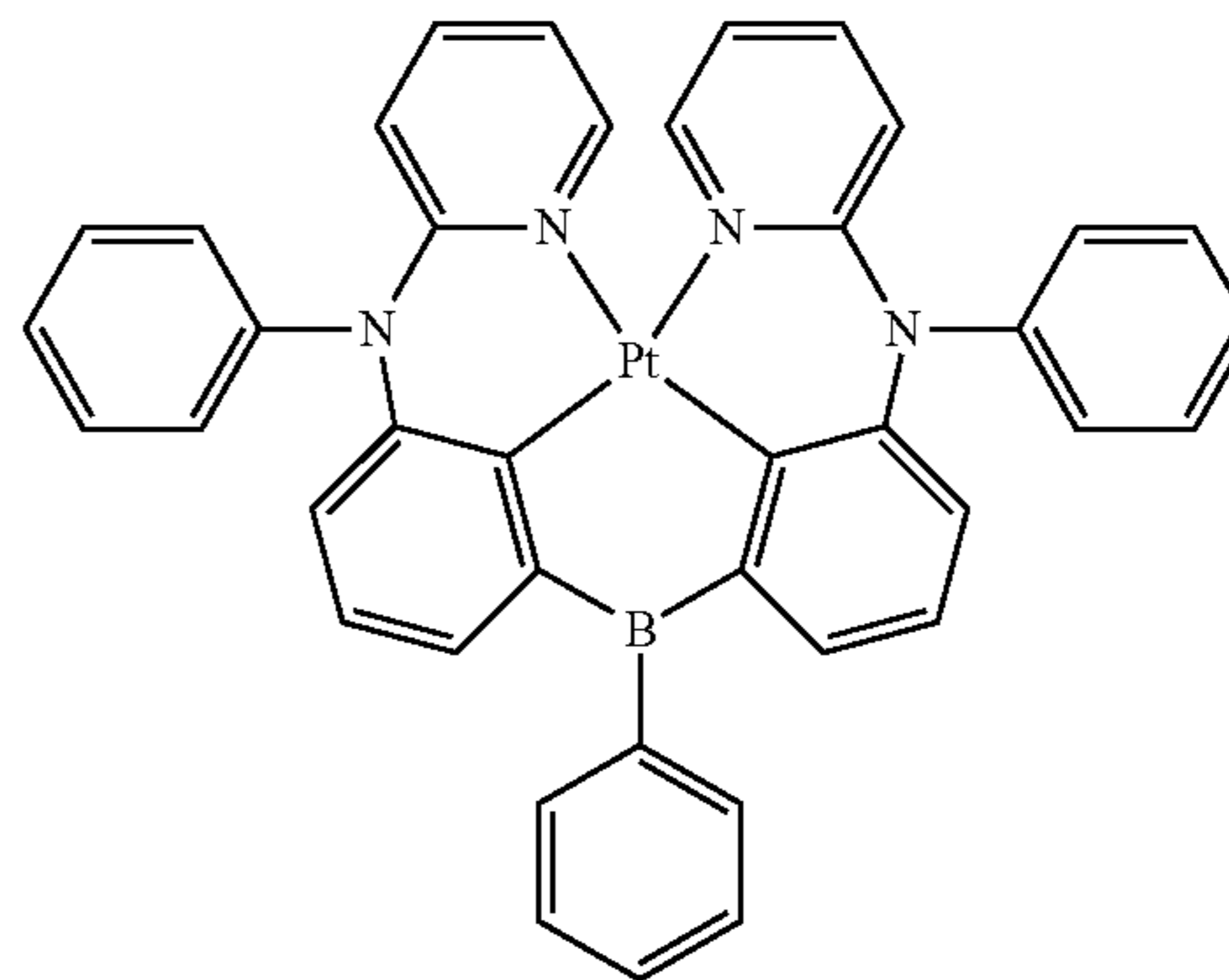
Compound 28
