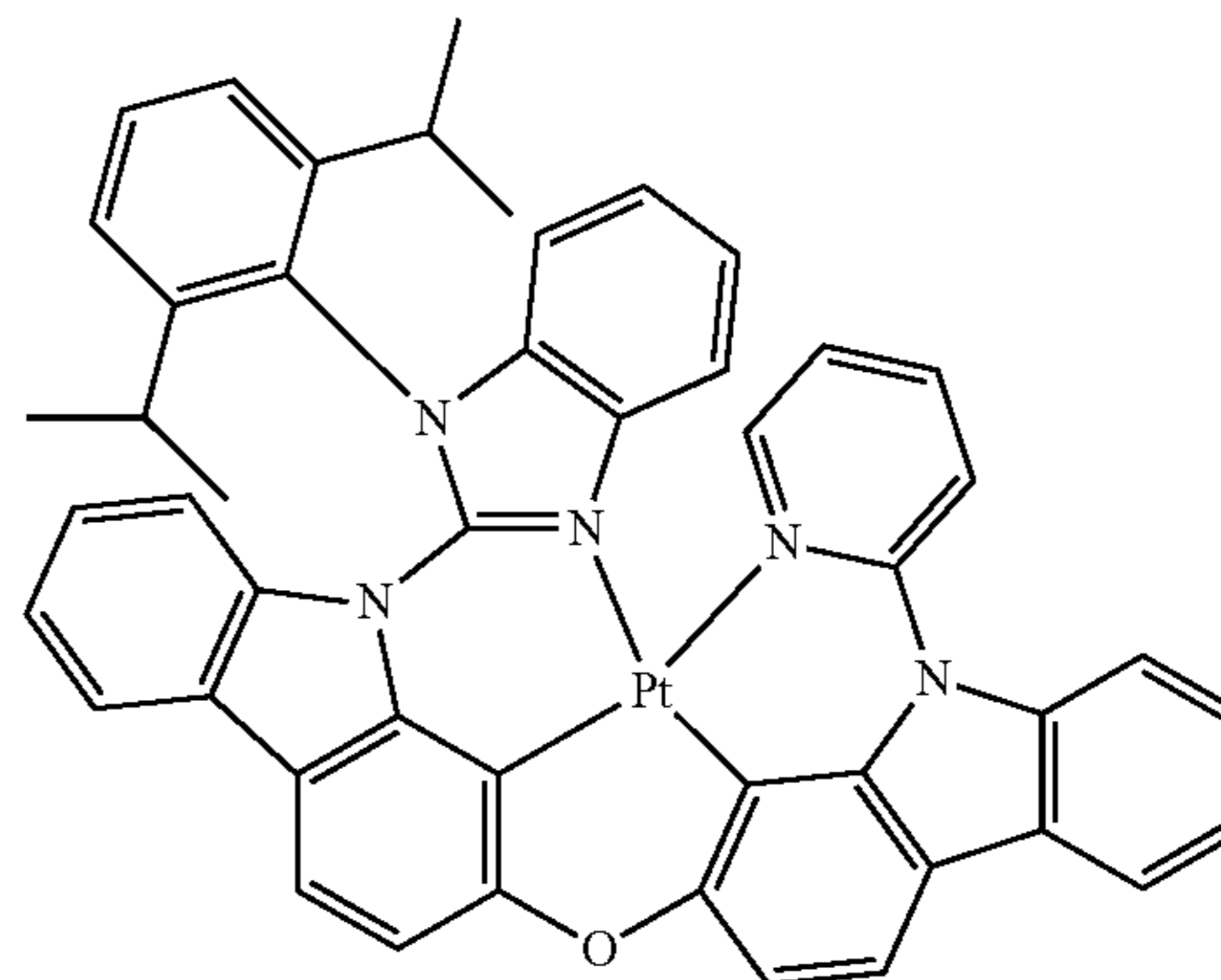
Compound 58
