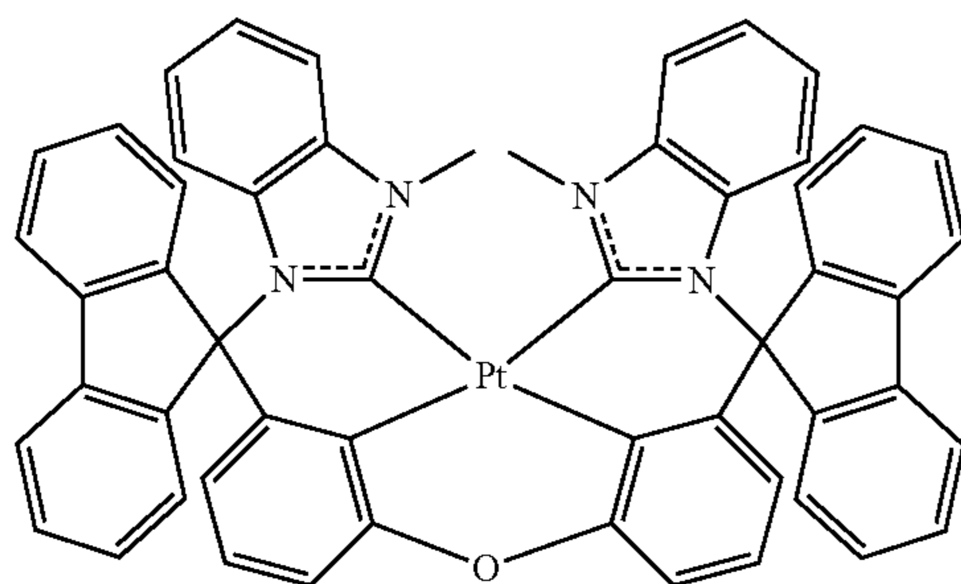
Compound 76
