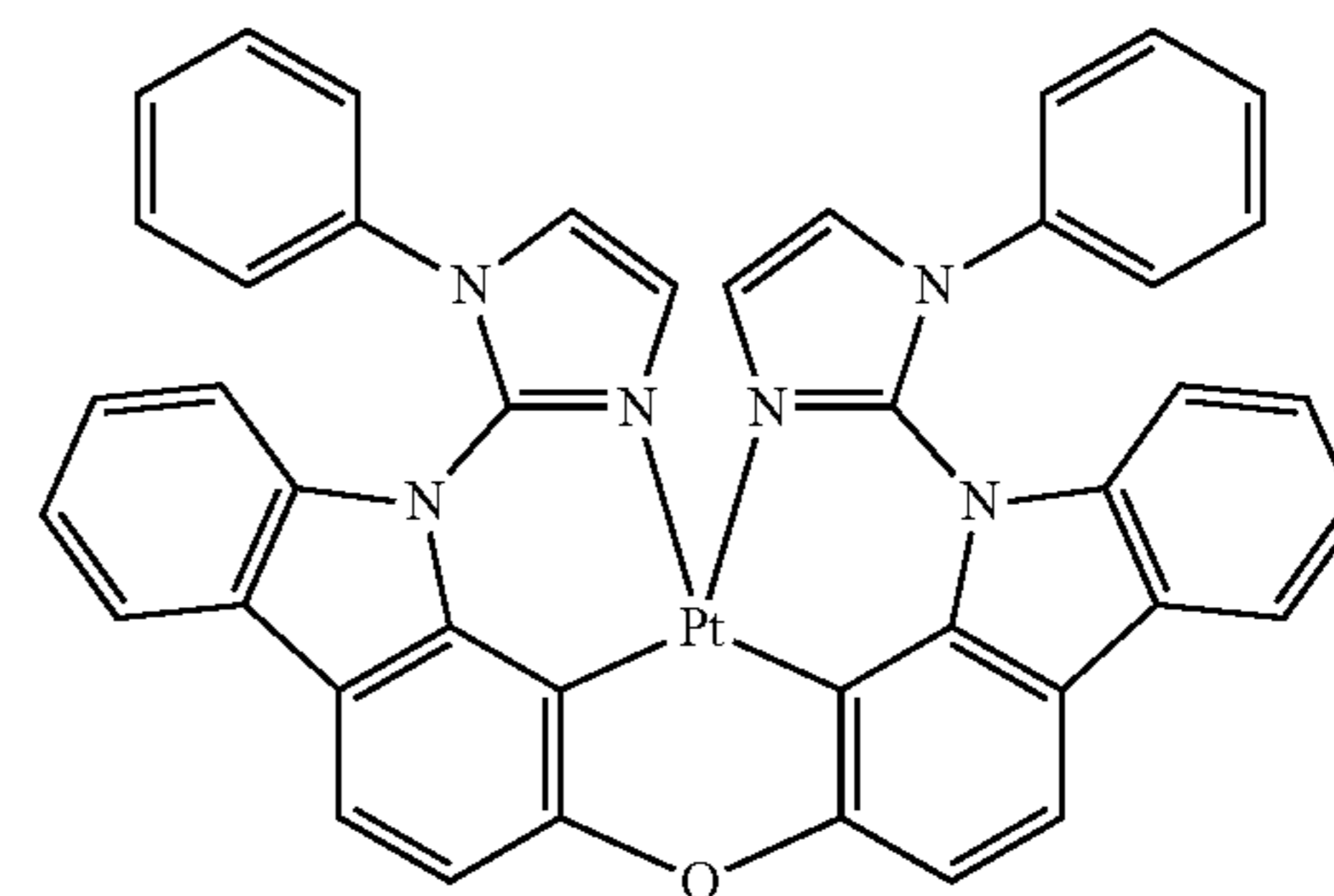
Compound 34
