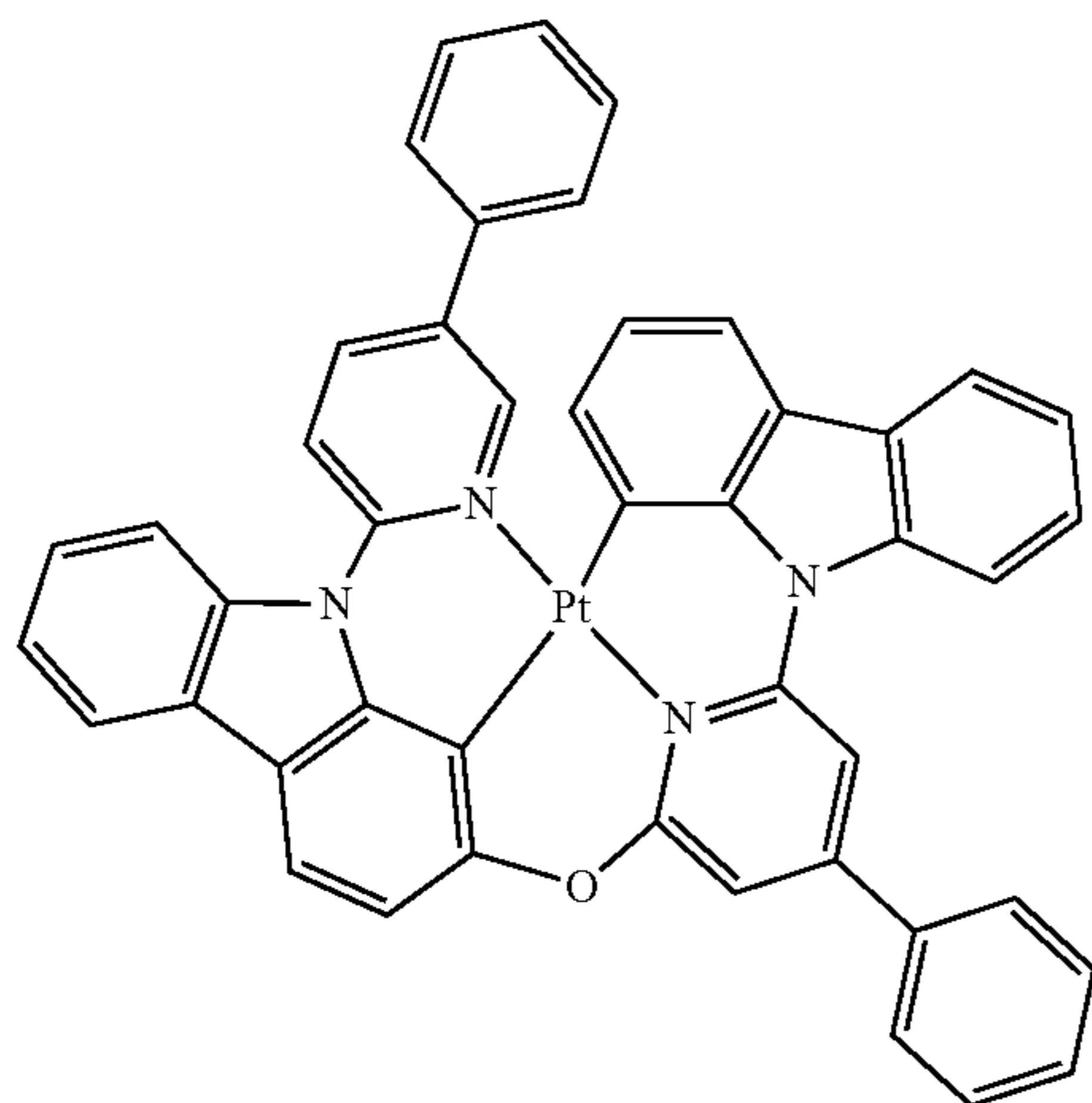
Compound 111
