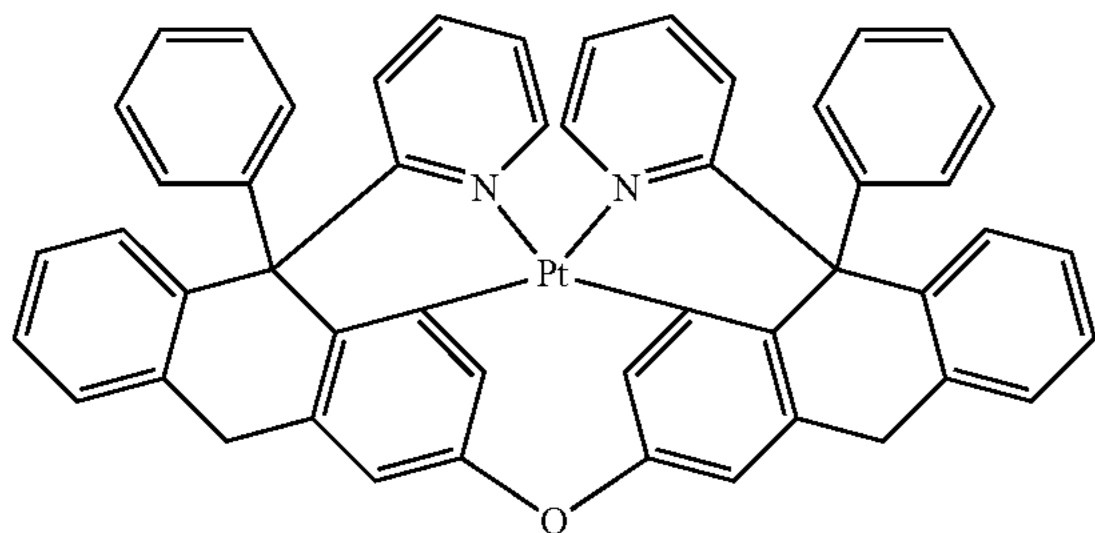
Compound 95
