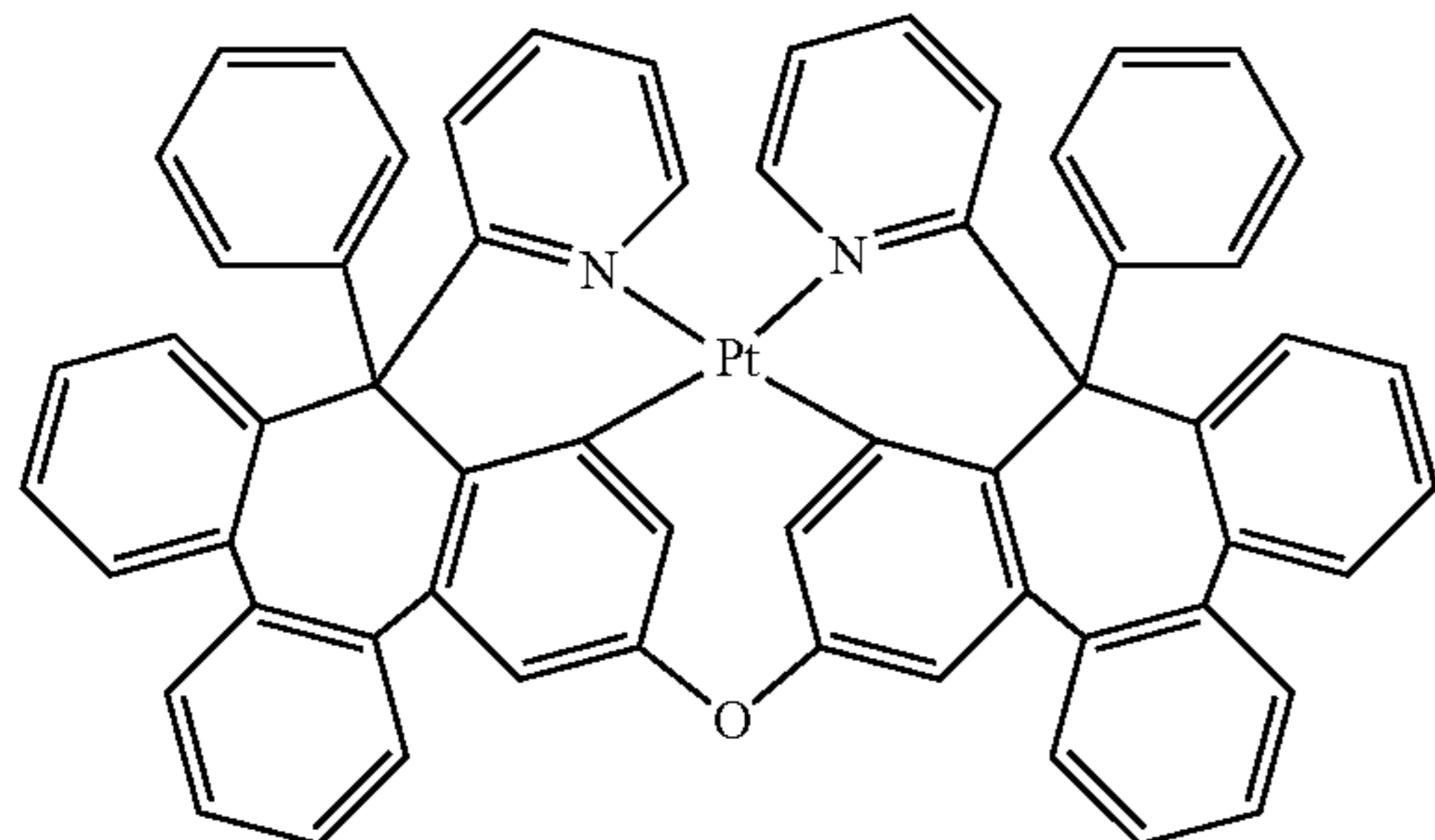
Compound 97
