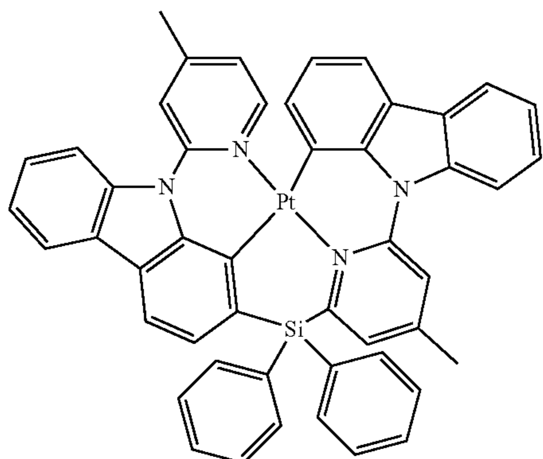
Compound 110
