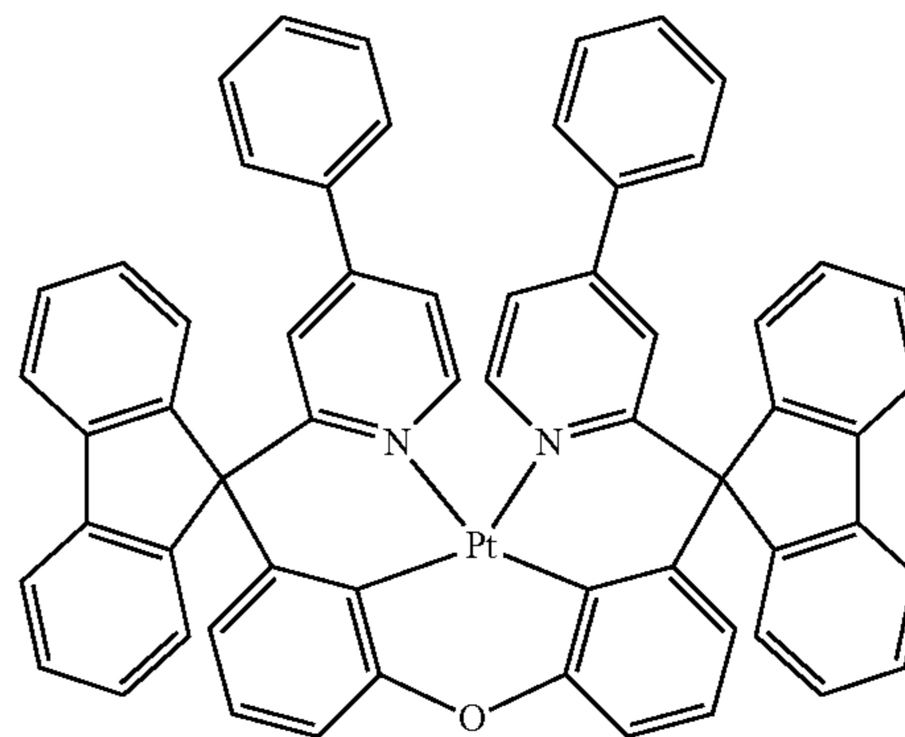
Compound 92
