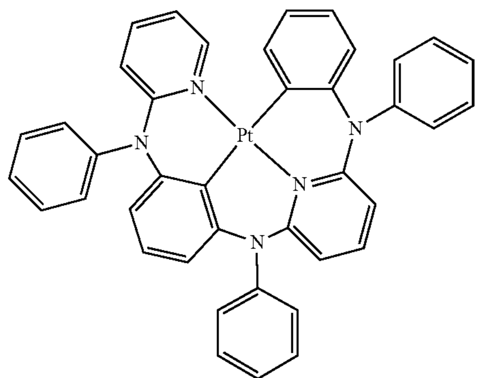
Compound 117
