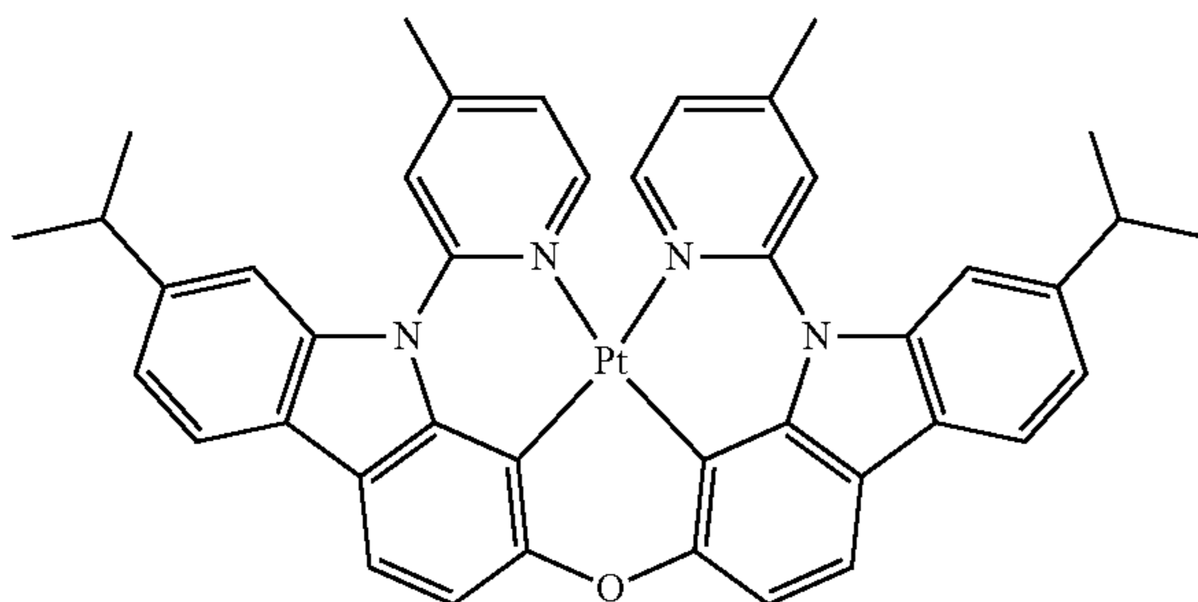
Compound 21
