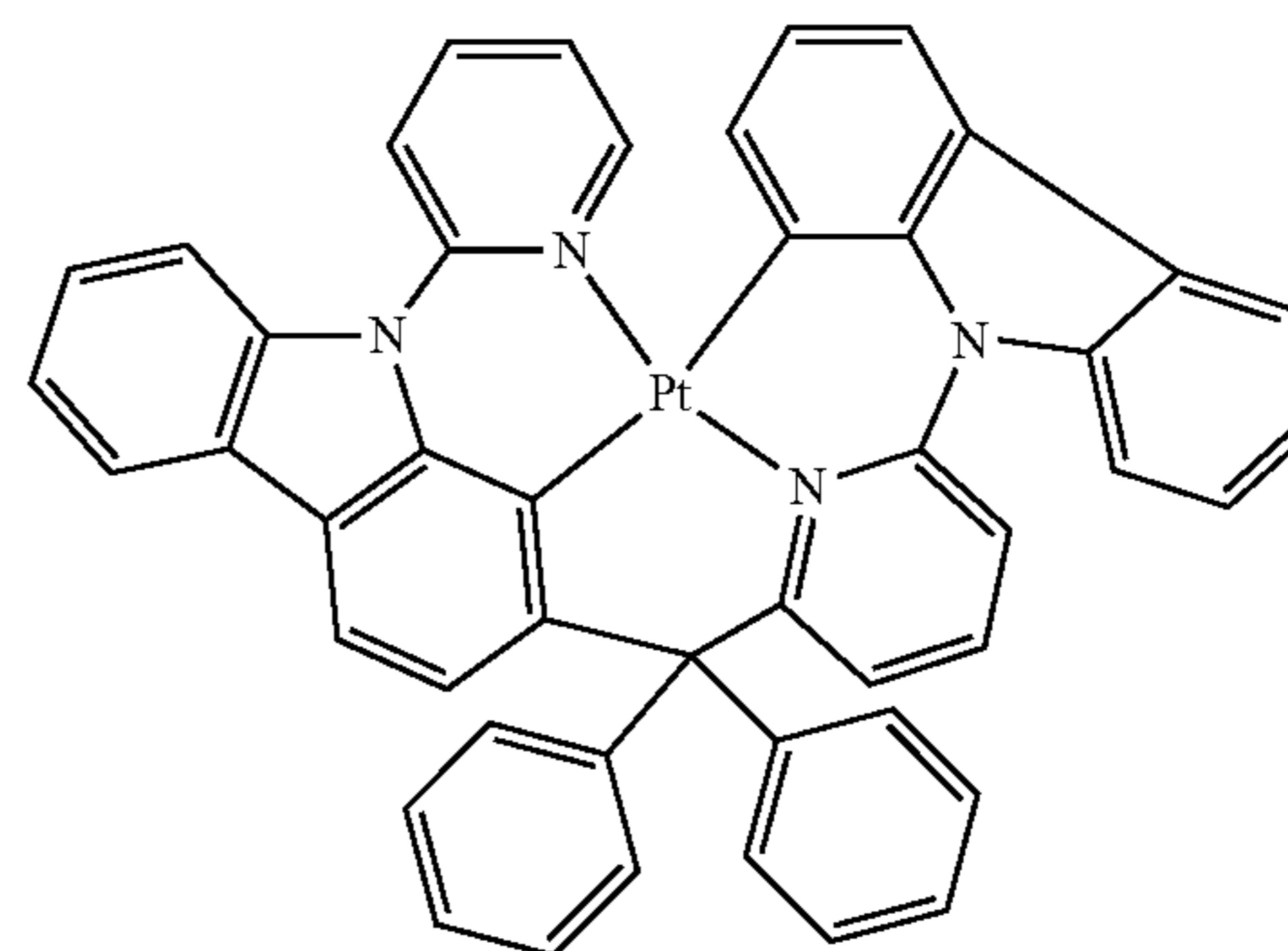
Compound 101
