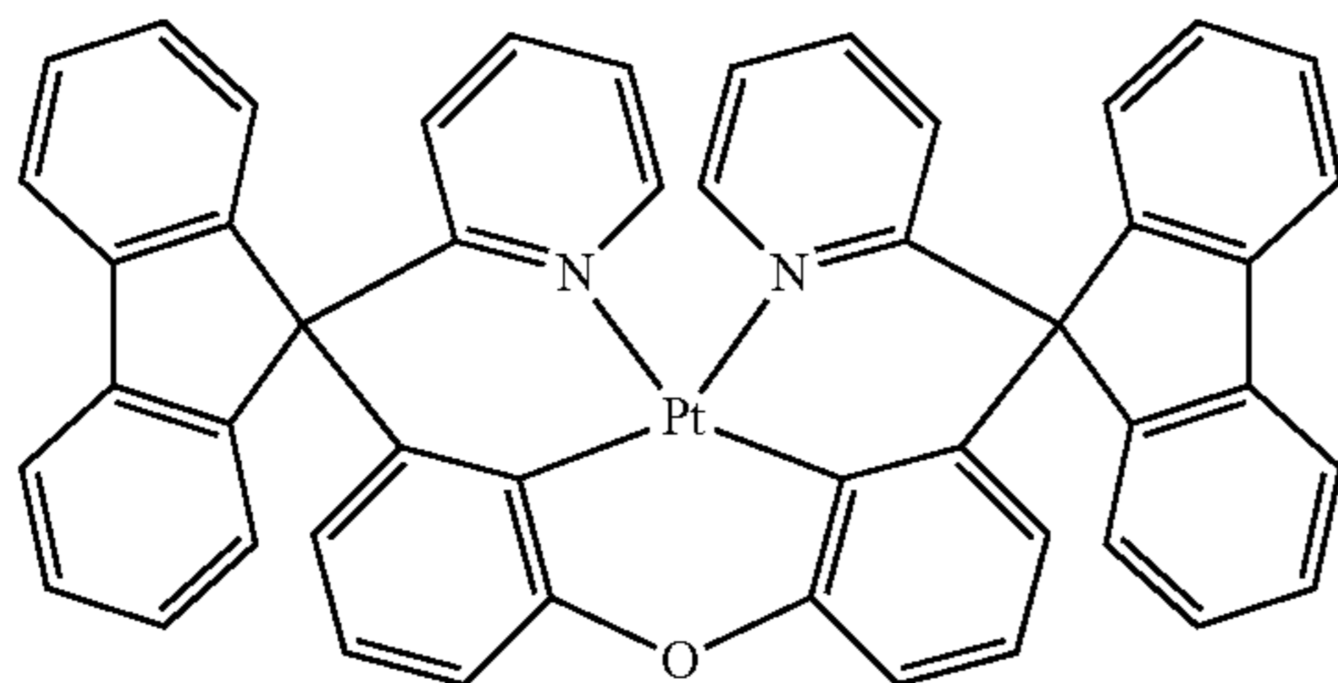
Compound 88
