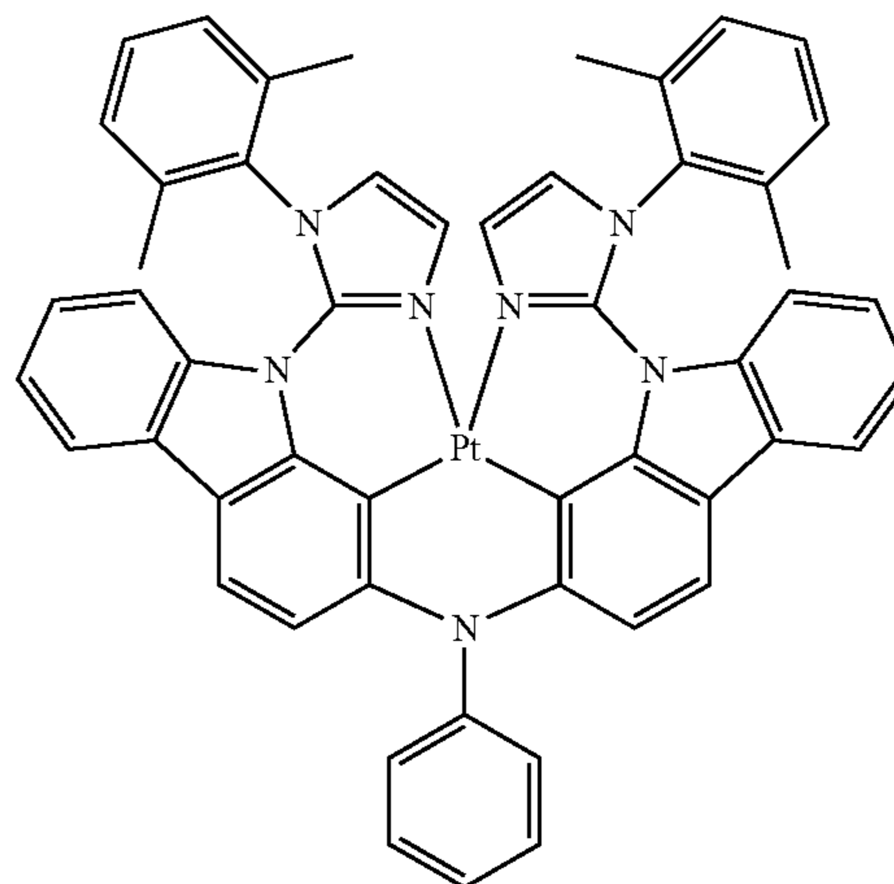
Compound 38
