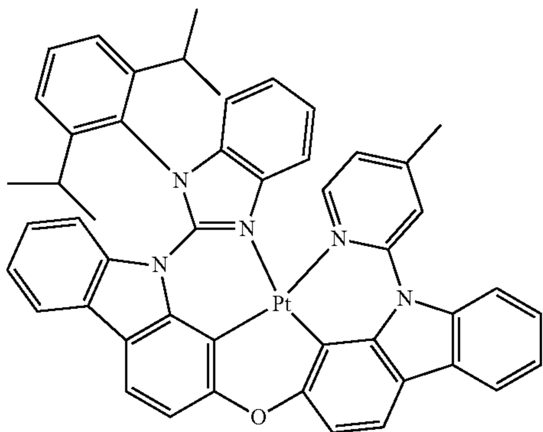
Compound 59
