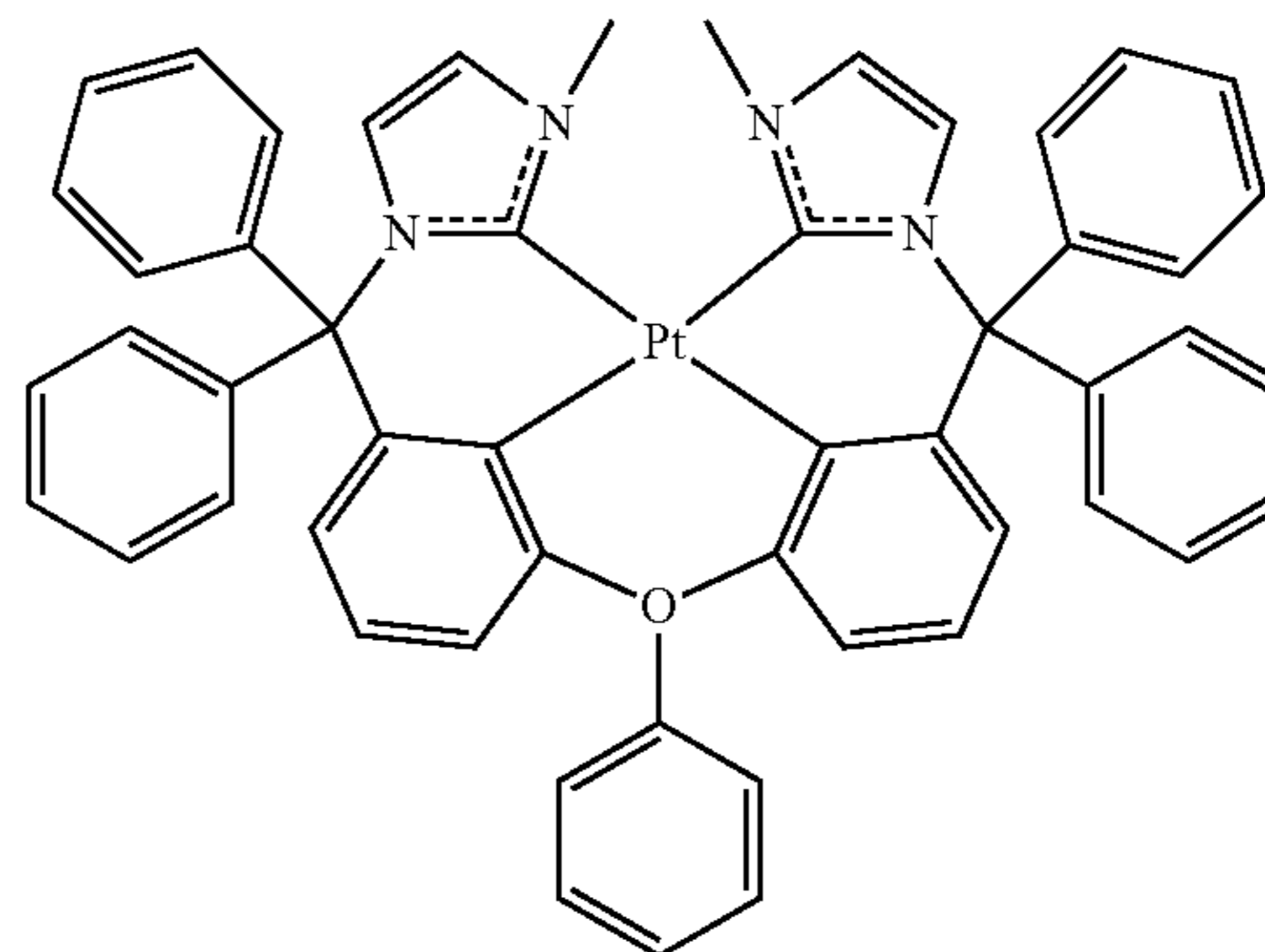
Compound 68
