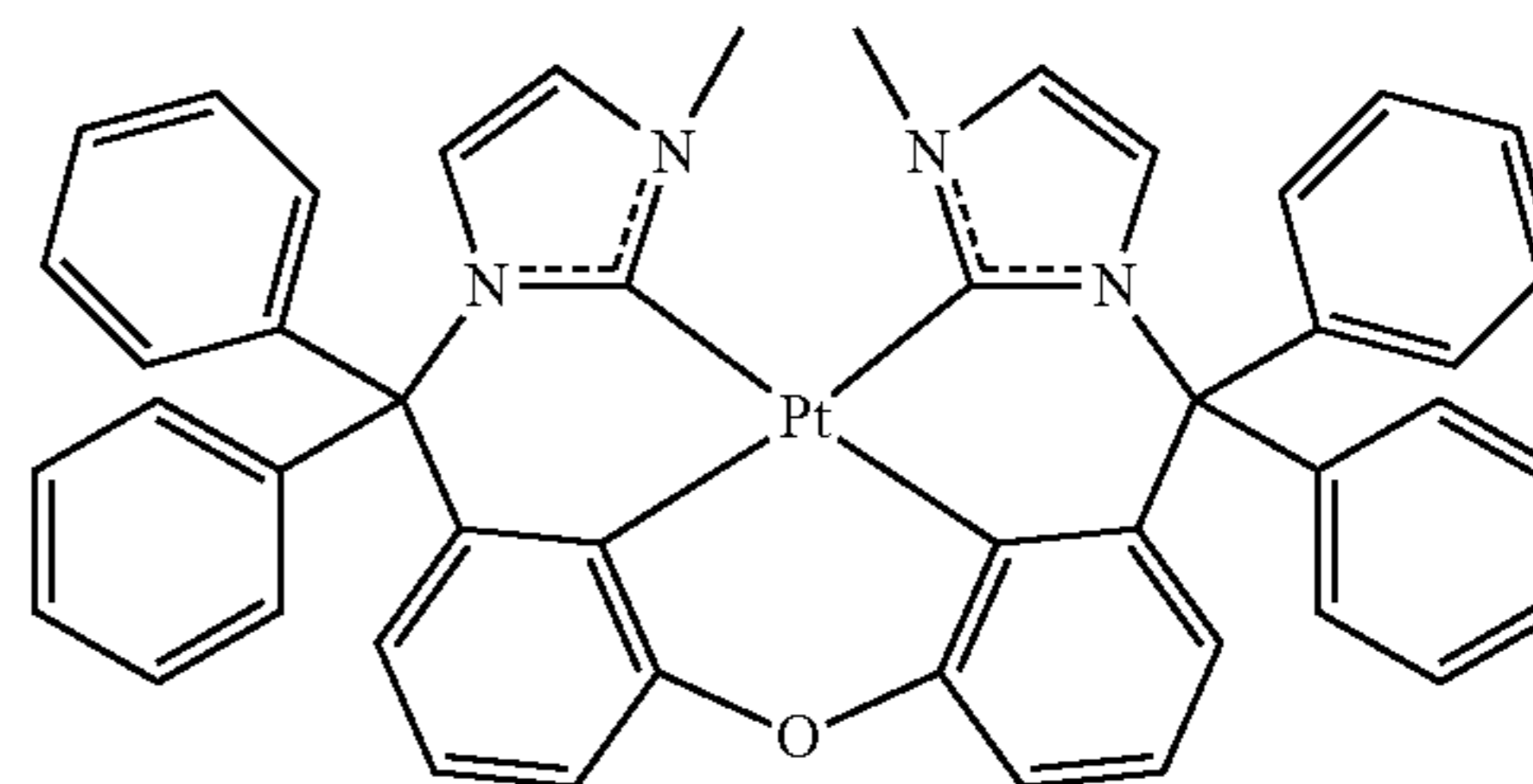
Compound 66
