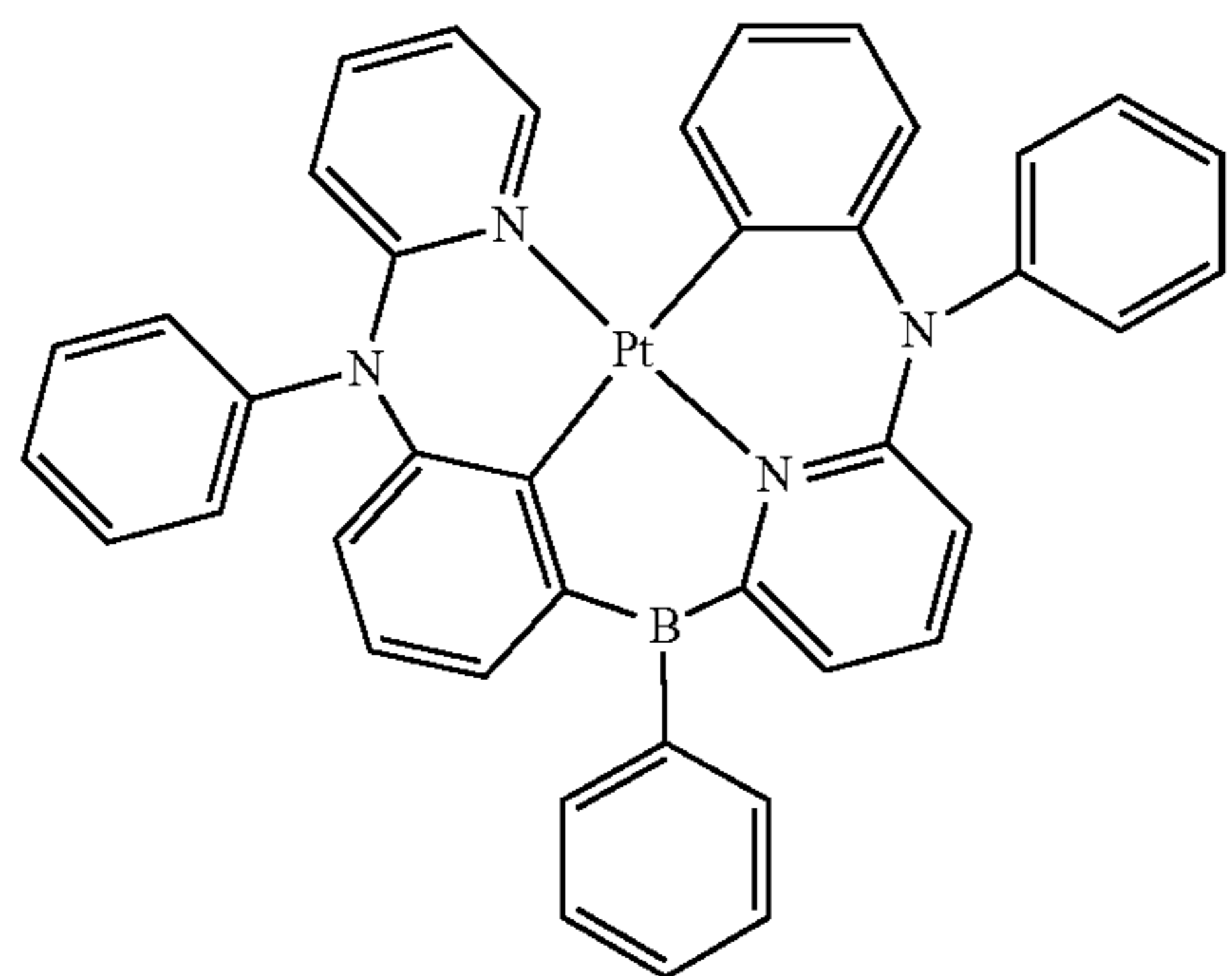
Compound 118
