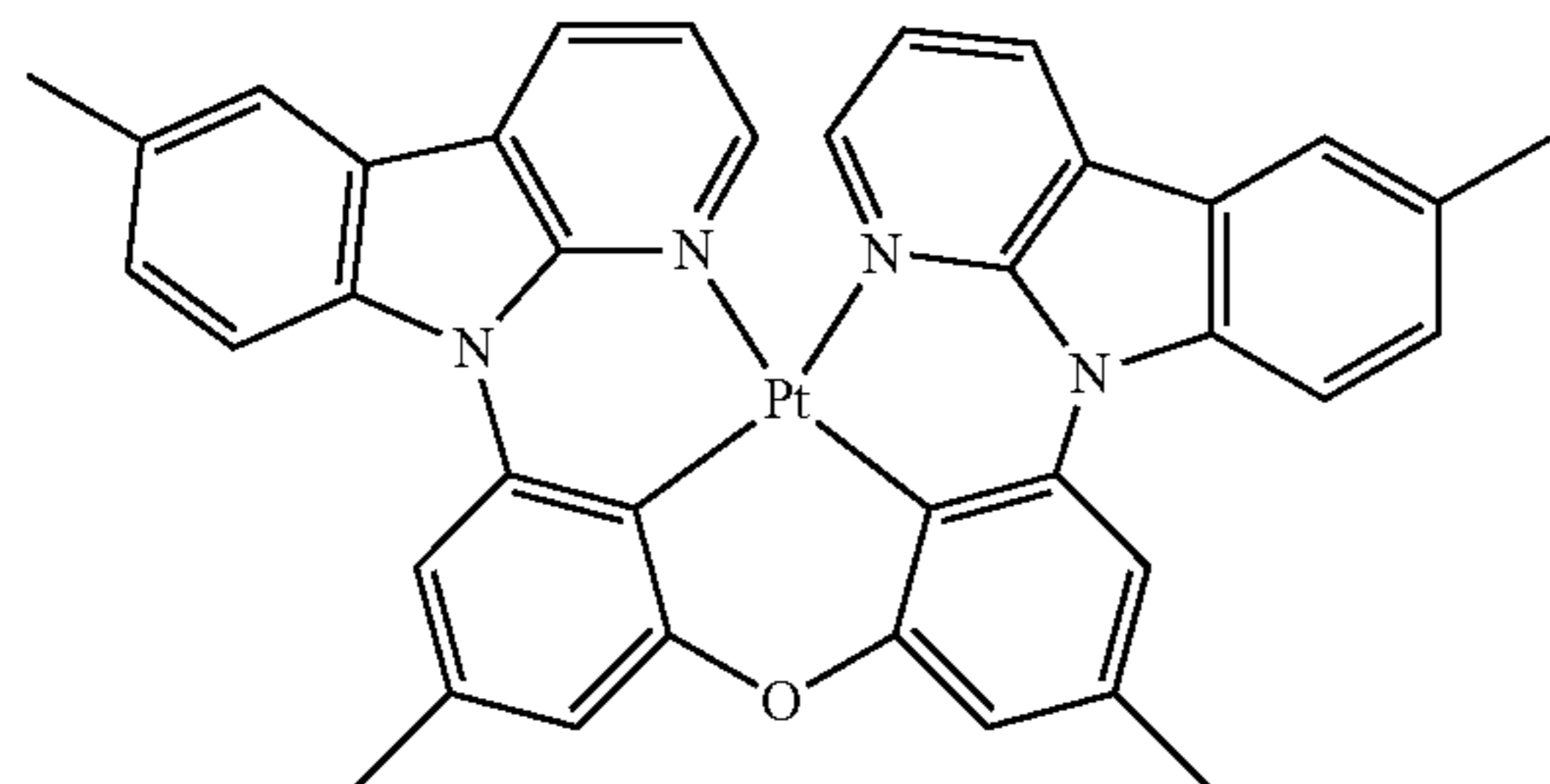
Compound 24
