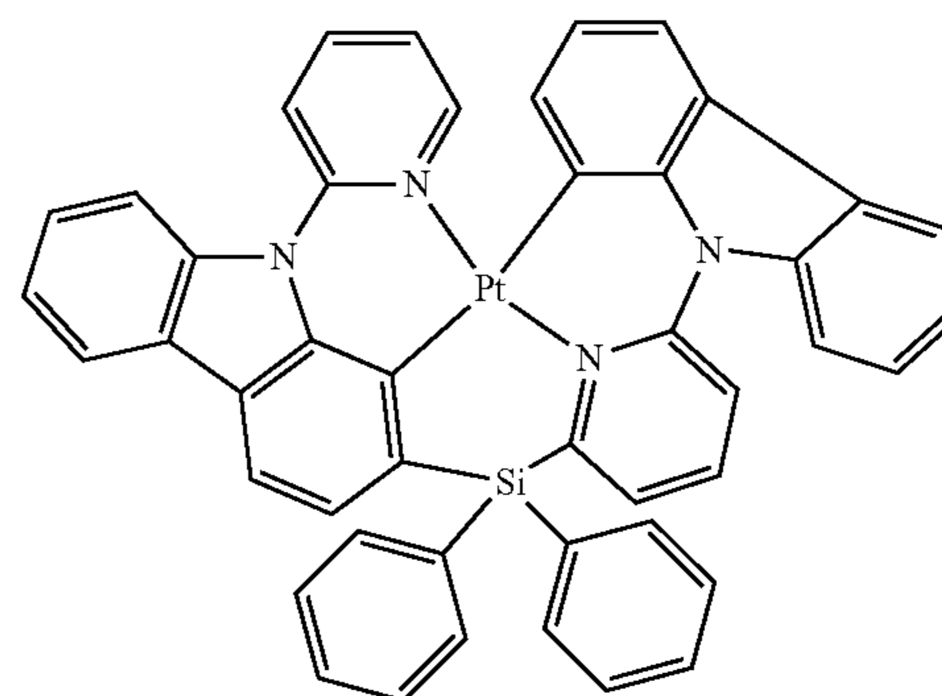
Compound 102
