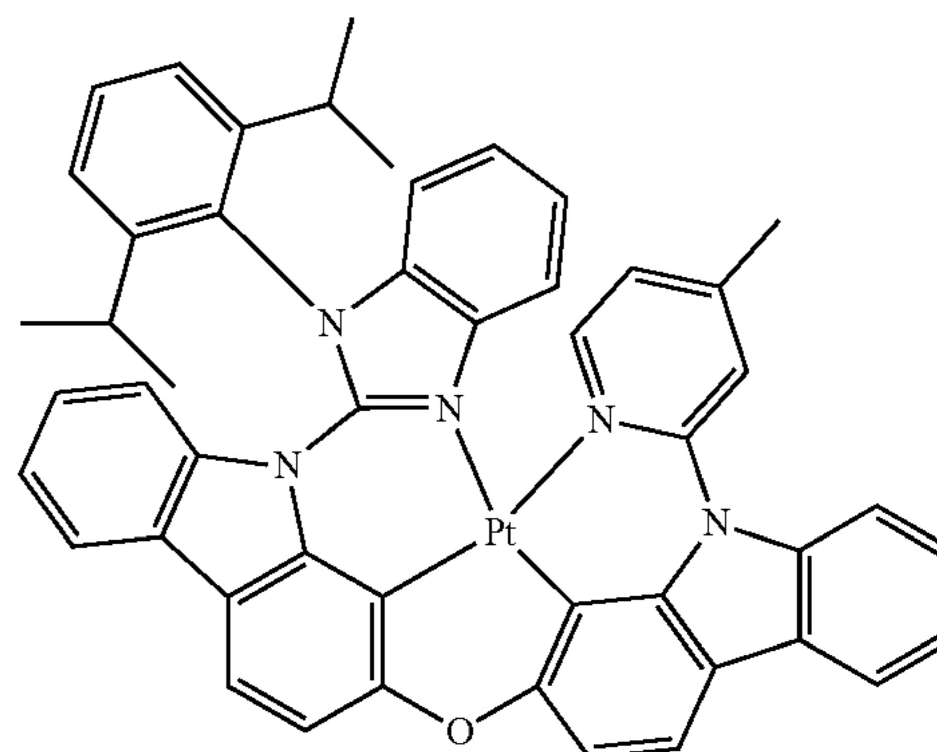
Compound 59
