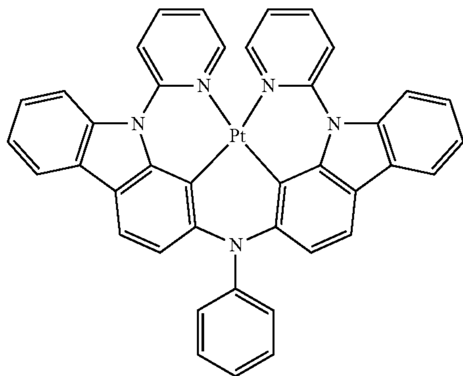
Compound 2
