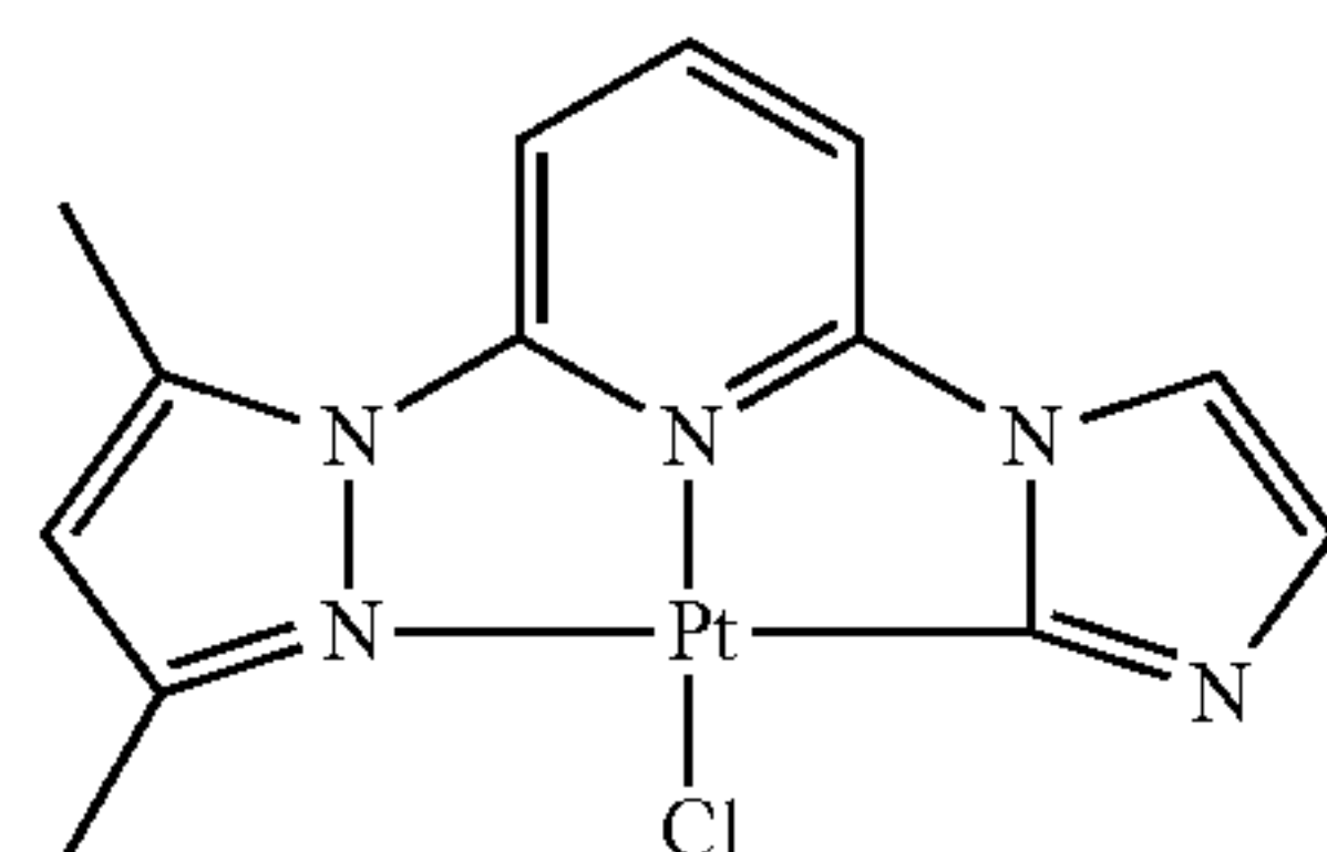
DMPz-Py-Iz-PtCl
