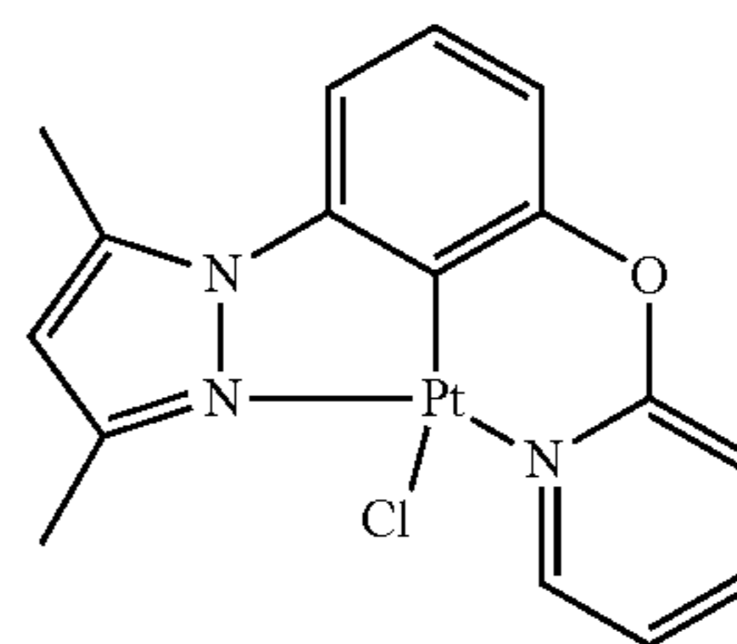
DMPz-Ph-O-Py-PtCl
