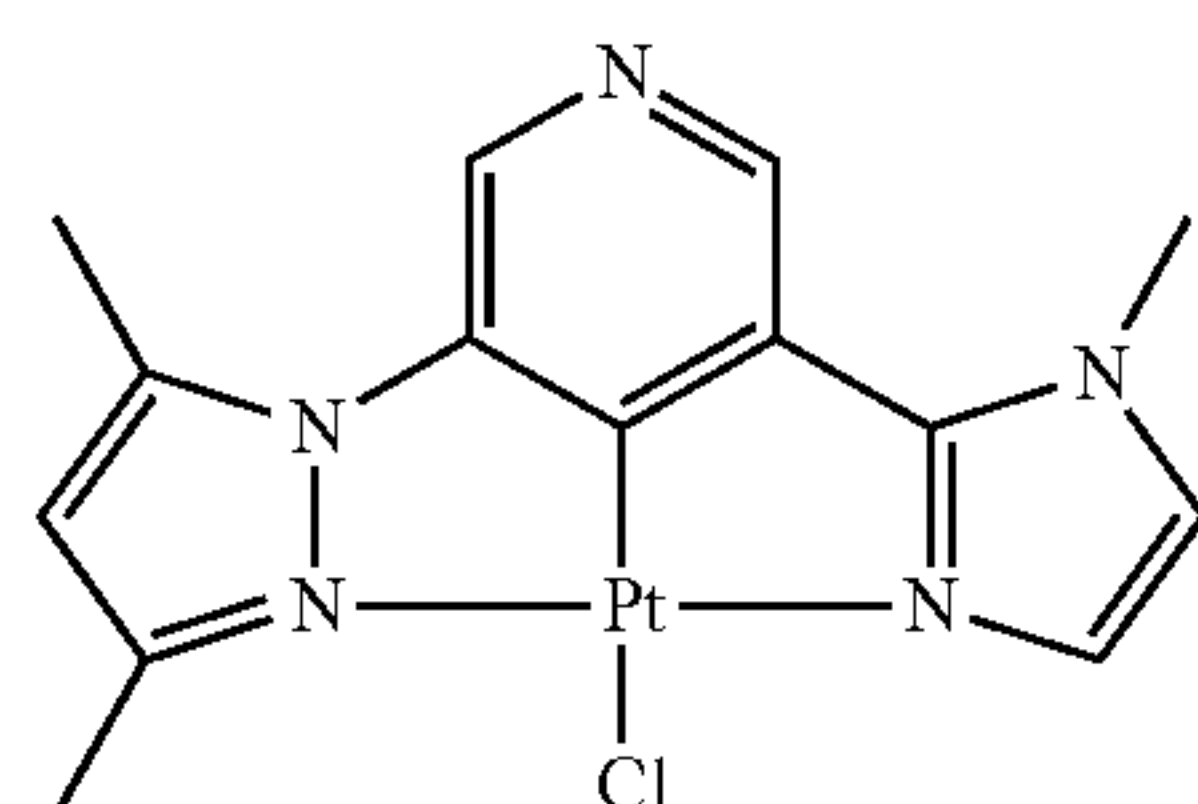
DMPz—Py—MIz—PtCl
