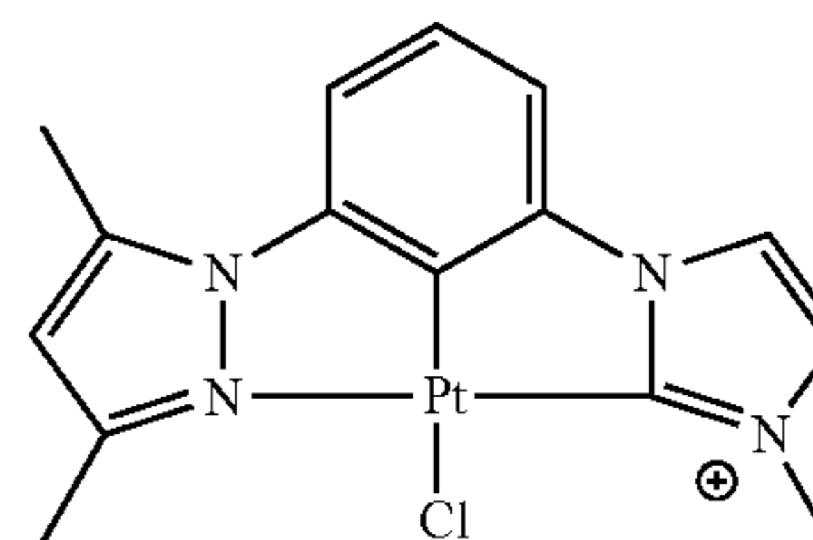
DMPz—Ph—MIzCb—PtCl
