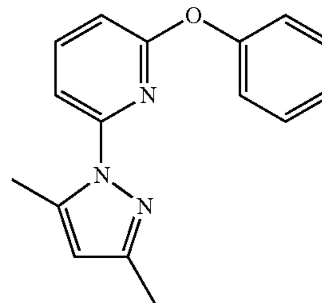
DMPz-Py-O-Ph
