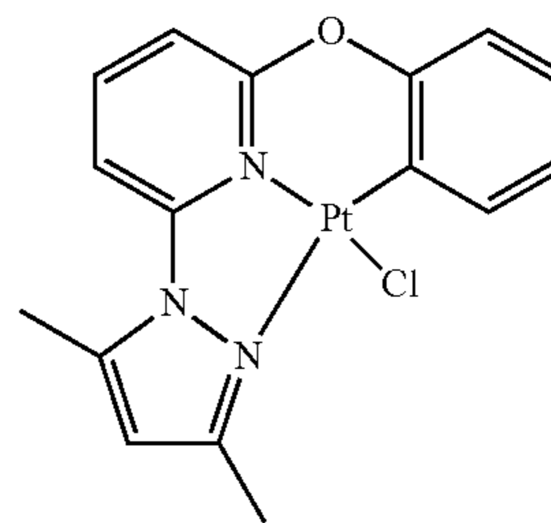
DMPz-Py-O-Ph-PtCl
