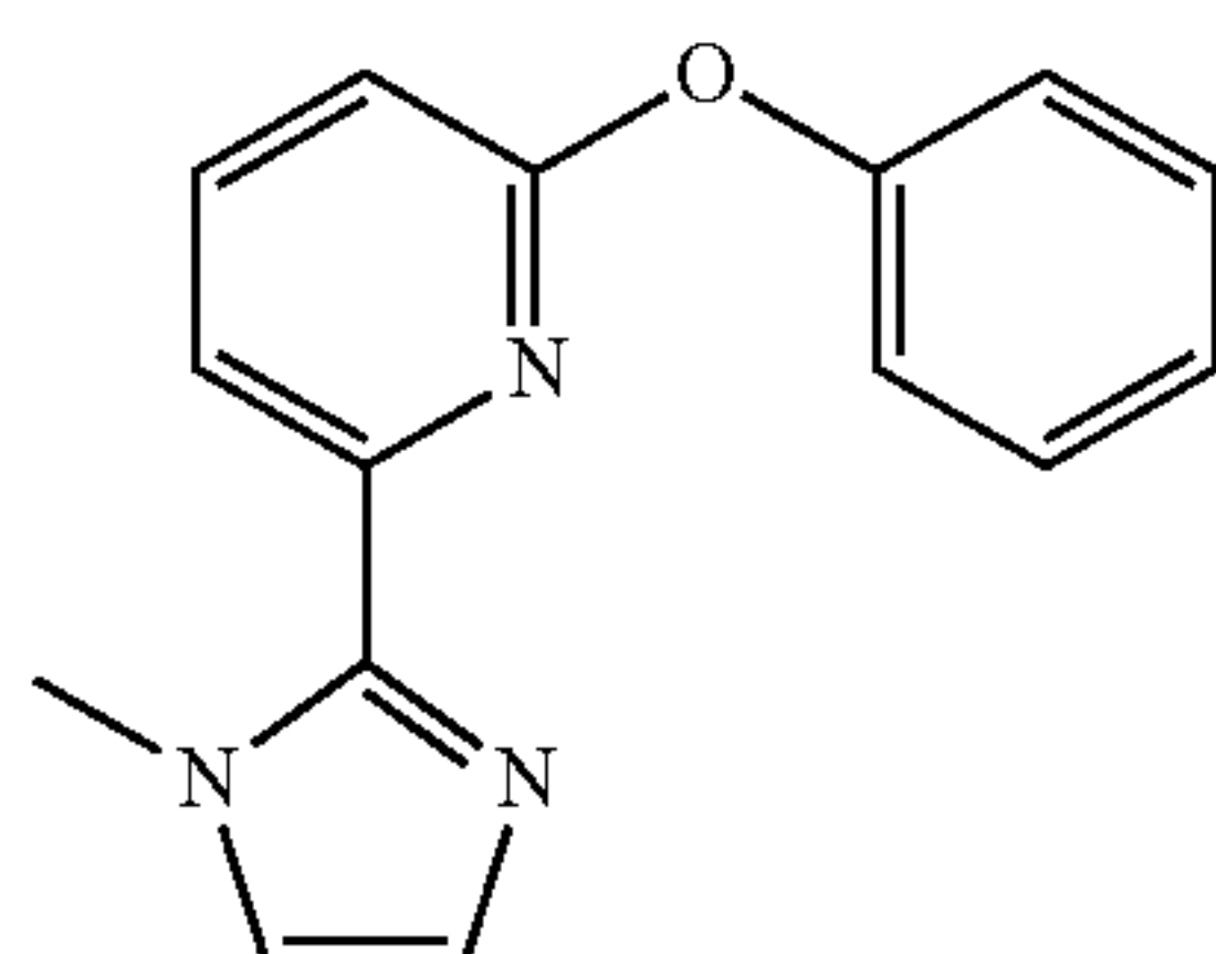
MIz-Py-O-Ph
