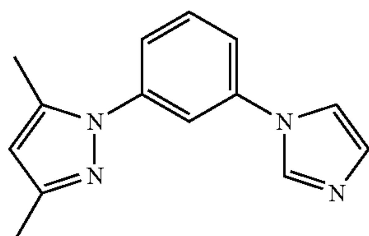
DMPz—Ph—Iz
