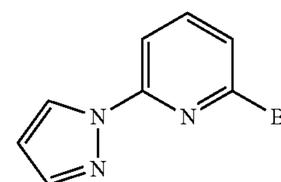
Pz-Py-Br
