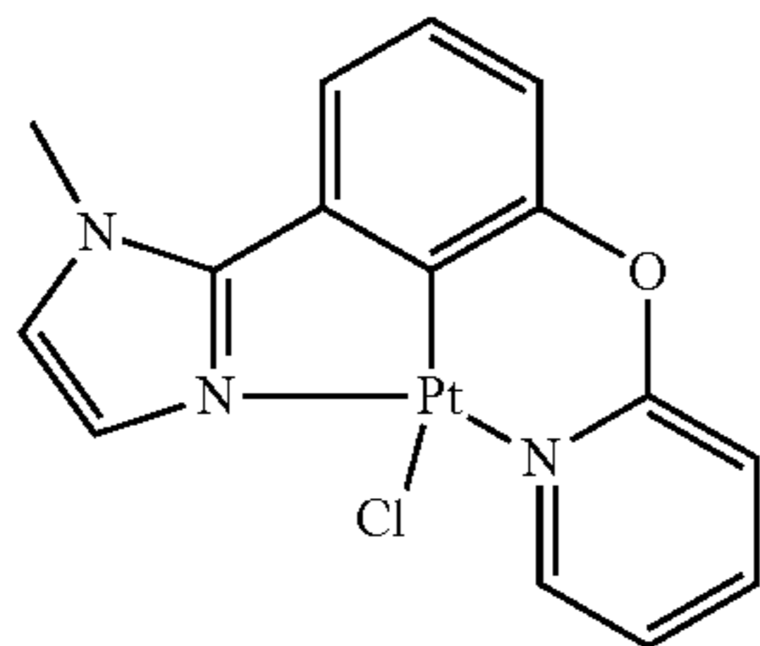
MIz-Ph-O-Py-PtCl
