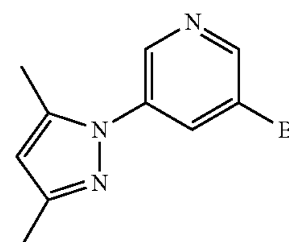
DMPz—Ph—Br
