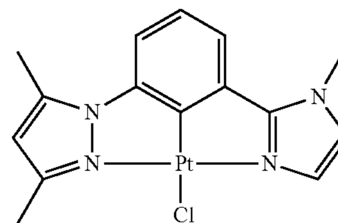
DMPz—Ph—MIz—PtCl
