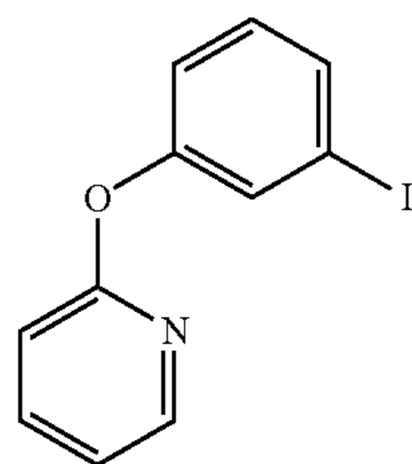
Py-O-Ph-I
