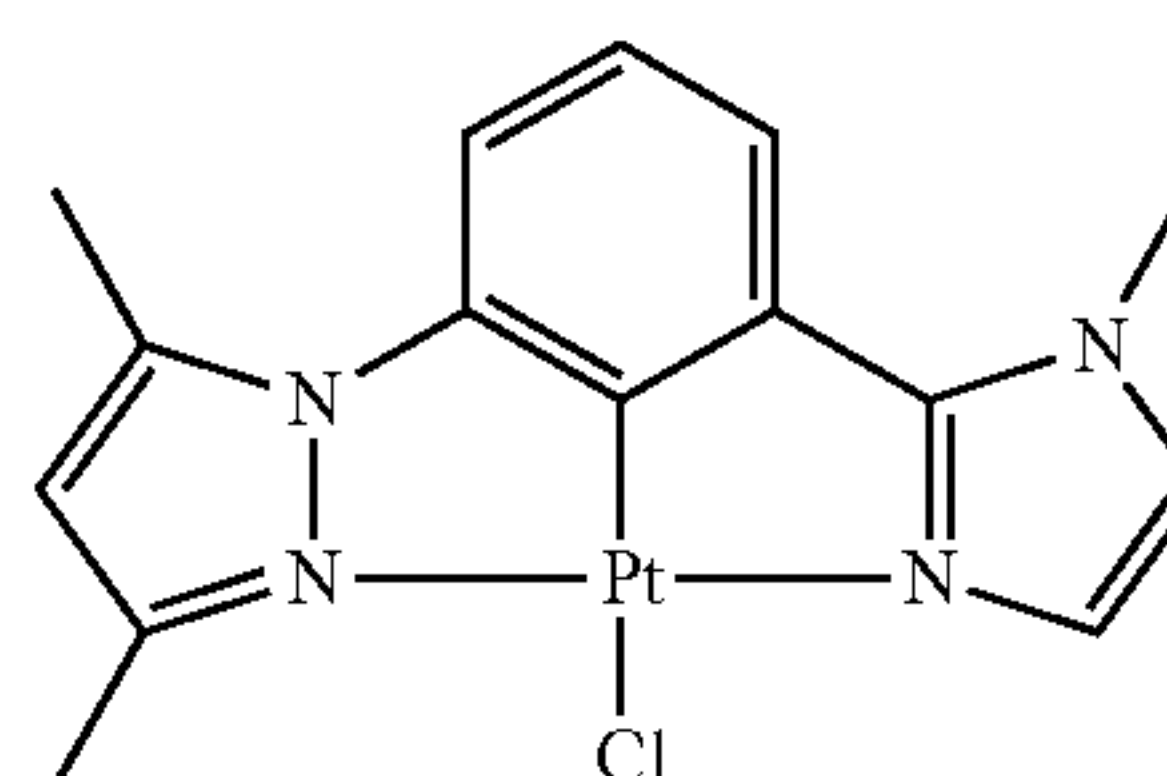
DMPz—Ph—MIz—PtCl
