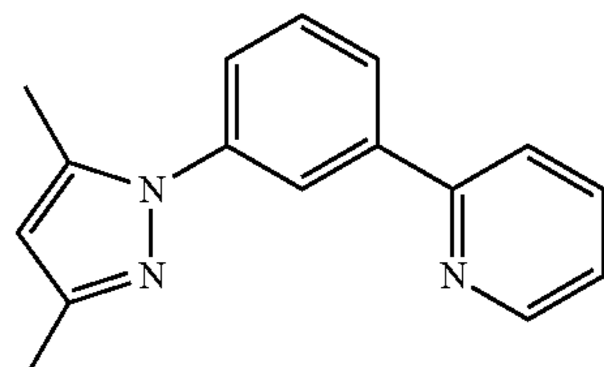
DMPz—Ph—Py
