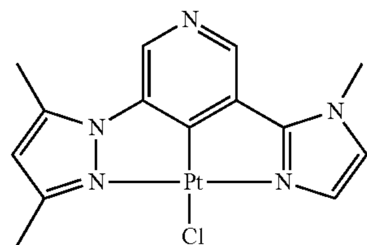
DMPz—Py—MIz—PtCl
