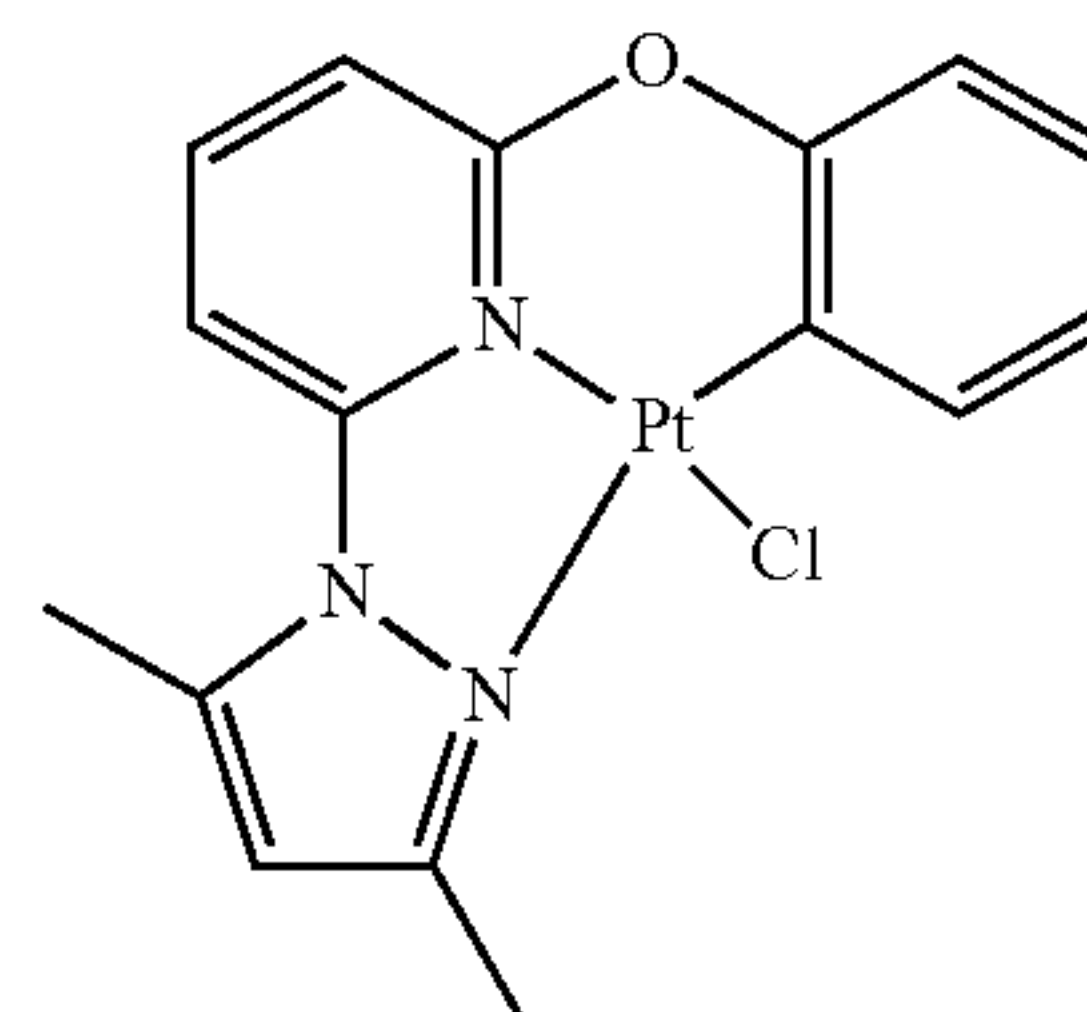
DMPz-Py-O-Ph-PtCl
