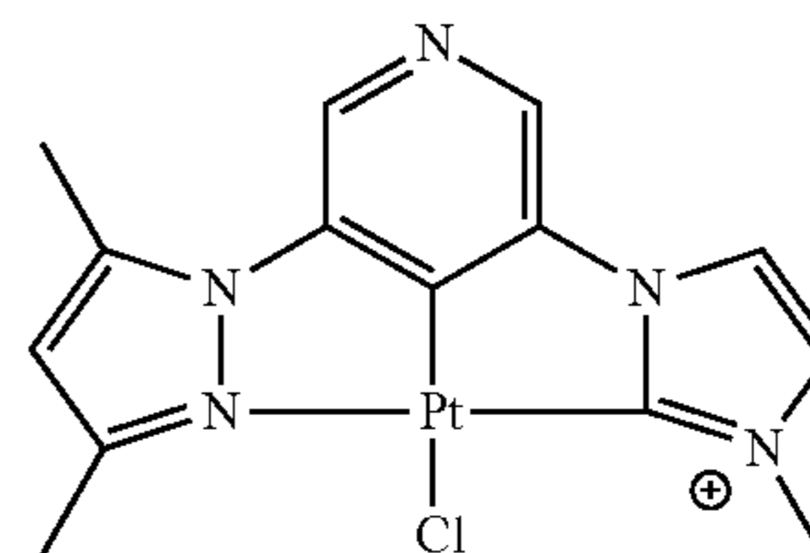
DMPz—Py—MIzCb—PtCl
