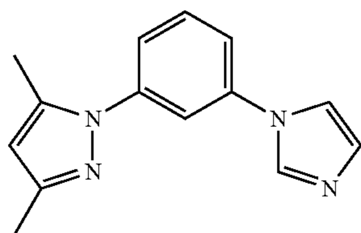
DMPz—Ph—Iz
