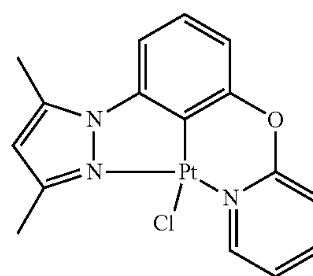
DMPz-Ph-O-Py-PtCl
