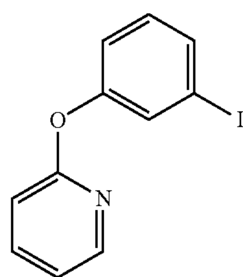
Py-O-Ph-I
