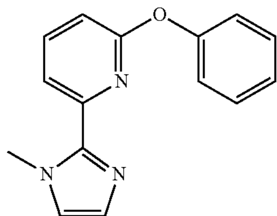
MIz-Py-O-Ph
