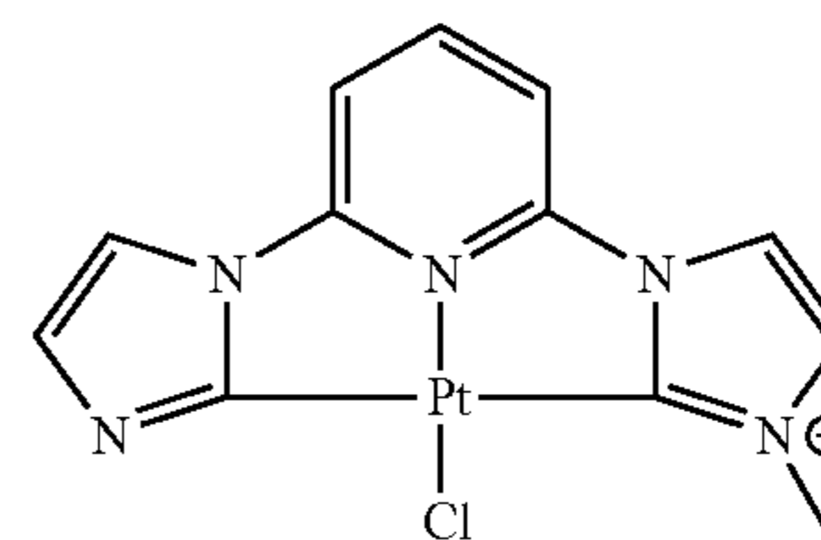
Iz-Py-MIzCb-PtCl
