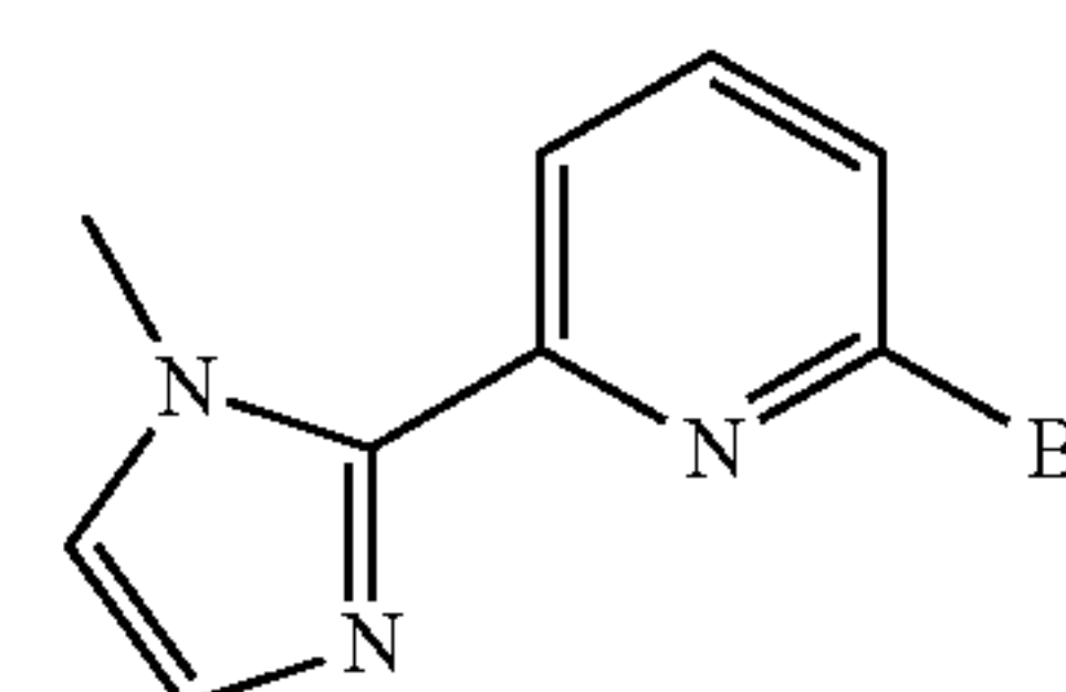
MIz-Py-Br
