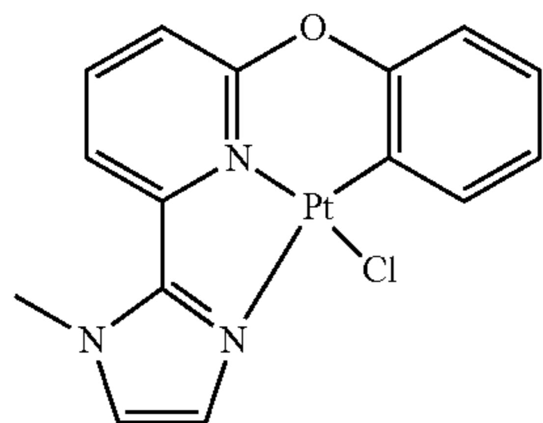
MIz-Py-O-Ph-PtCl
