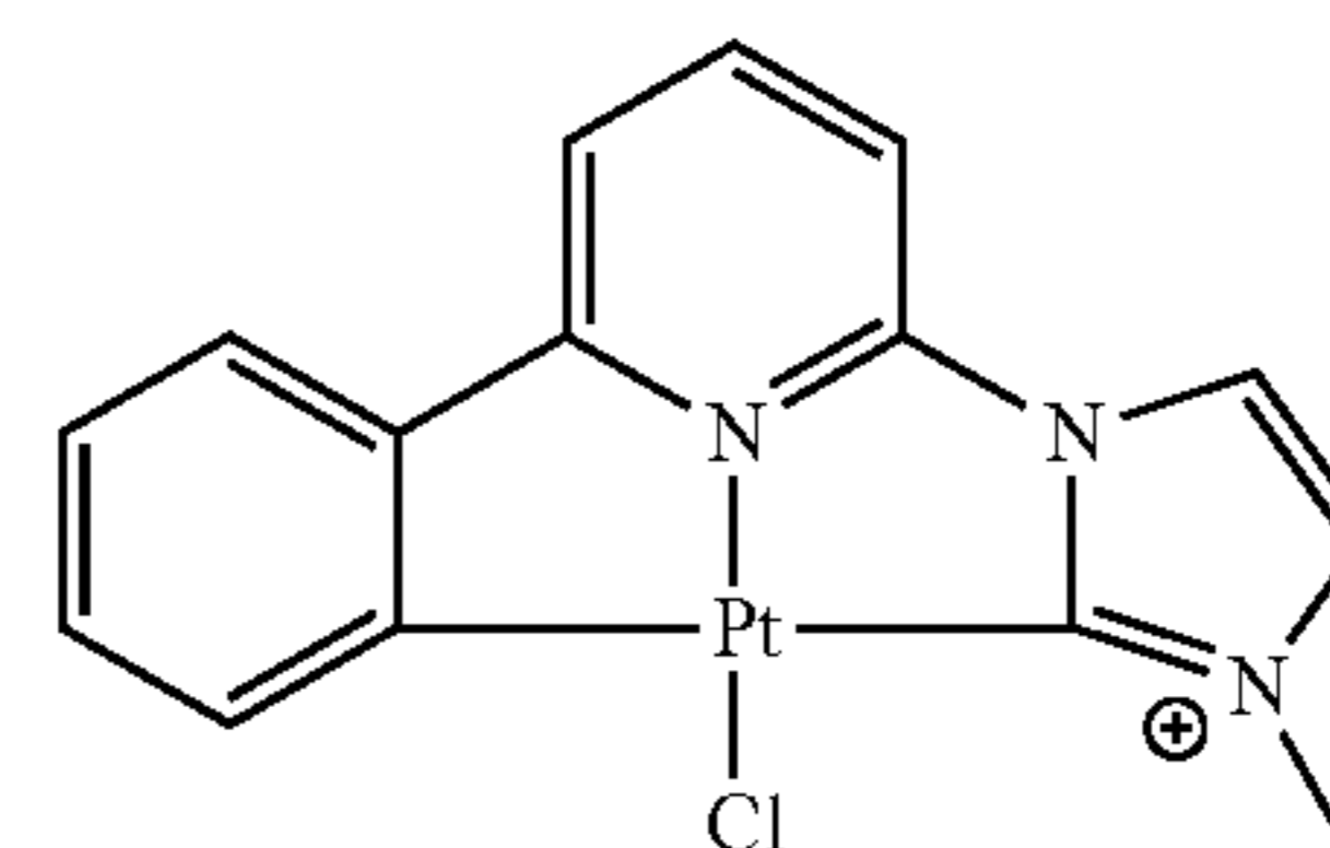
Ph-Py-MIzCb-PtCl
