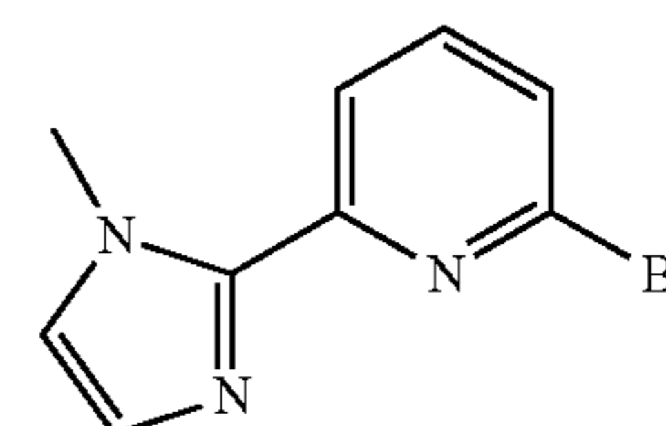
MIz-Py-Br
