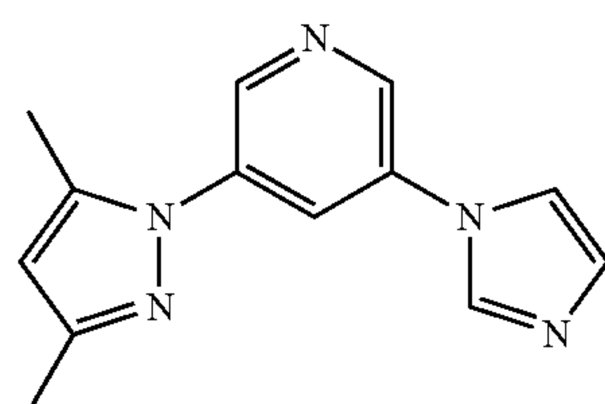
DMPz—Py—Iz
