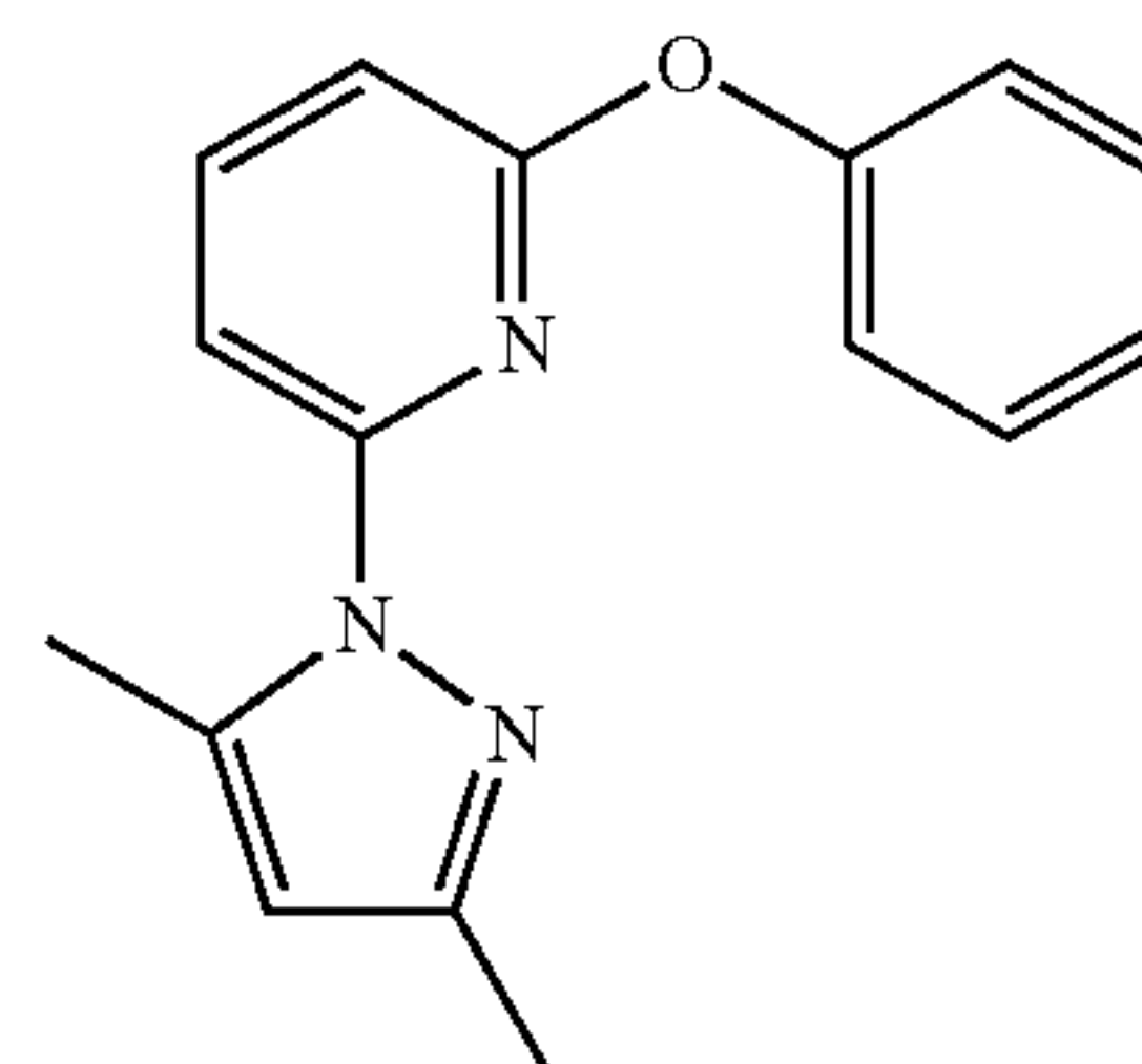
DMPz-Py-O-Ph
