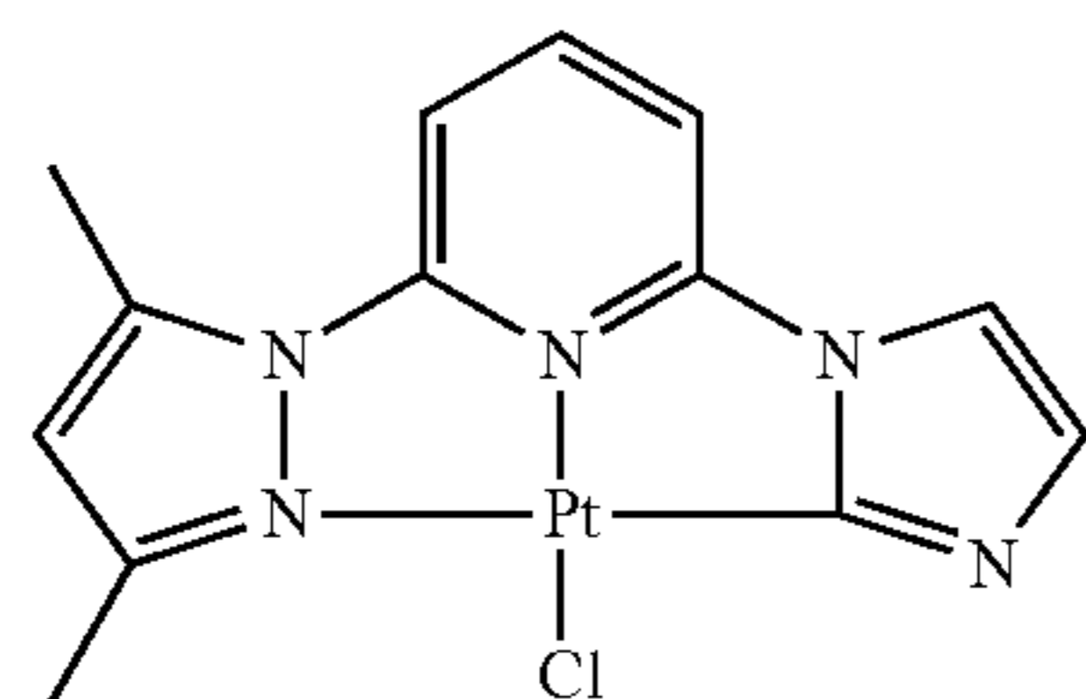
DMPz-Py-Iz-PtCl
