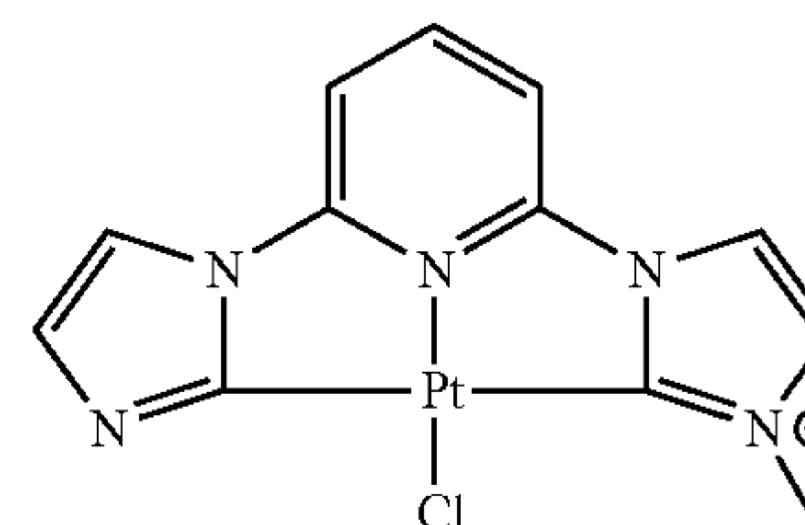
Iz-Py-MIzCb-PtCl
