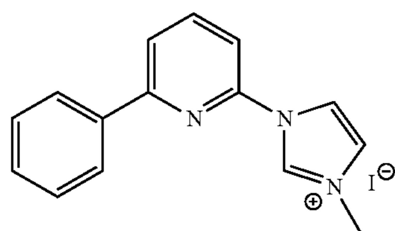
Ph-Py-IMIz
