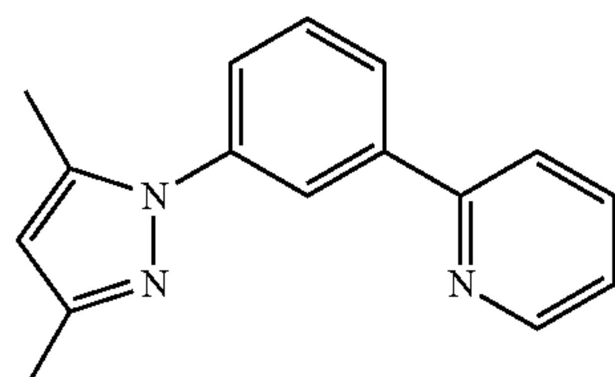
DMPz—Ph—Py
