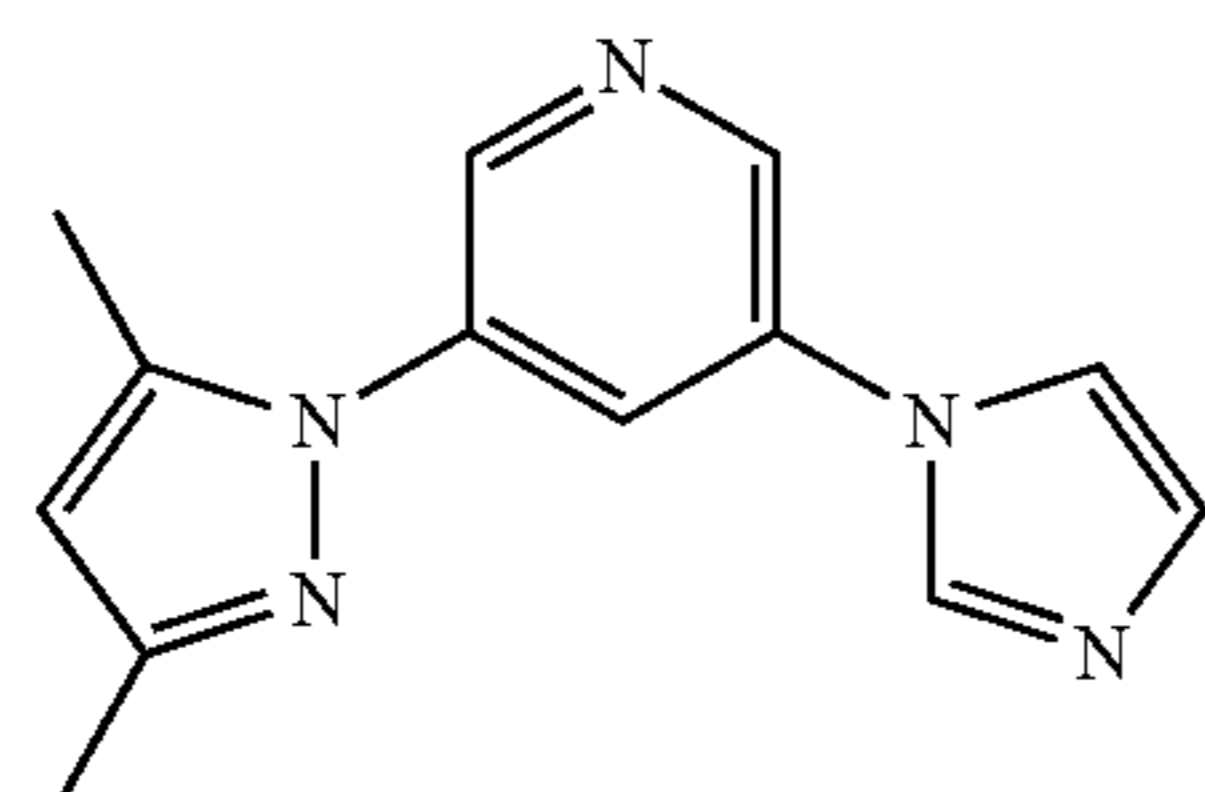
DMPz—Py—Iz
