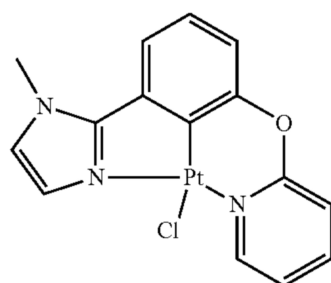
MIz-Ph-O-Py-PtCl
