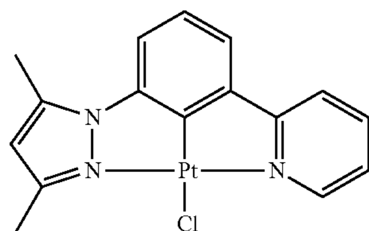
DMPz—Ph—Py—PtCl
