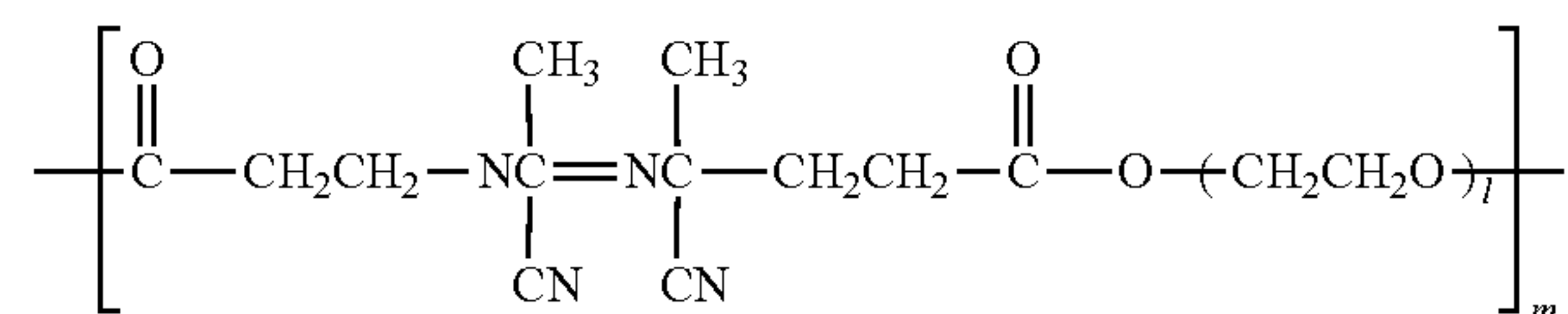
Formula 1
