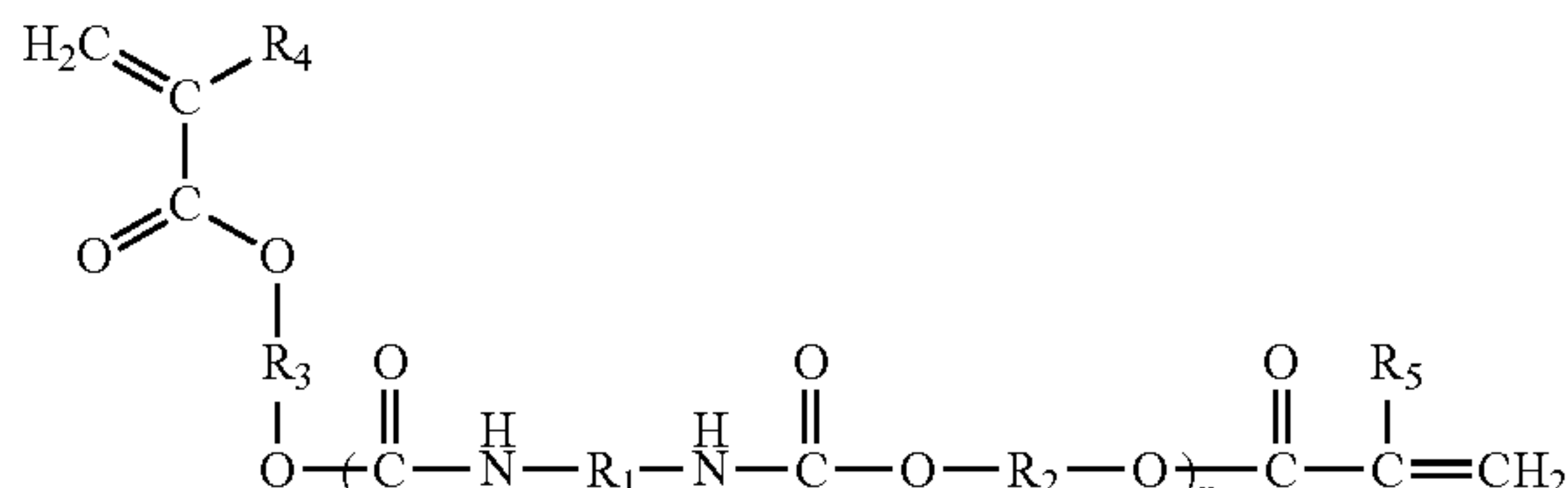
Formula 2
