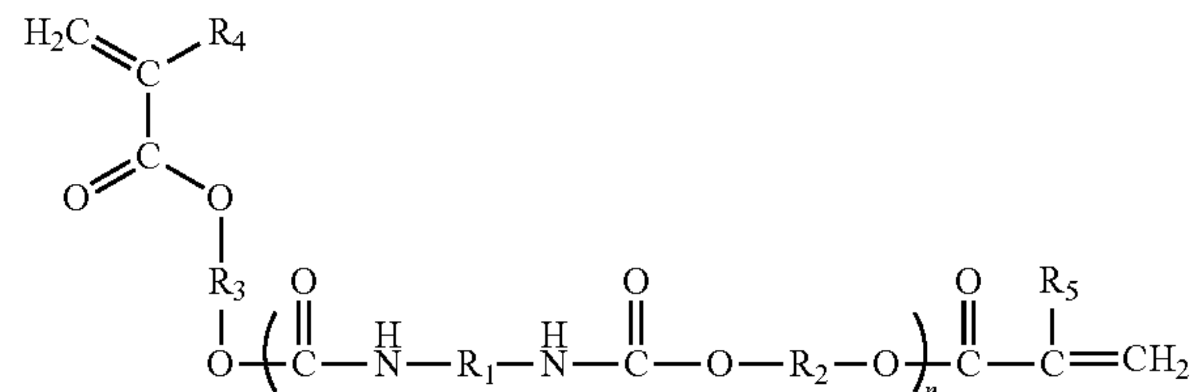
Formula 2
