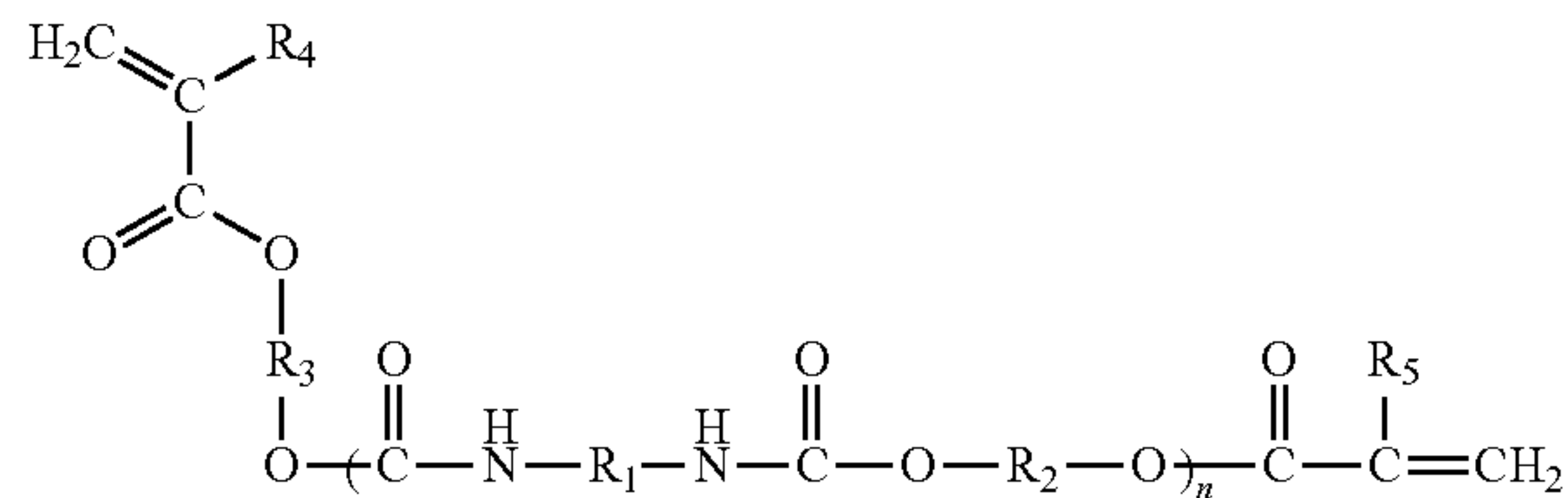
Formula 2
