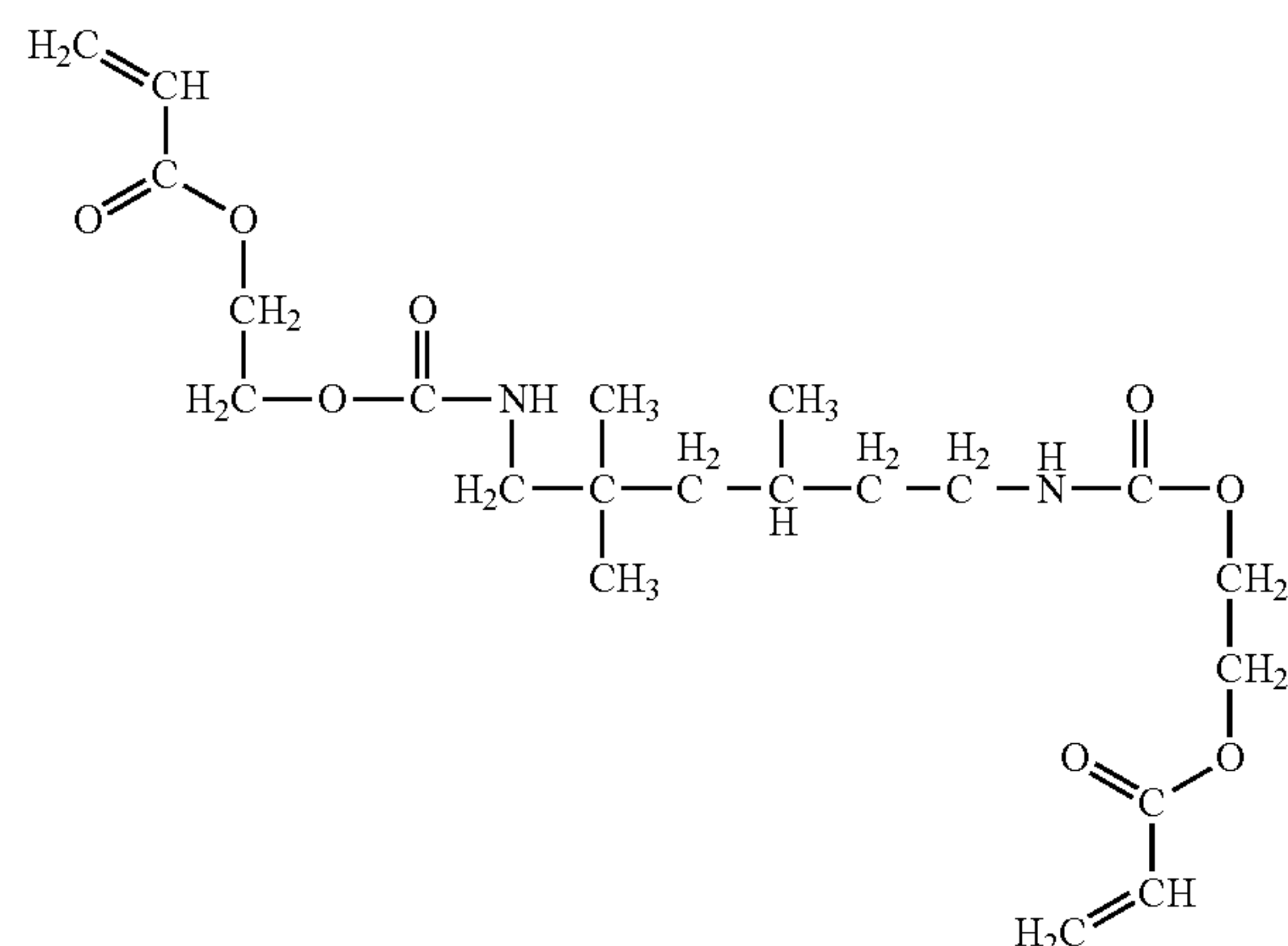
Formula 7
