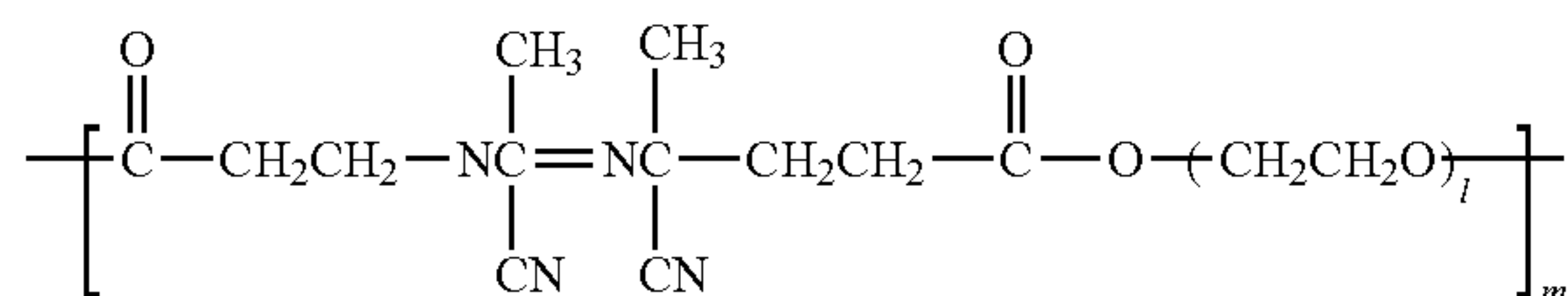
Formula 1
