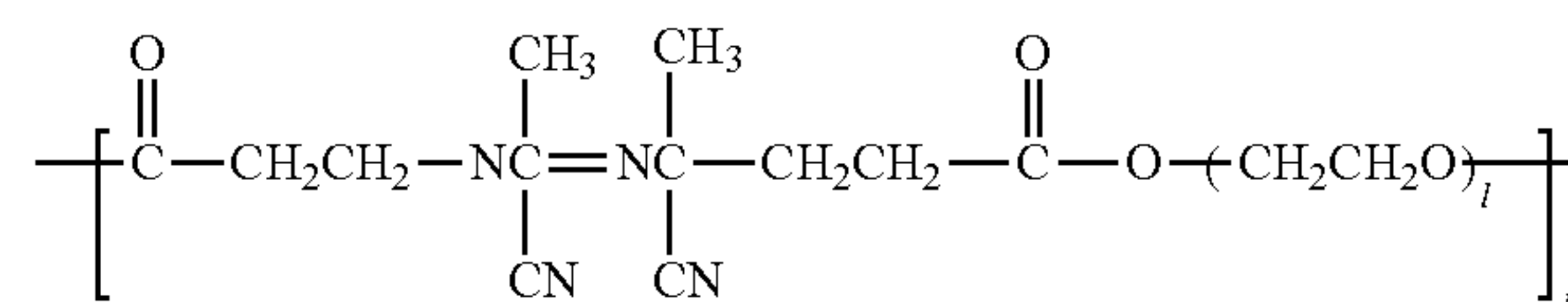
Formula 6
