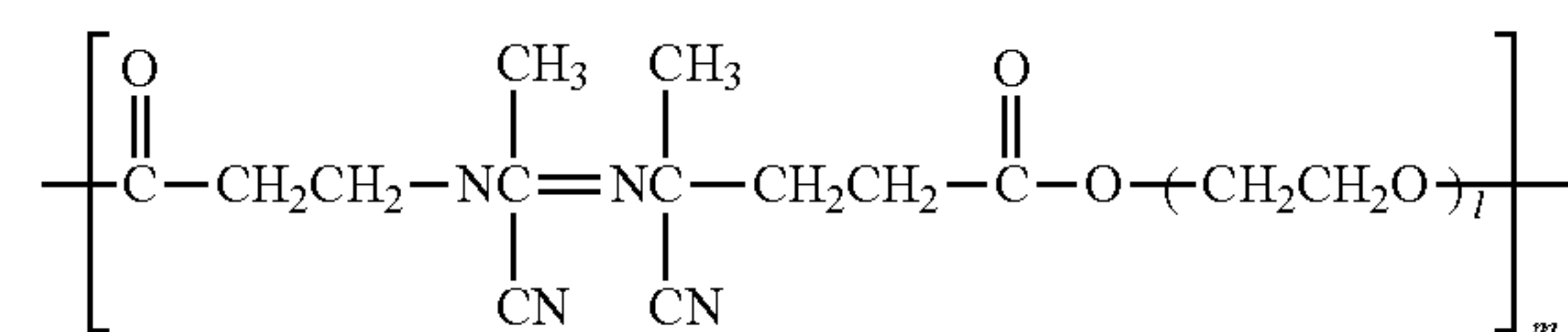
Formula 1
