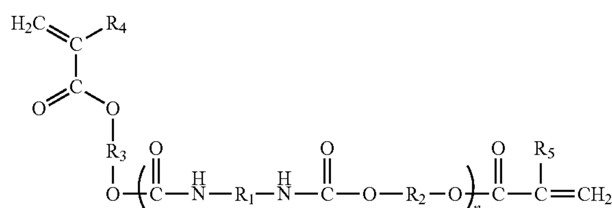
Formula 2
