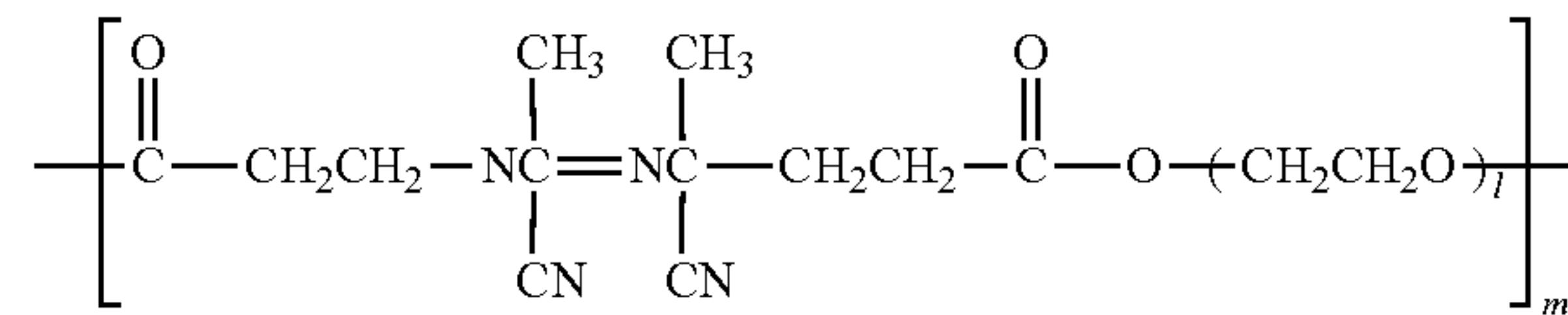
Formula 1
