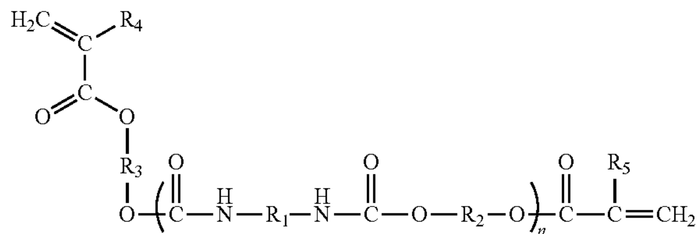
Formula 2
