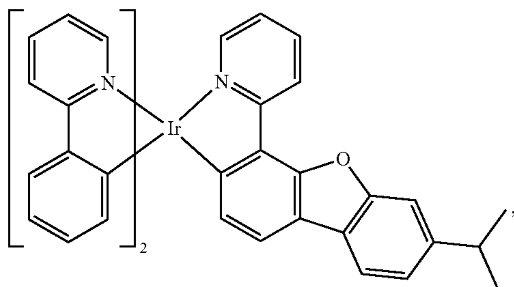
Compound 14
