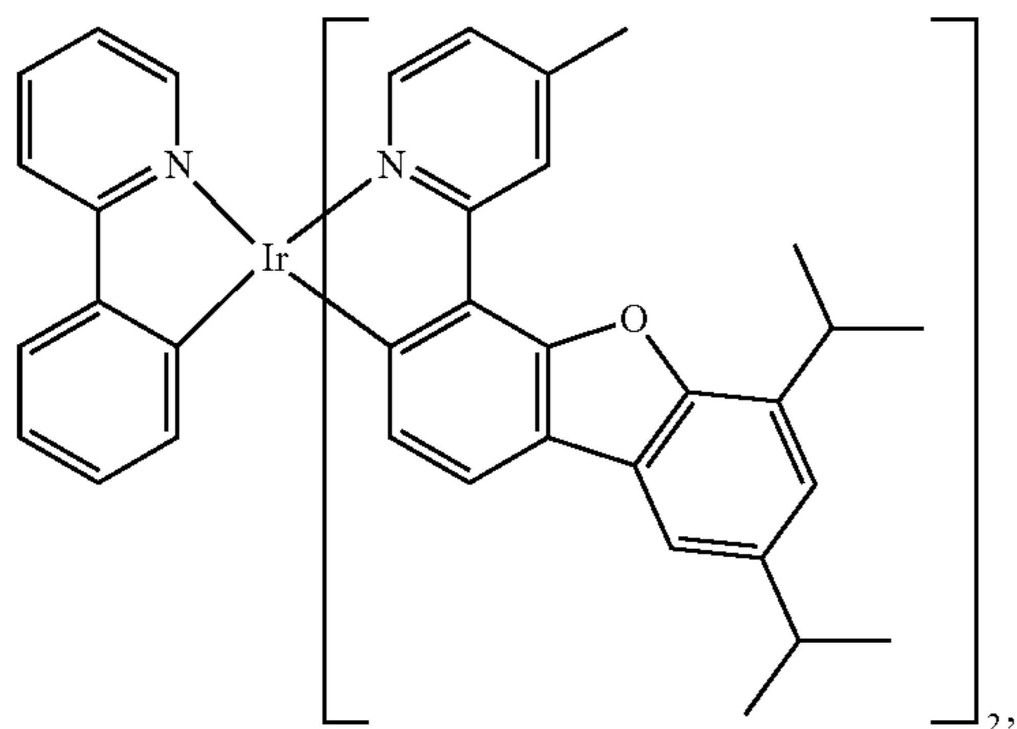
Compound 32
