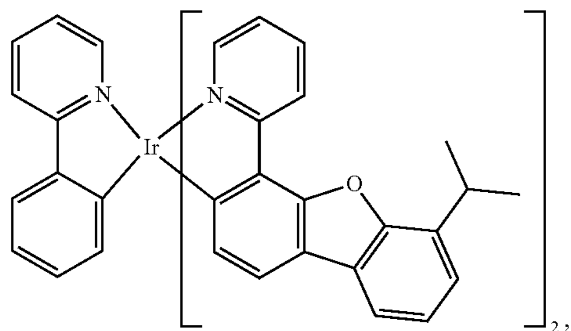
Compound 23
