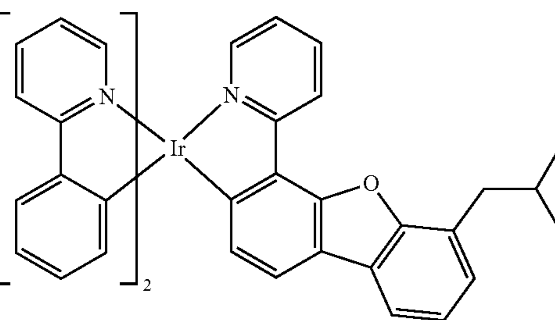
Compound 8
