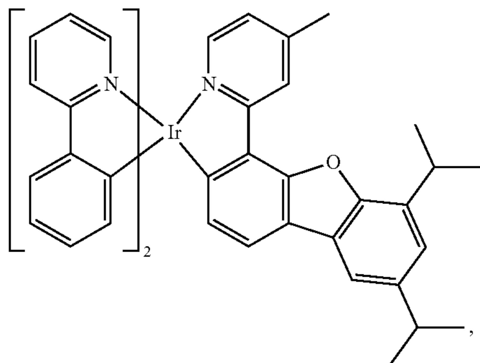
Compound 31
