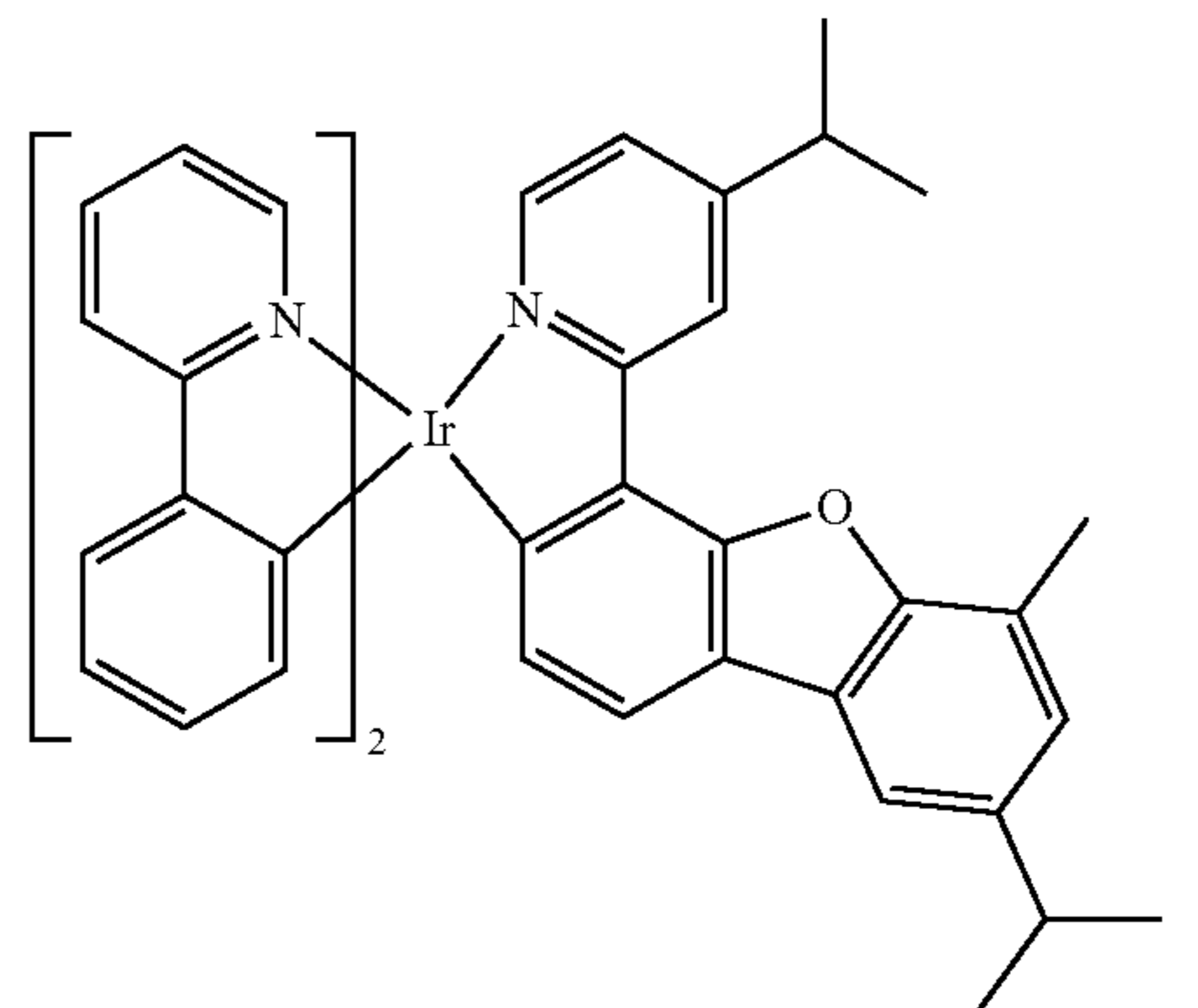
Compound 36
