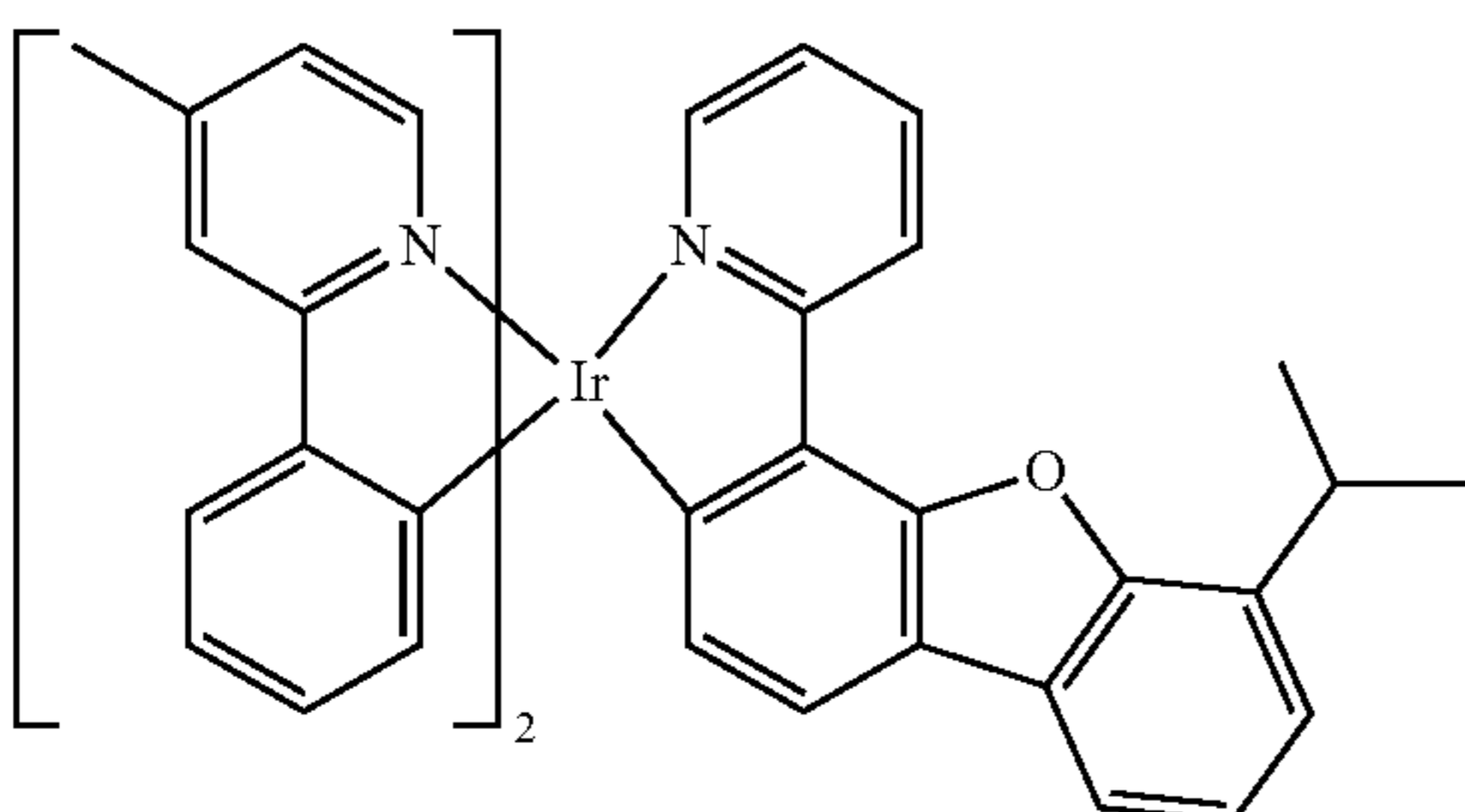
Compound 51
