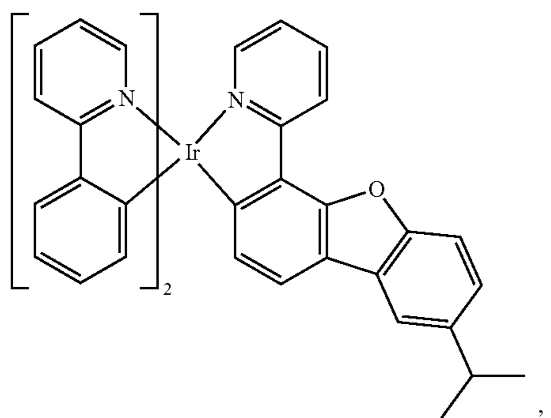
Compound 13
