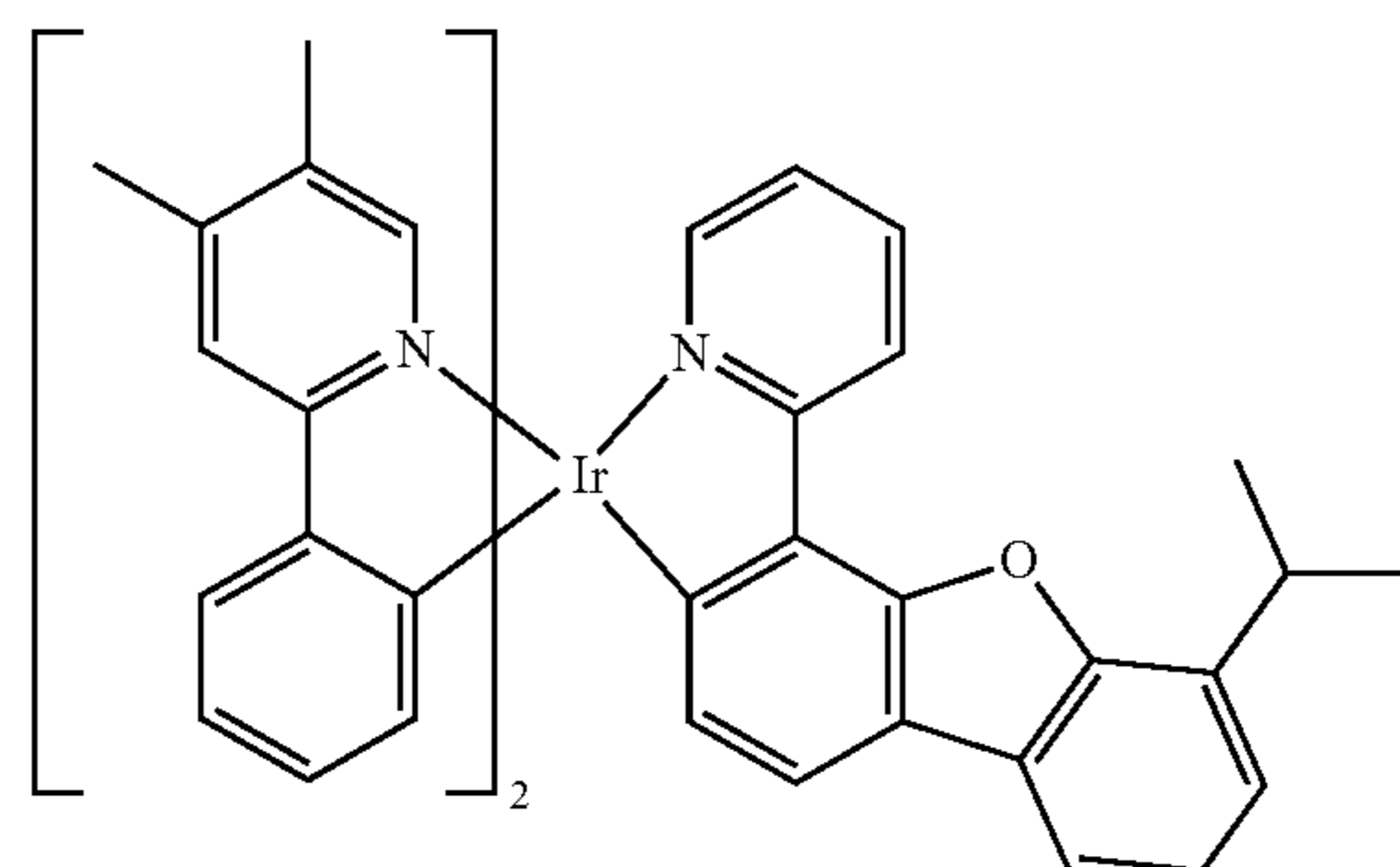
Compound 49
