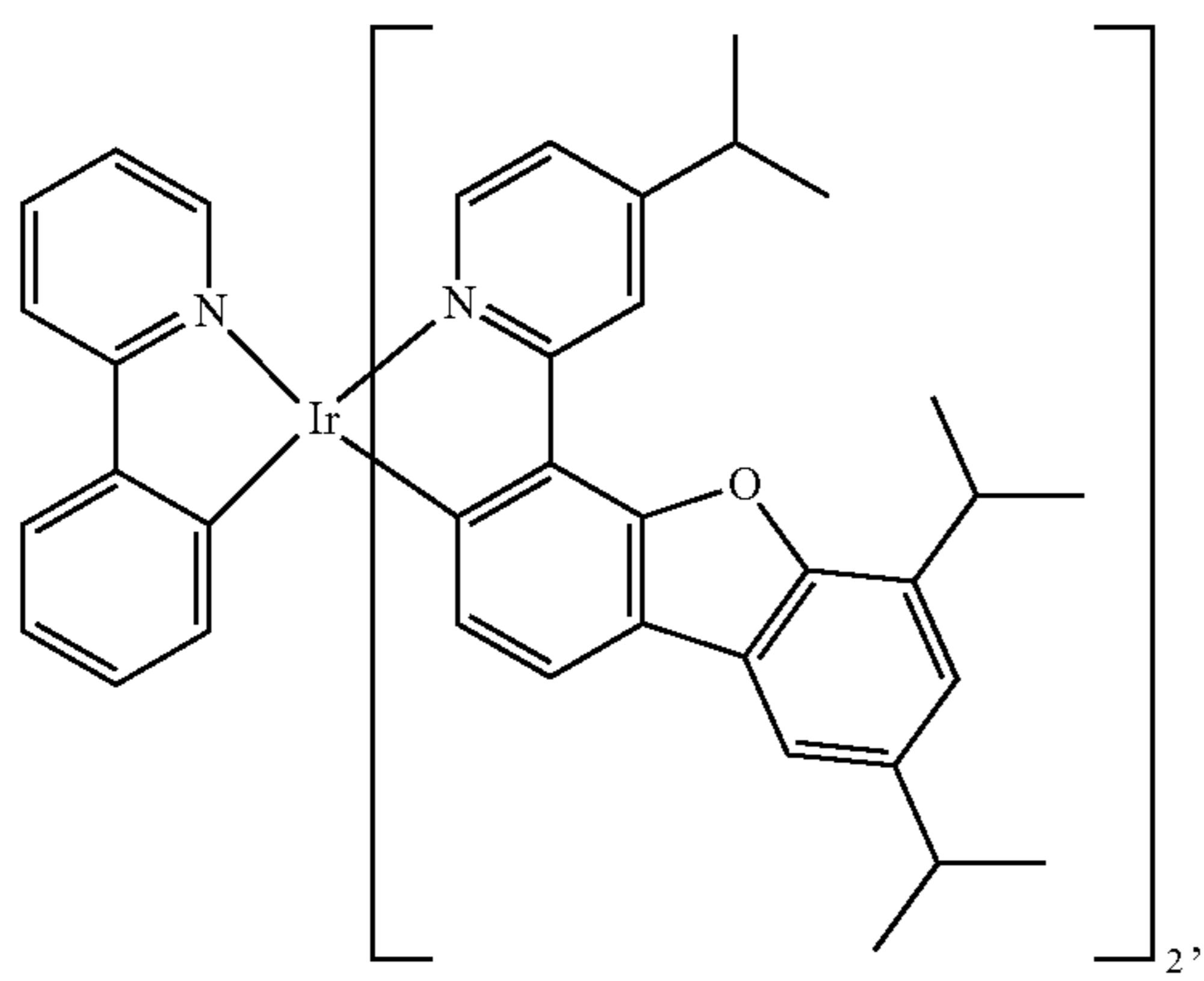
Compound 30
