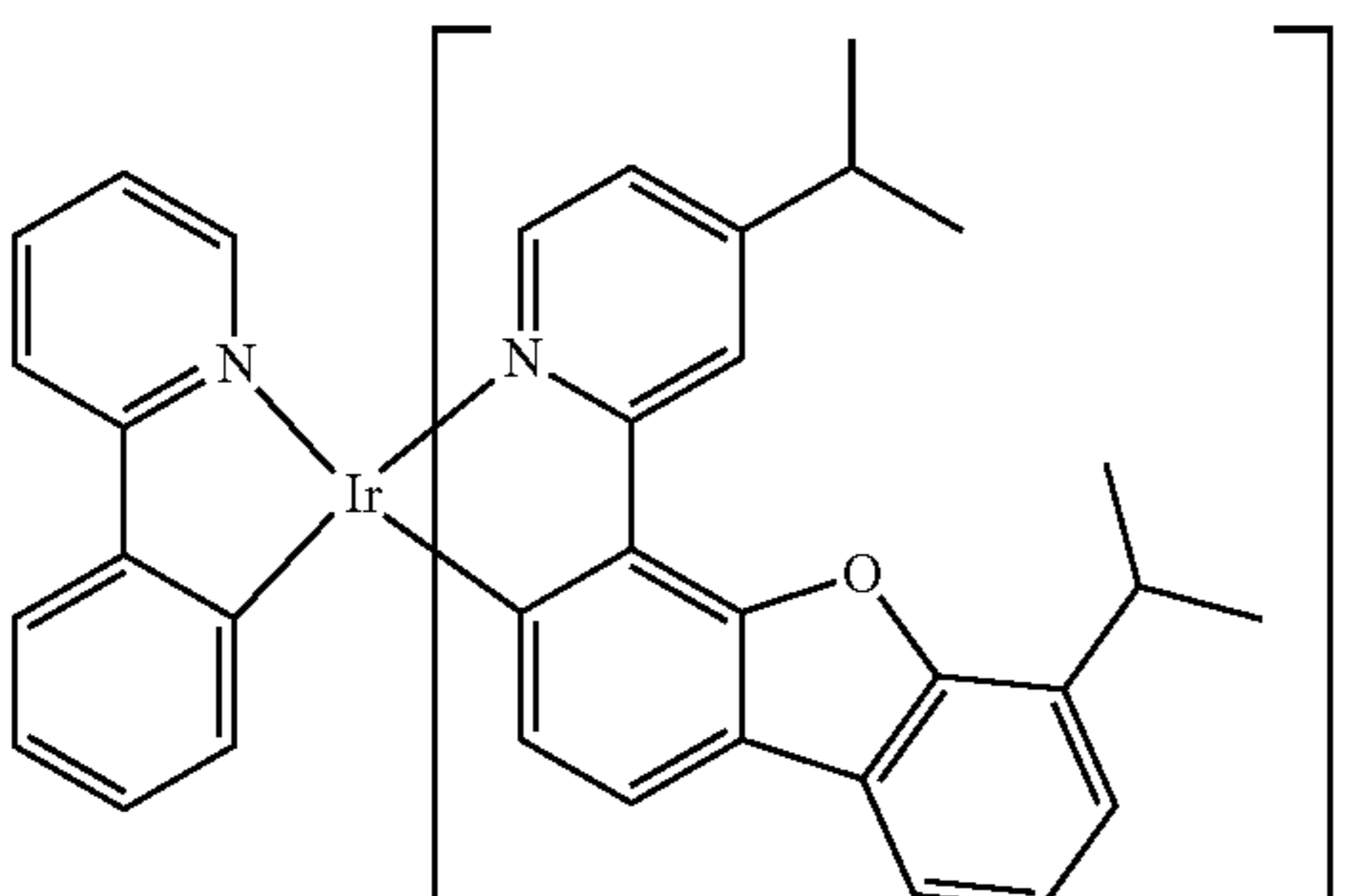
Compound 7
