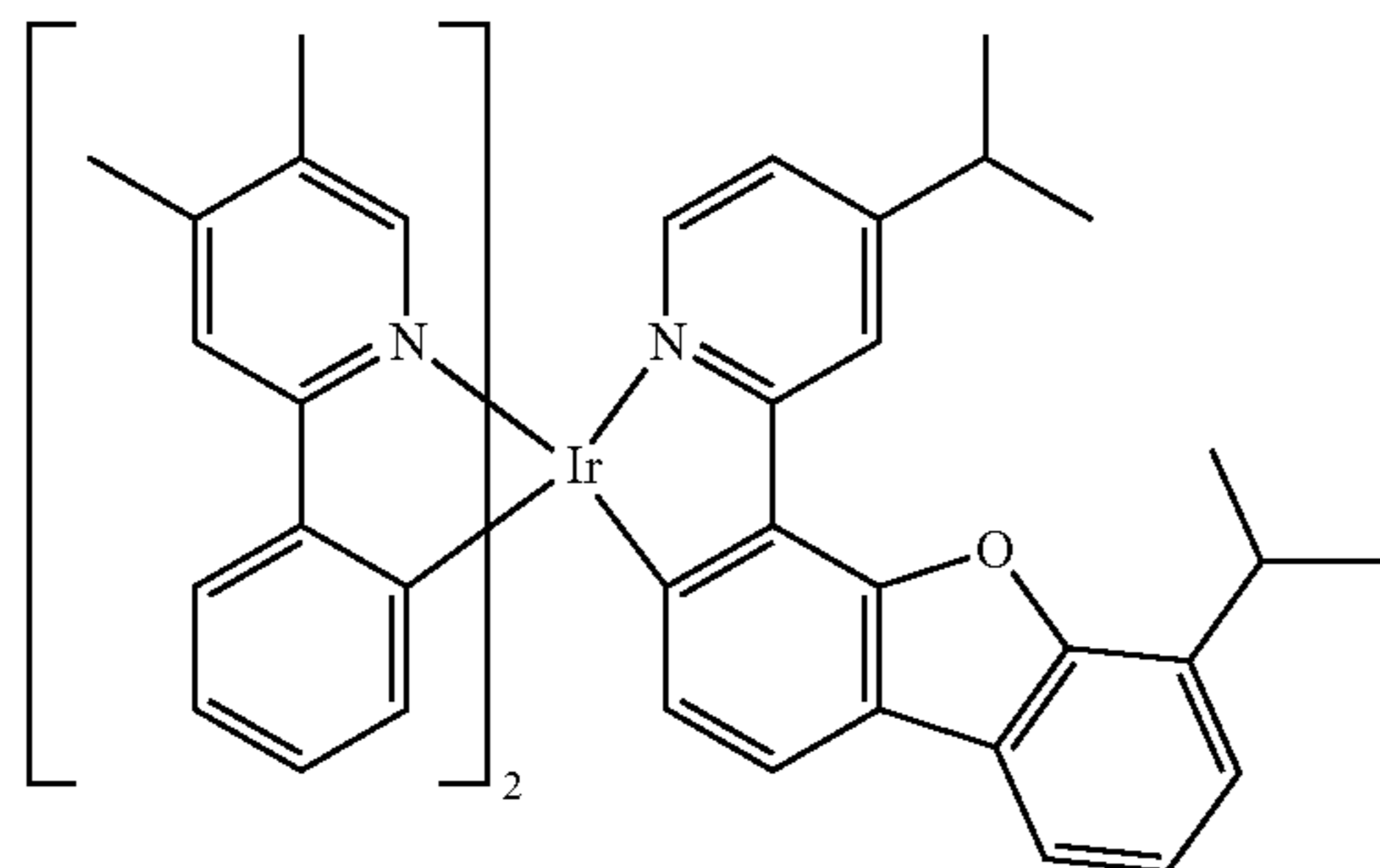
Compound 54
