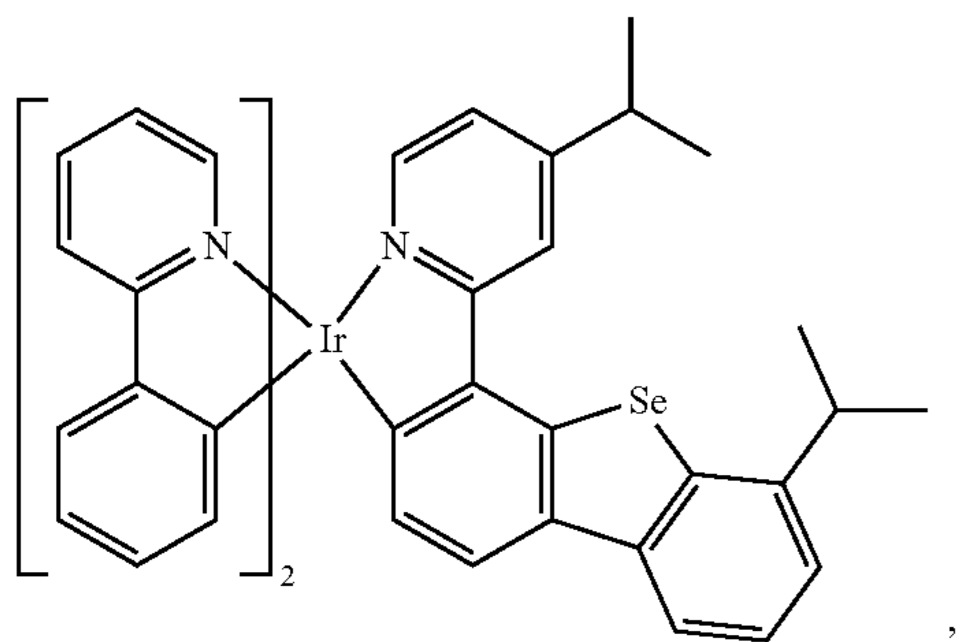
Compound 46
