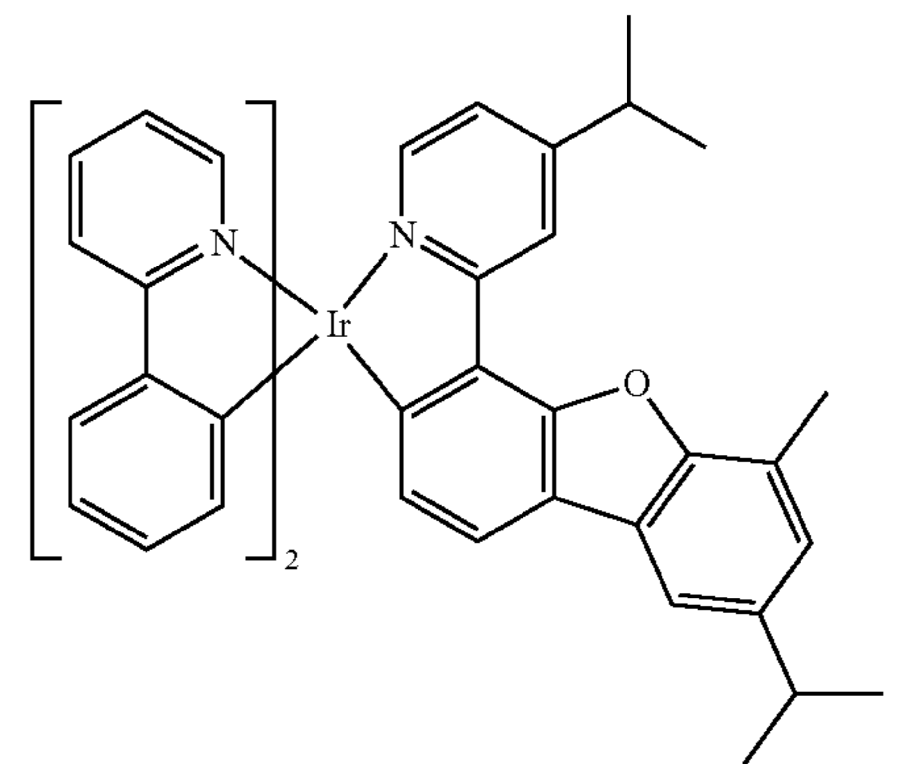
Compound 36
