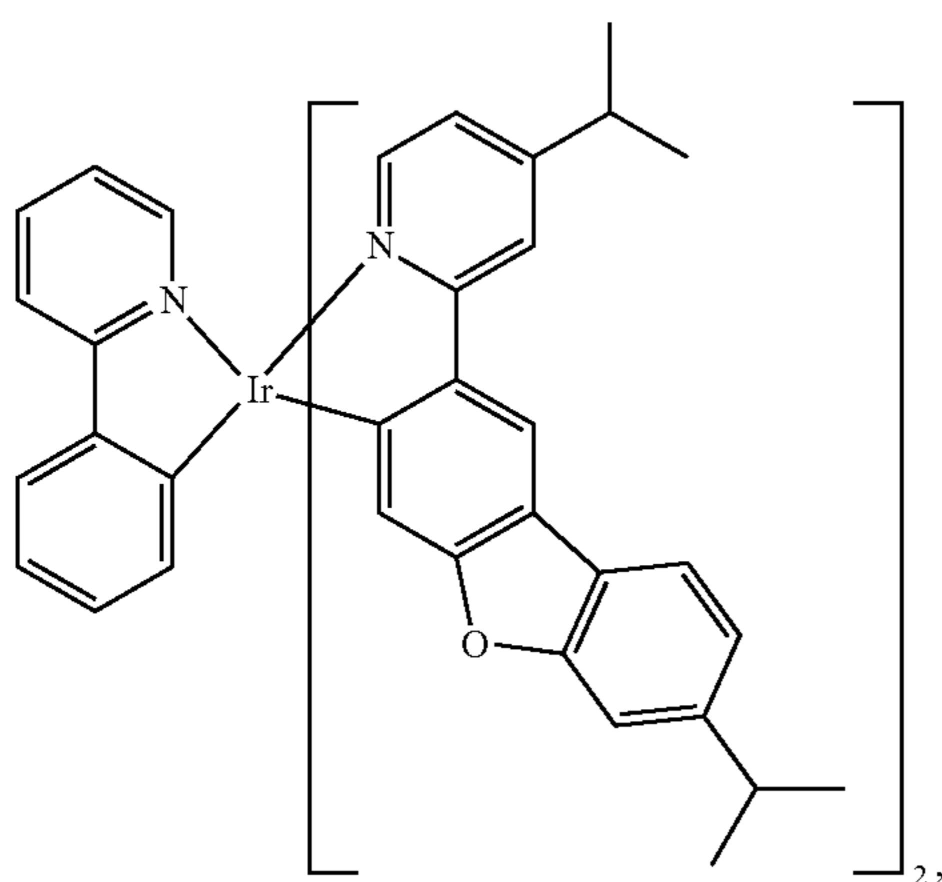
Compound 61
