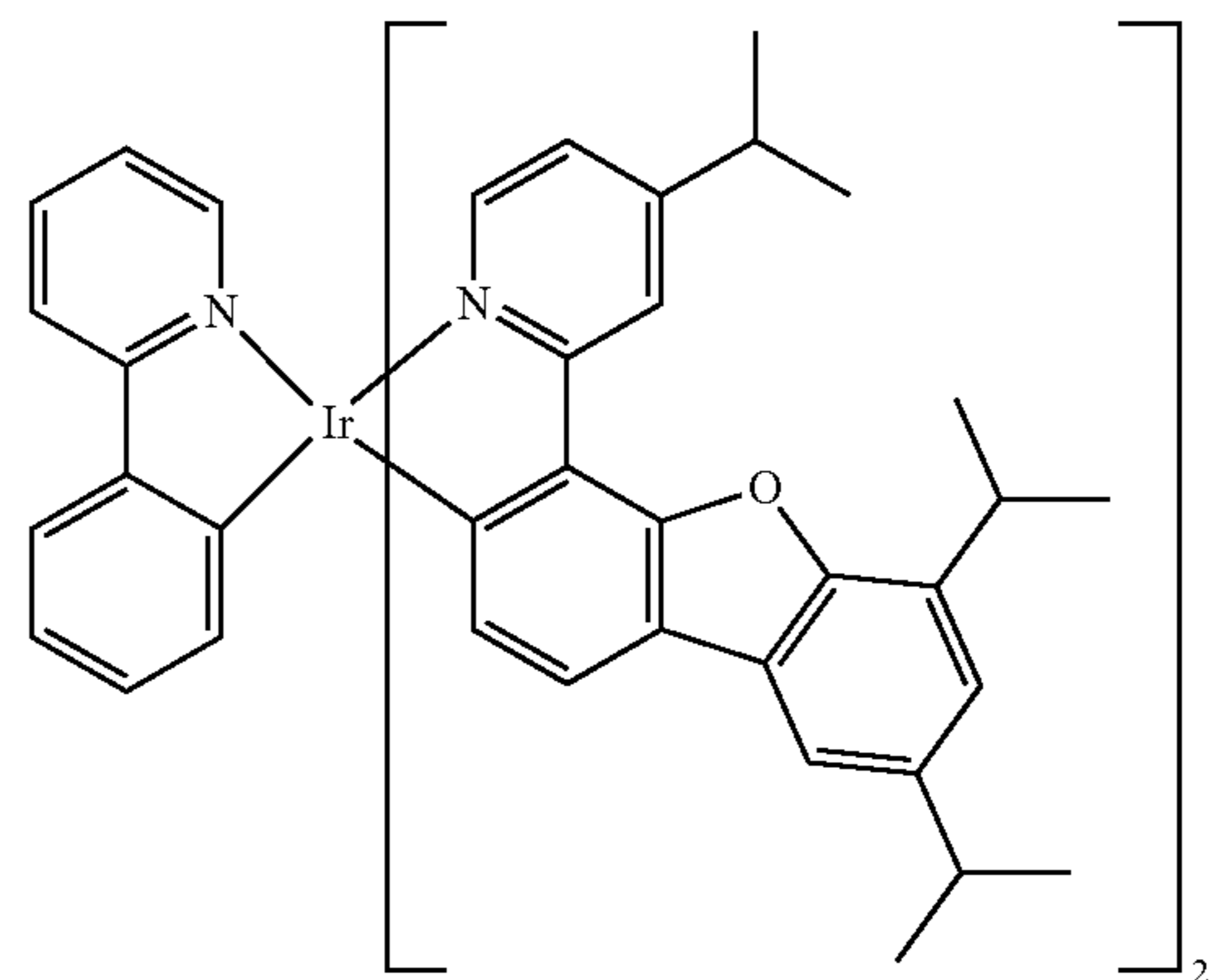
Compound 30
