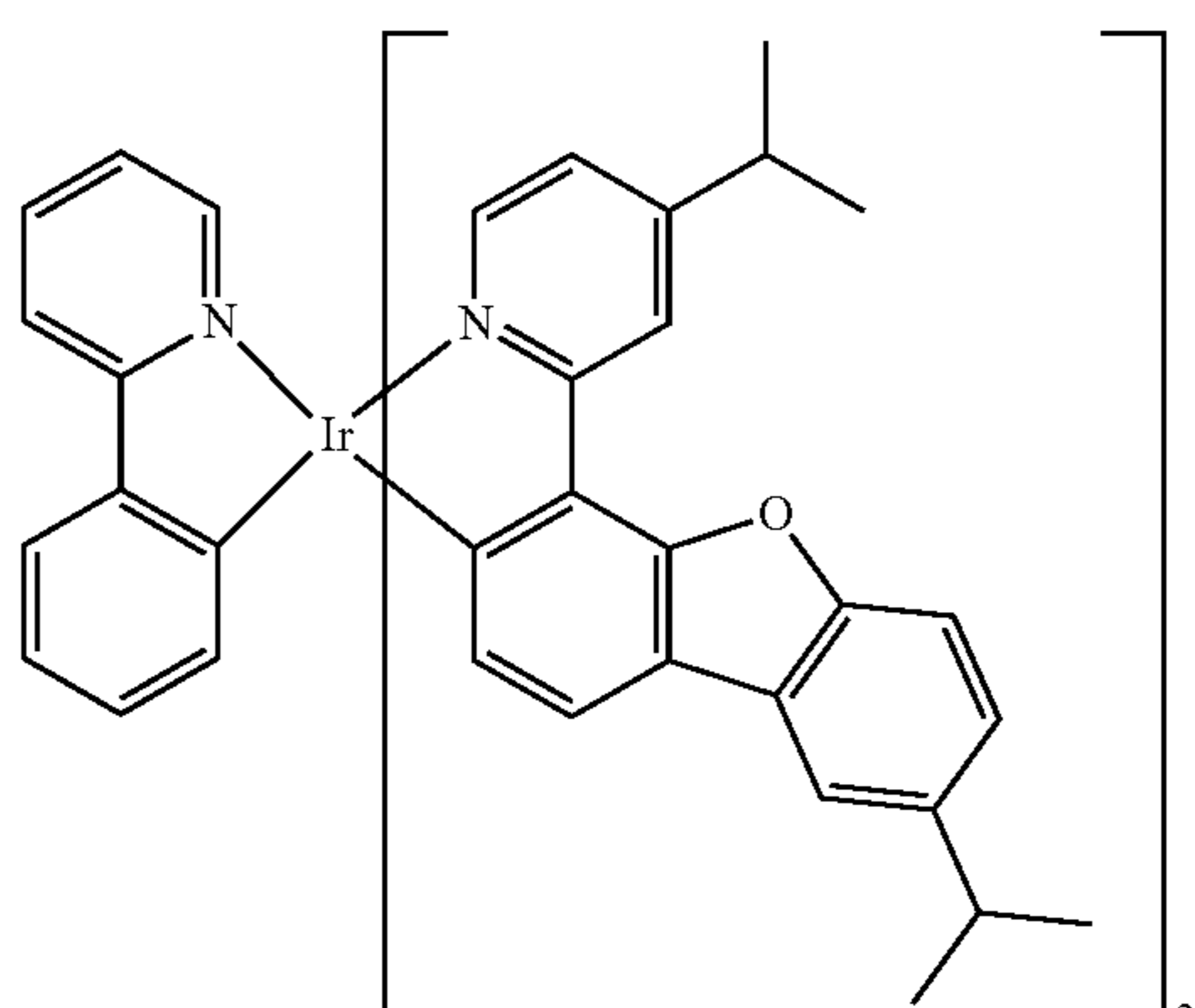
Compound 27
