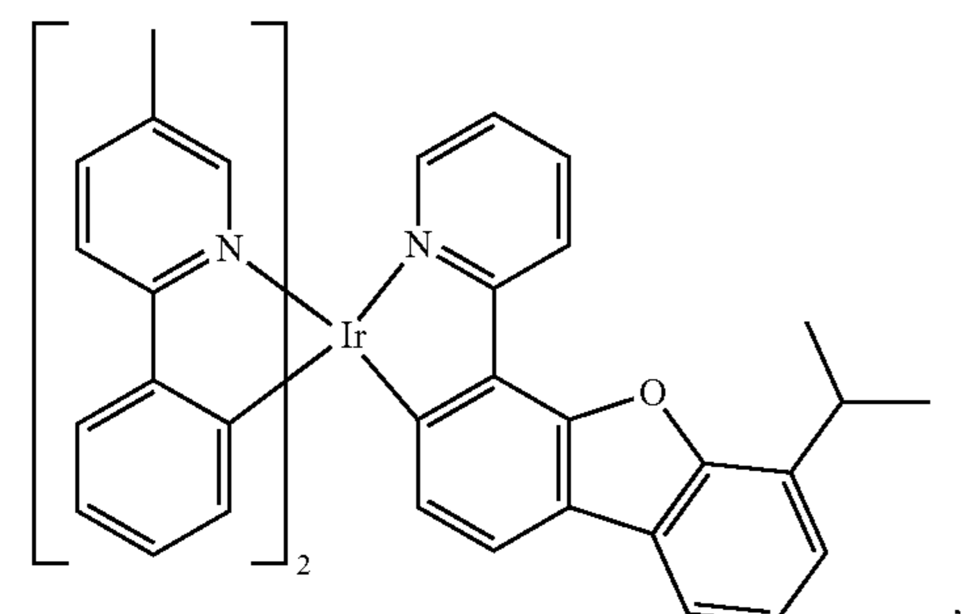
Compound 49
