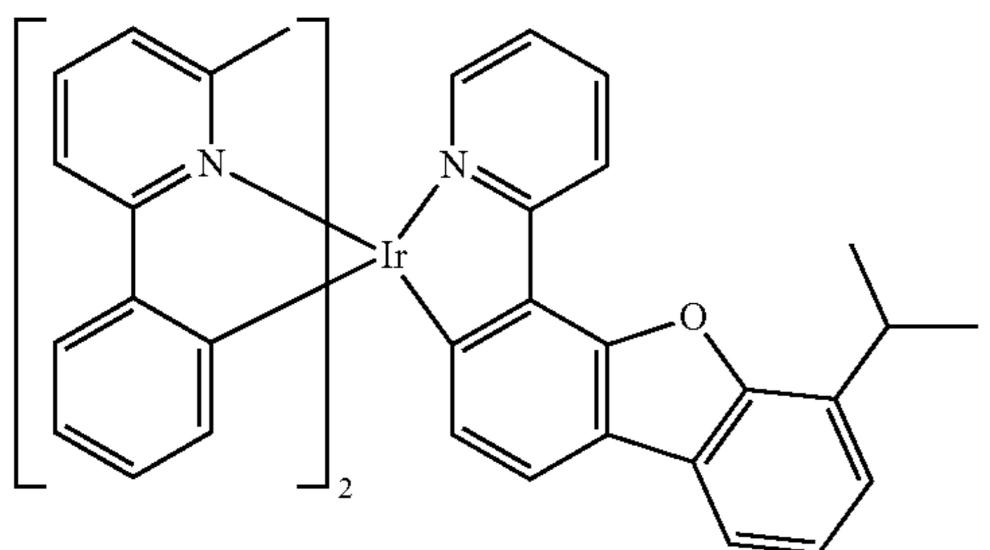
Compound 47
