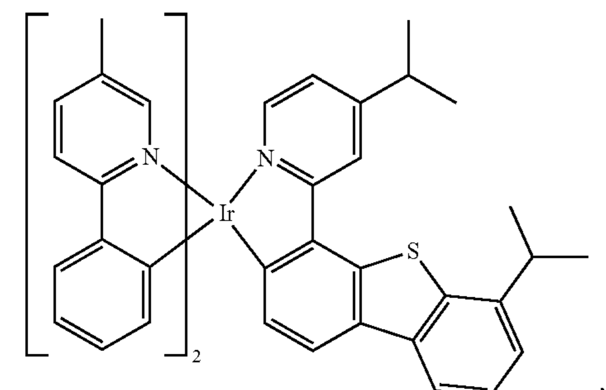
Compound 50
