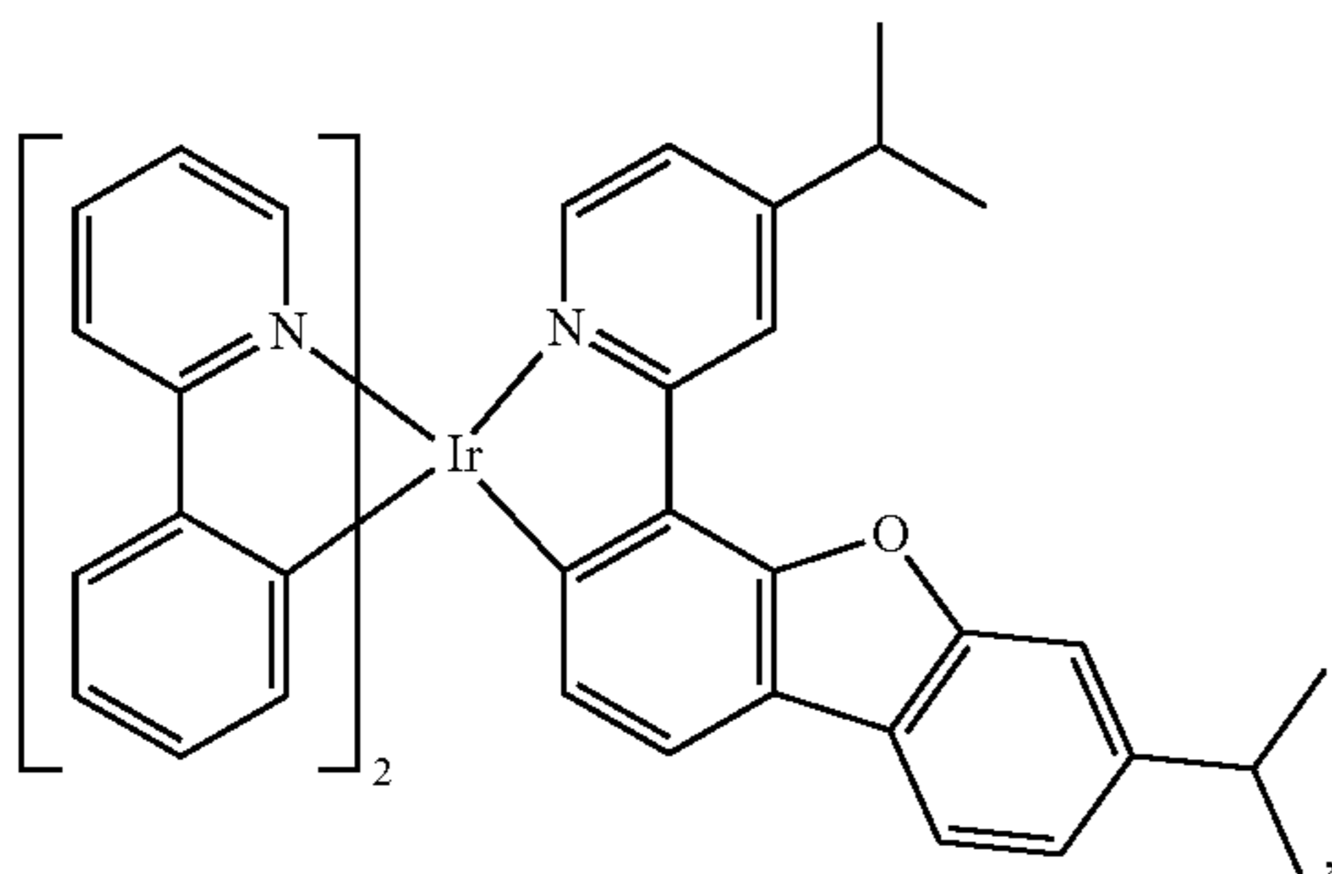
Compound 16
