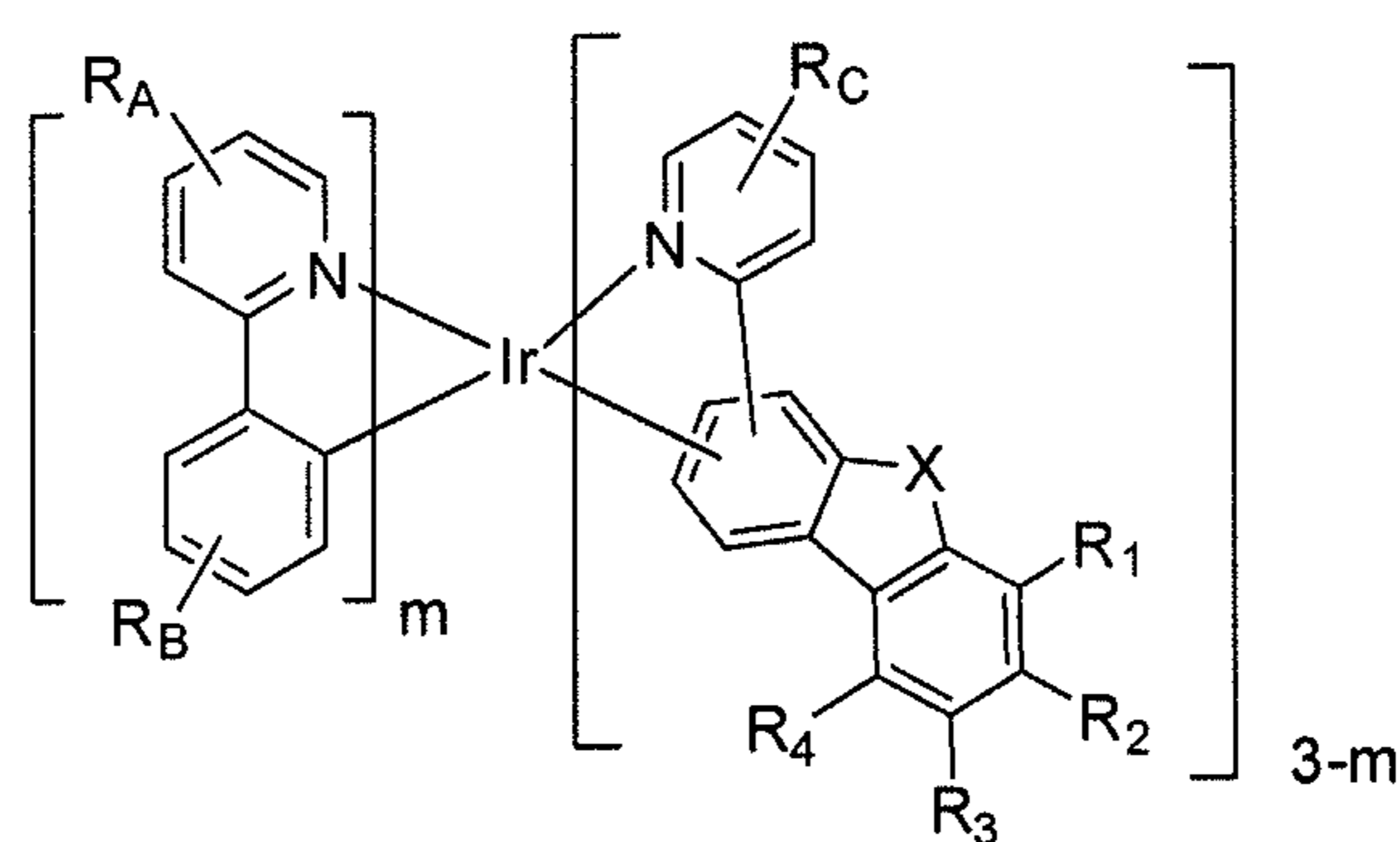
Formula I
