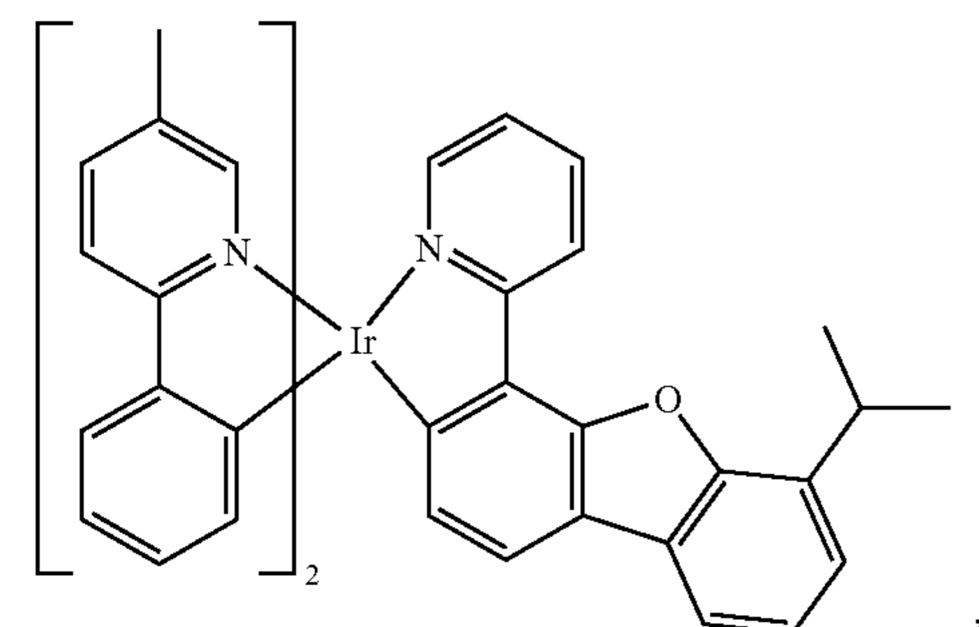
Compound 49
