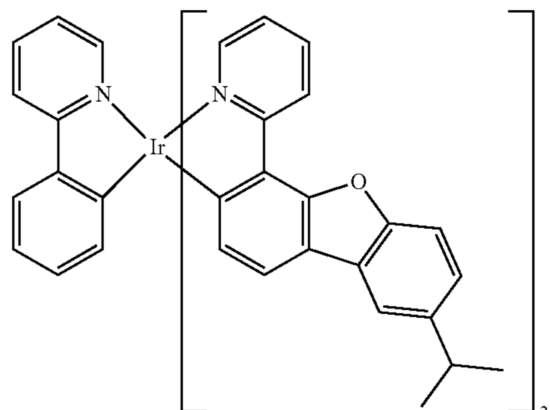
Compound 26
