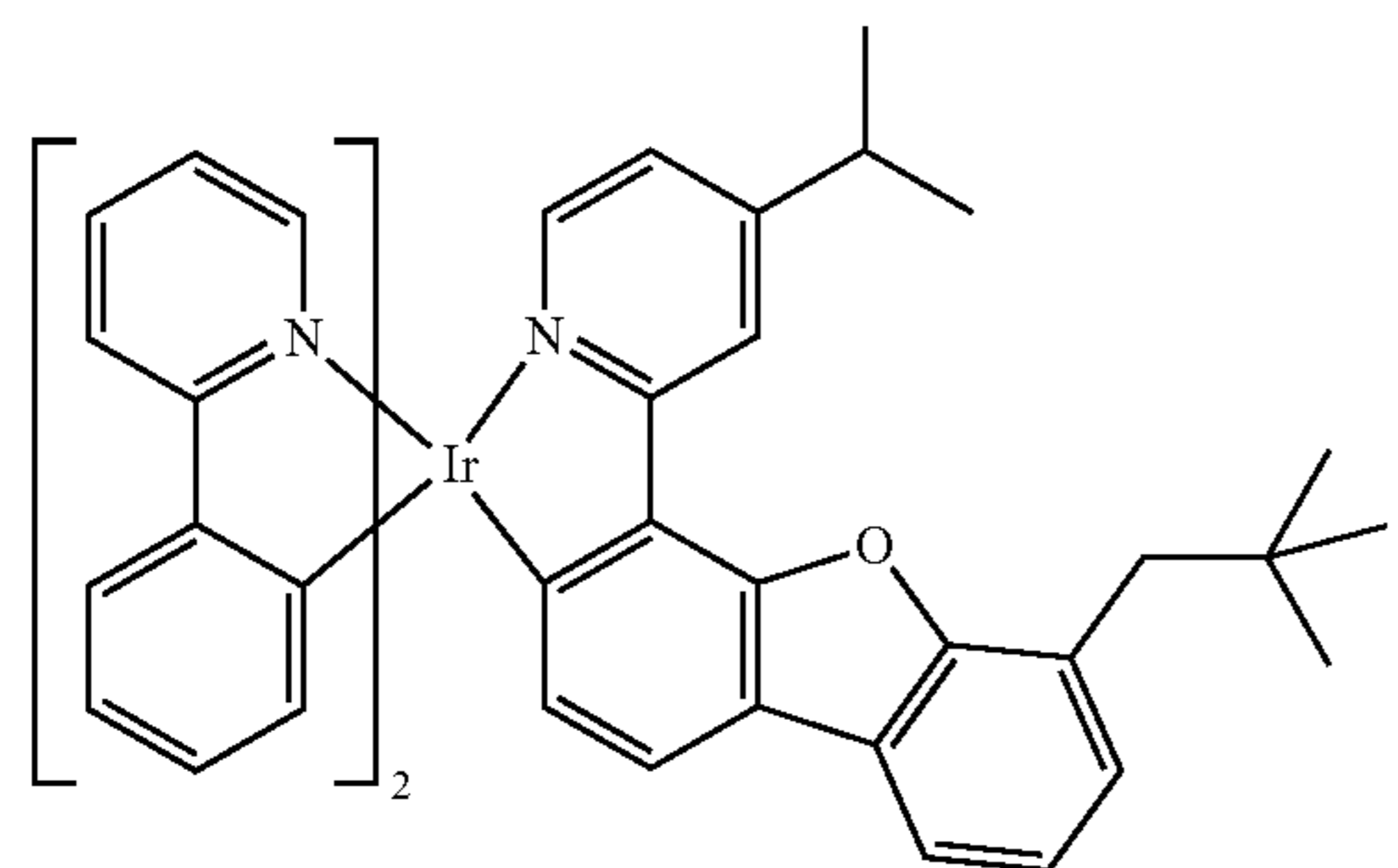
Compound 38
