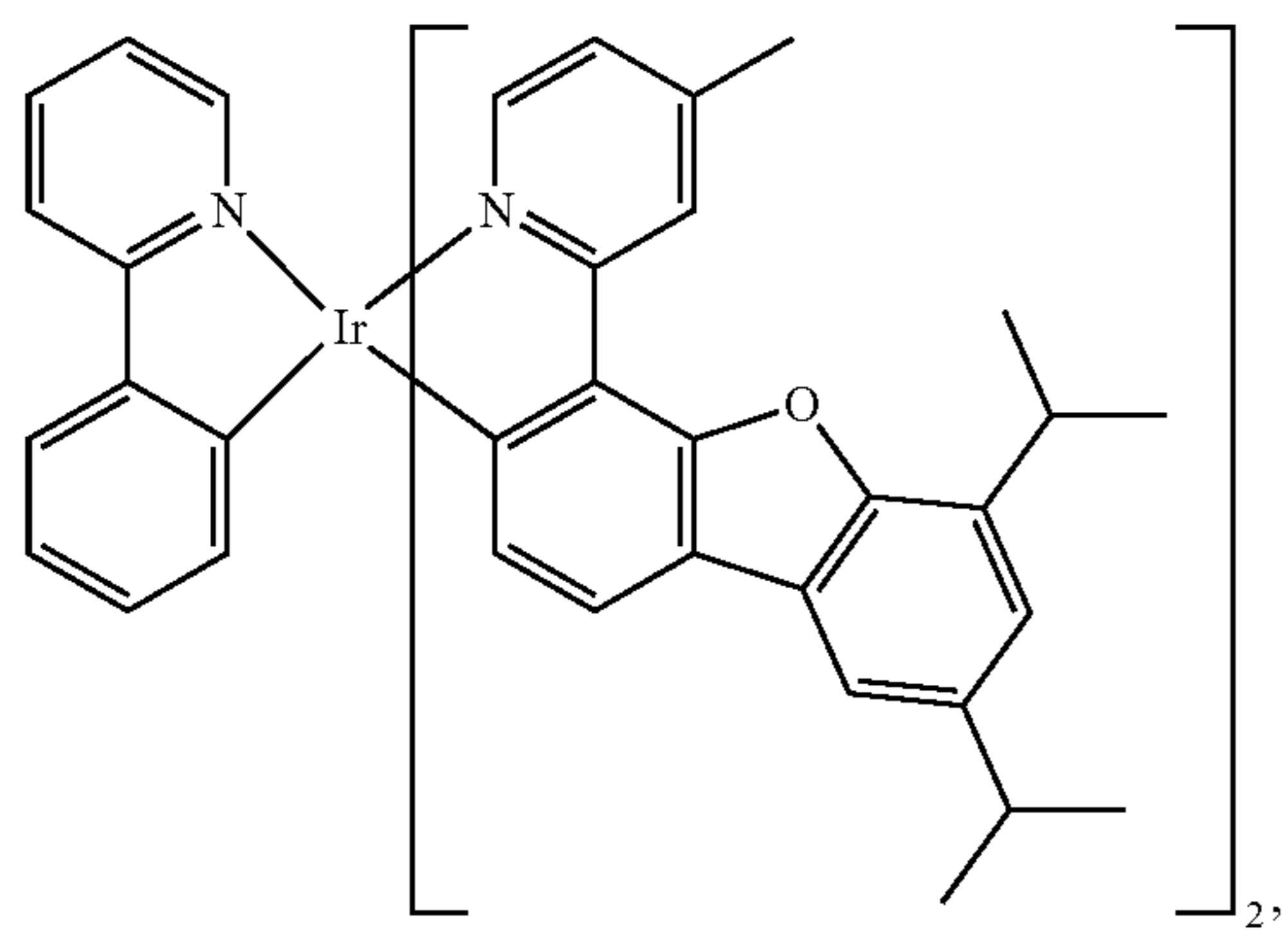
Compound 31
