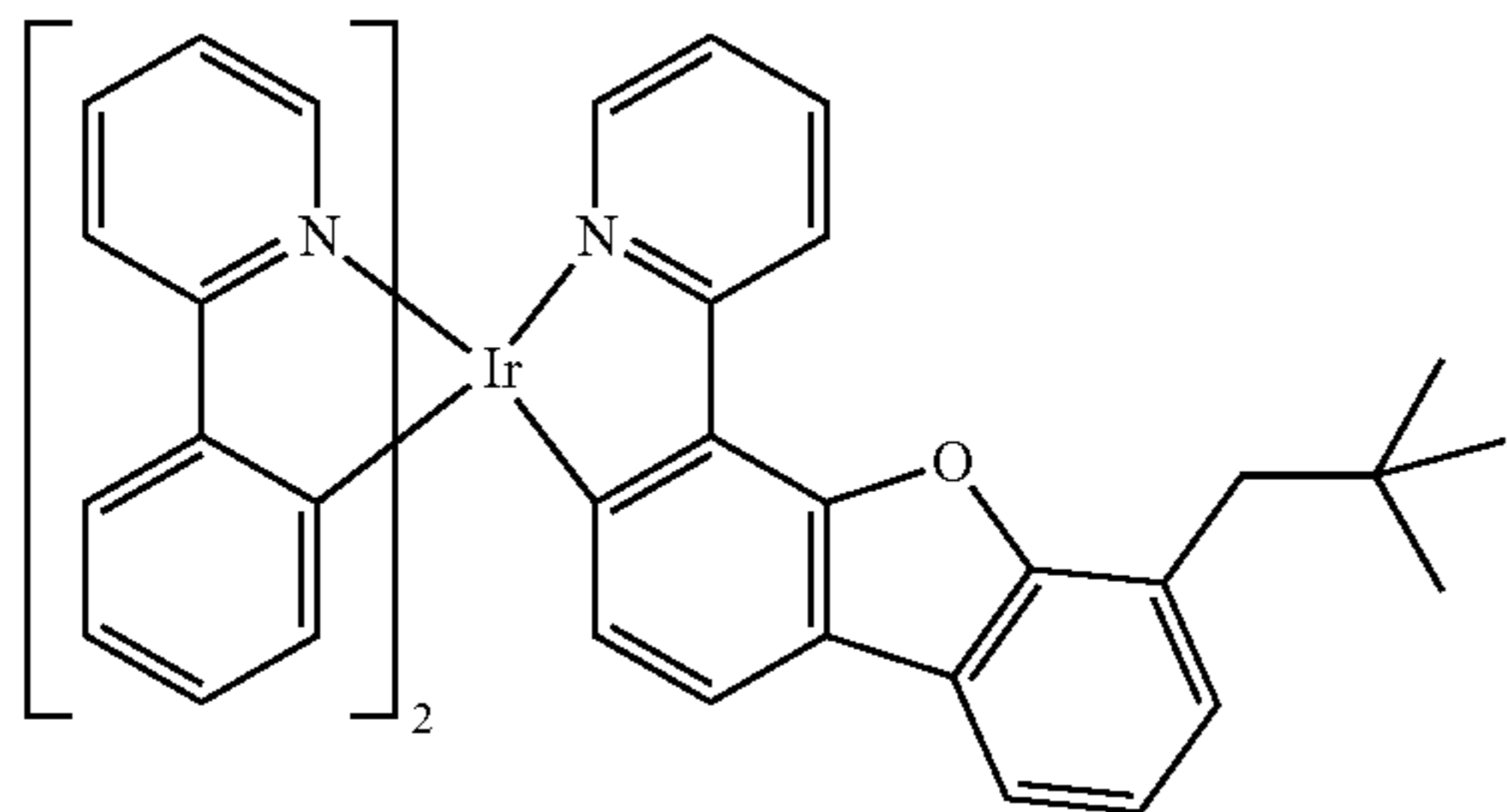
Compound 38
