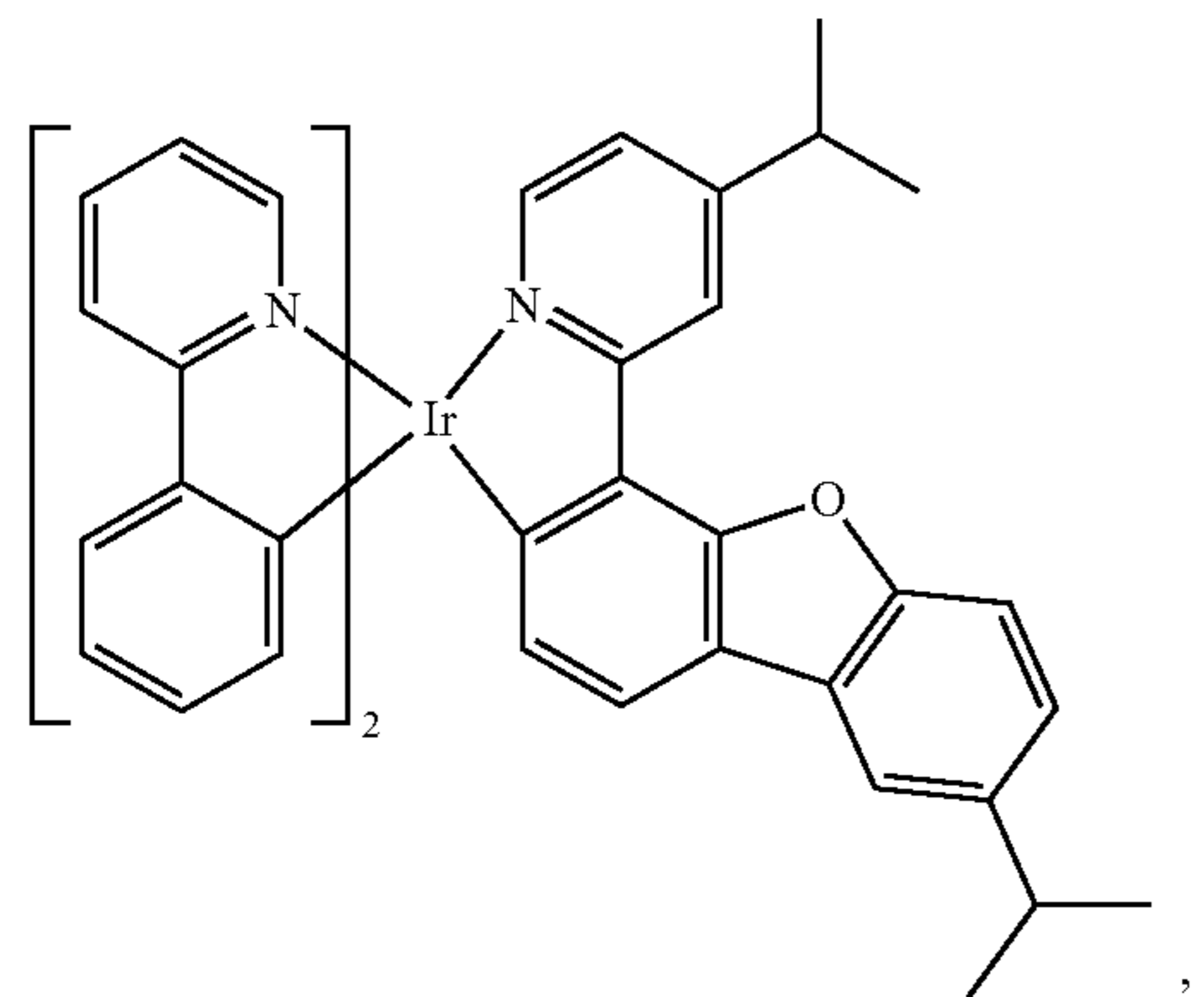
Compound 17
