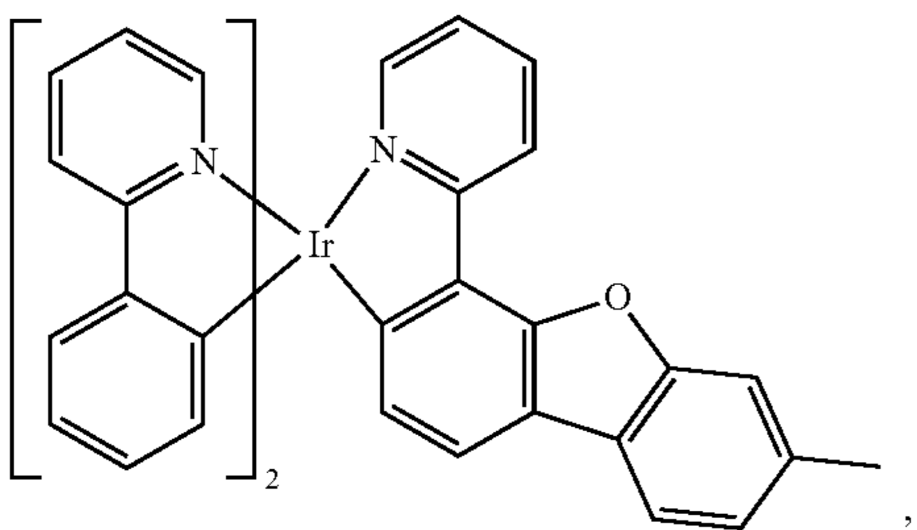
Compound 15
