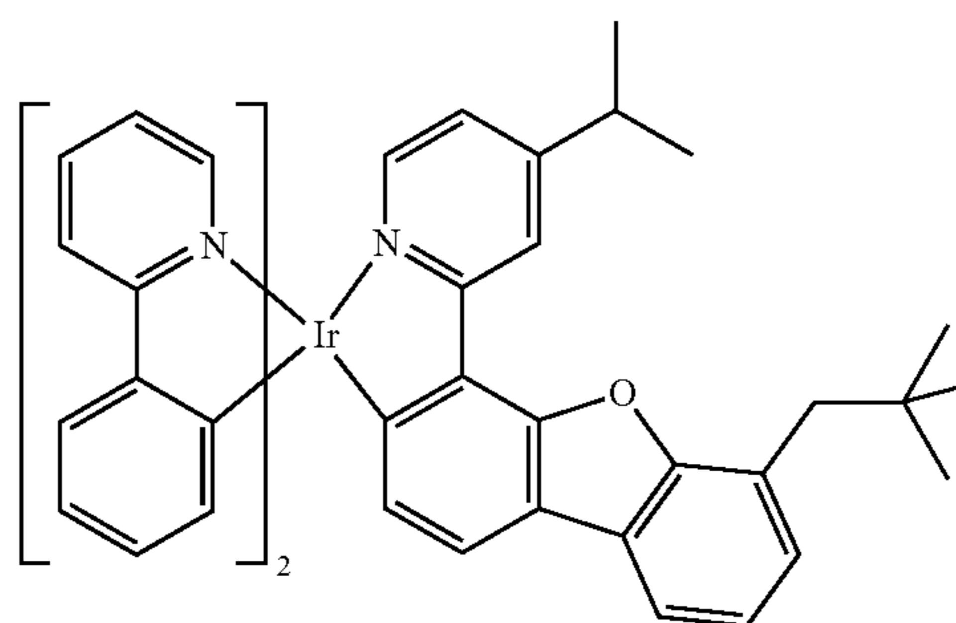
Compound 38
