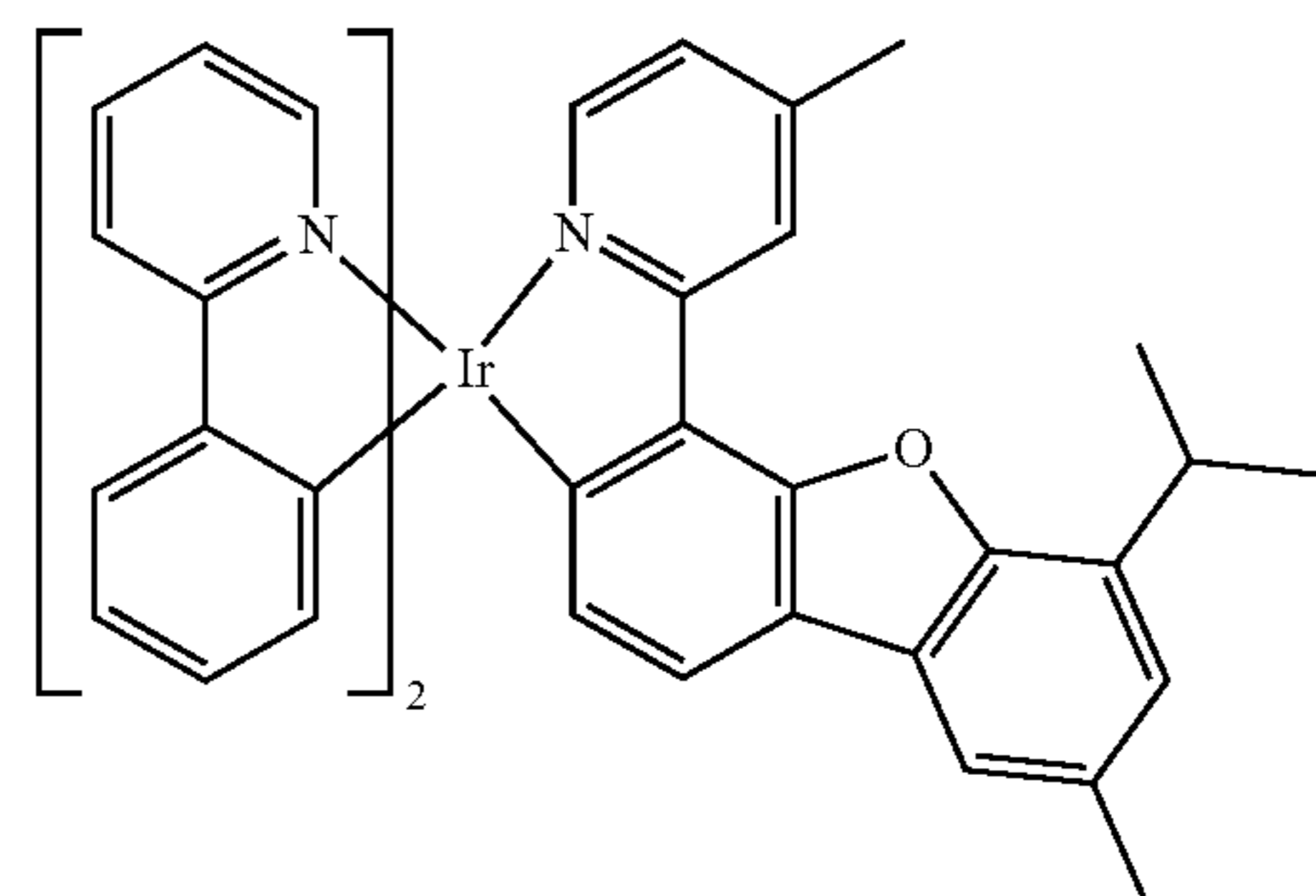
Compound 34
