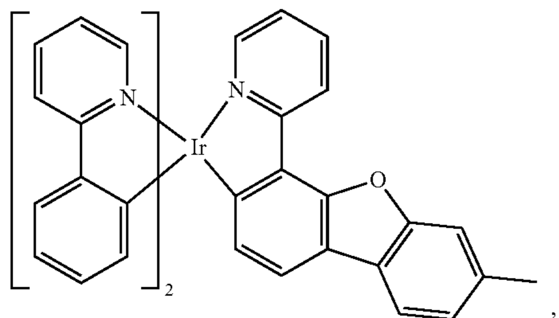
Compound 15
