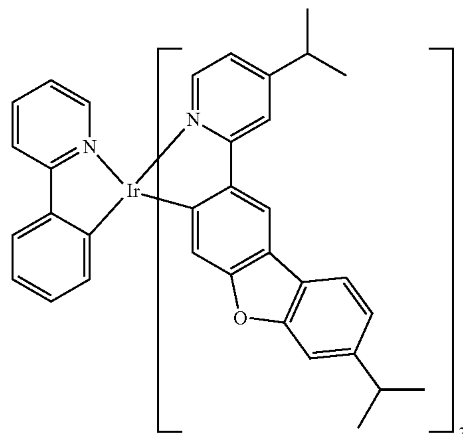
Compound 61
