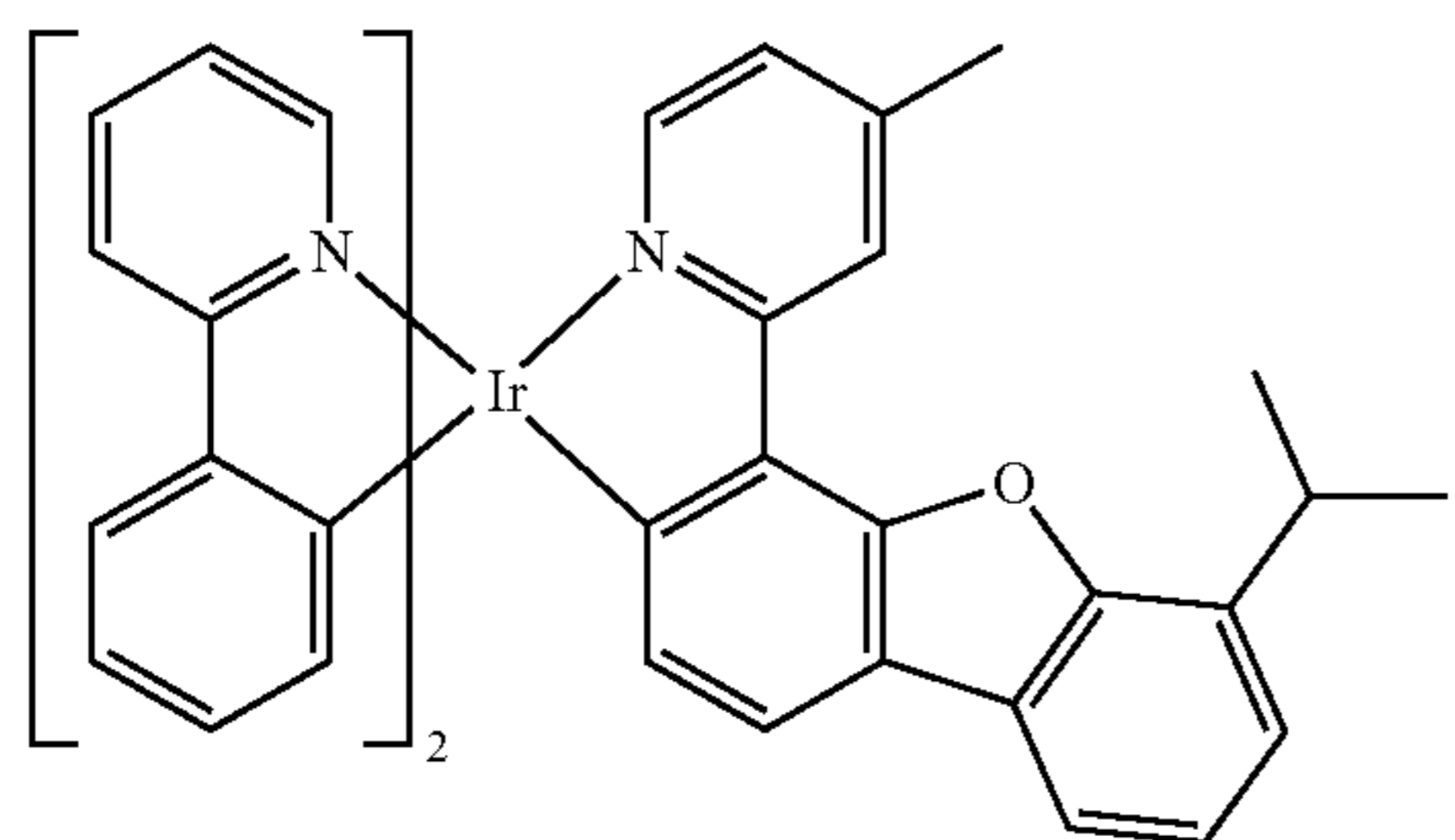
Compound 6
