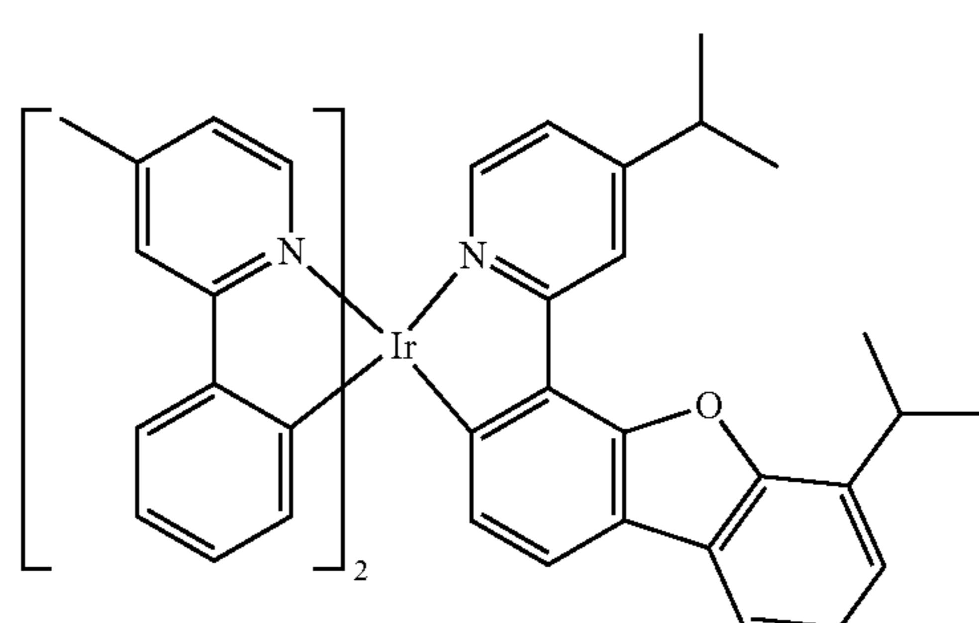
Compound 52
