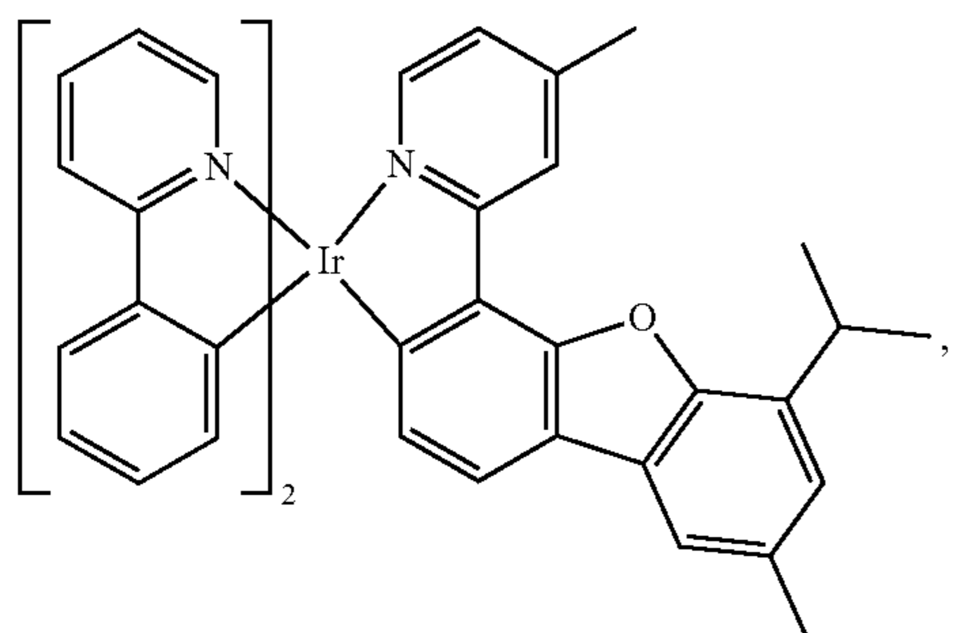
Compound 34
