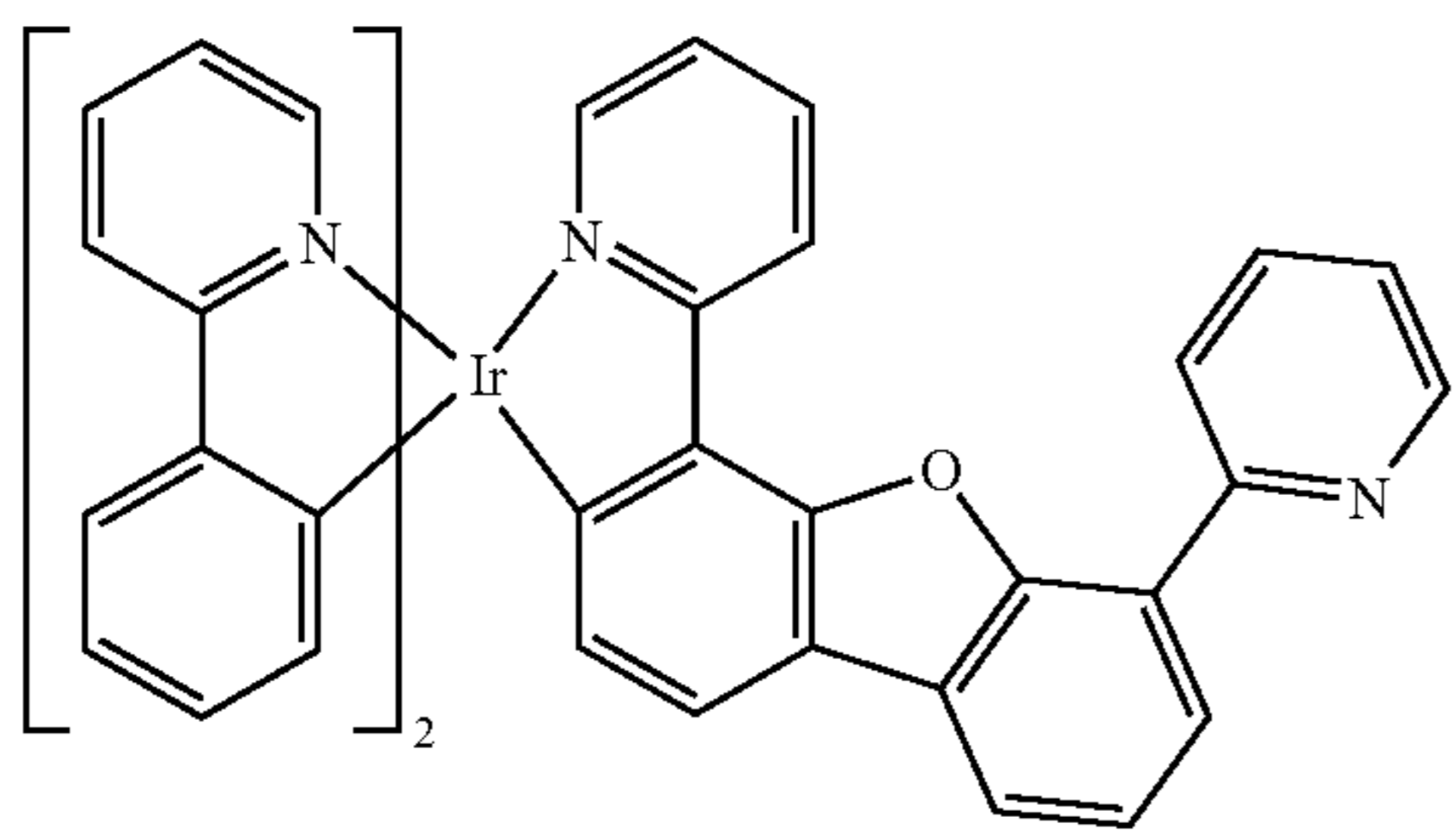
Compound 12
