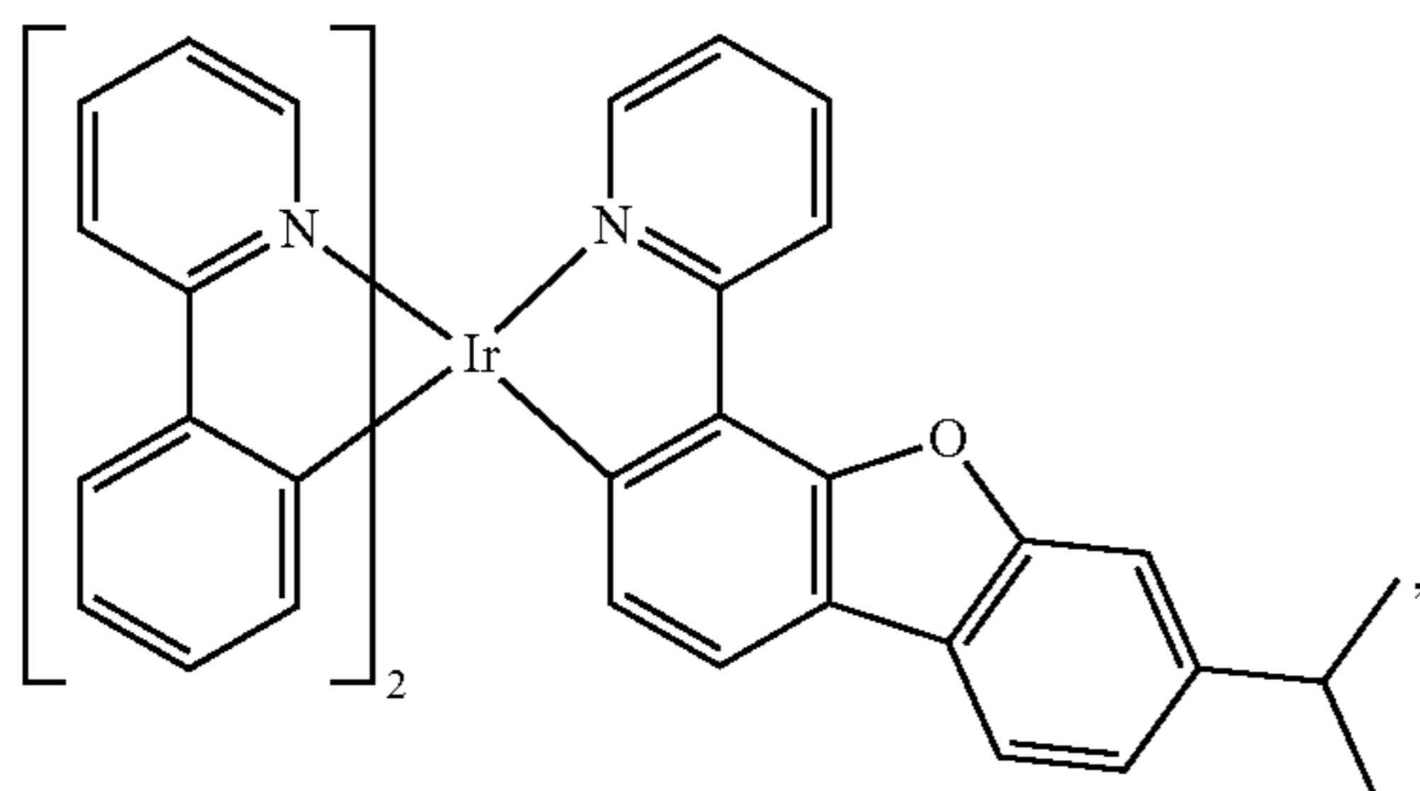
Compound 15
