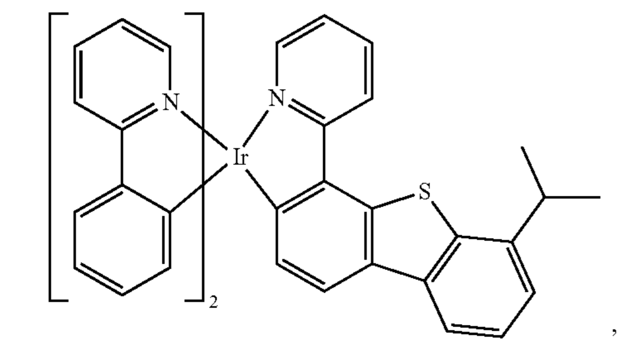
Compound 41
