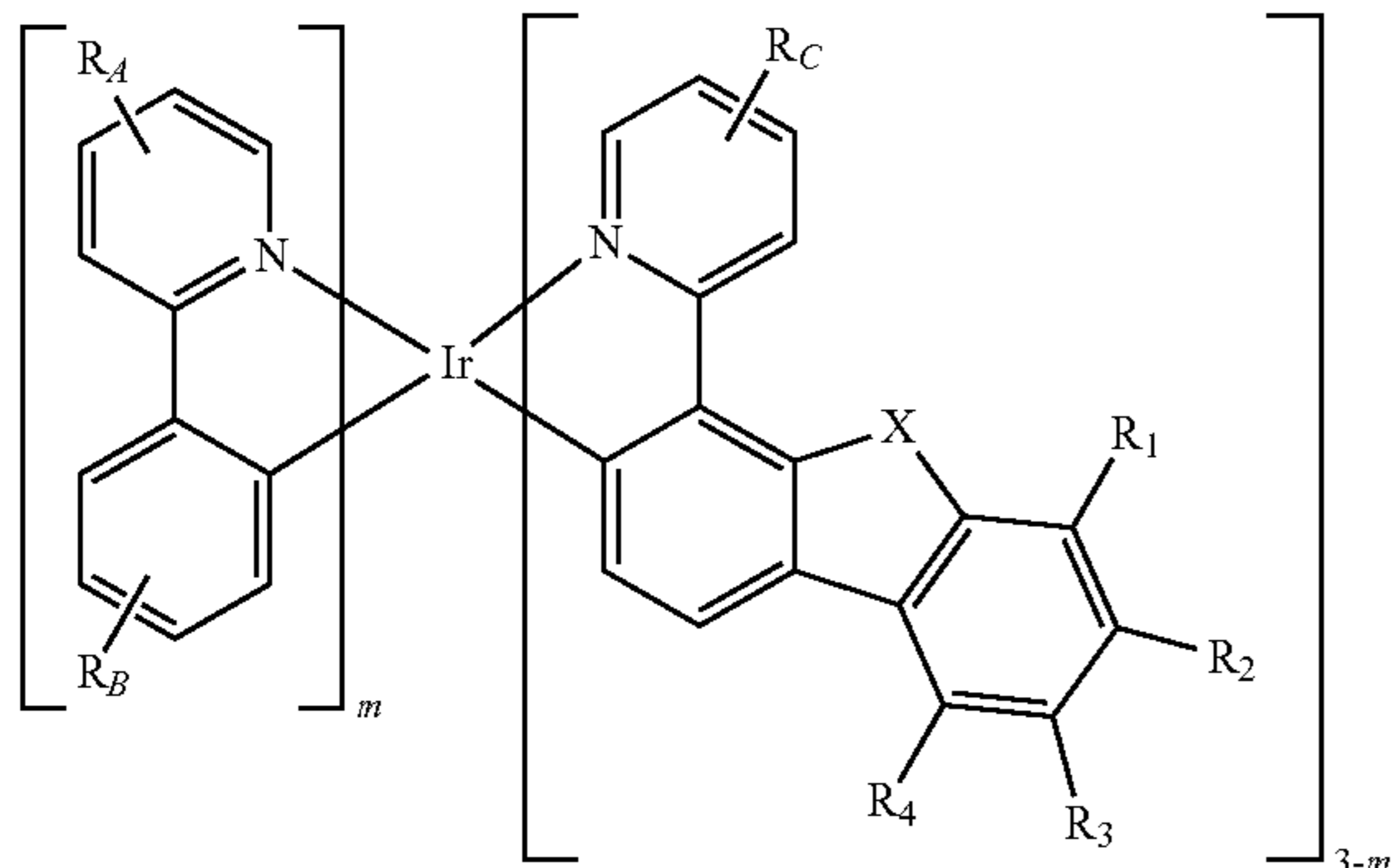
Formula II.
