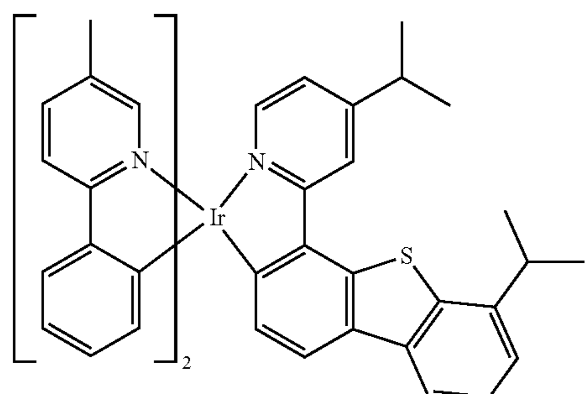
Compound 50
