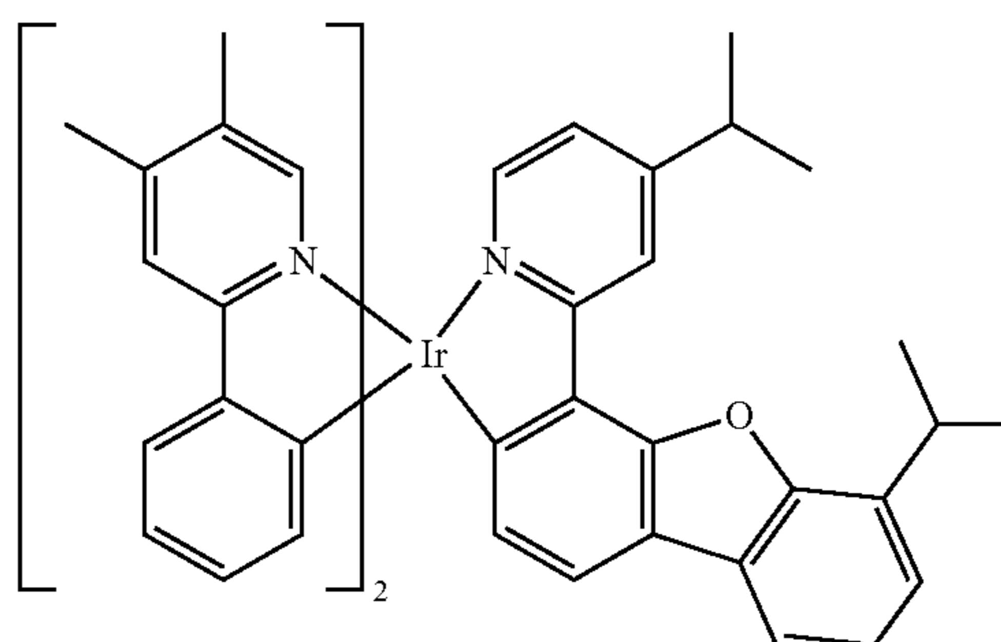
and Compound 54
