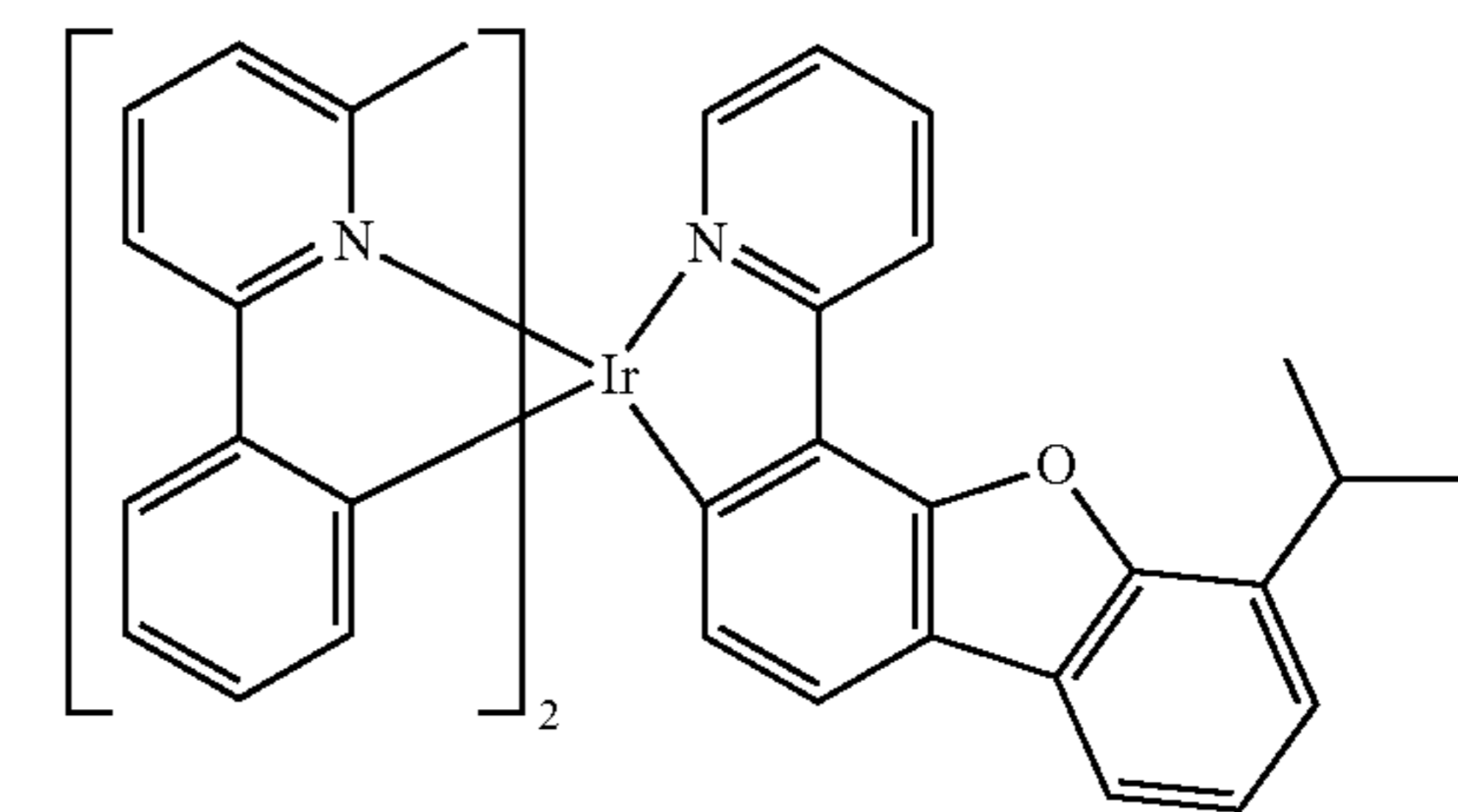
Compound 47
