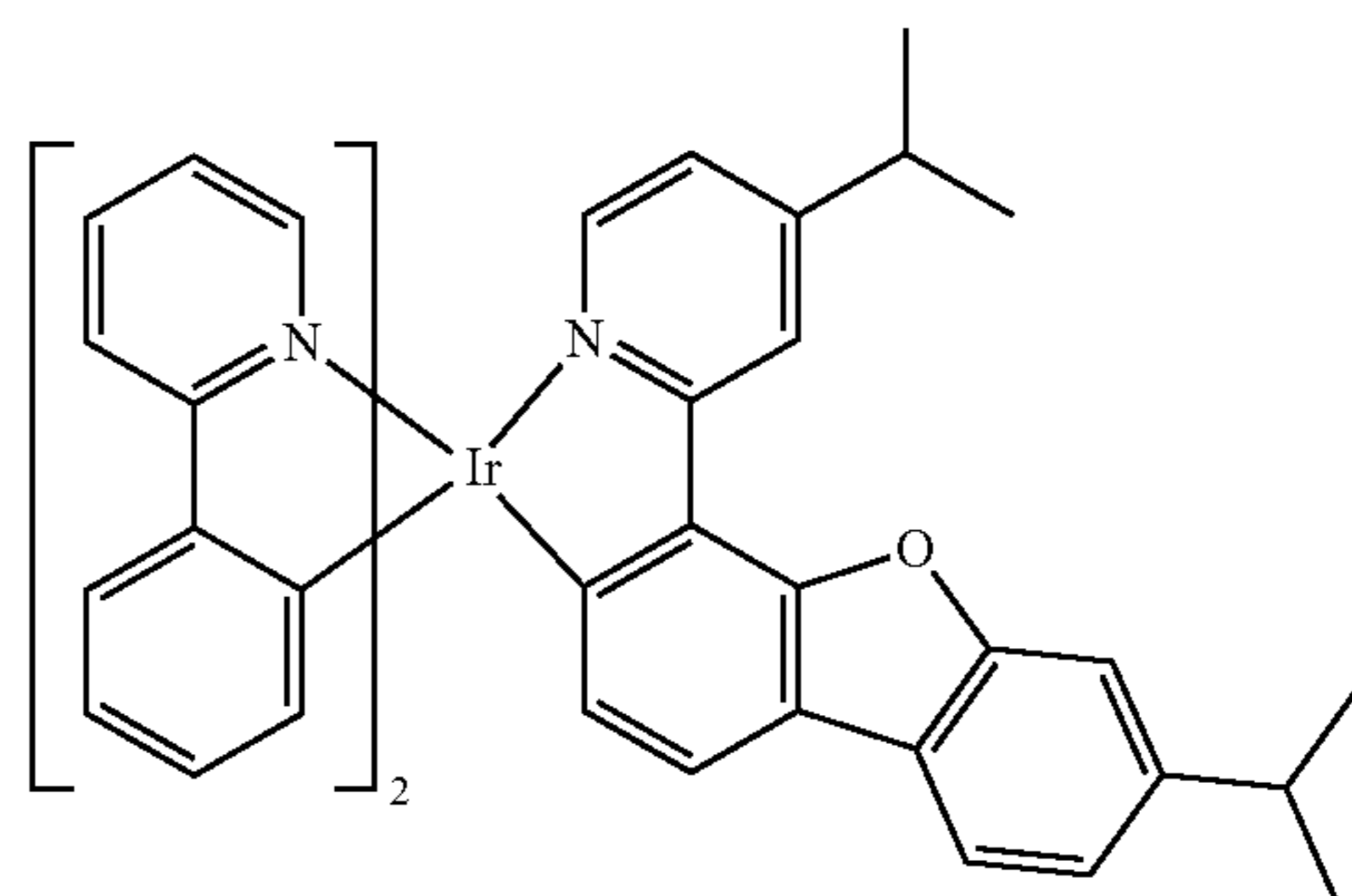
Compound 17
