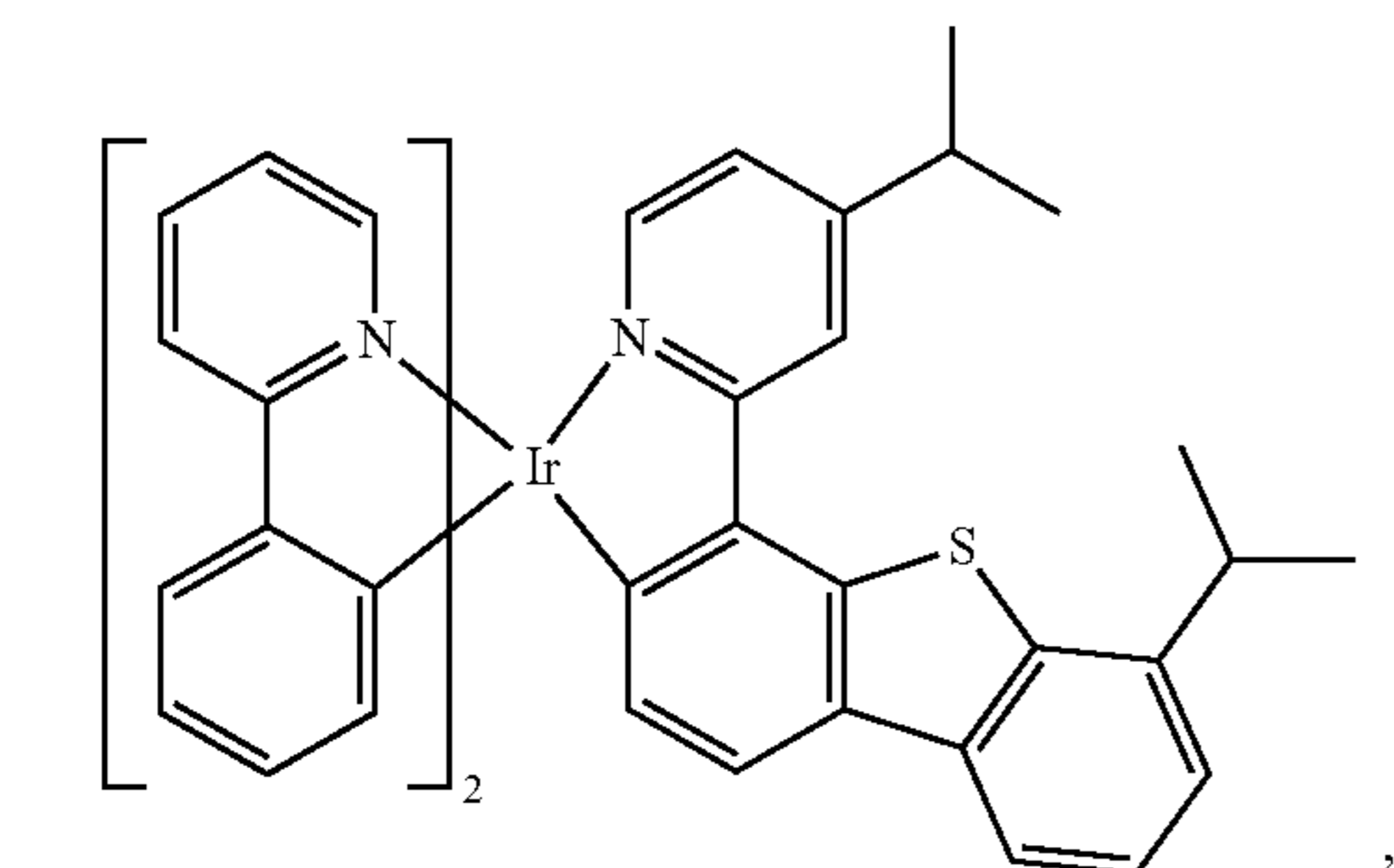
Compound 42
