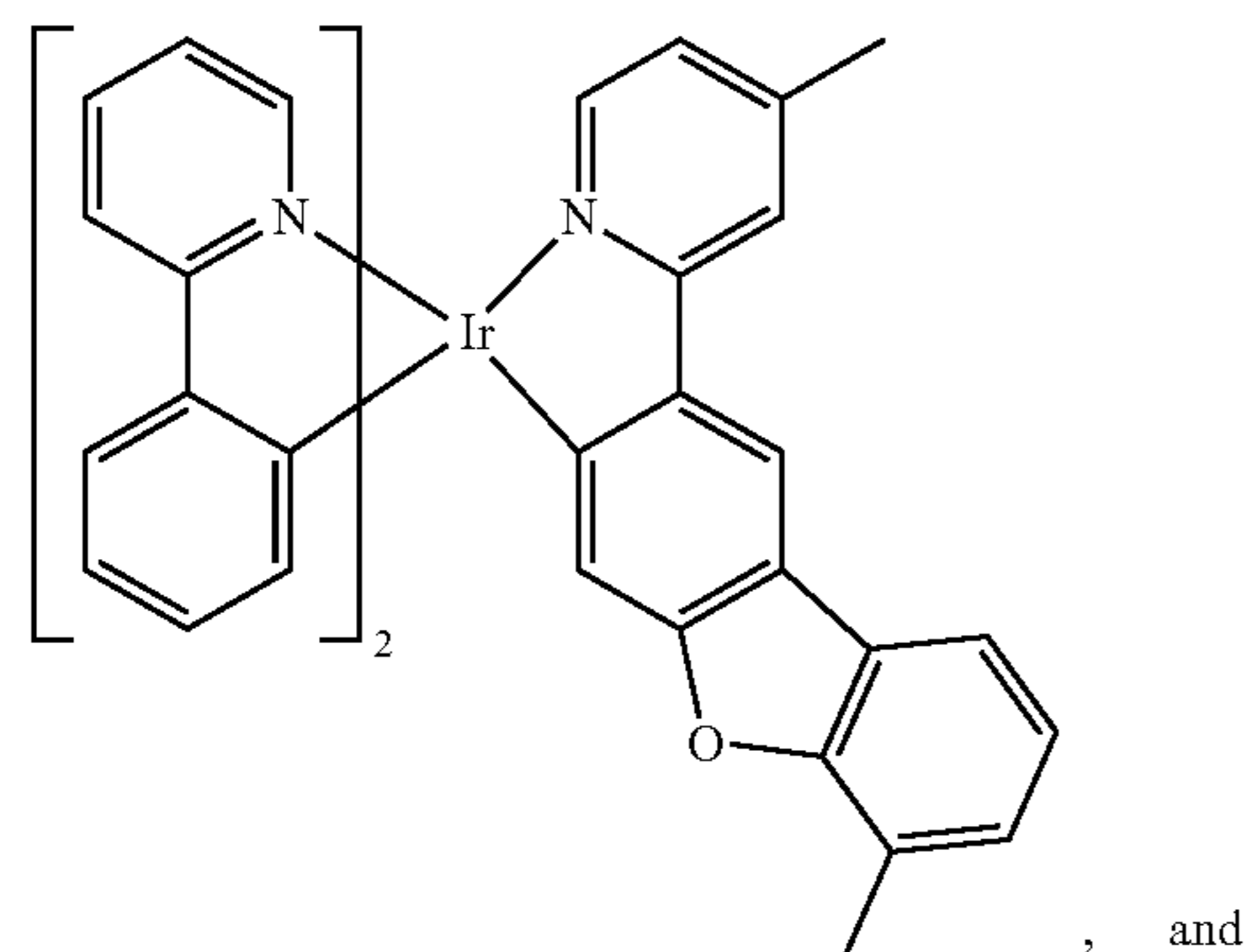
Compound 62
