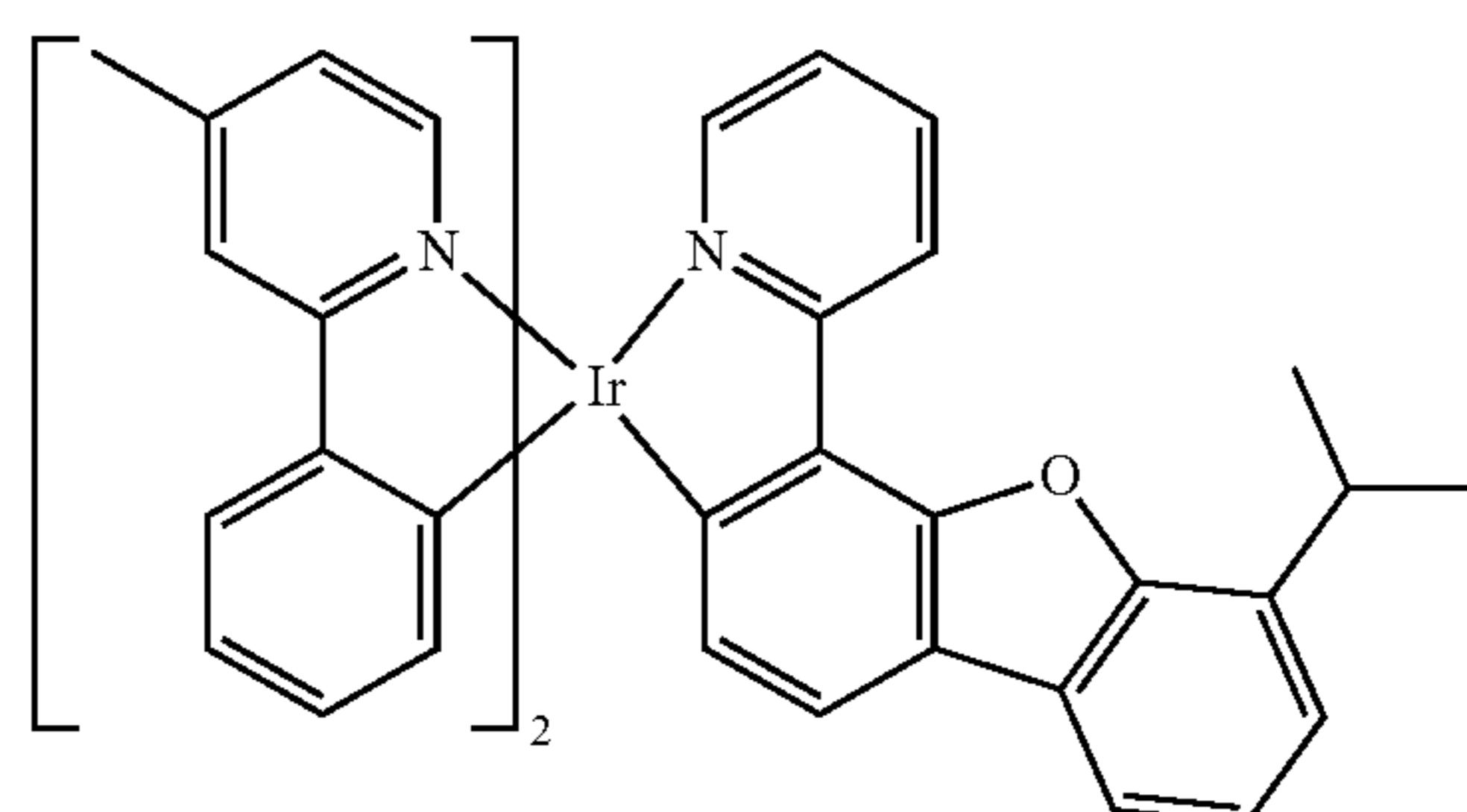
Compound 51
