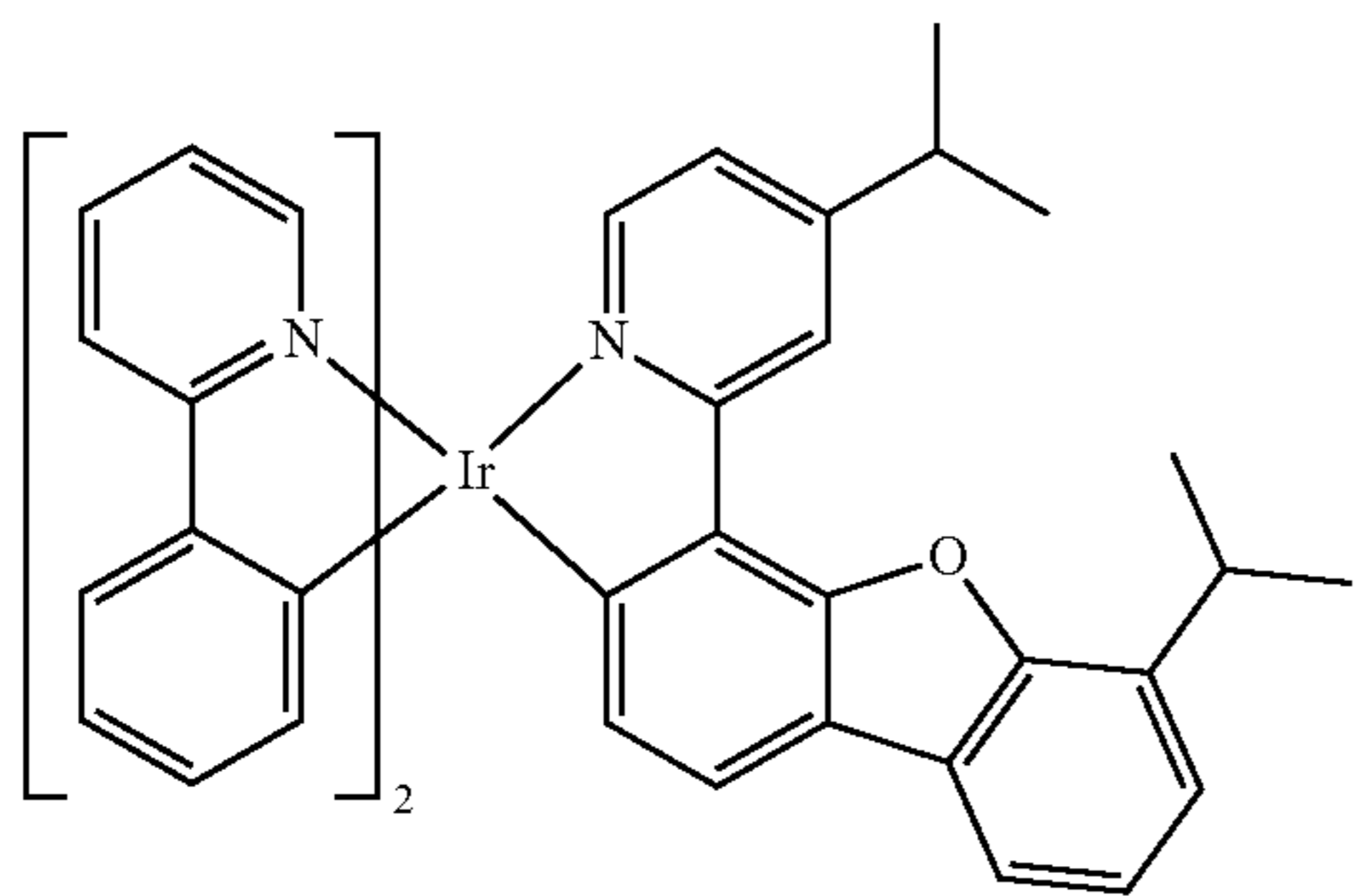
Compound 5
