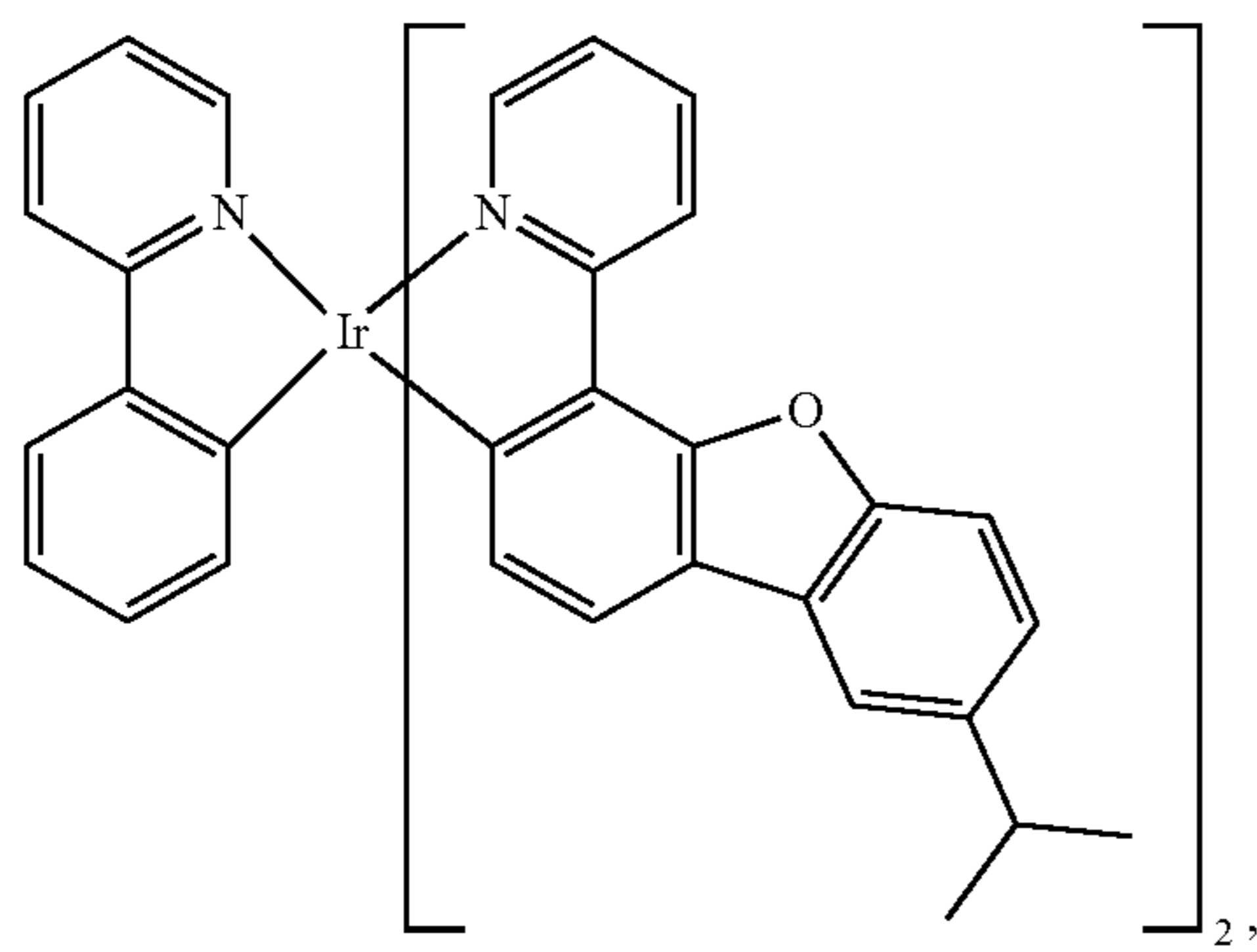
Compound 25
