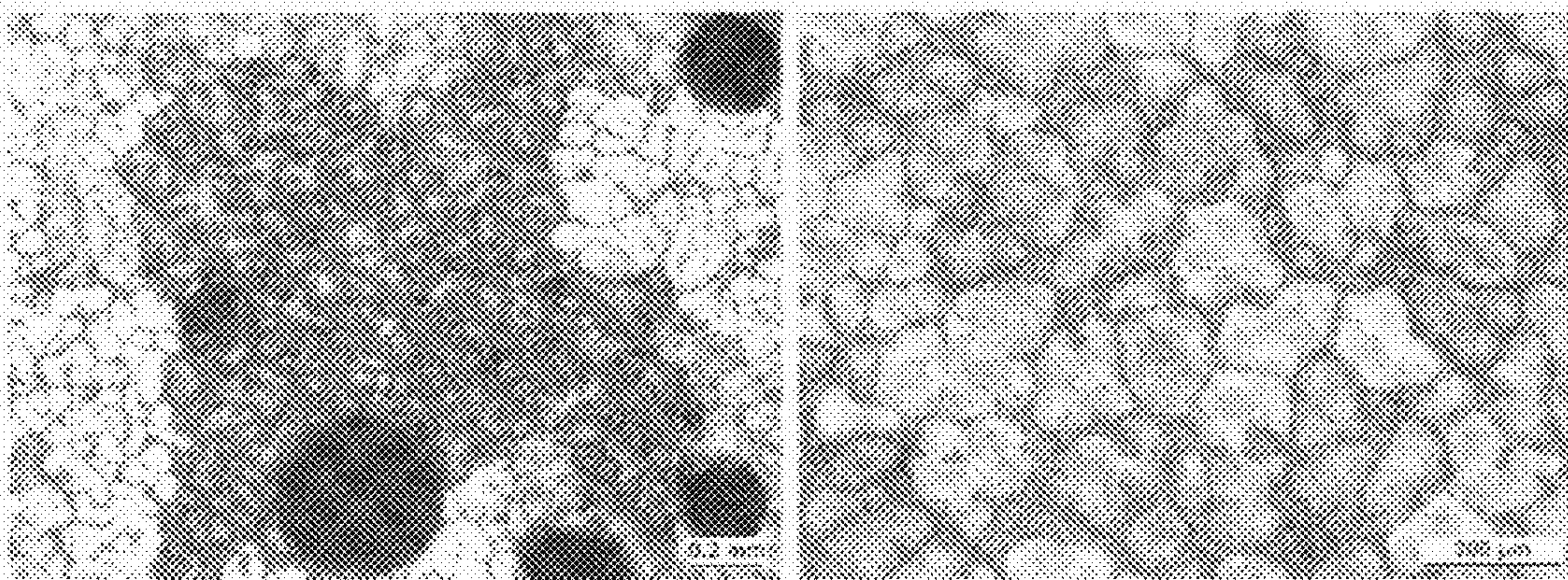
Figure 5a: Alteration from a coarse grained dendritic structure to a fine grained dendritic 'rosette' structure. Images obtained from cooling curve experiments
