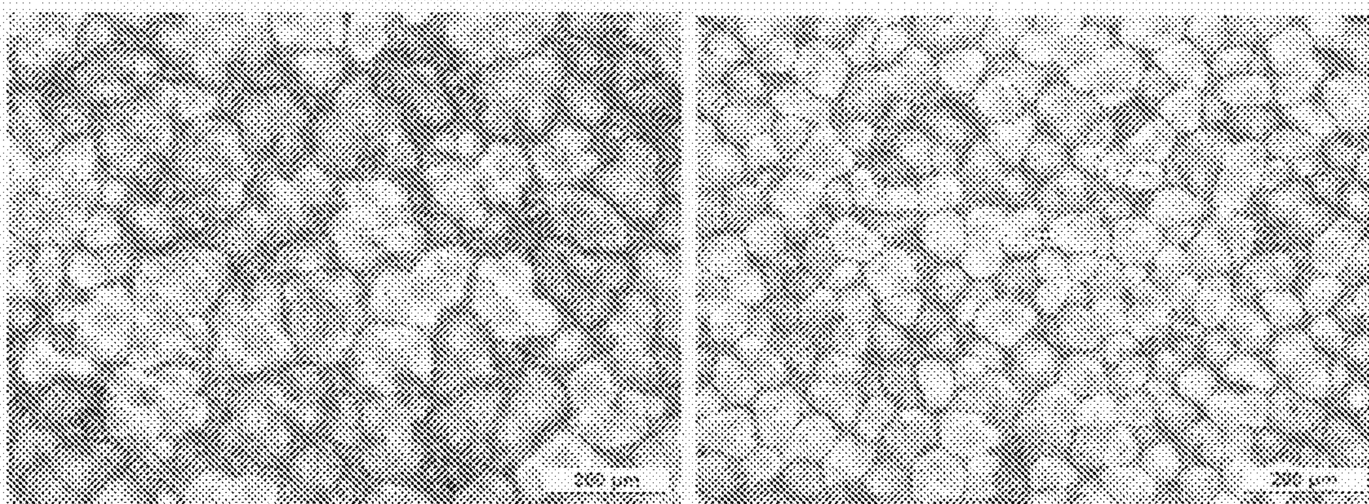
Figure 5b: Alteration from fine grained dendritic structure to a cellular fine grained structure, images obtained from cooling curve experiments
