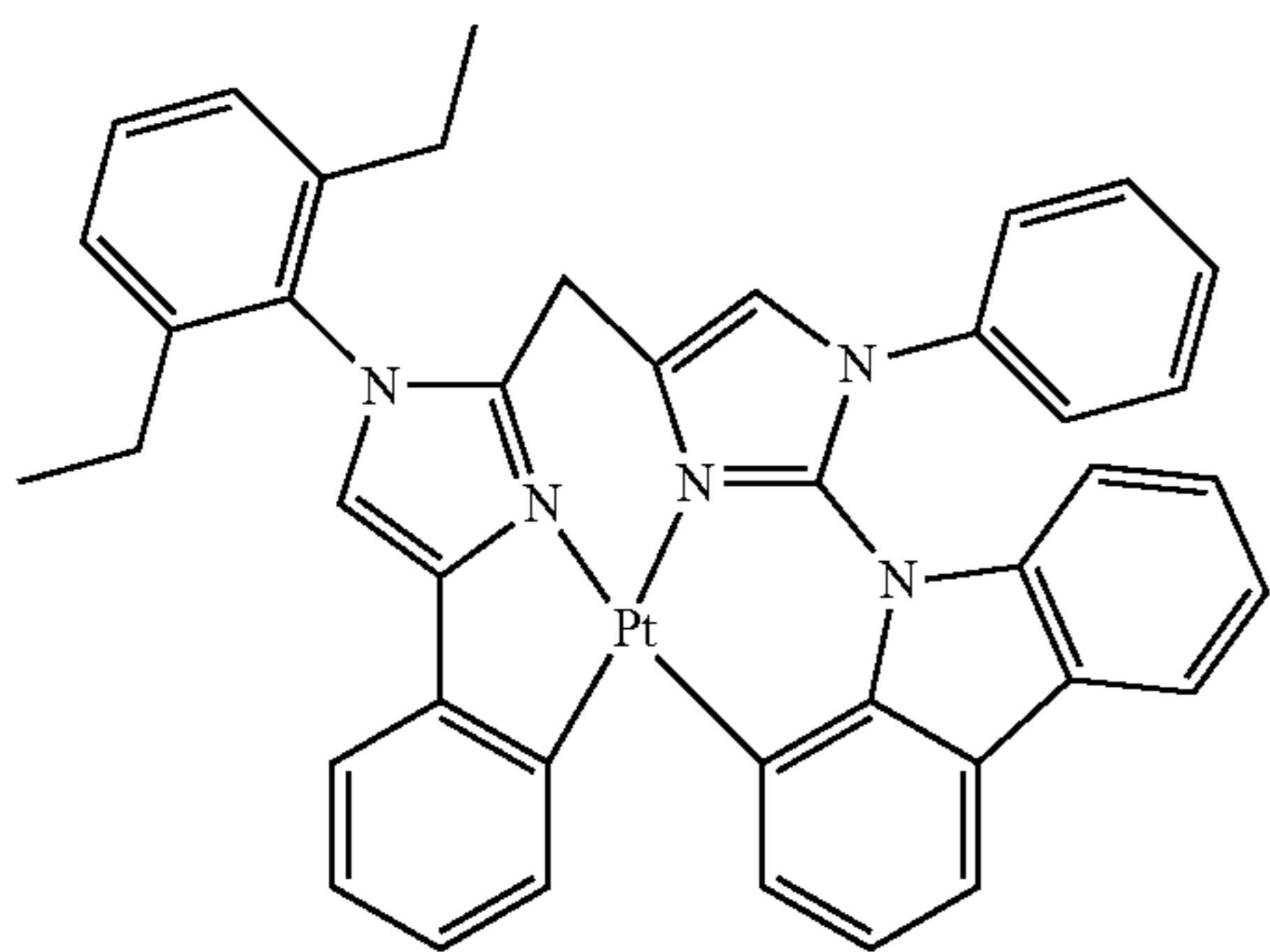
Compound 43
