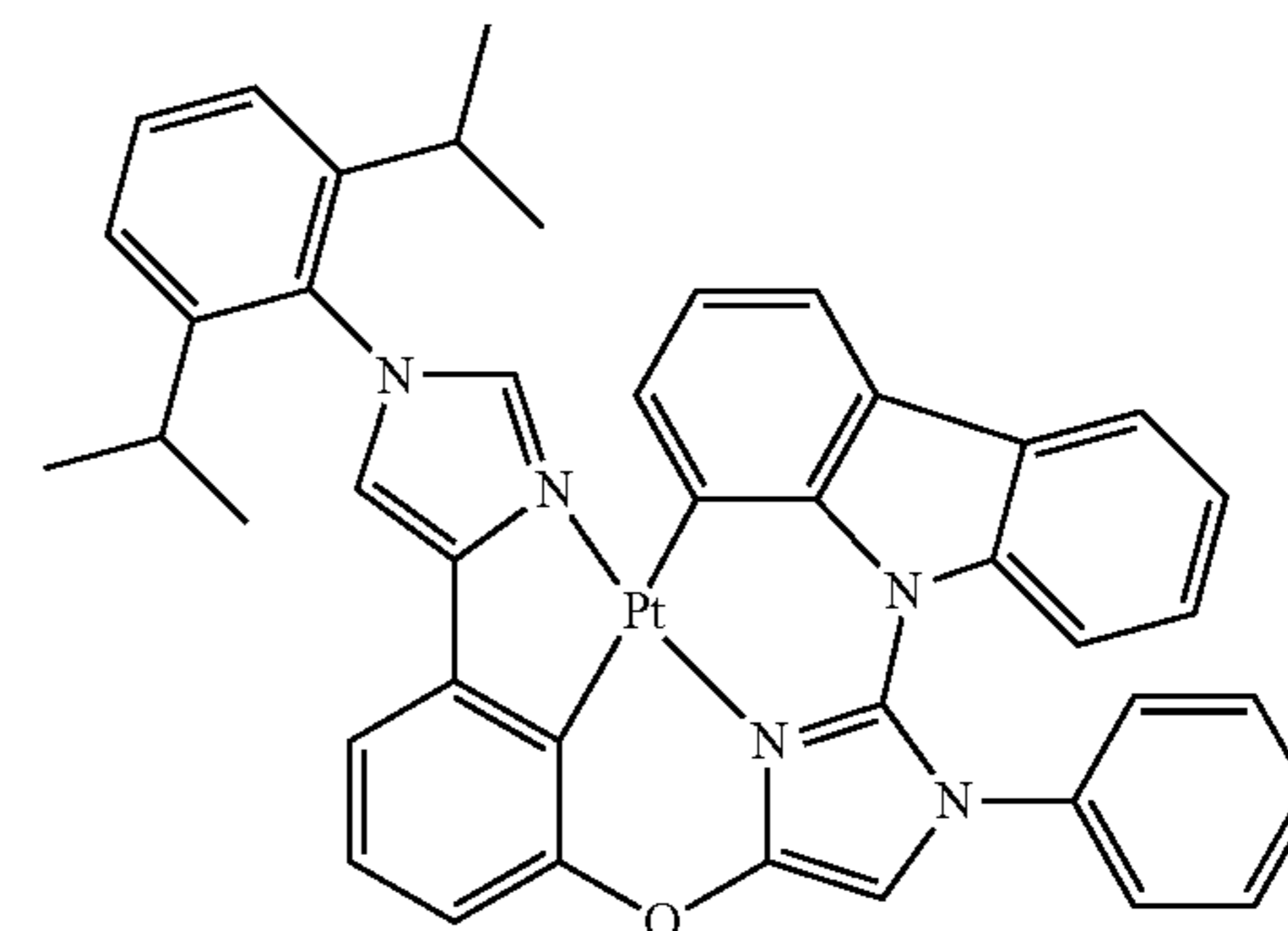
Compound 56
