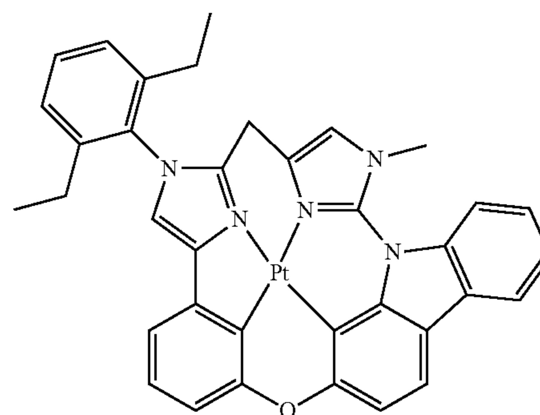
Compound 41
