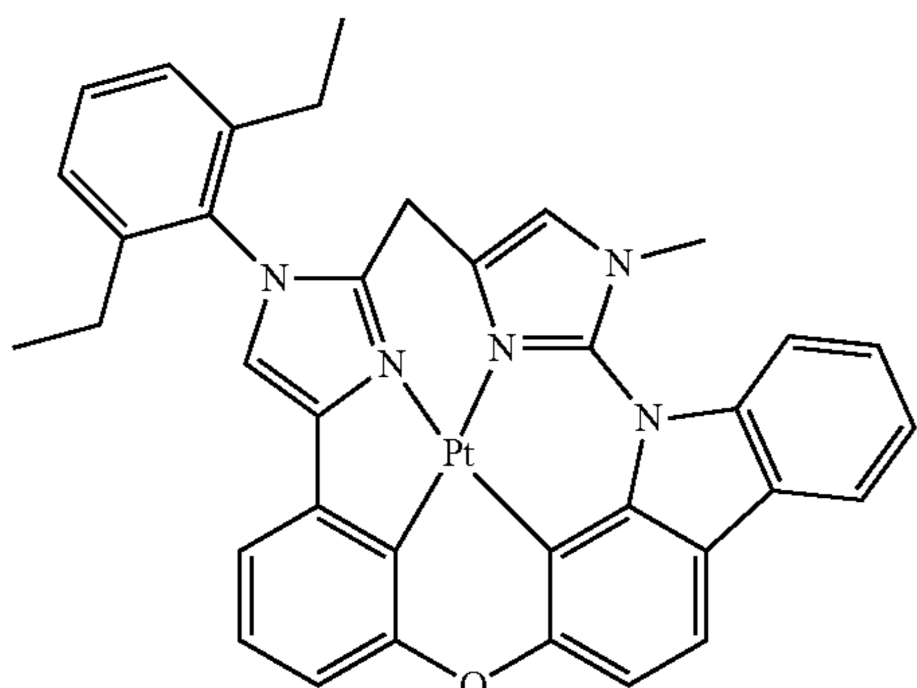
Compound 42
