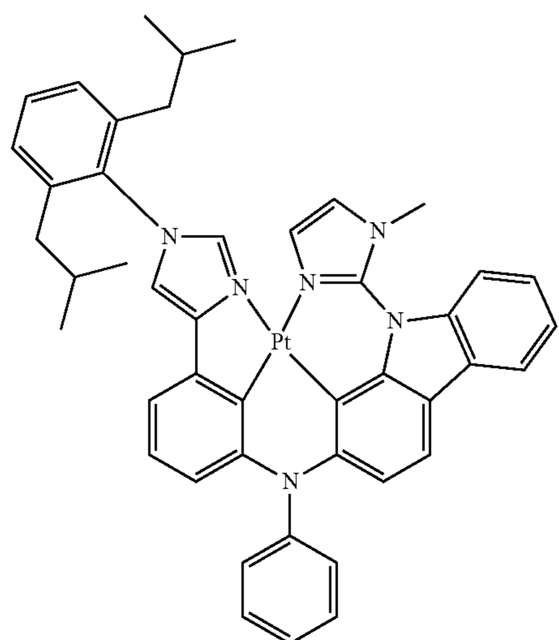
Compound 72
