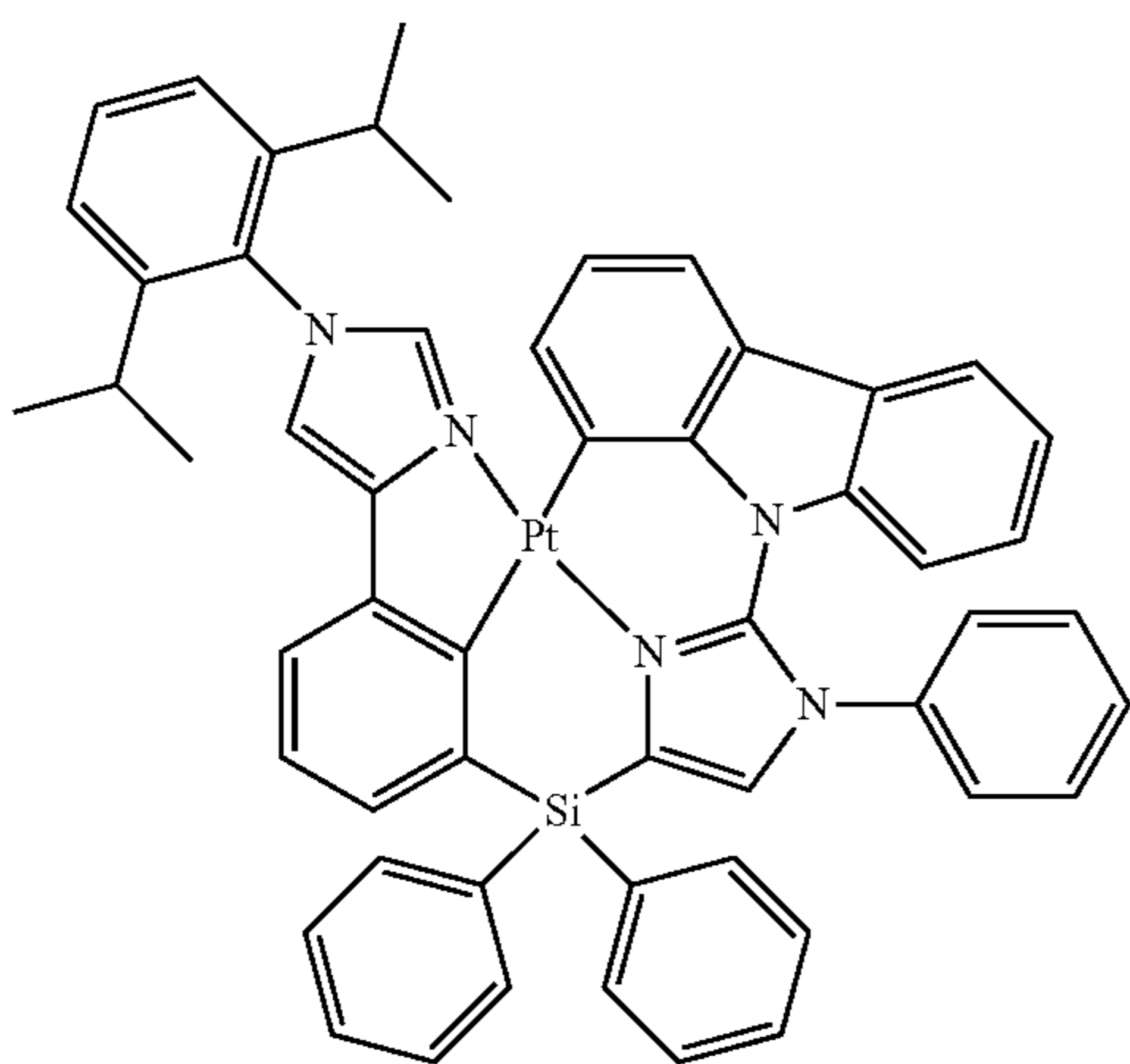
Compound 58
