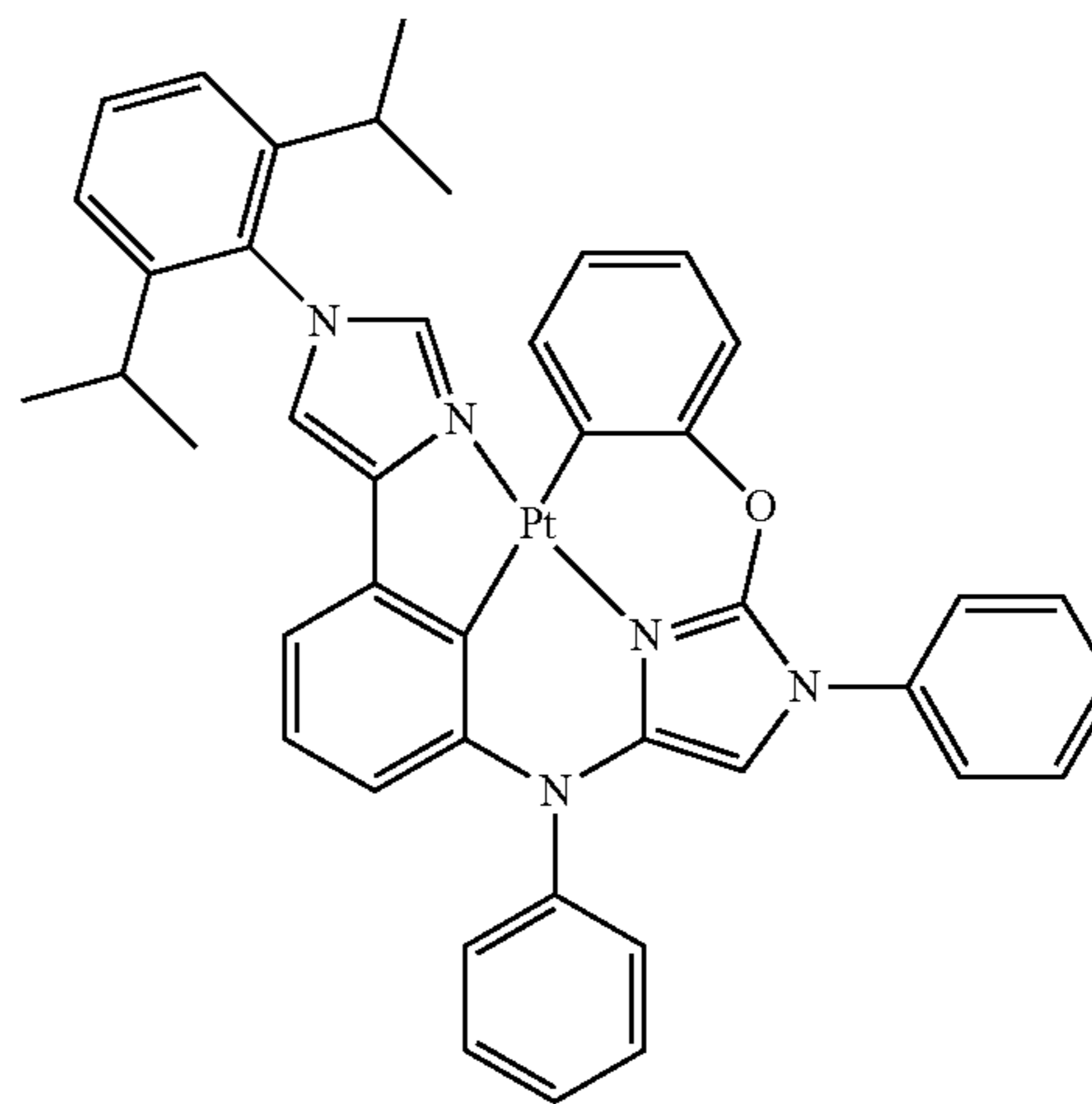
Compound 52
