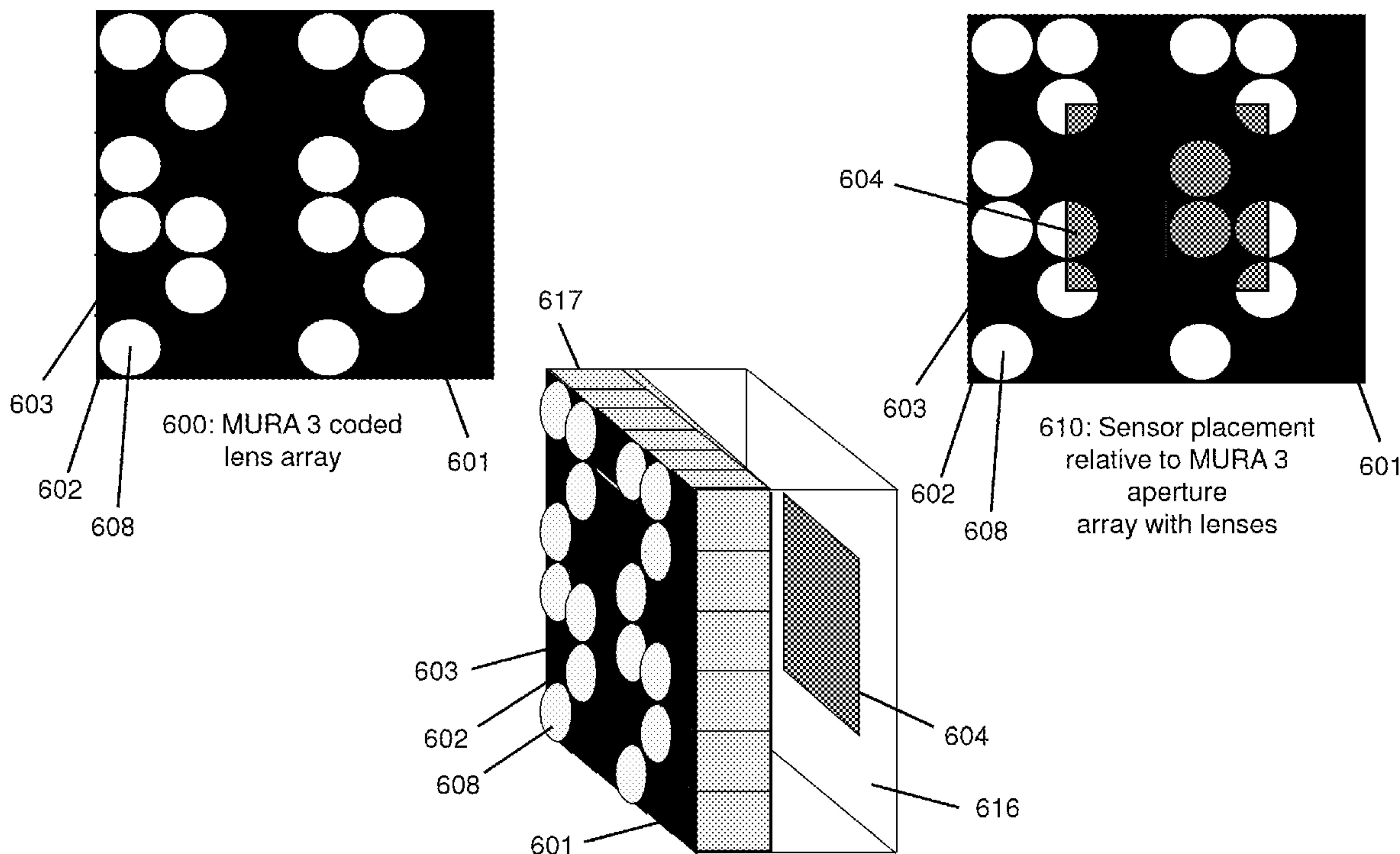
620: Orthographic view of MURA 3 aperture array with lenses, baffles and sensor (camera enclosure is transparent for illustration purposes)
