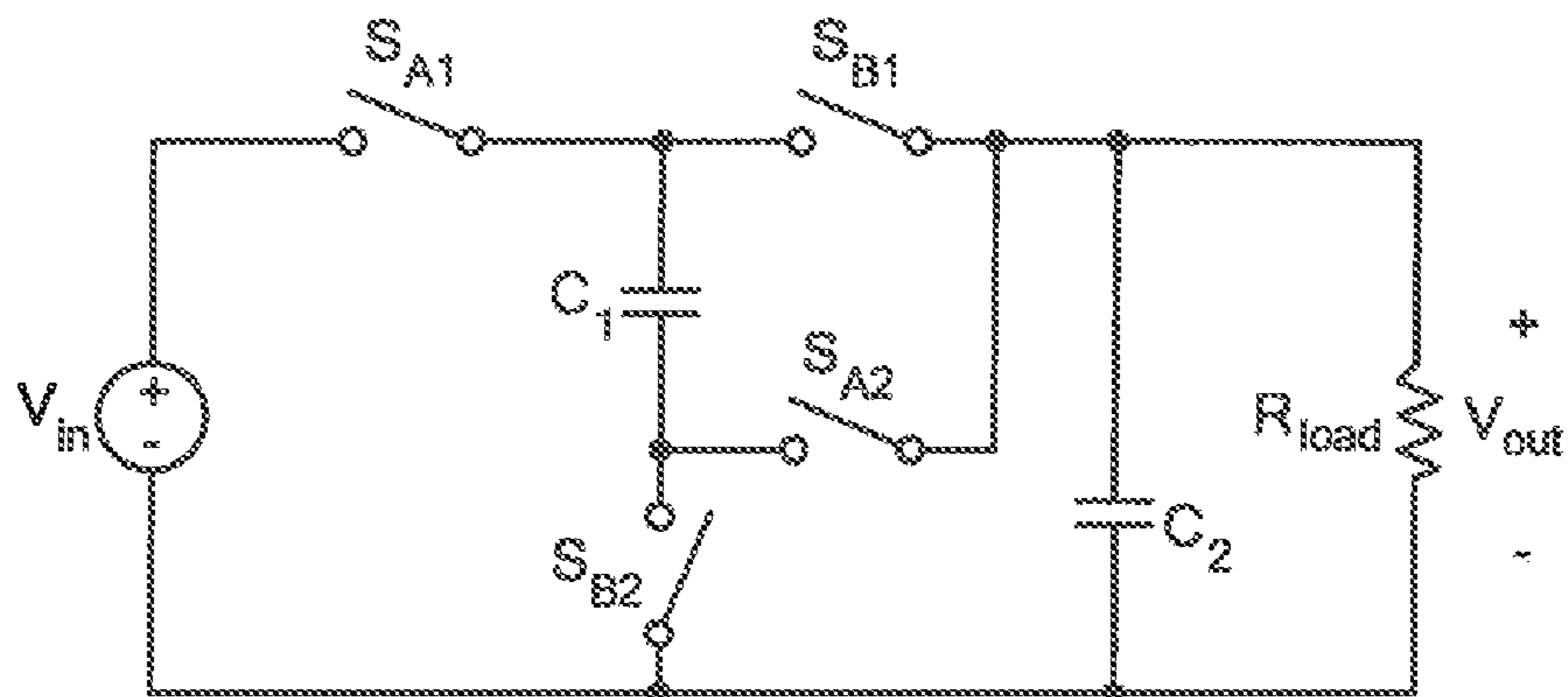
FIG. 1 PRIOR ART
