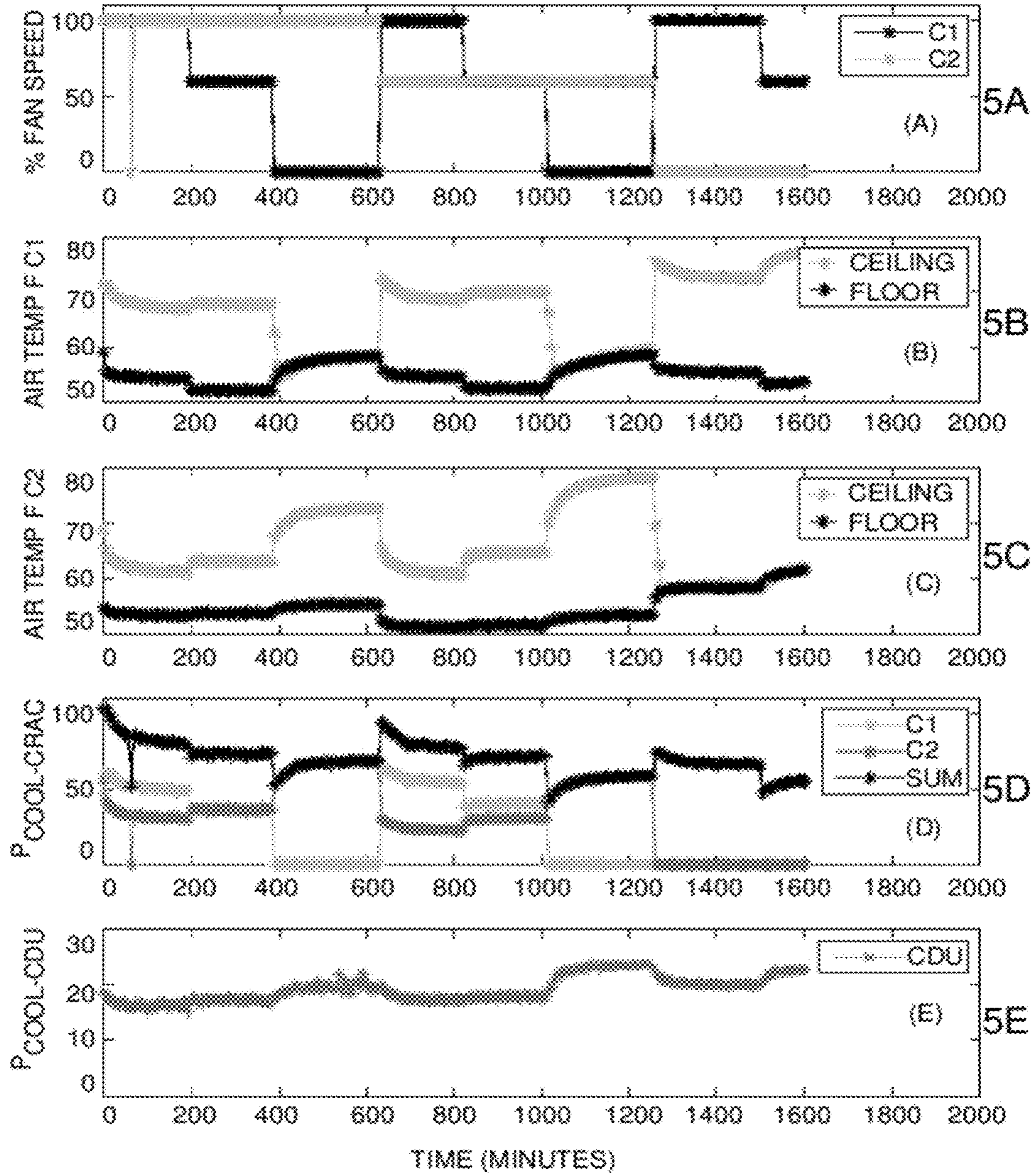
COOLING POWER MEASUREMENTS
