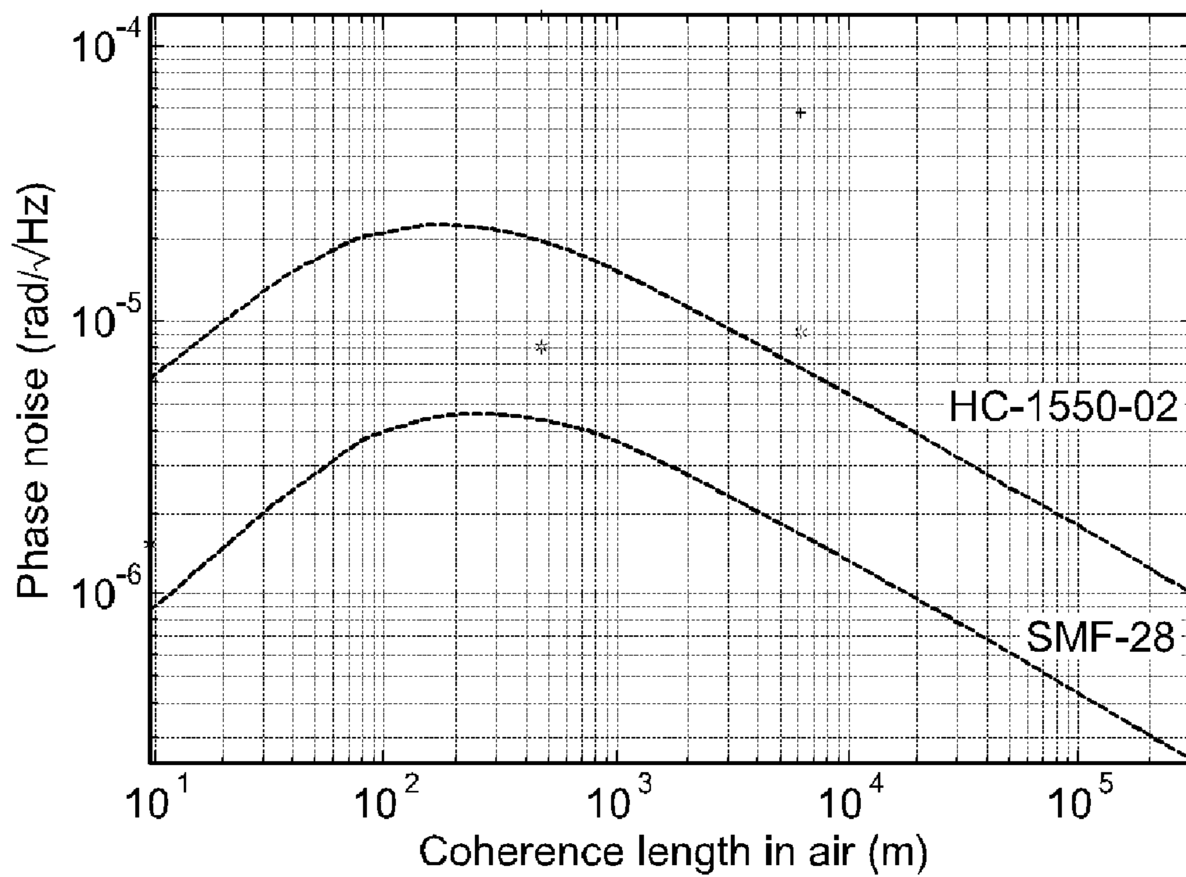
Experimental and predicted noise for air-core and solid-core FOGs
