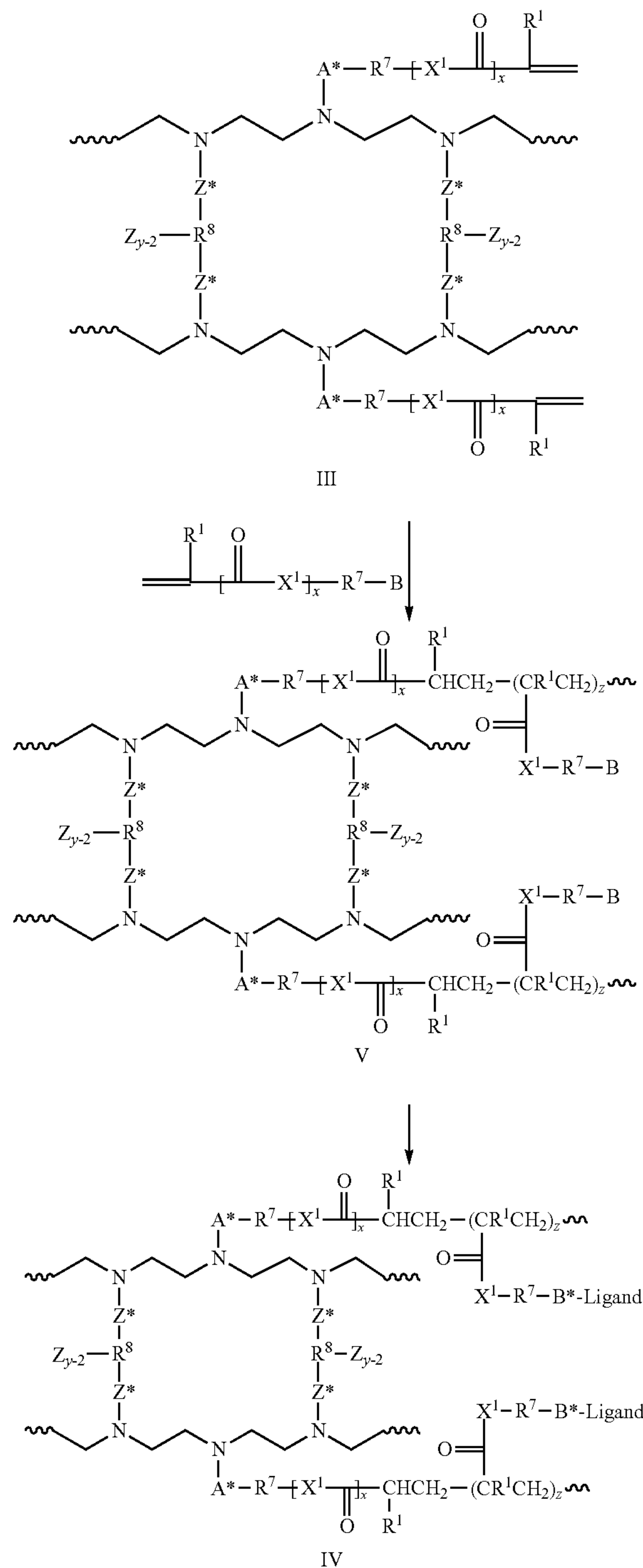
Scheme 2
