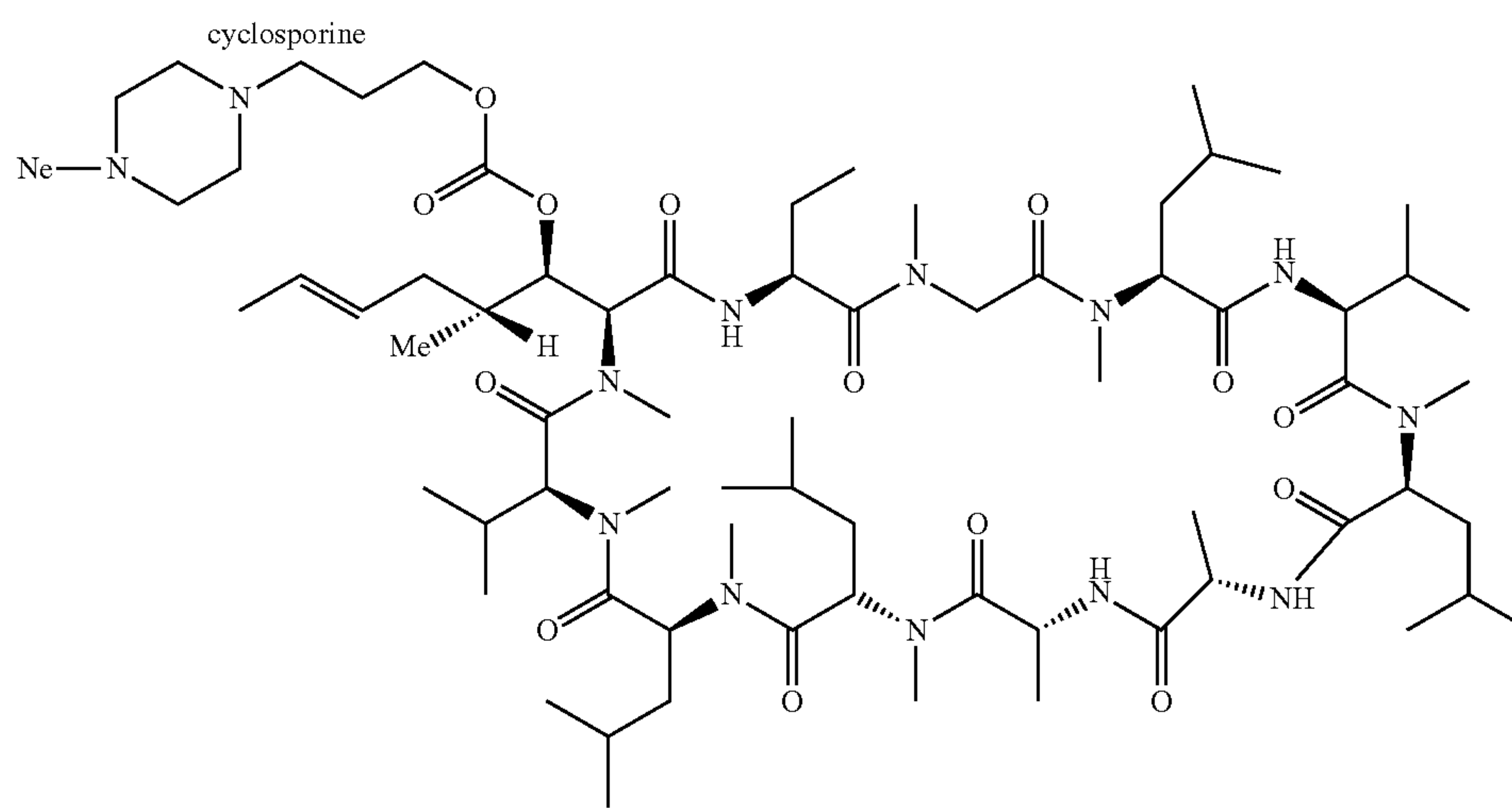
cyclosporine derivative Figure 7
