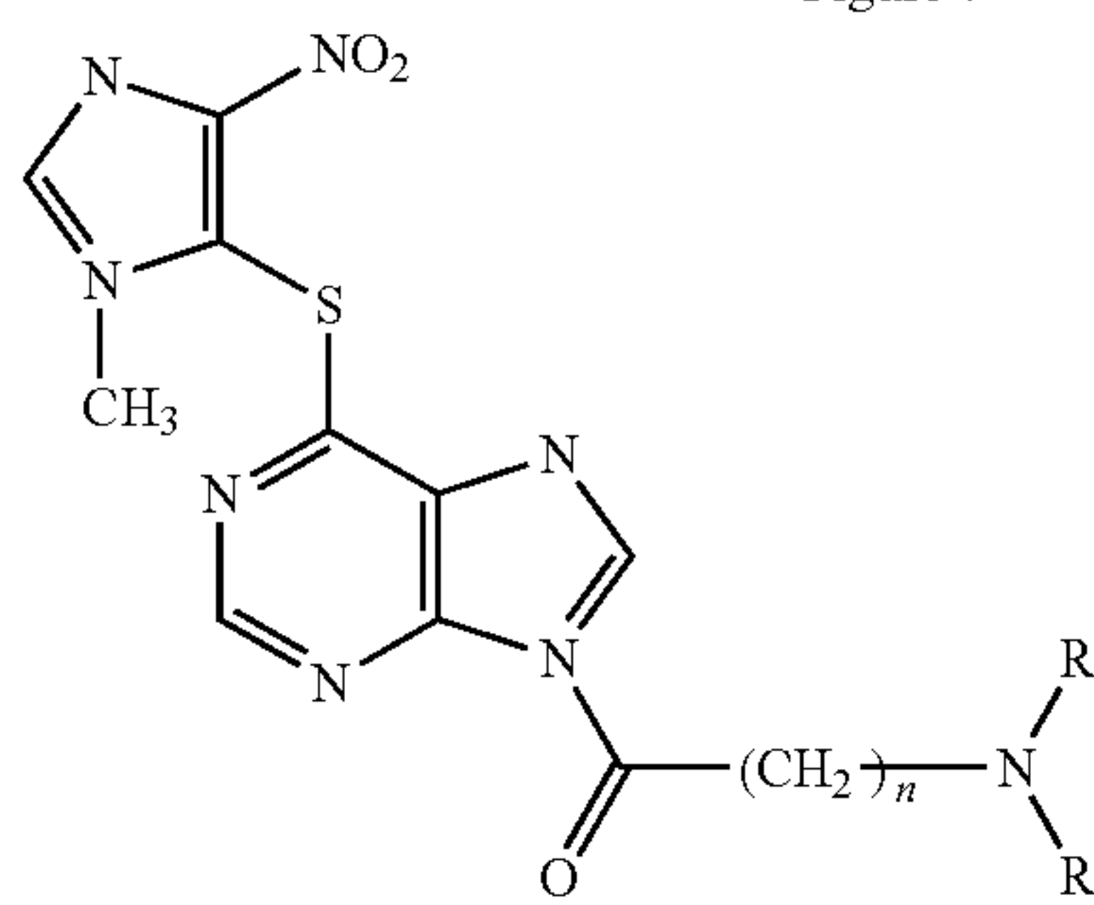
azathioprine derivatives
