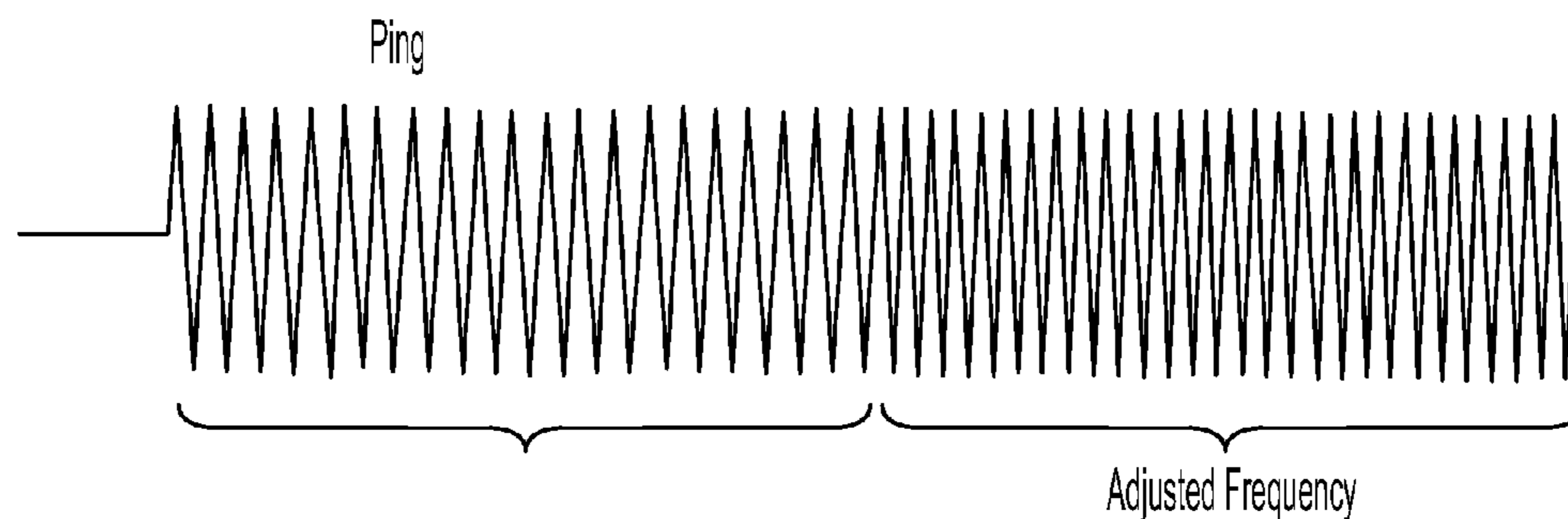
Voltage Applied to Charger Coil
