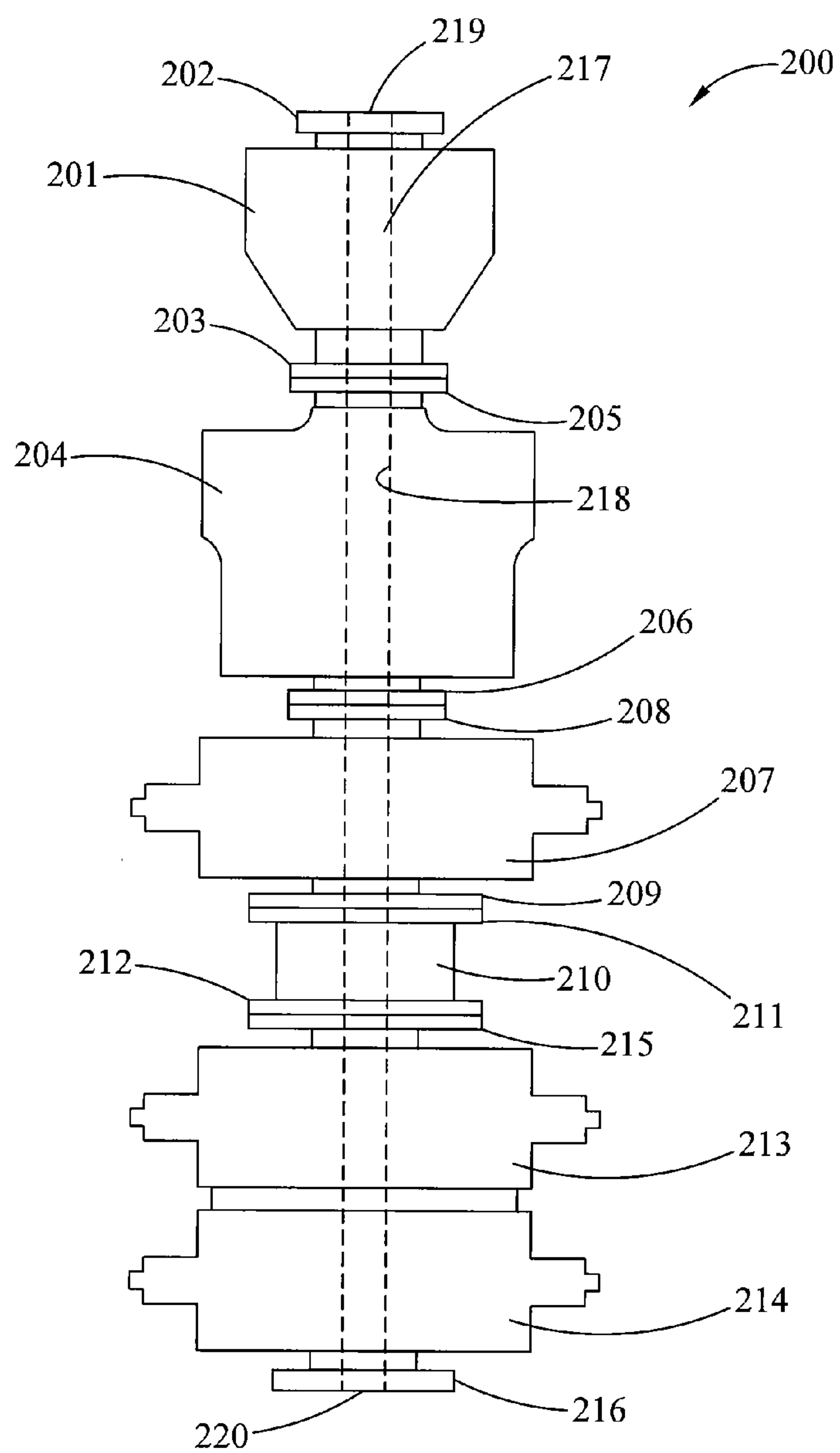
Fig. 2 (Prior Art)
