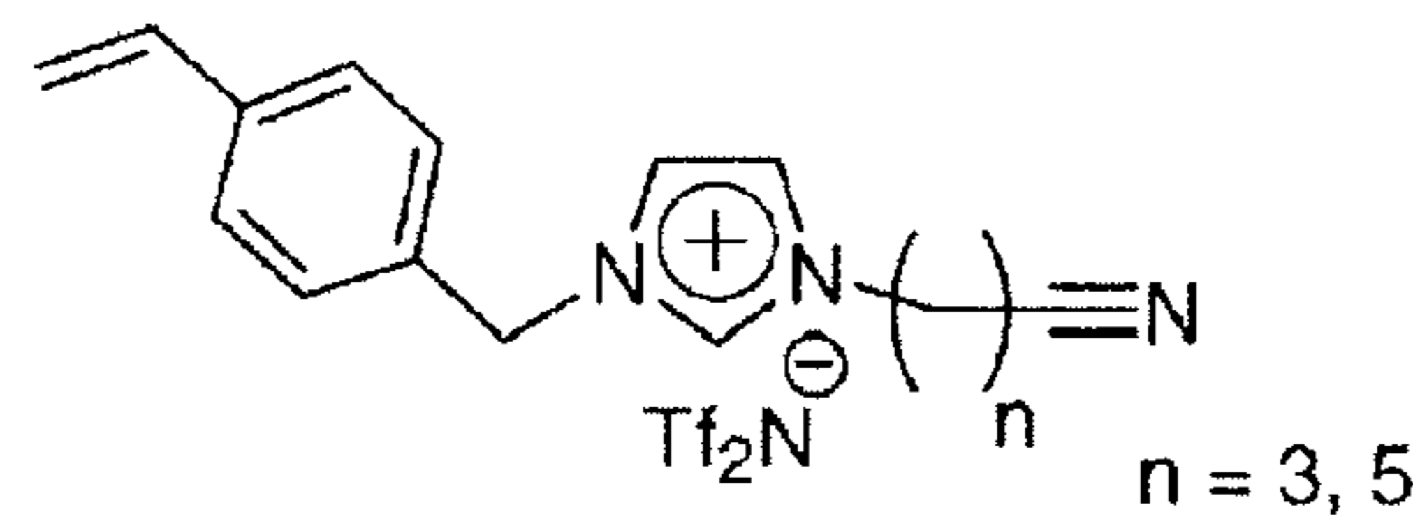
4a, b: C n CN-type
