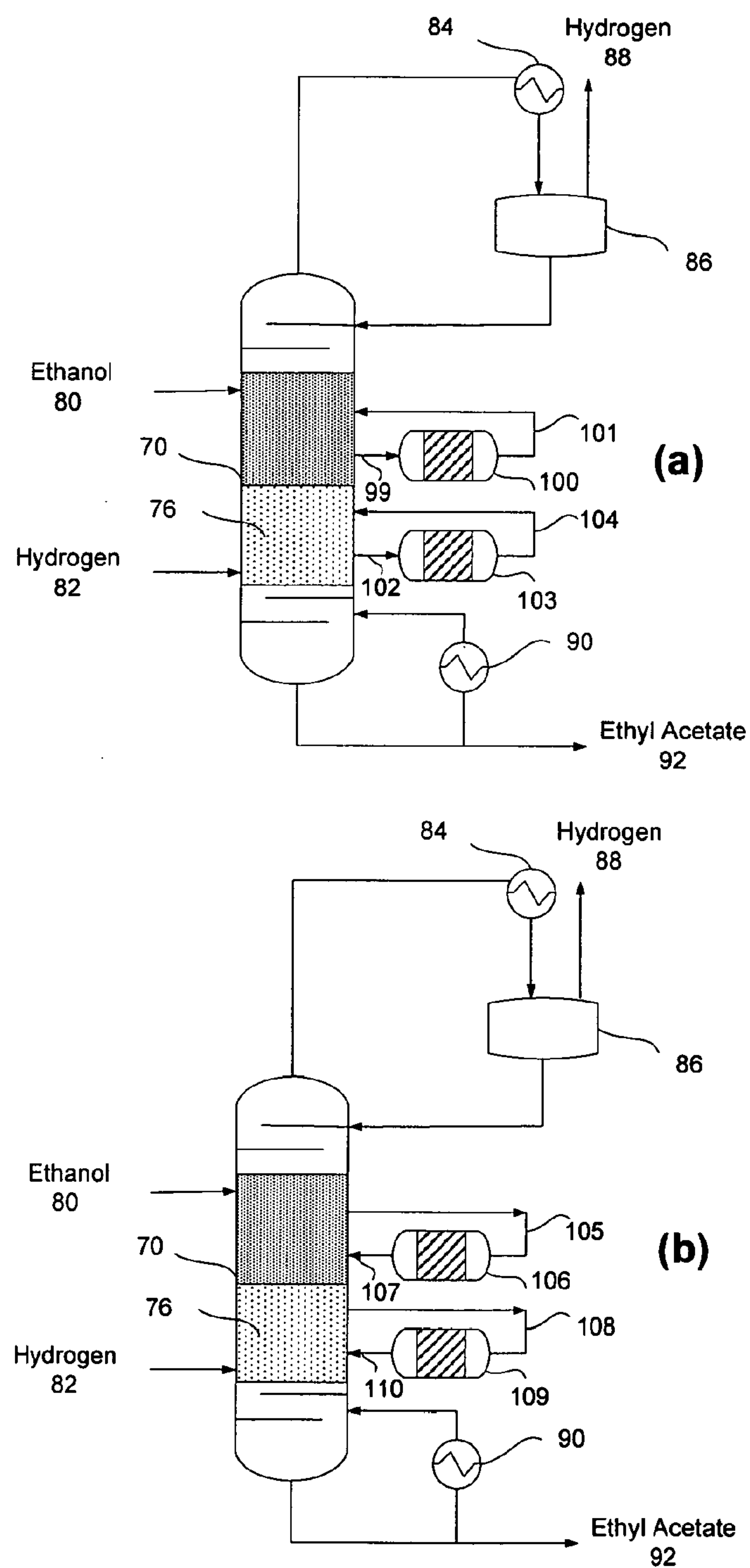
Figure 8: Double Side reactor configuration (a) upward flow feed to multiple side reactors (b) downward flow feed to multiple side reactors.
