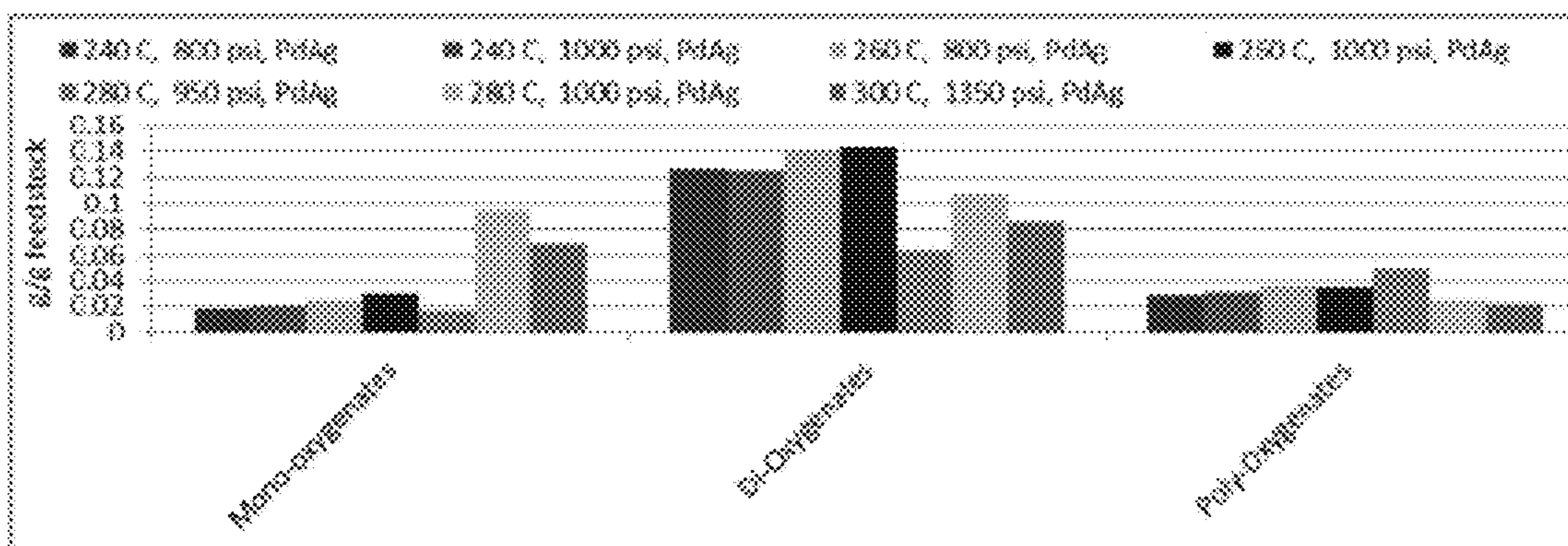
Figure 33B Biomass Conversion Results of Loblolly Pine Deconstruction at Varying Temperature and Pressure
