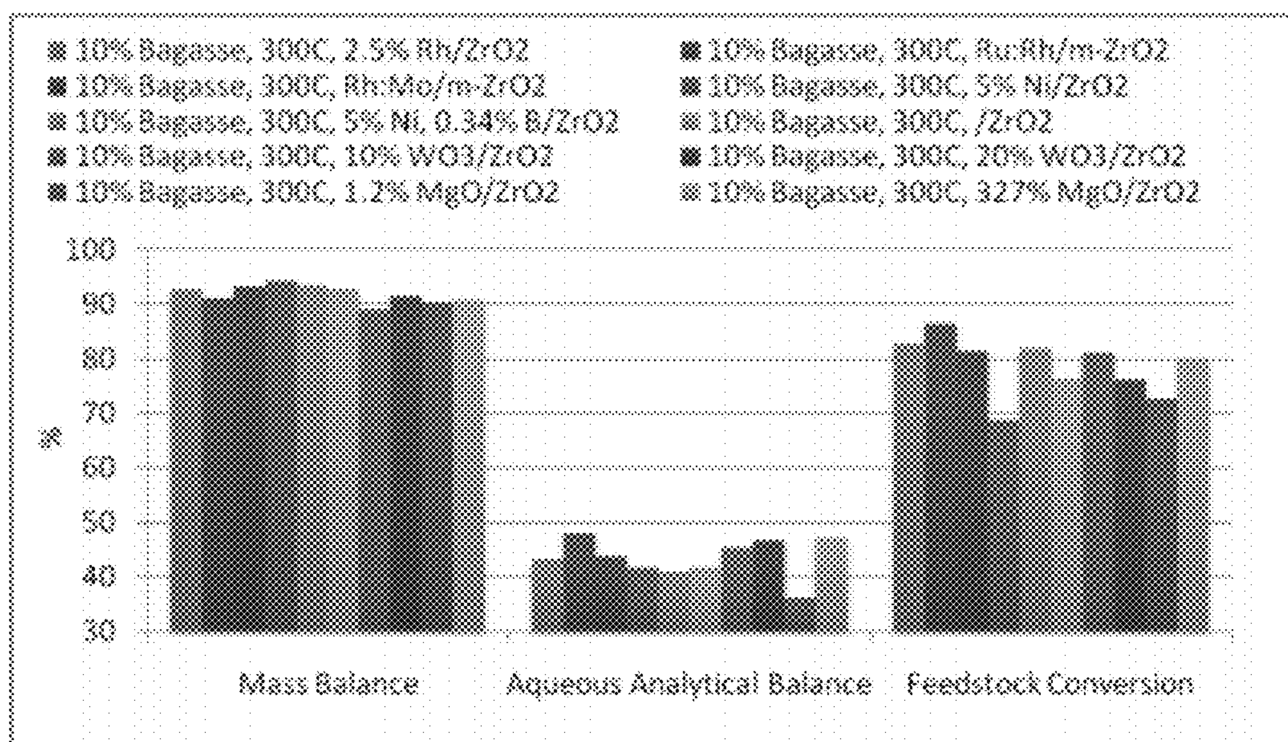
Figure 20. Conversion of sugarcane bagasse over various catalysts.
