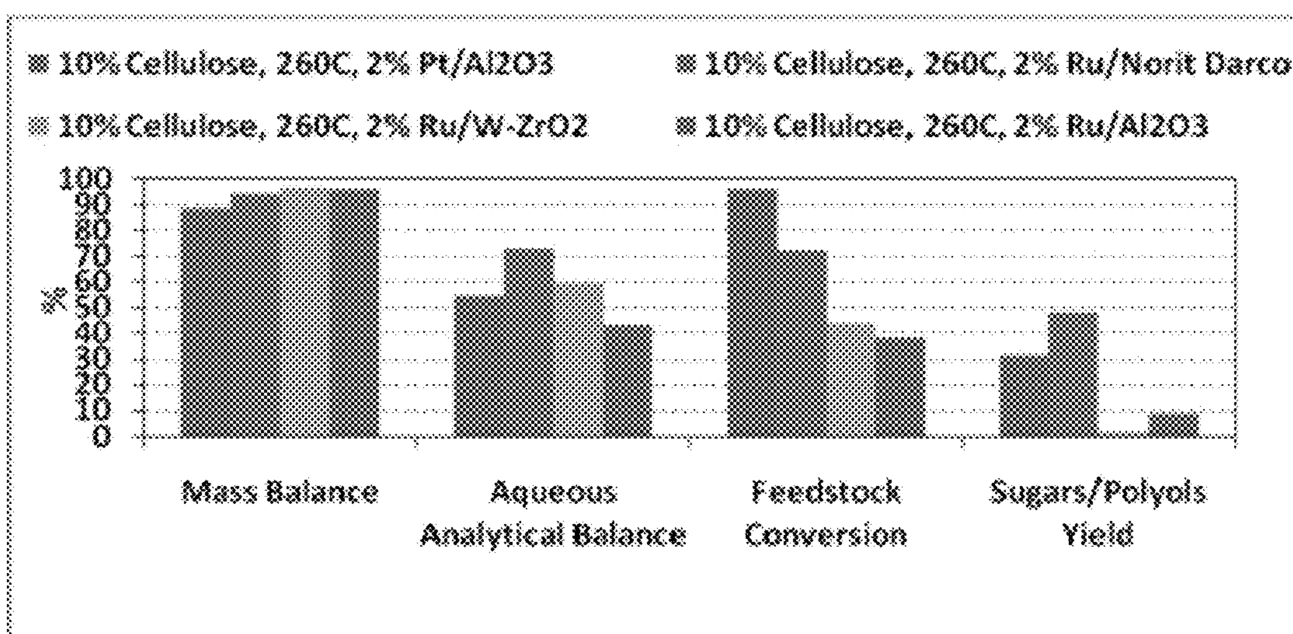
Figure 14: Hydrogenolysis of microcrystalline cellulose with different catalysts.
