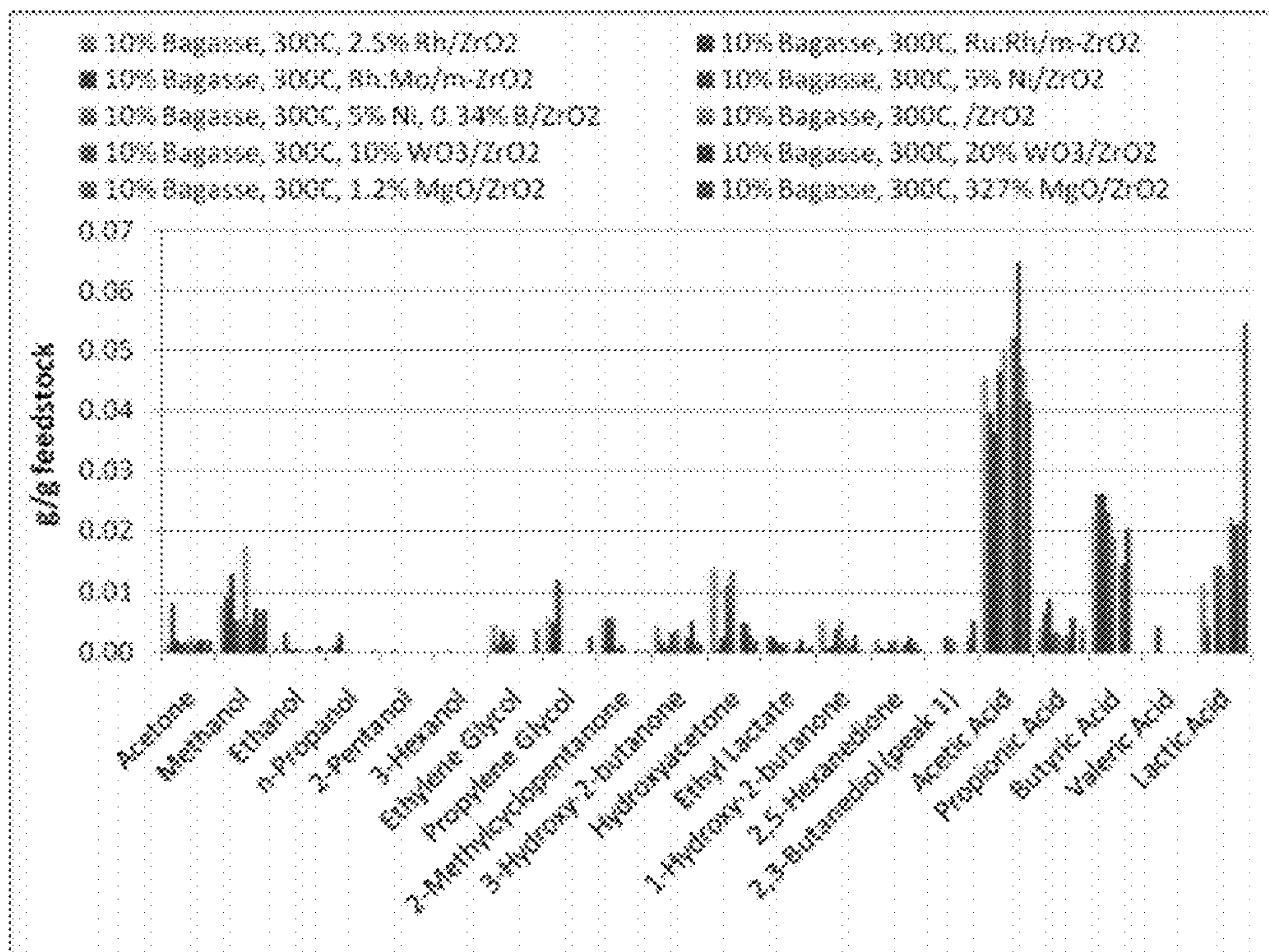
Figure 22. Detailed product distribution of the conversion of sugarcane bagasse over various catalysts.
