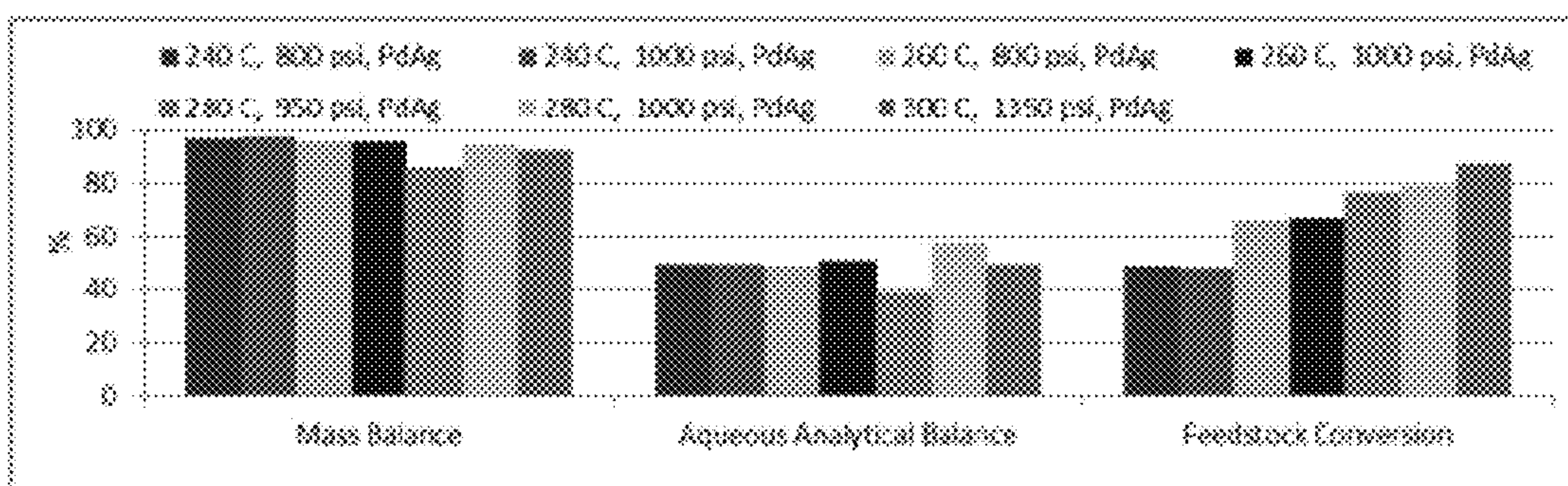
Figure 33A Overall Balances of Loblolly Pine Deconstruction at Varying Temperature and Pressure
