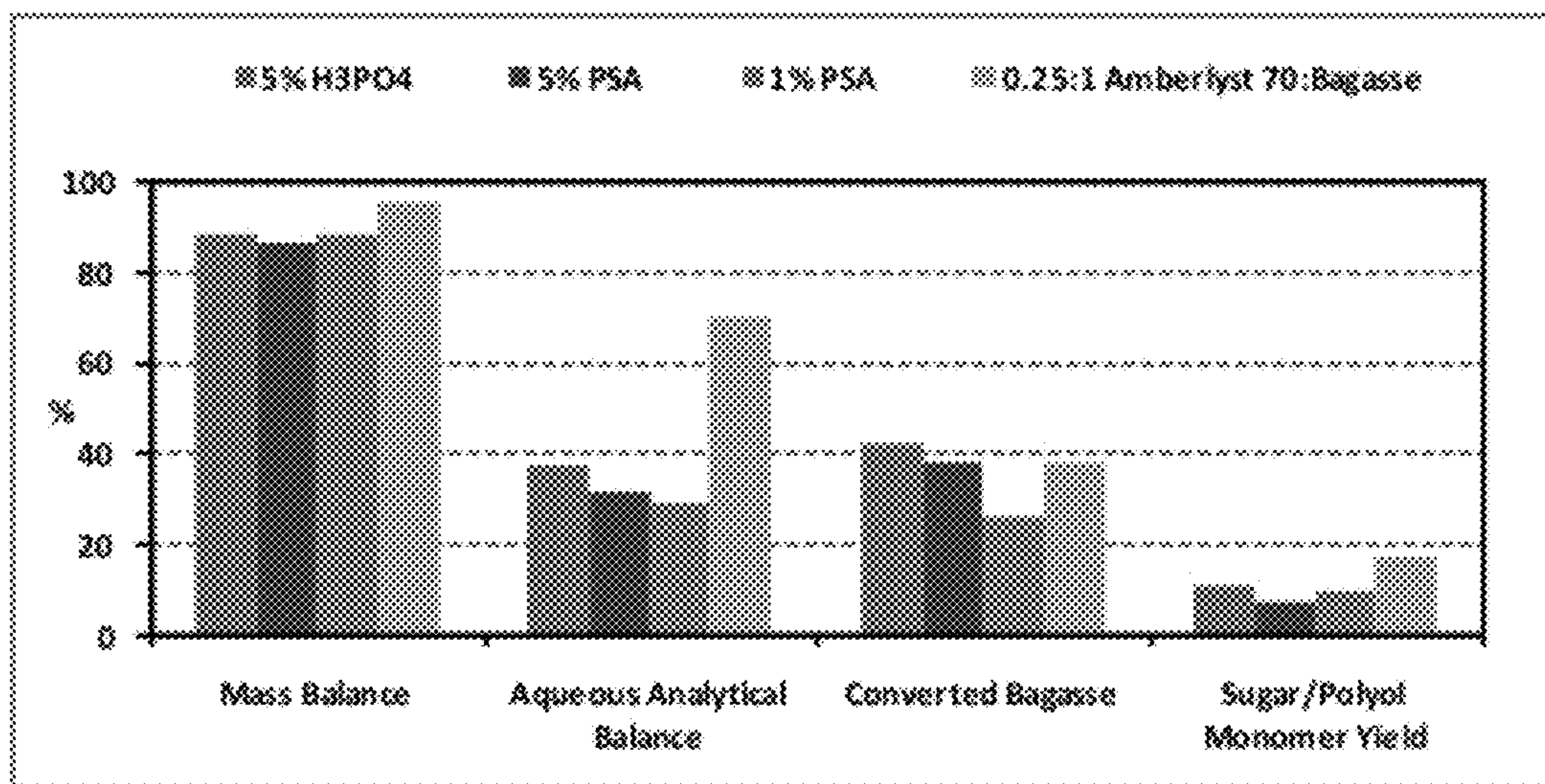
Figure 10. Overall results of bagasse hydrolysis using phosphoric acid, PSA and Amberlyst 70.
