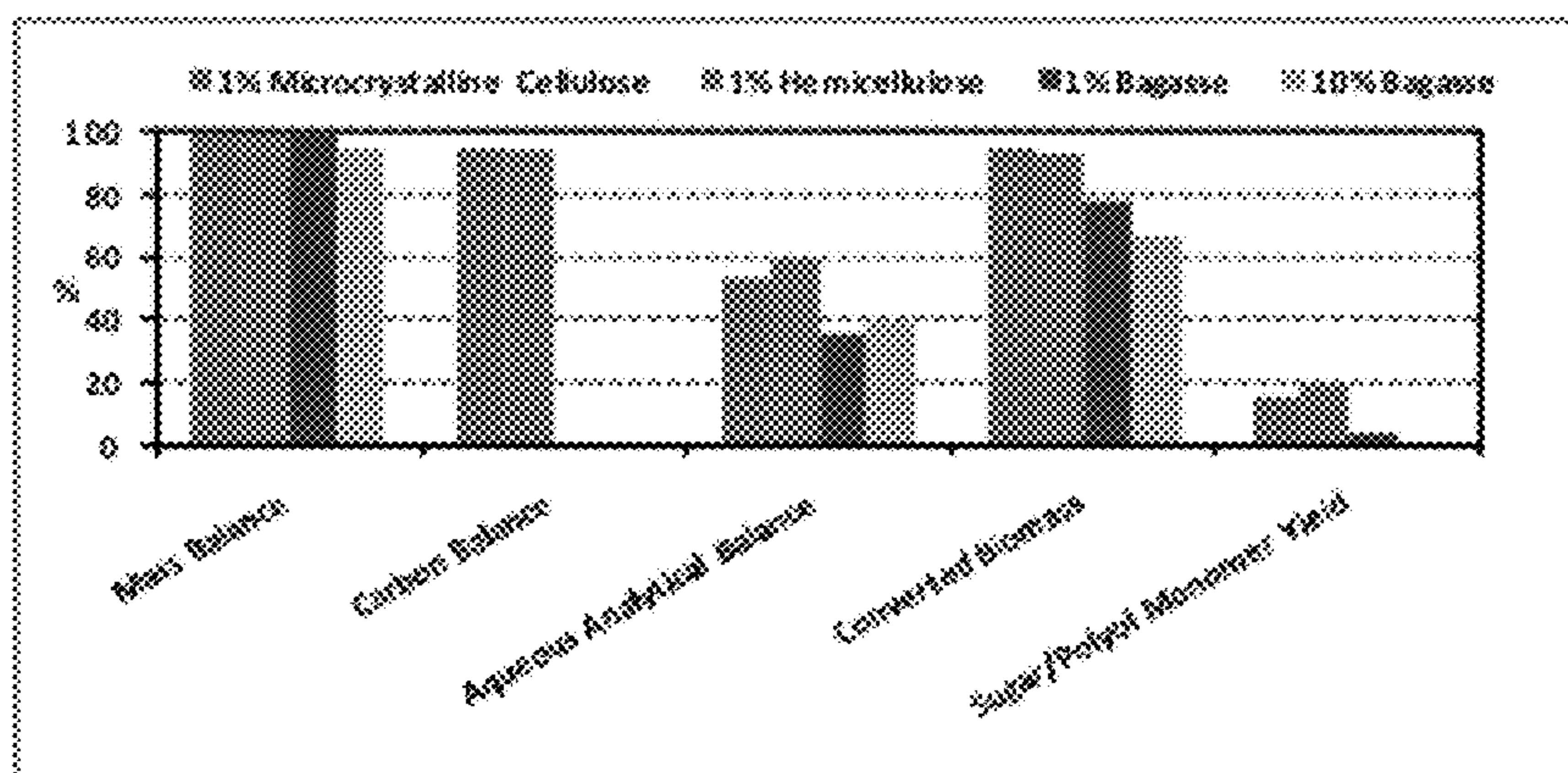
Figure 23. Cellulosic conversion over nickel tungsten carbide catalyst
