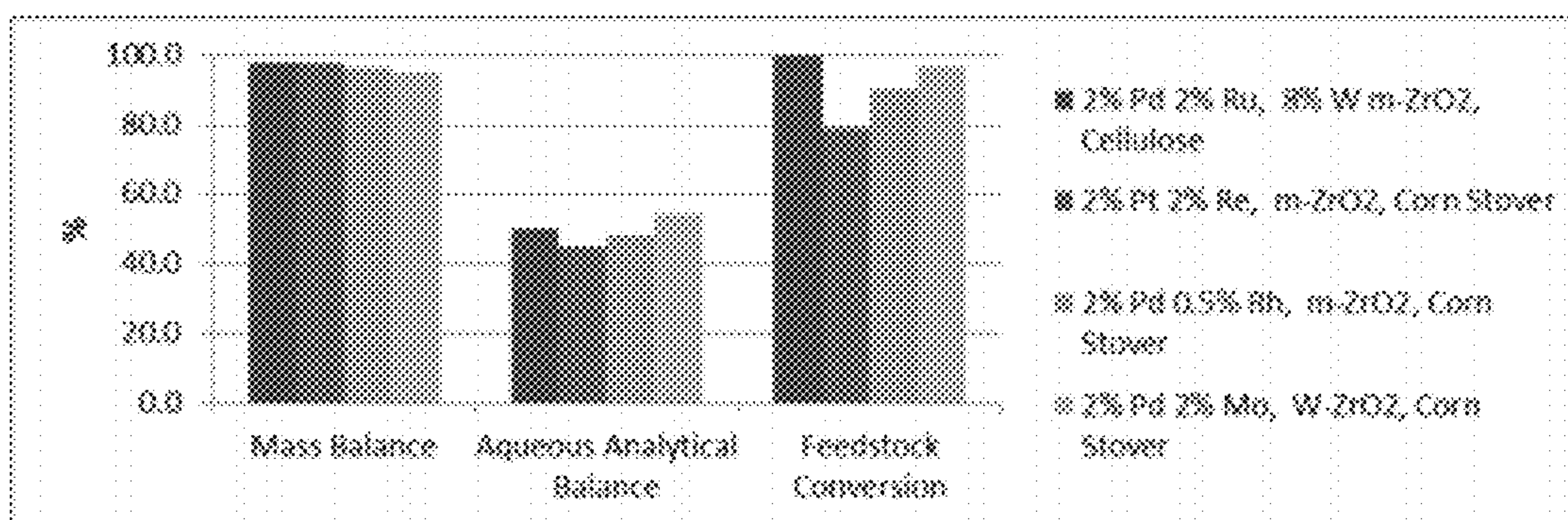
Figure 26. Mass and Analytical Balances and Feedstock Conversion of Catalytic Deconstruction
