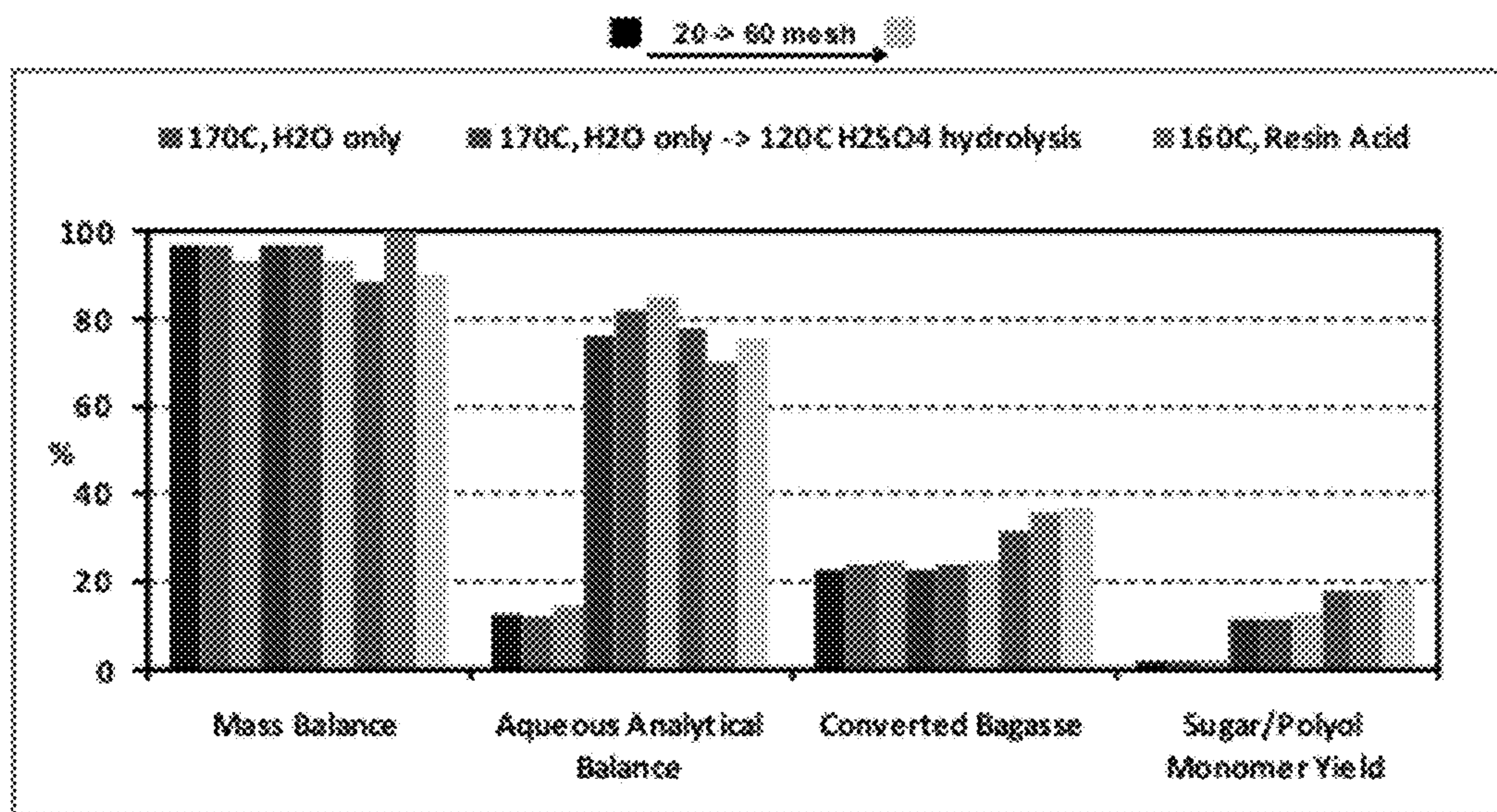
Figure 12. Results of hydrolysis using different bagasse particle sizes (<20, 40, and 60 mesh).
