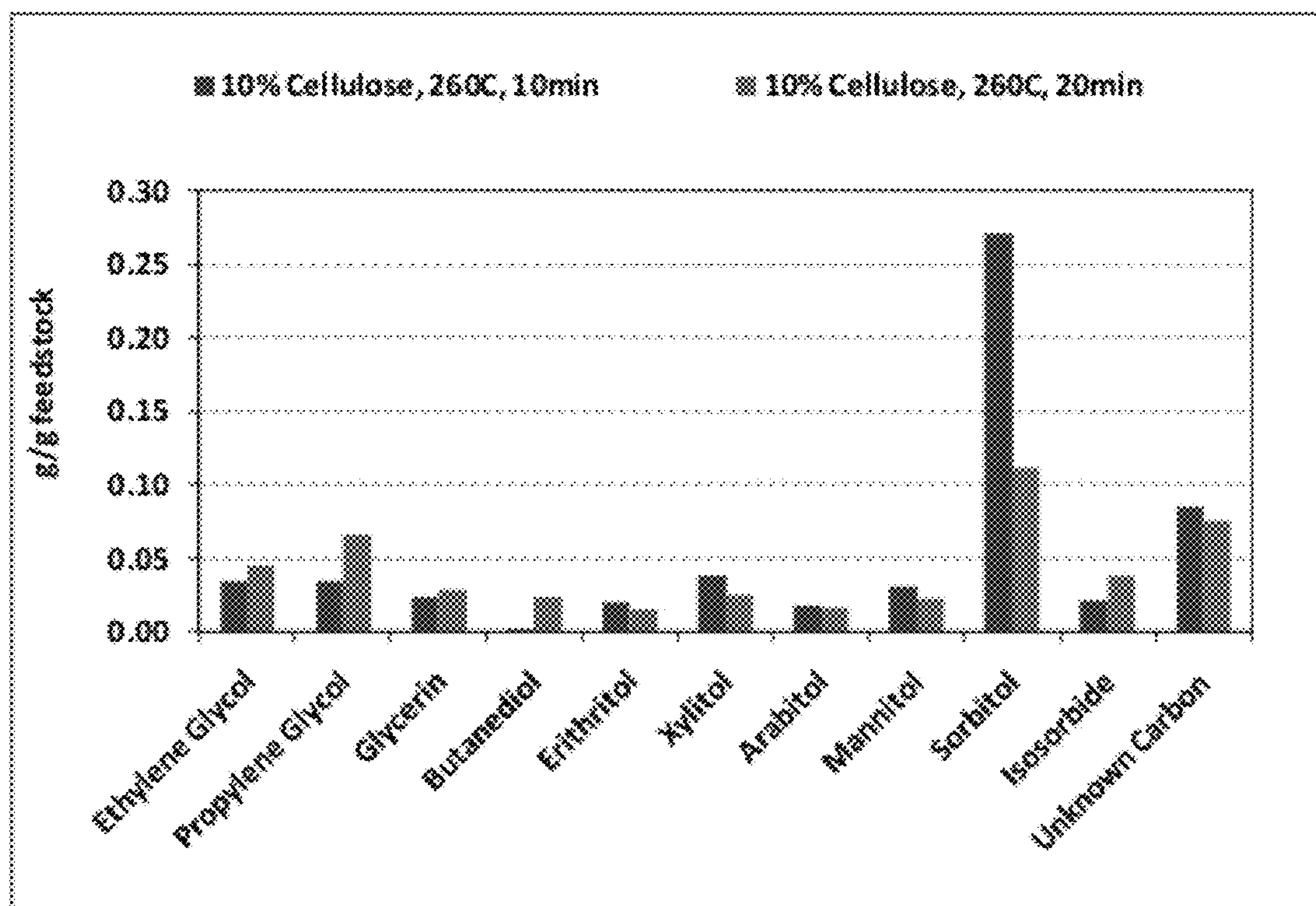
Figure 5. Product yields in aqueous from MCC
