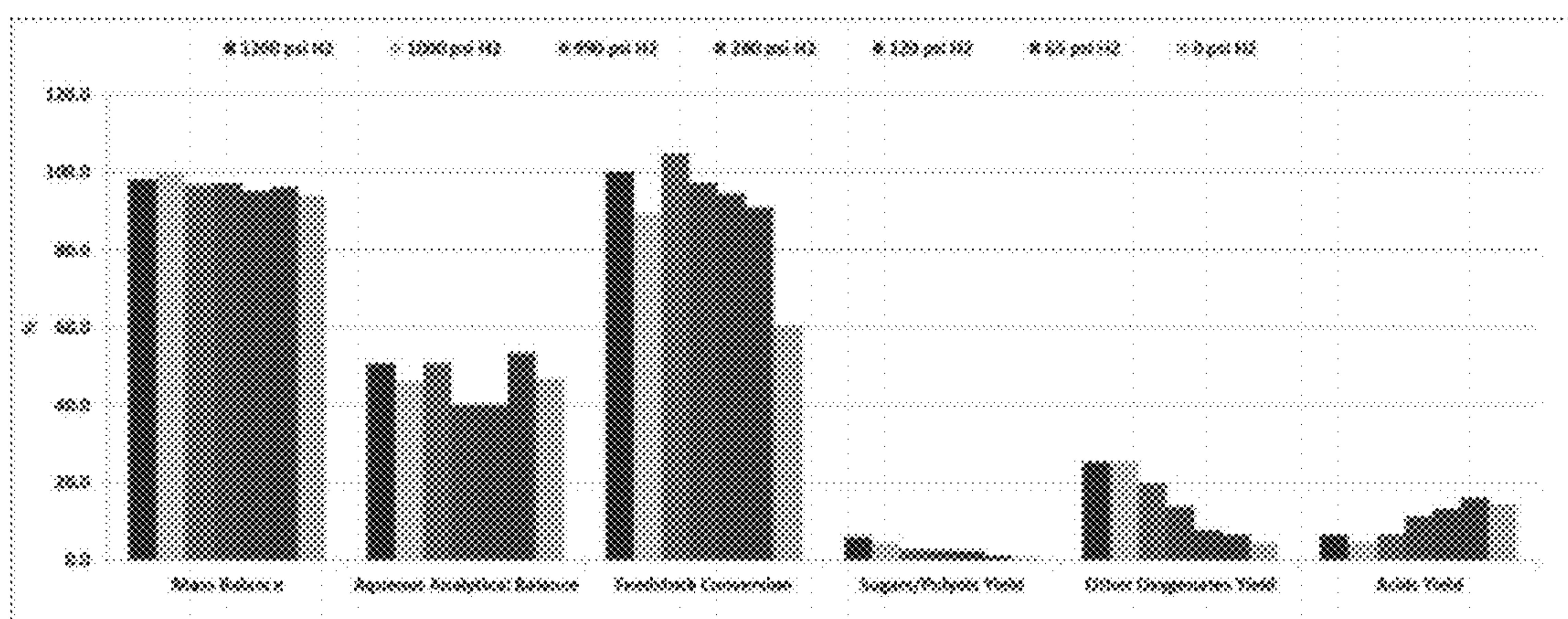
Figure 30-A. Carbon Conversion to the Aqueous Phase at Varying Reaction Hydrogen Partial Pressures with Microcrystalline Cellulose
