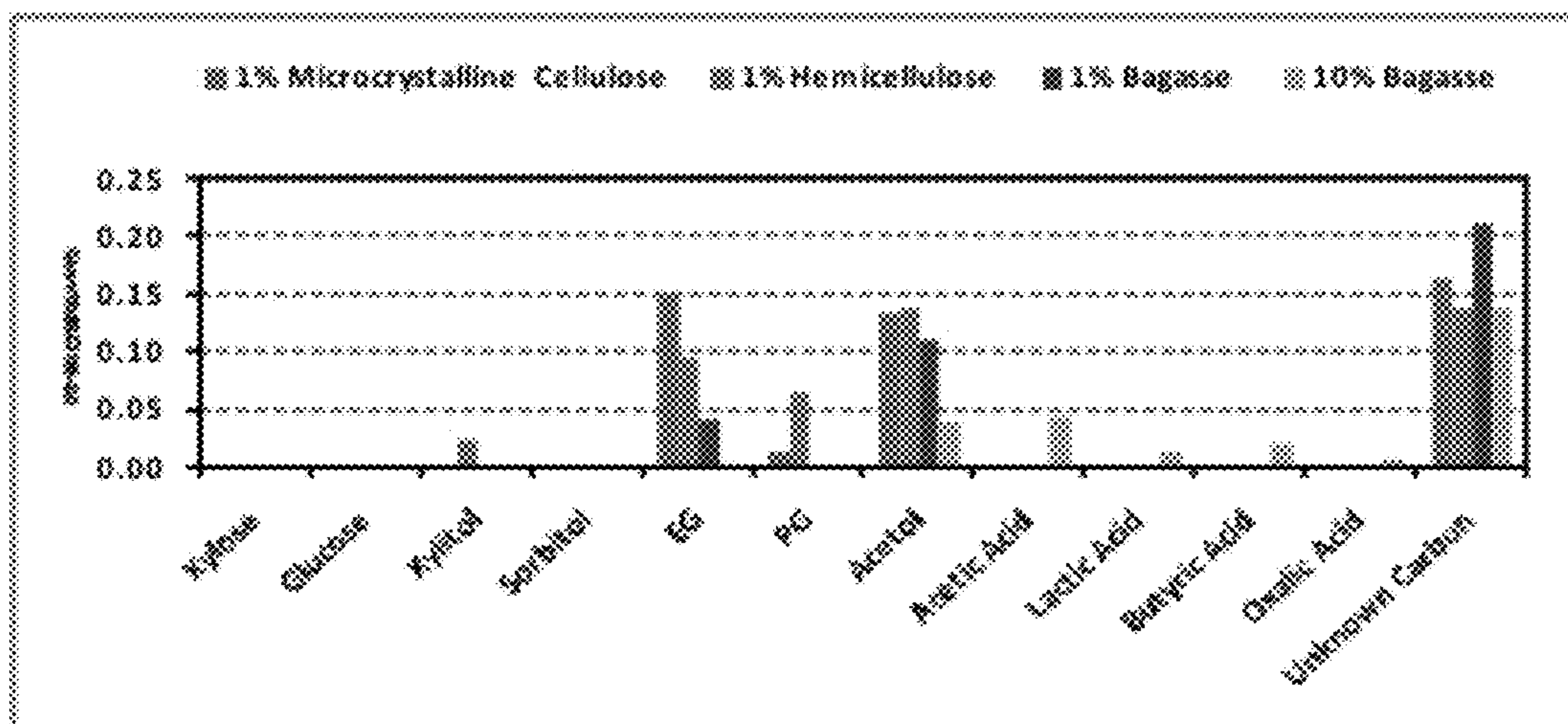
Figure 24. Product distribution of celluloses conversion over nickel tungsten carbide catalyst
