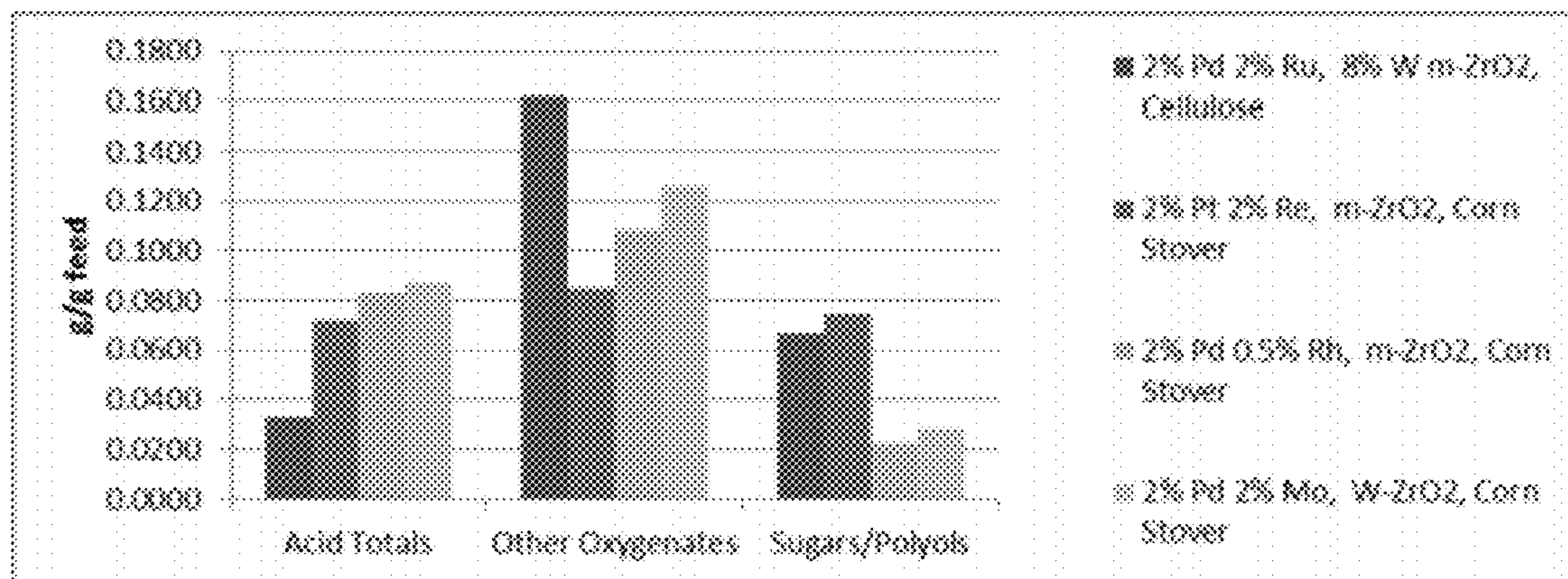
Figure 28. Product Yields of Catalytic Deconstruction
