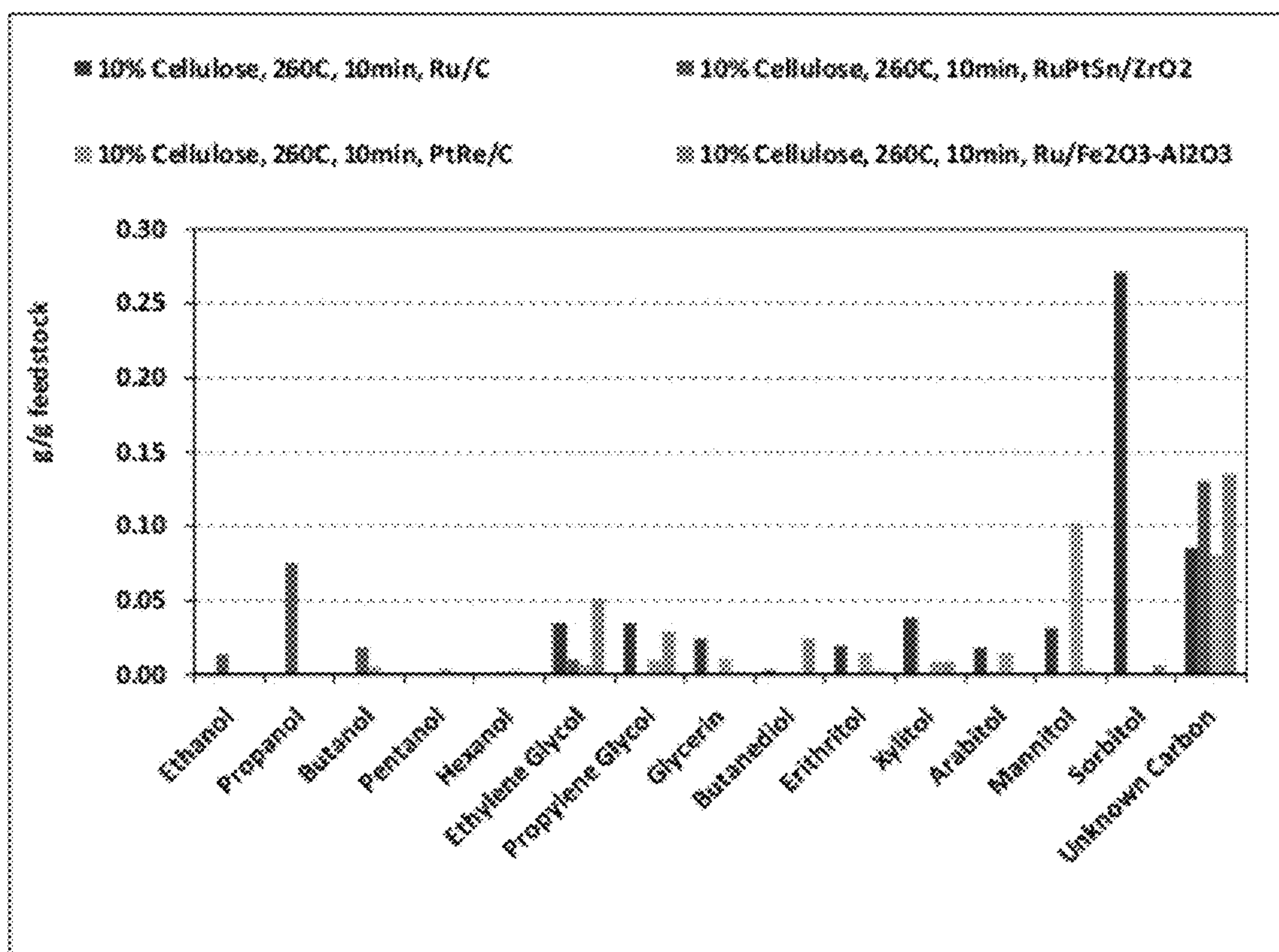
Figure 7. Product yields from the conversion of MCC using various deconstruction catalysts.
