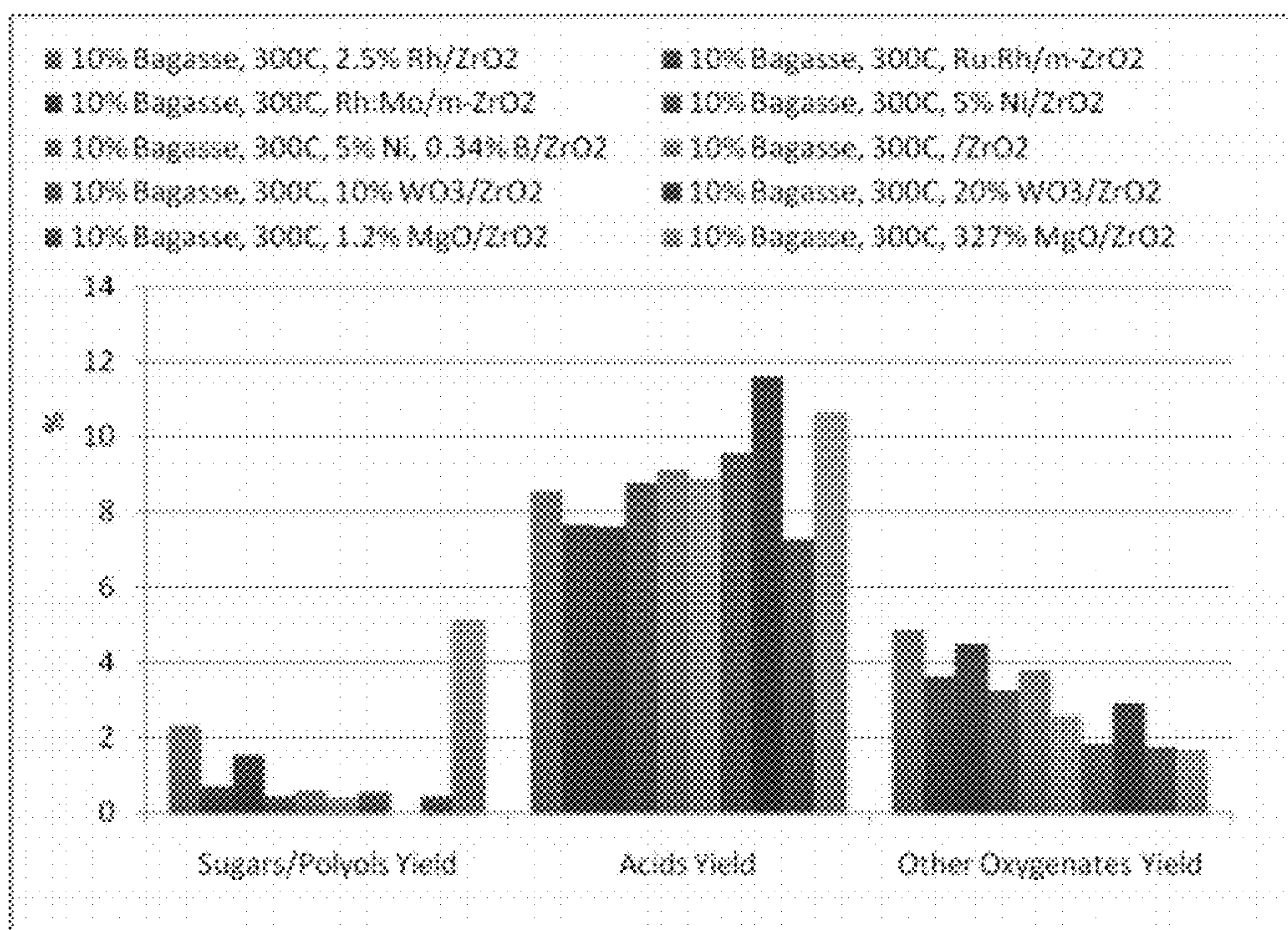
Figure 21. Oxygenated product yields for the conversion of sugarcane bagasse over various catalysts.
