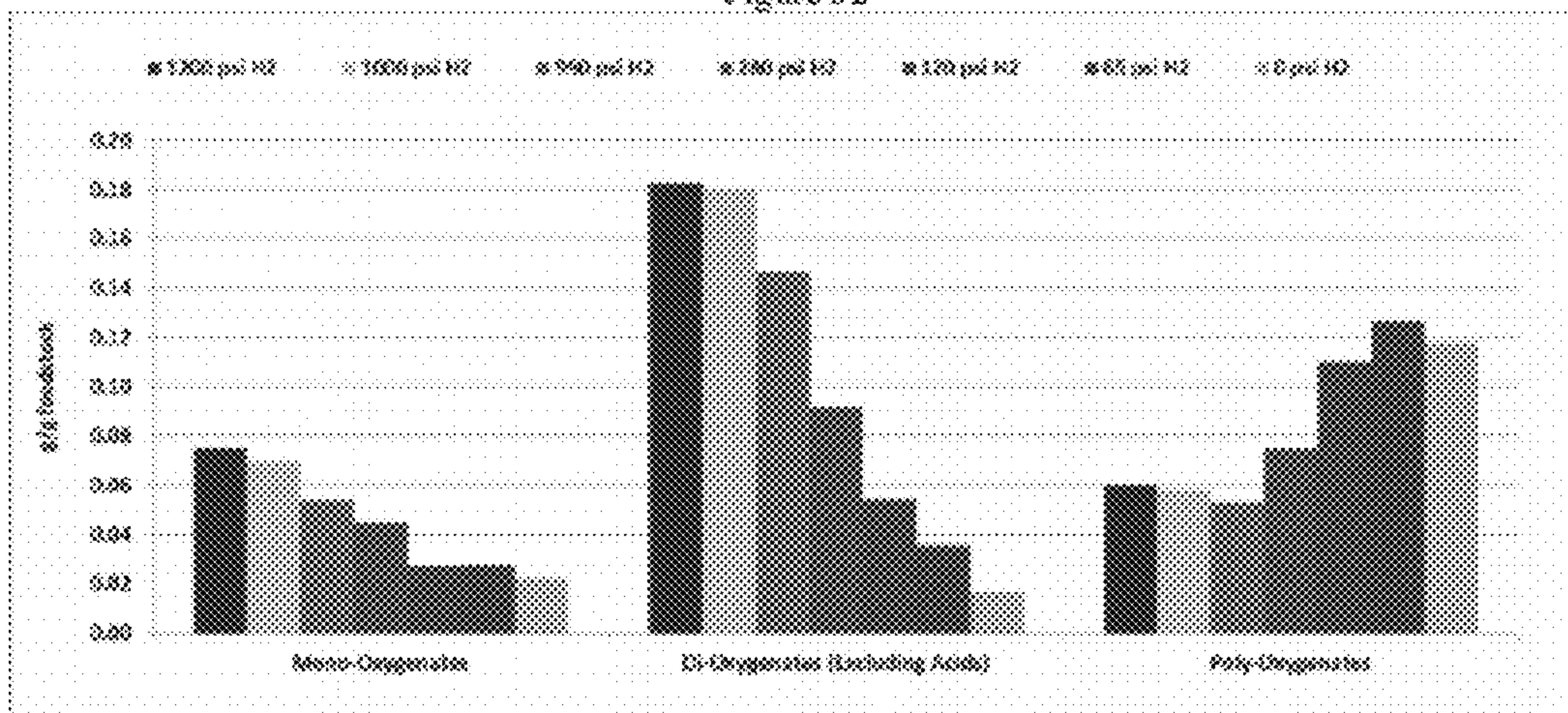
Figure 32. Degree of Oxygenates at Varying Reaction Hydrogen Partial Pressures with Microcrystalline Cellulose
