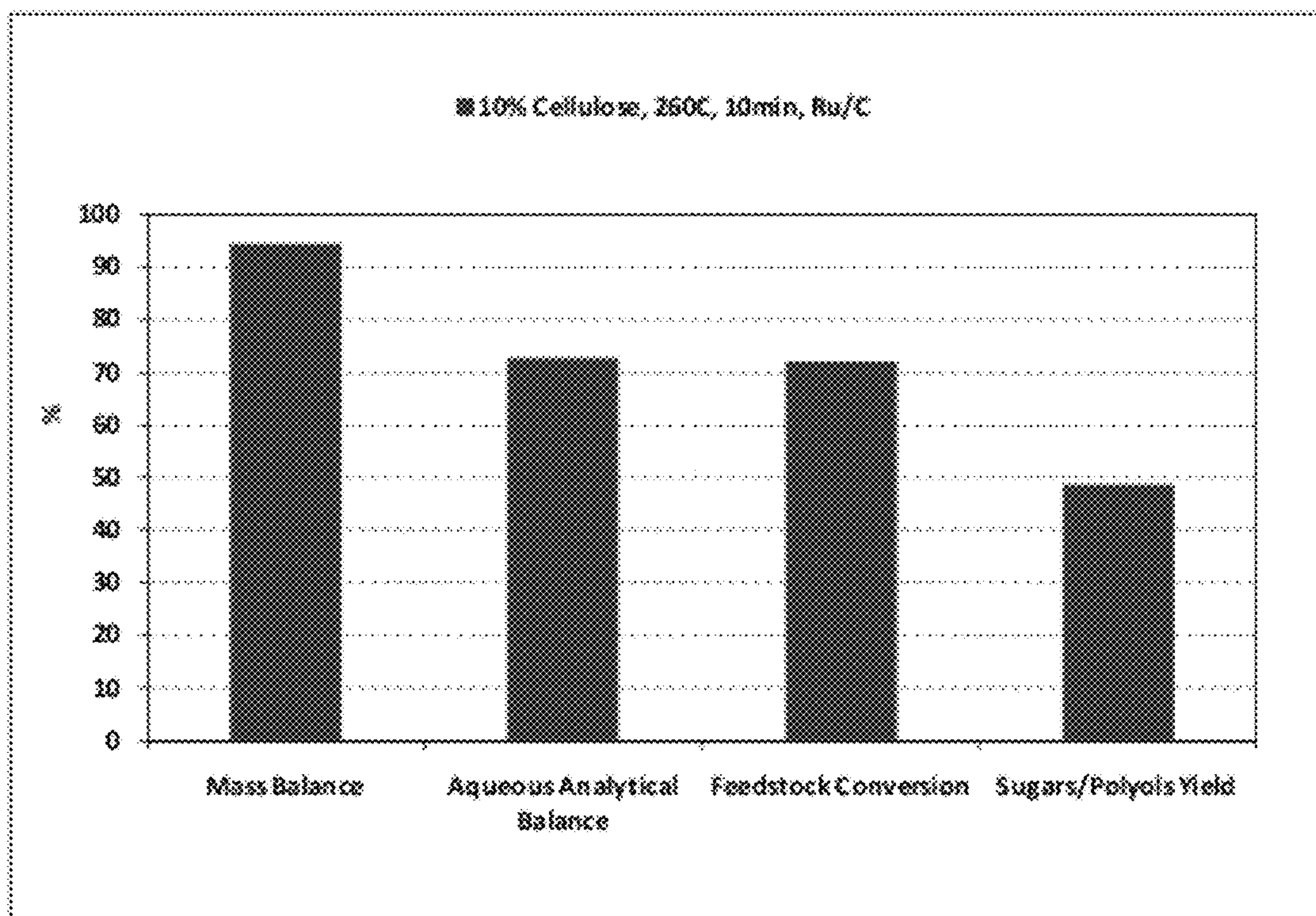
Figure 2. Microcrystalline cellulose conversion data.
