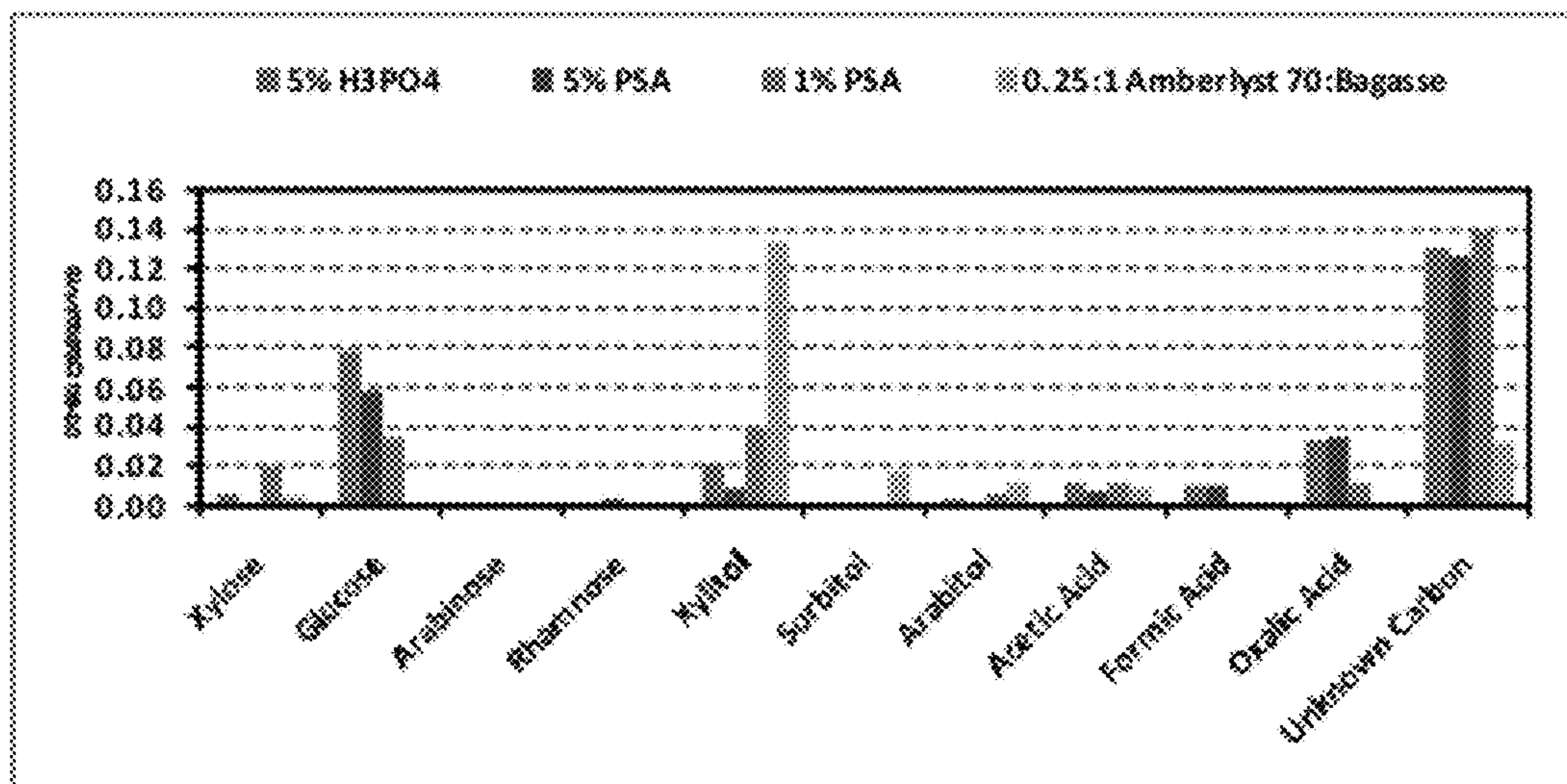
Figure 11. Major products of bagasse hydrolysis using phosphoric acid, PSA and Amberlyst 70.
