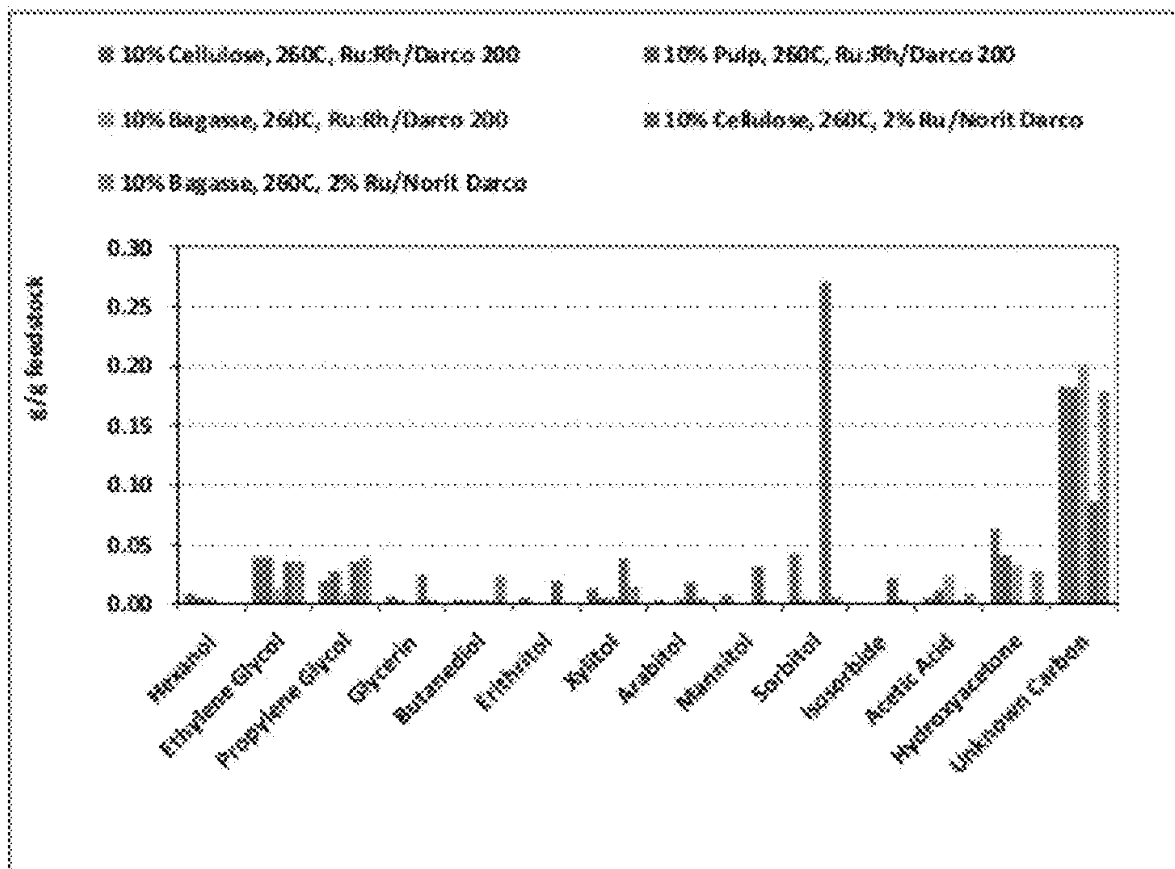
Figure 19: Products in aqueous fraction resulting from biomass deconstruction.
