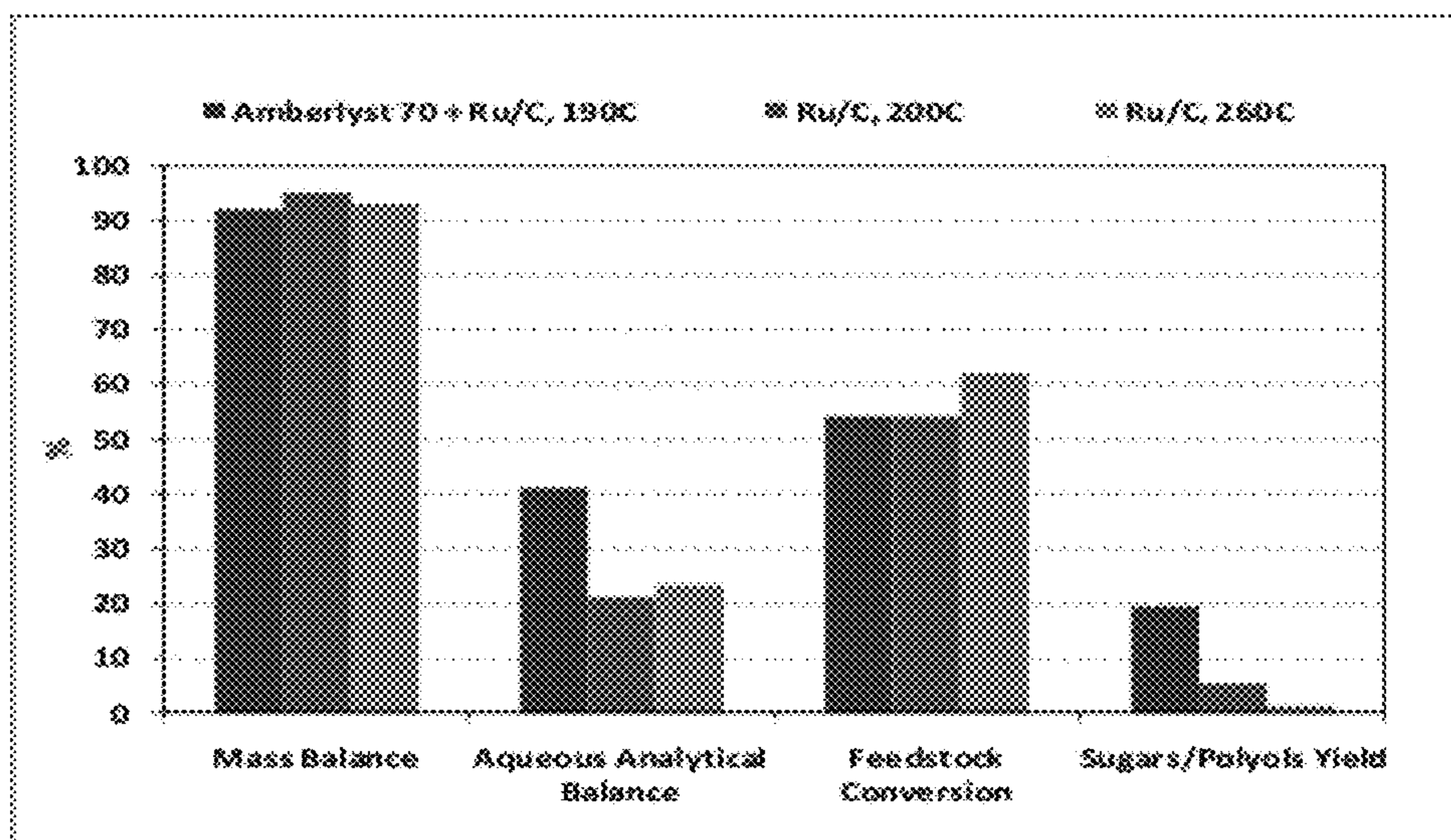
Figure 16: Hydrogenolysis of corn fiber.
