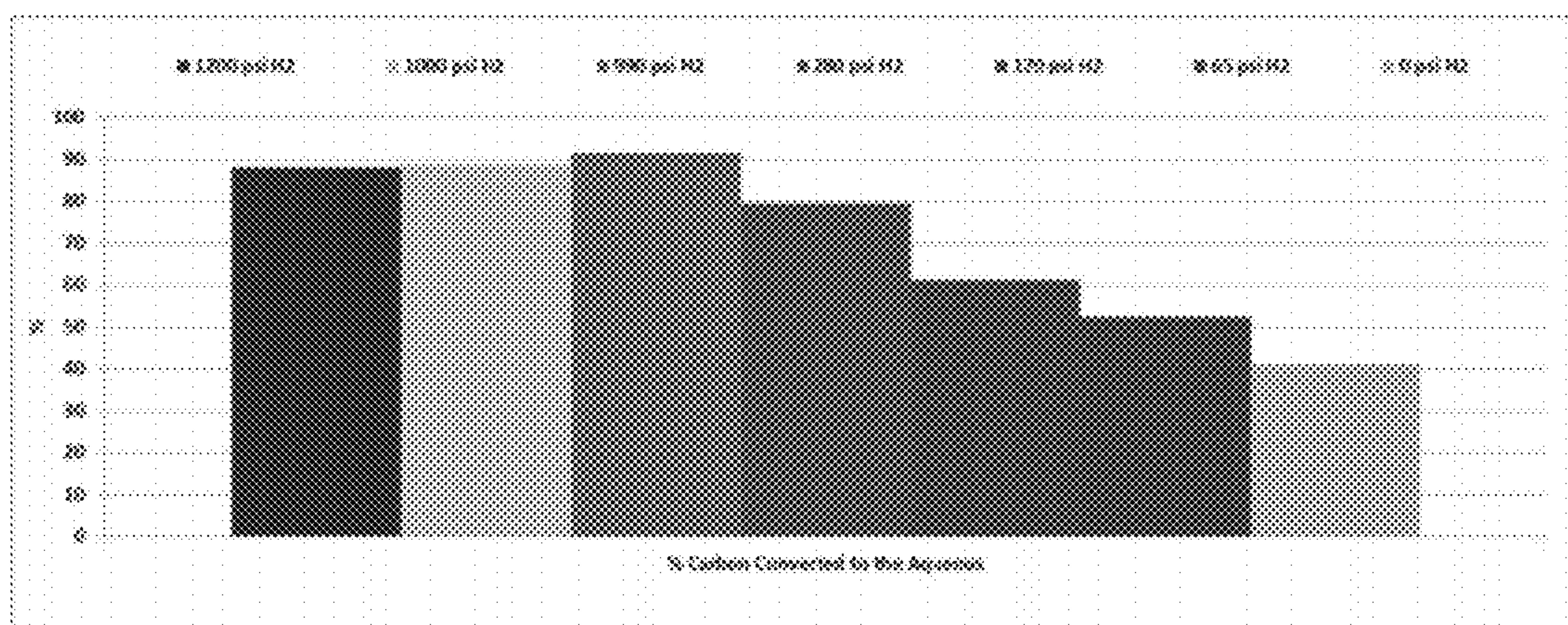
Figure 30-B. Carbon Conversion to Aqueous at Varying Reaction Hydrogen Partial Pressures with Microcrystalline Cellulose
