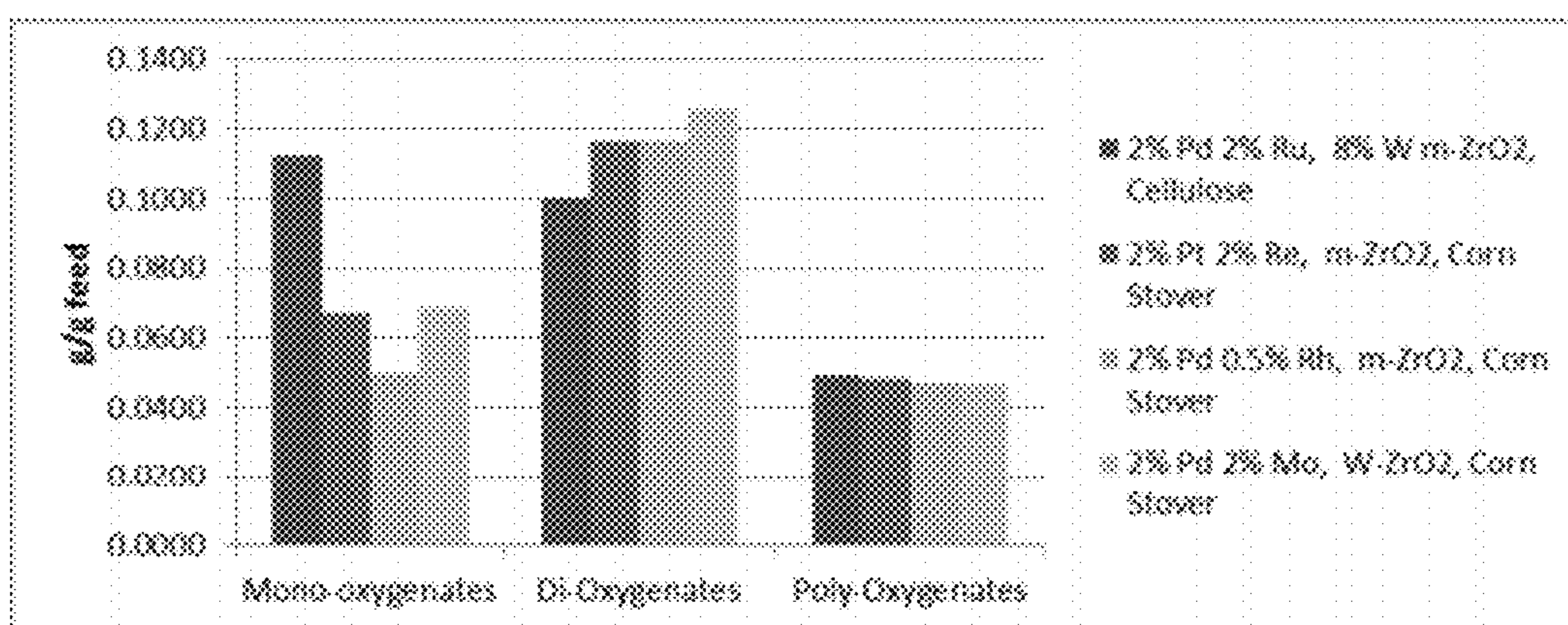
Figure 27. Levels of Deoxygenation of Catalytic Deconstruction
