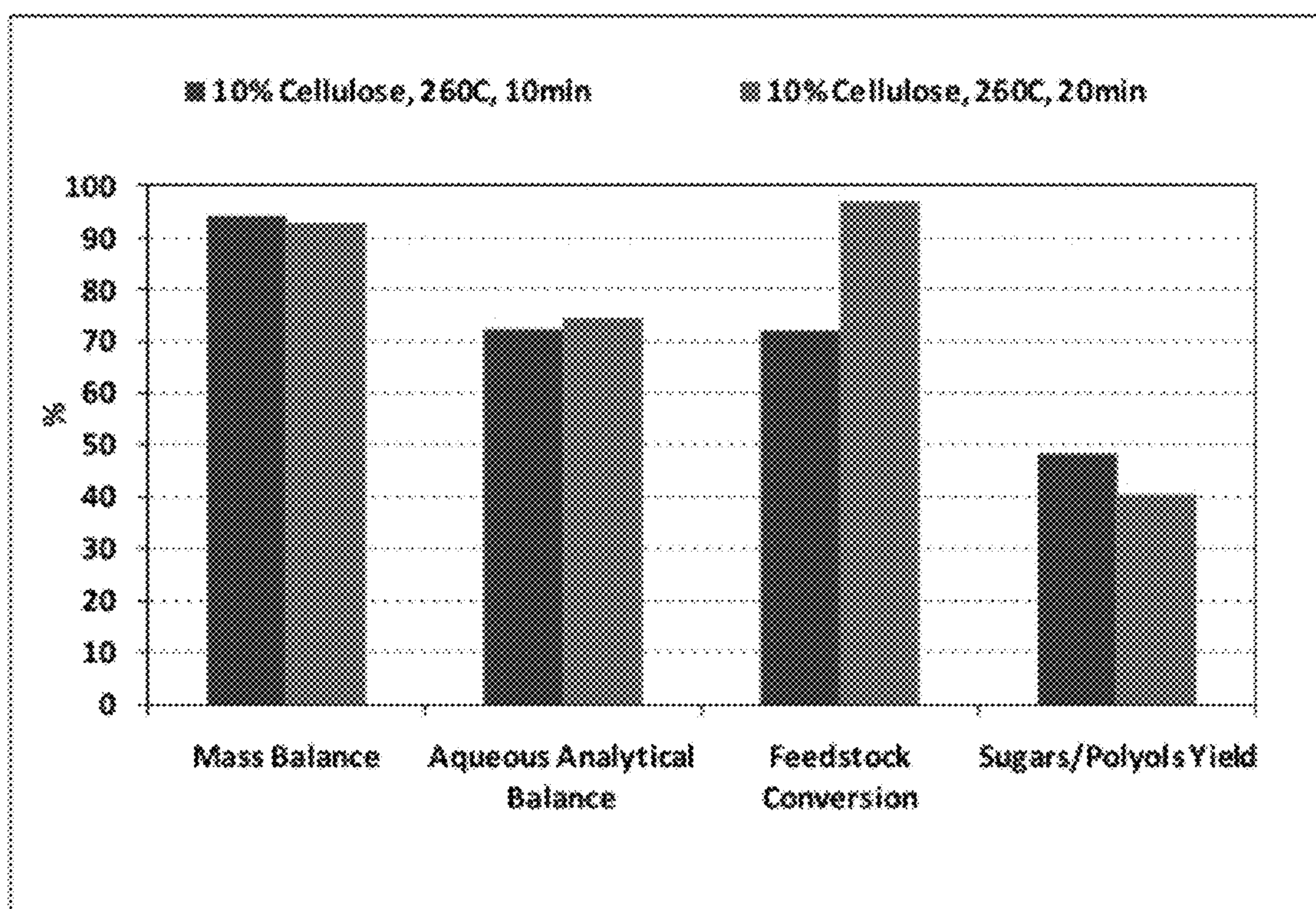
Figure 4. 10 minute vs. 20 minute conversion data
