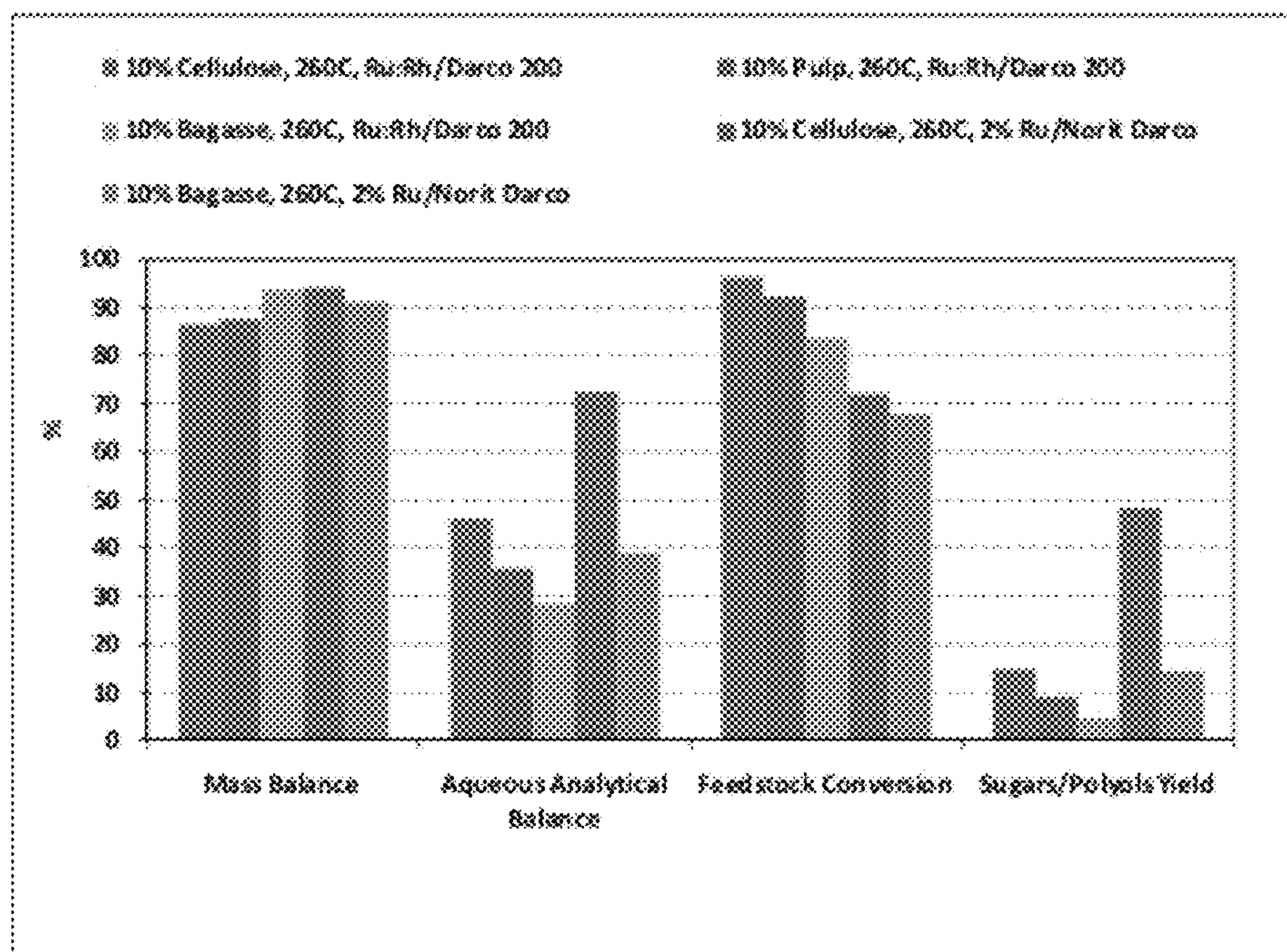
Figure 18: Catalytic deconstruction of lignocellulosics.
