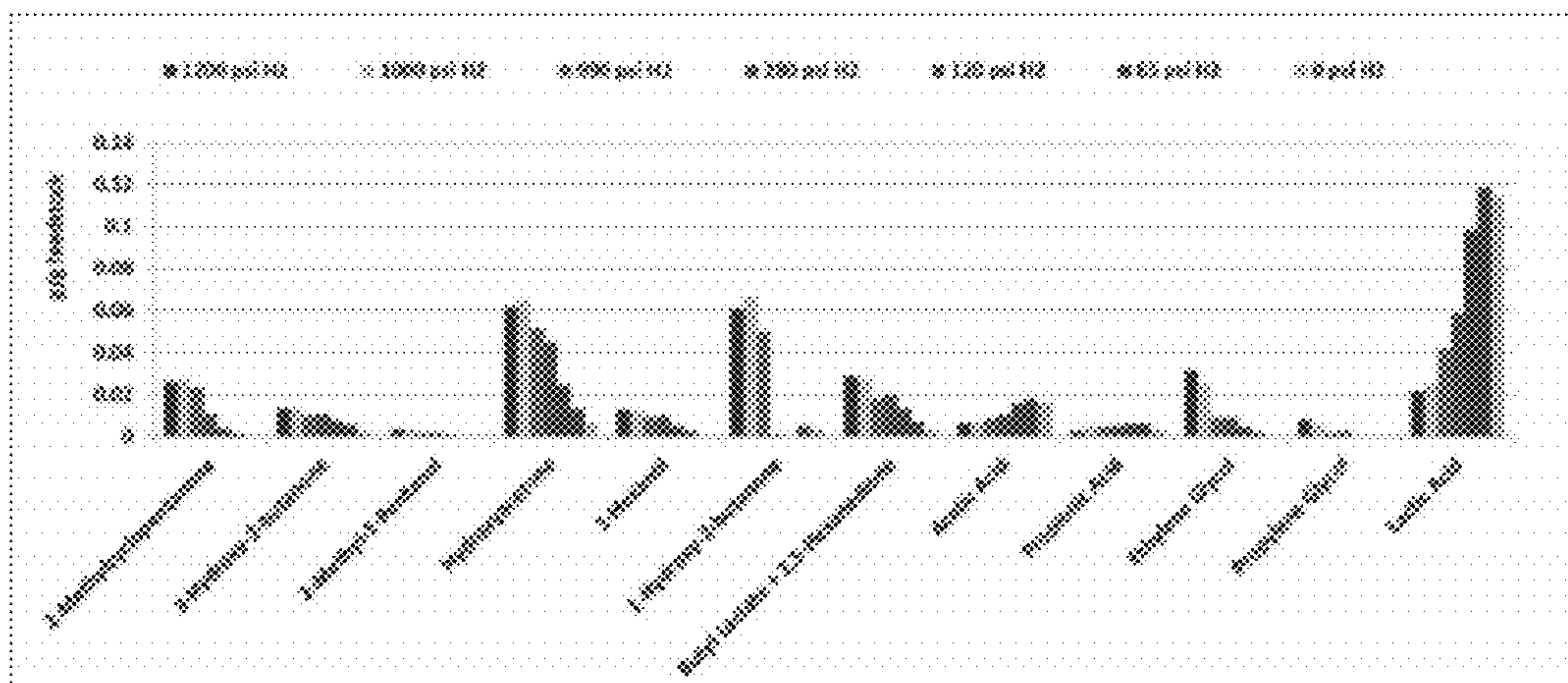
Figure 31. Product Selectivity at Varying Reaction Hydrogen Partial Pressures with Microcrystalline Cellulose
