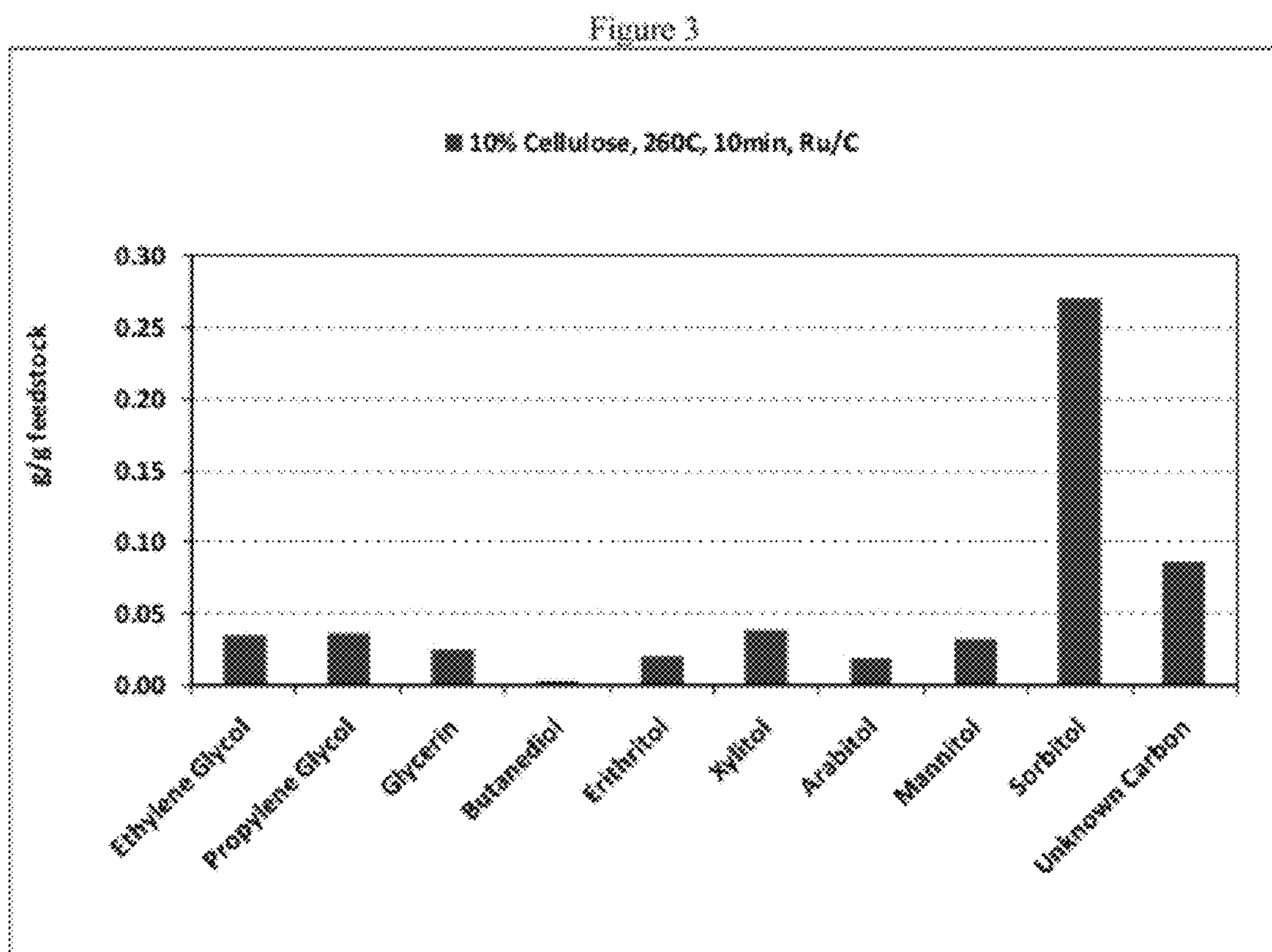
Figure 3. Product Yields in aqueous fraction from MCC
