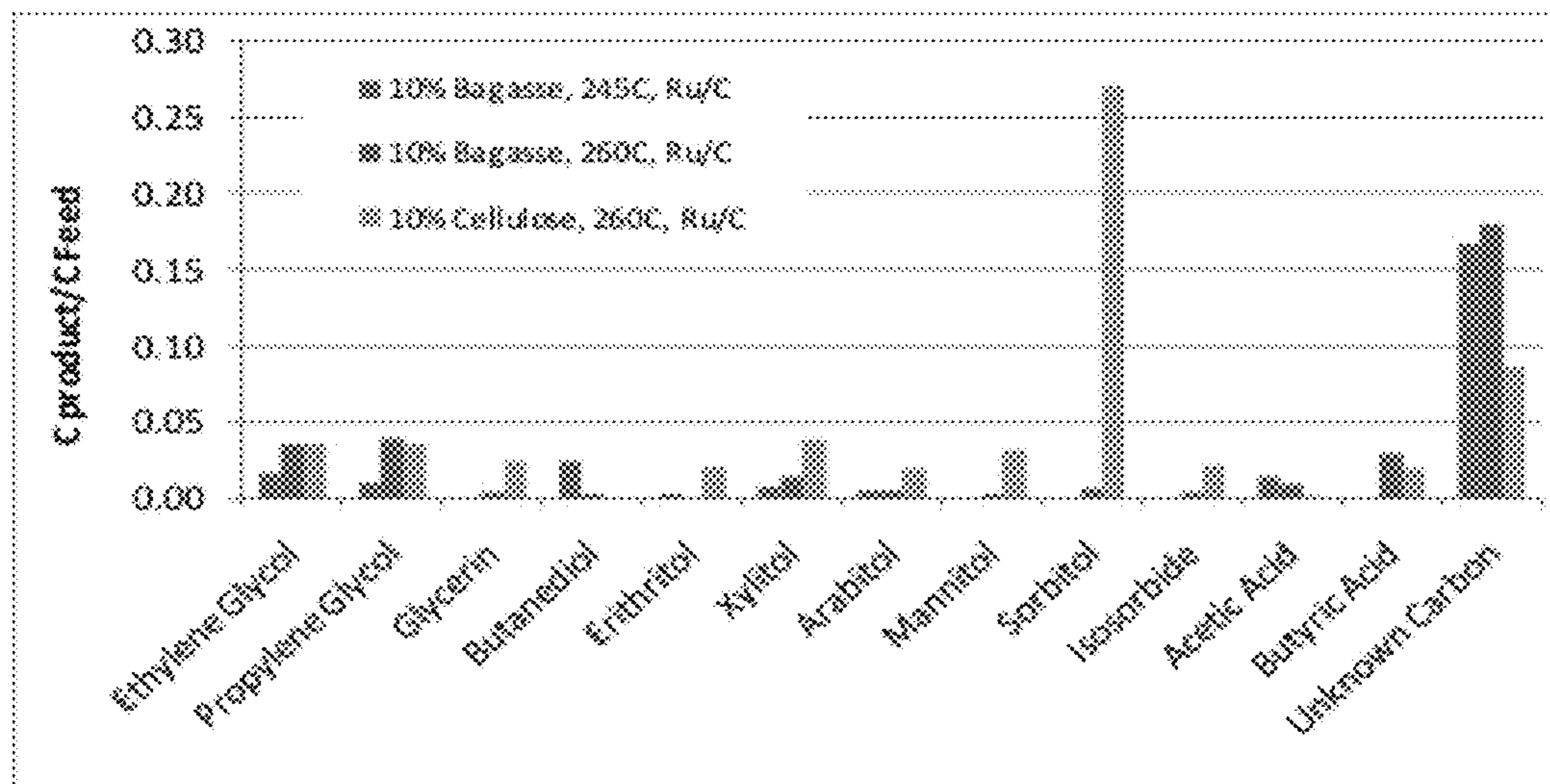
Figure 9. Product yields comparing bagasse and MCC conversion using Ru/C catalyst.
