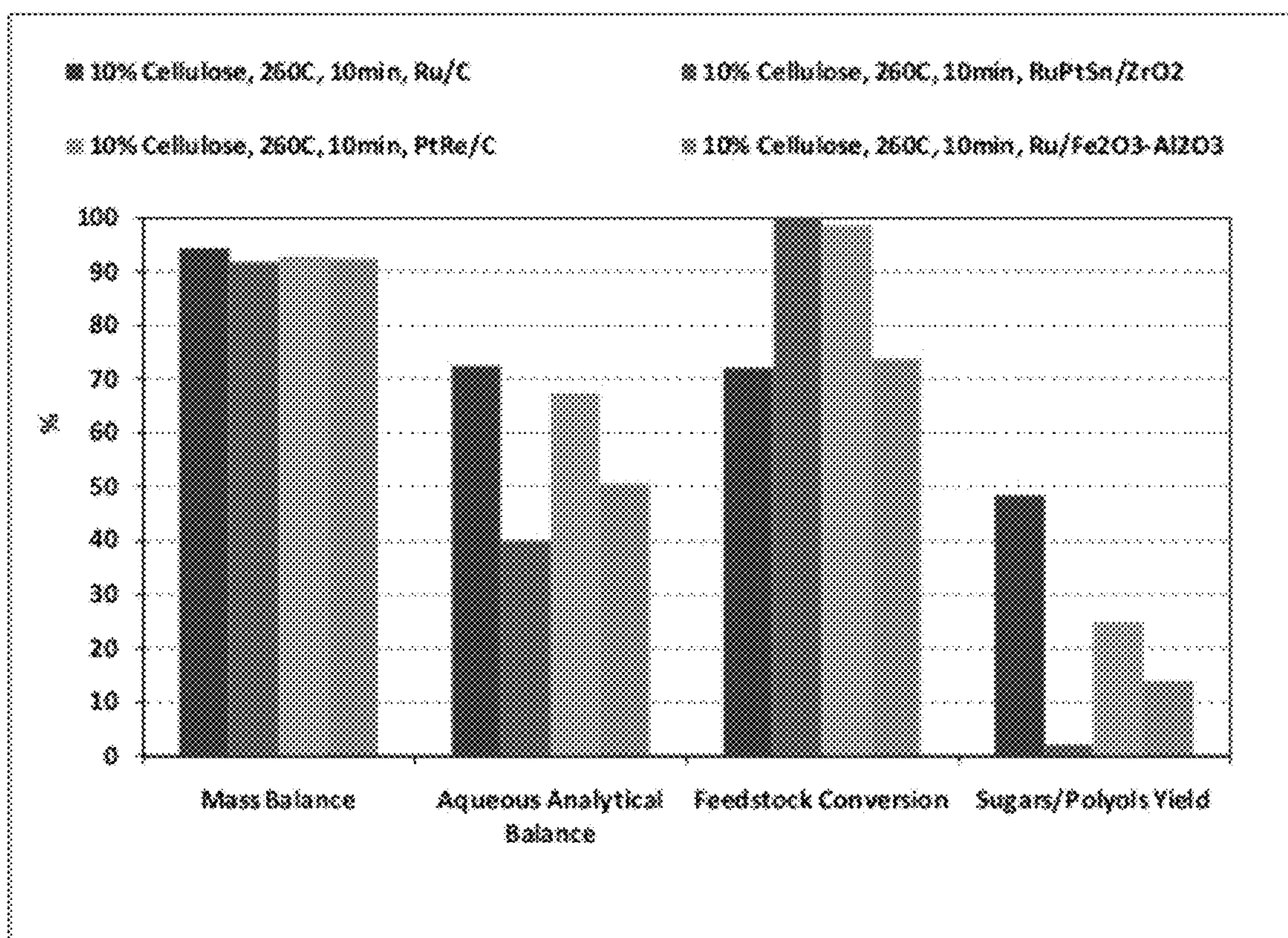
Figure 6. Conversion of MCC using various deconstruction catalysts
