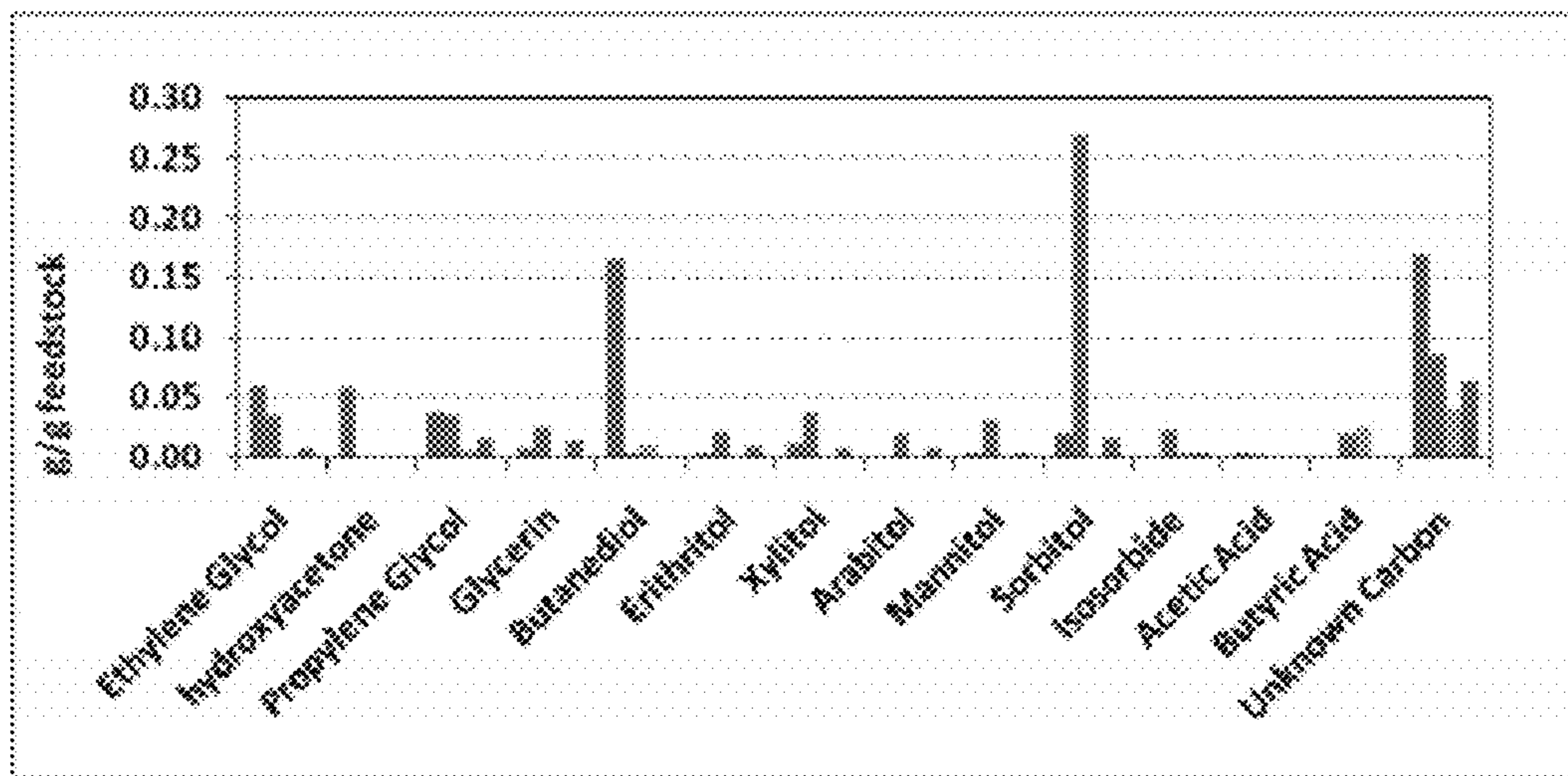
Figure 15: Products of hydrogenolysis of microcrystalline cellulose with different catalysts.
