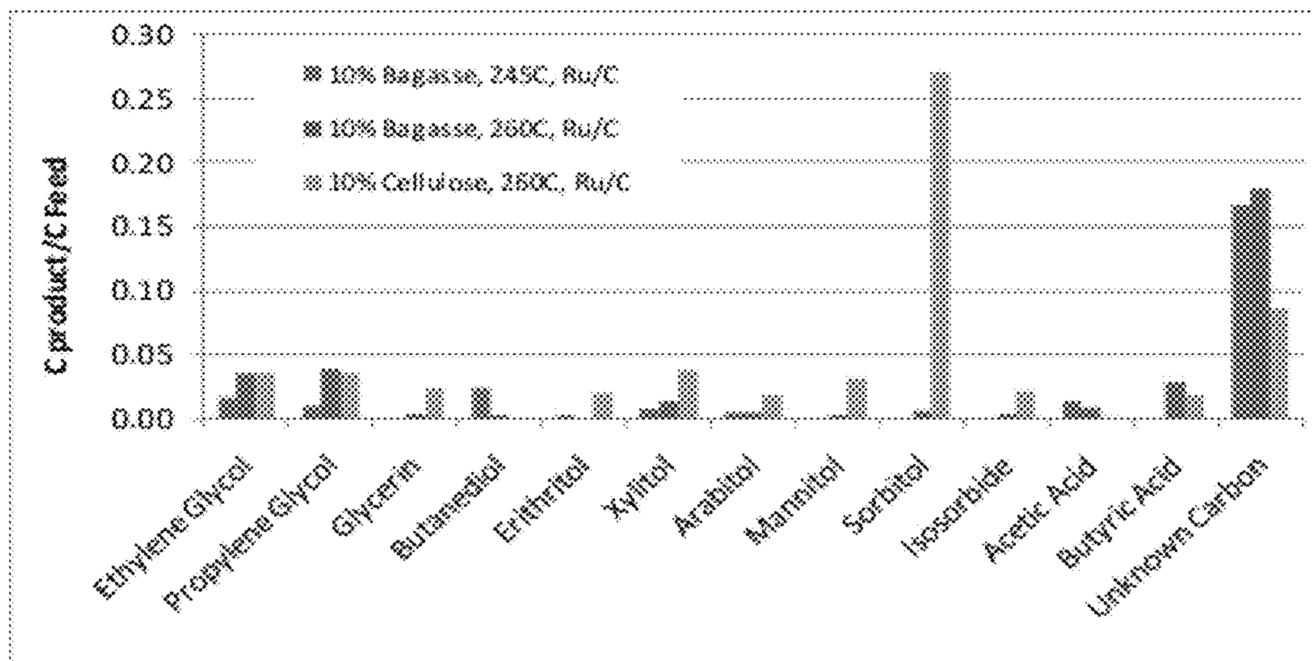
Figure 8. Comparison of bagasse conversion and MCC conversion using Ru/C catalyst.
