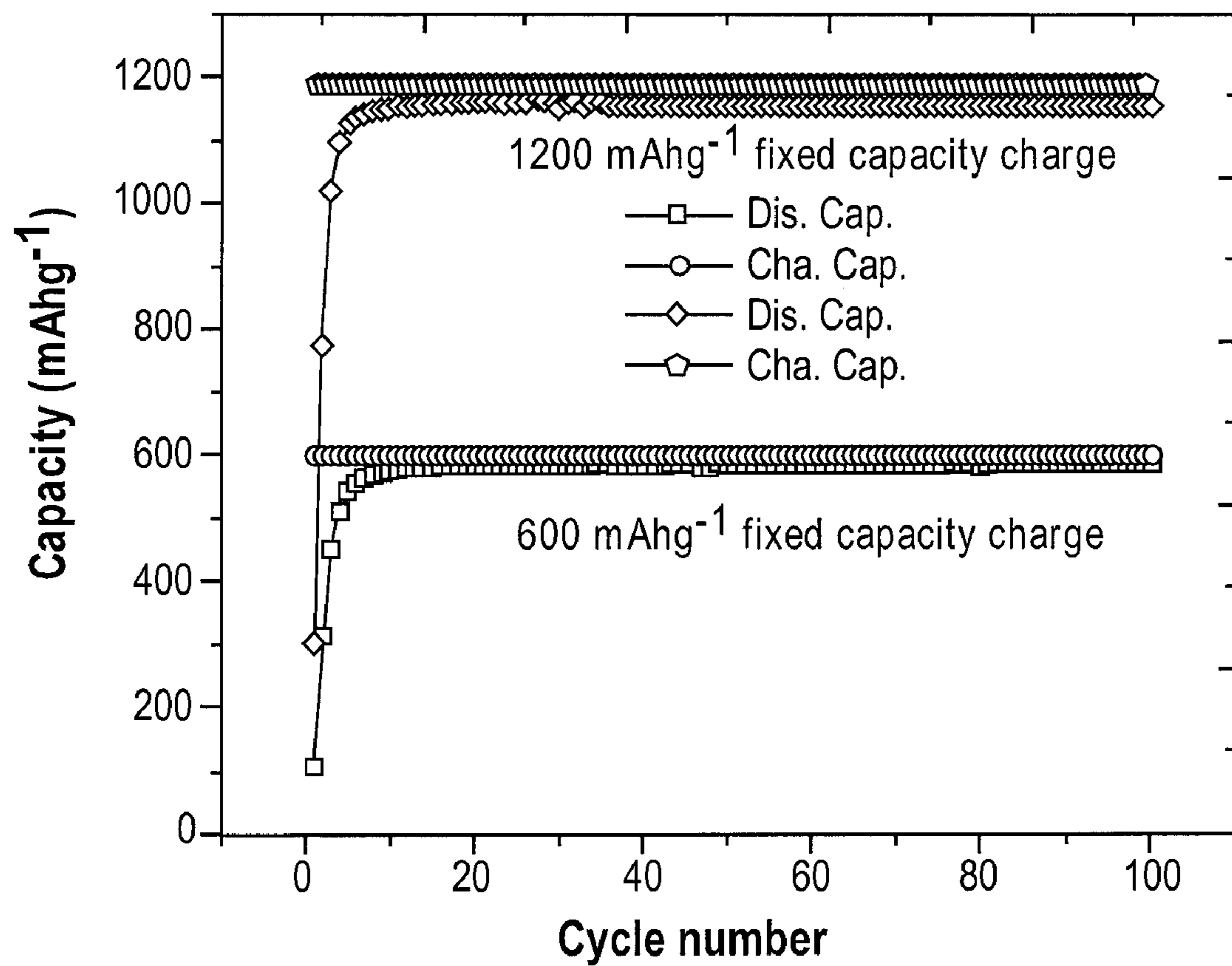
Si electrode cycling behavior at fixed capacity.
