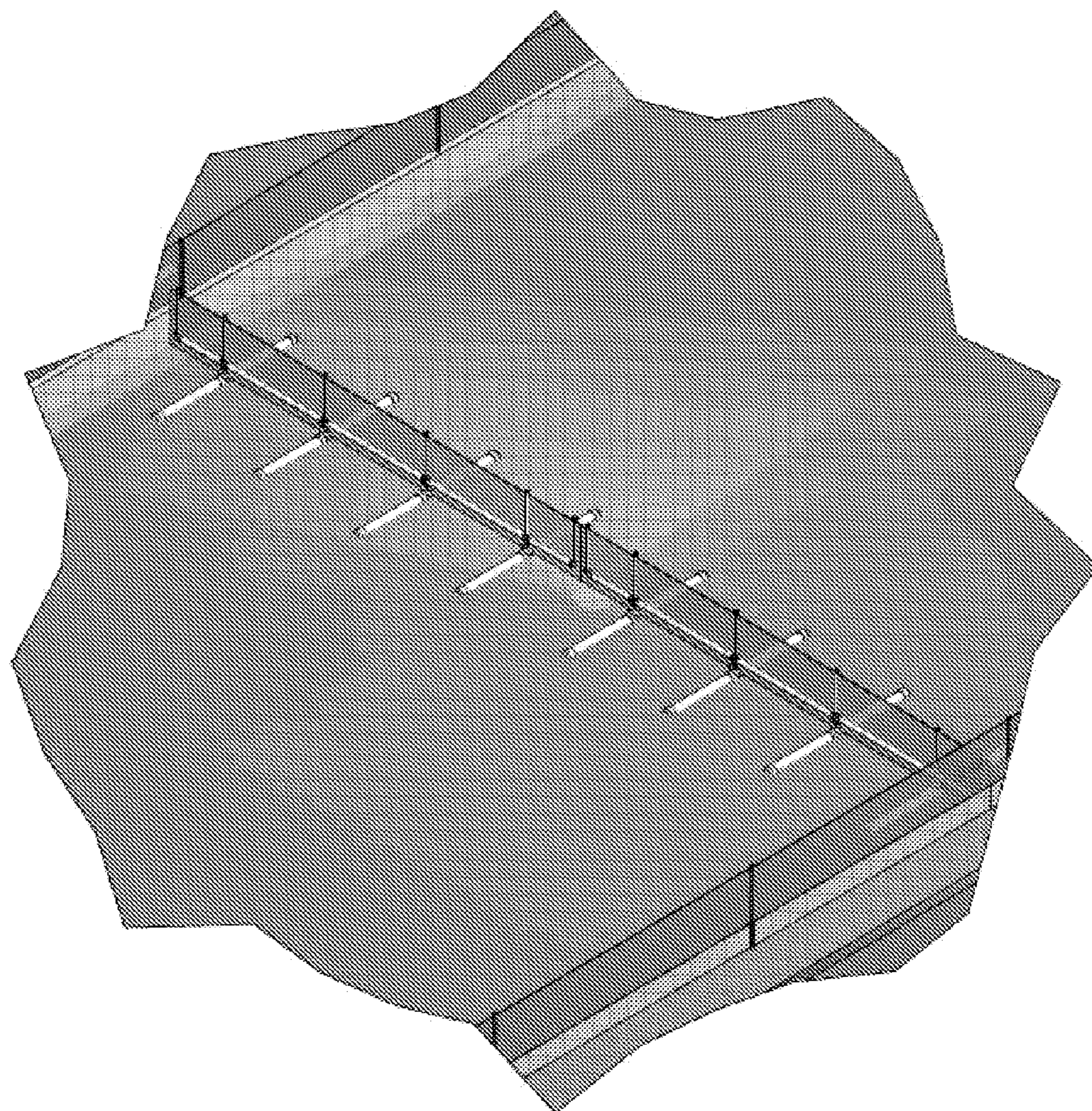
DETAIL C SCALE 1 / 75 Floating Windbreaks
