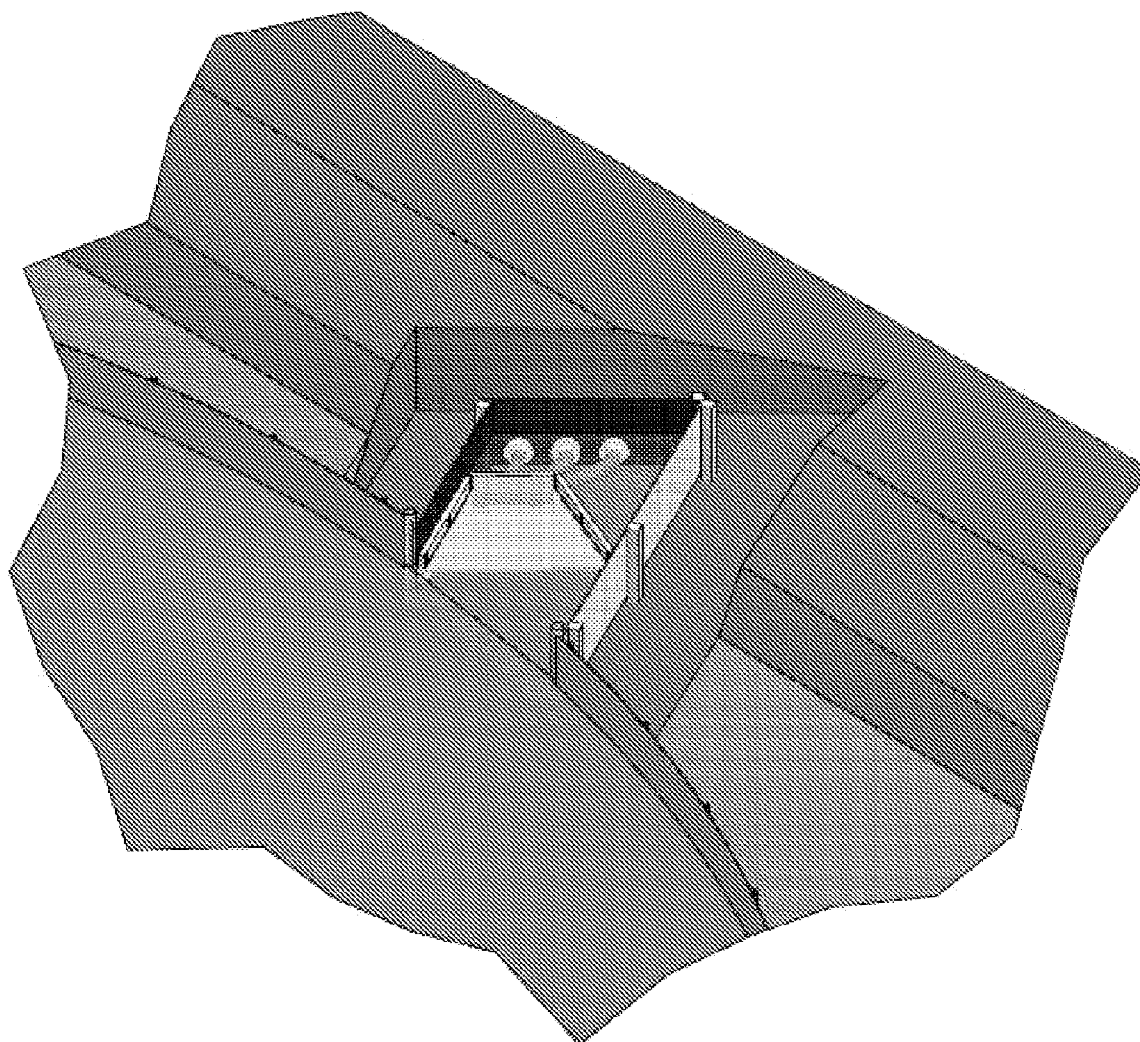
DETAIL D SCALE 1 / 75 Floating Harvesting Skimmer
